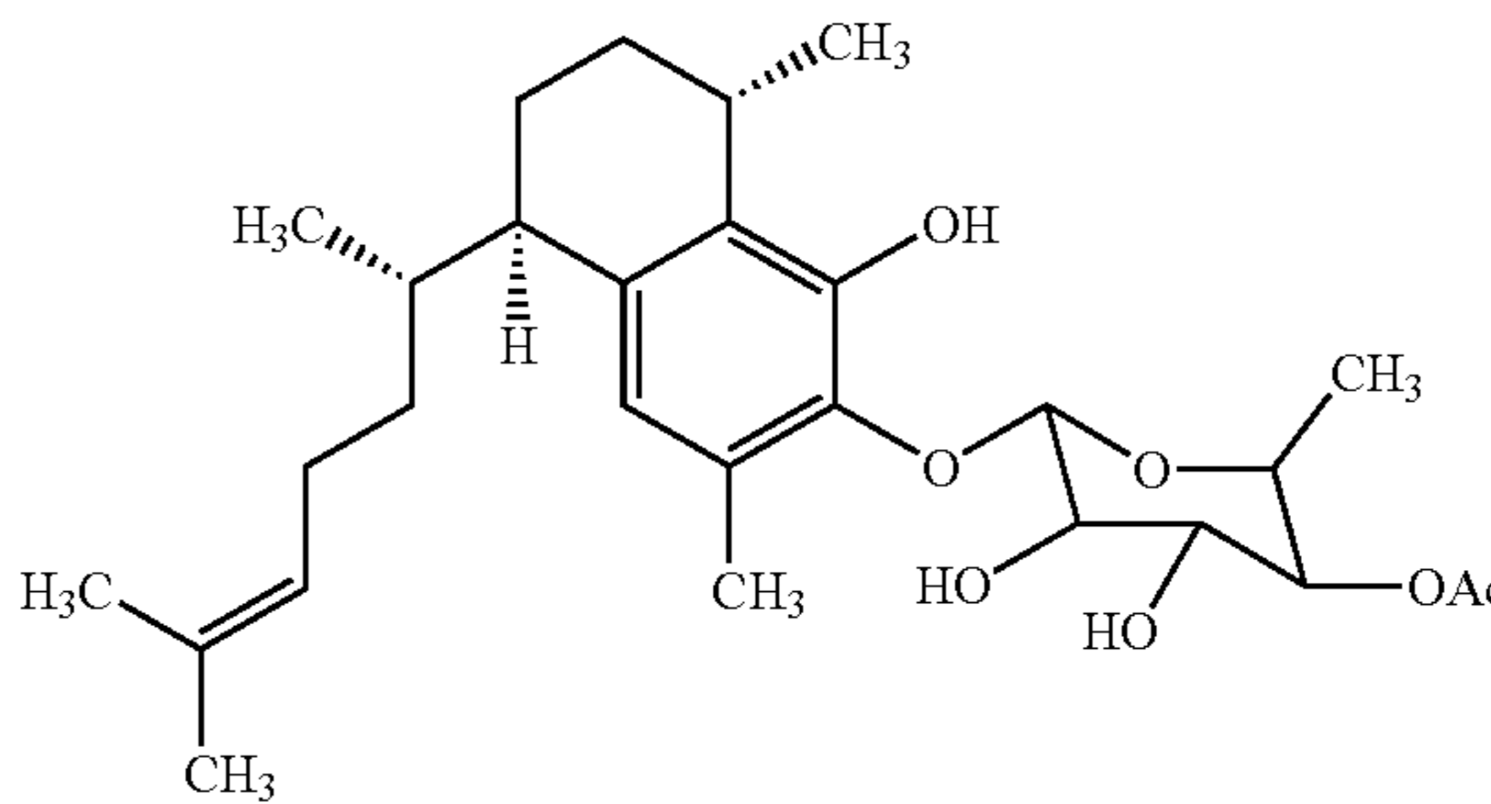
Seco-pseudopterosin G
