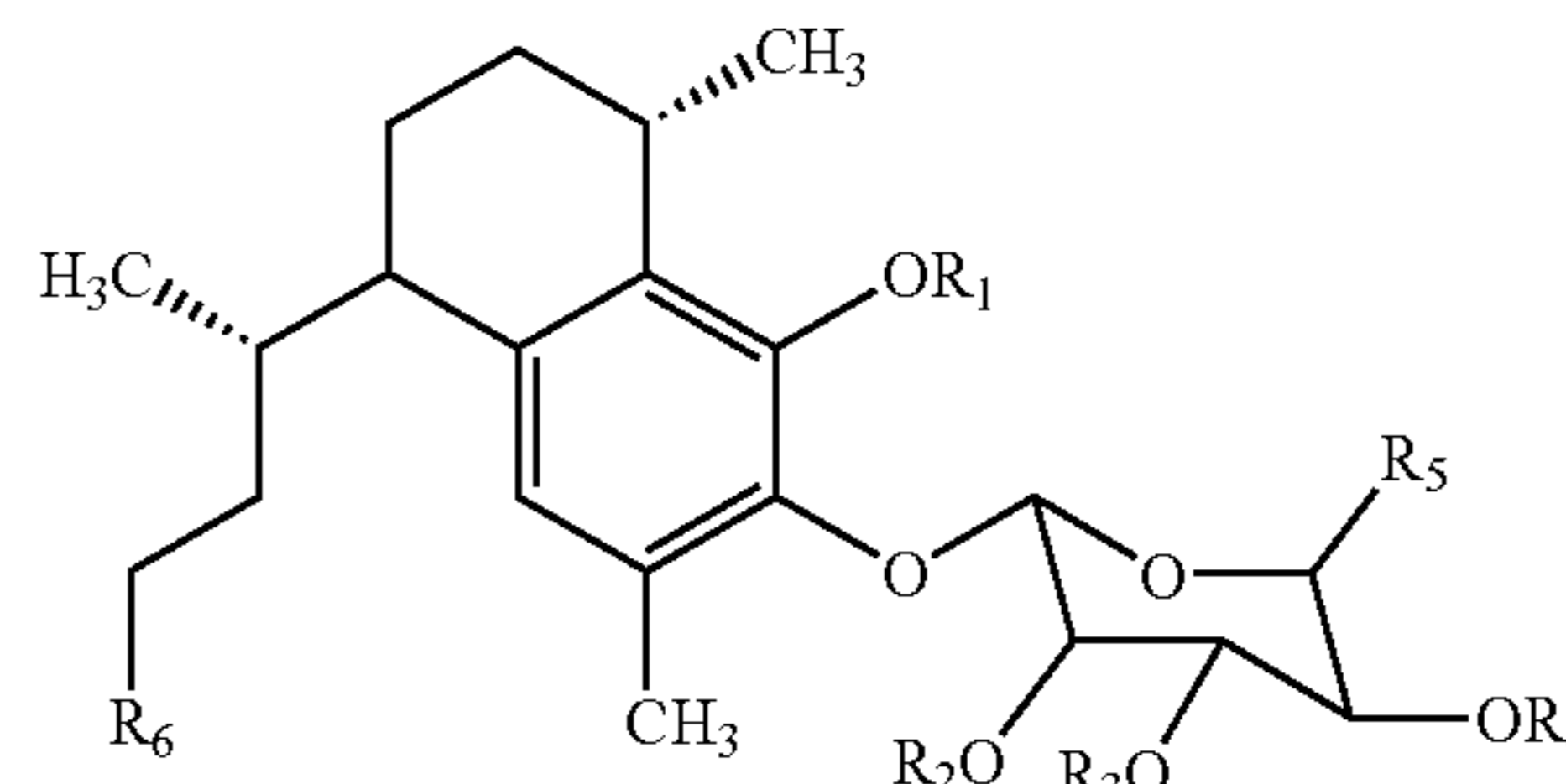
Structural Formula 2
