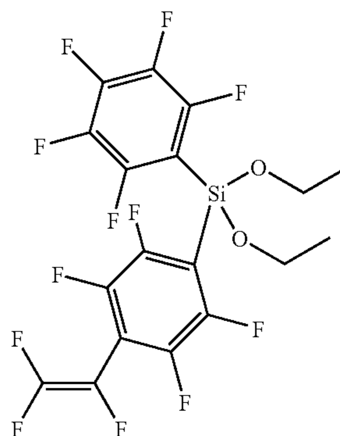
Perfluorostyreneperfluorotoluenediethoxy-silane
