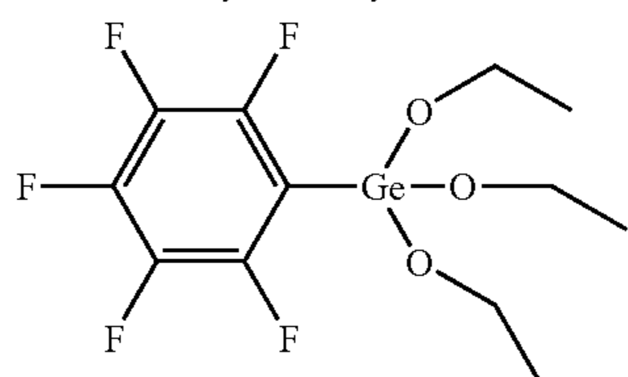
Pentafluorophenyltriethoxygermane
