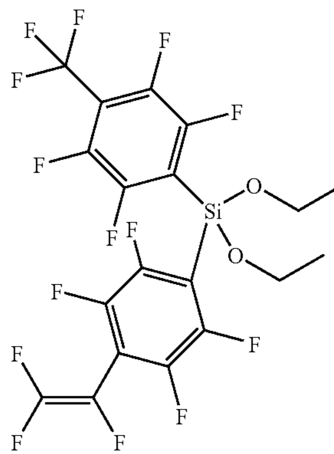
Perfluorostyreneperfluorotoluenediethoxy-silane
