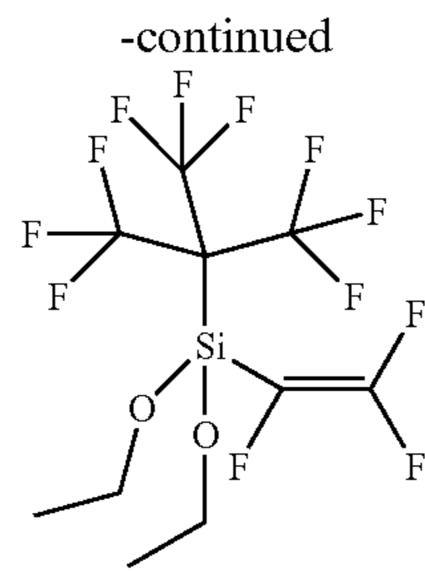
Perfluoro(t-butyl)trifluorovinyl-diethoxysilane
