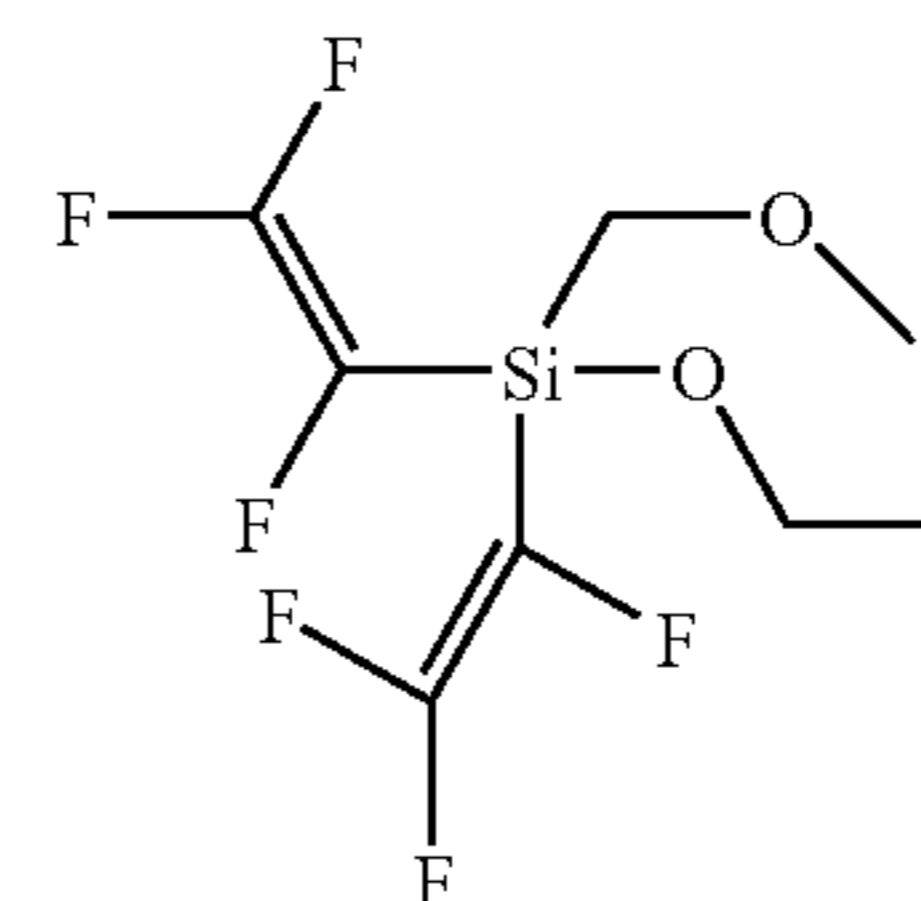
Bis(trifluorovinyl) diethoxysilane
