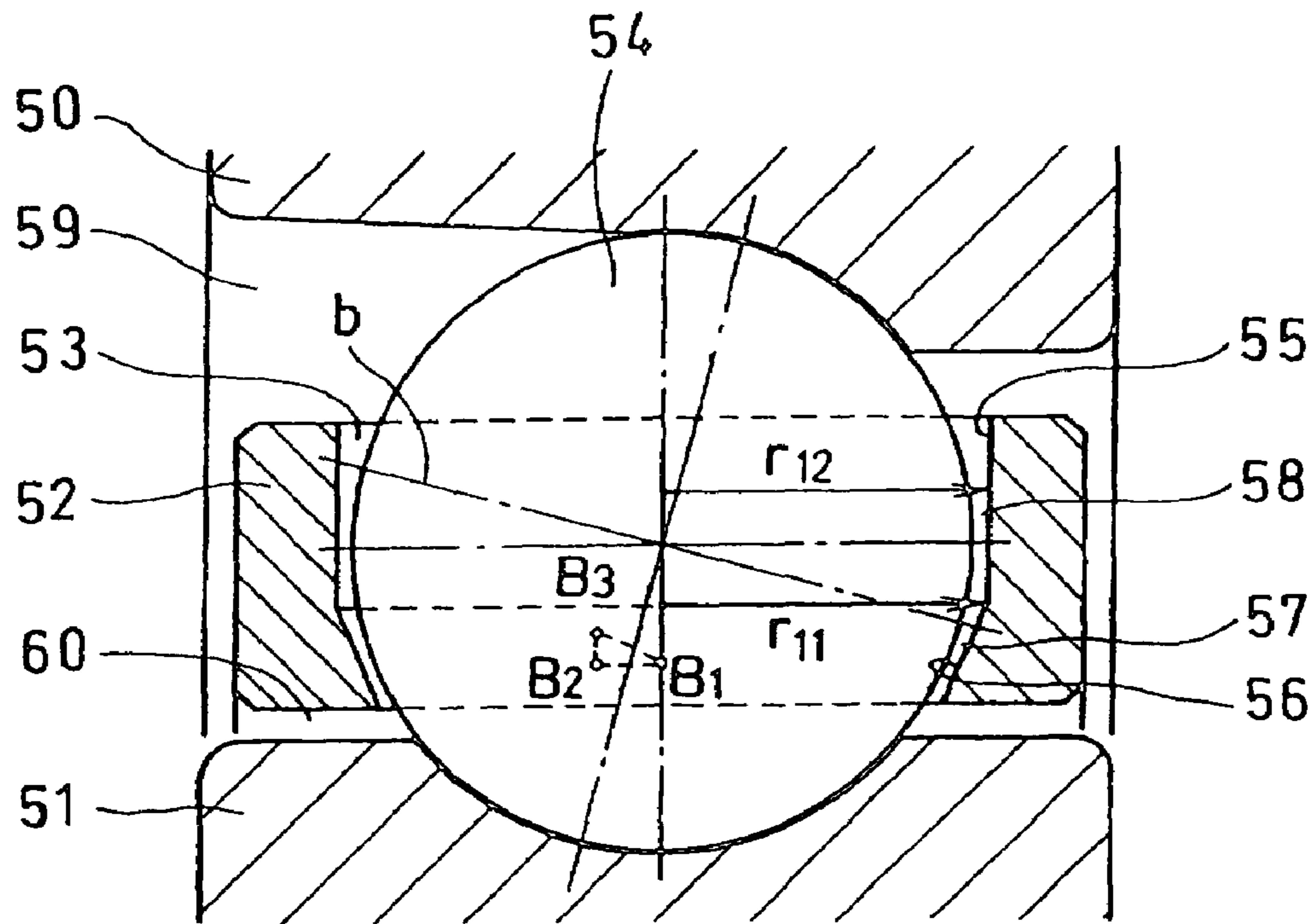
Fig.16 PRIOR ART
