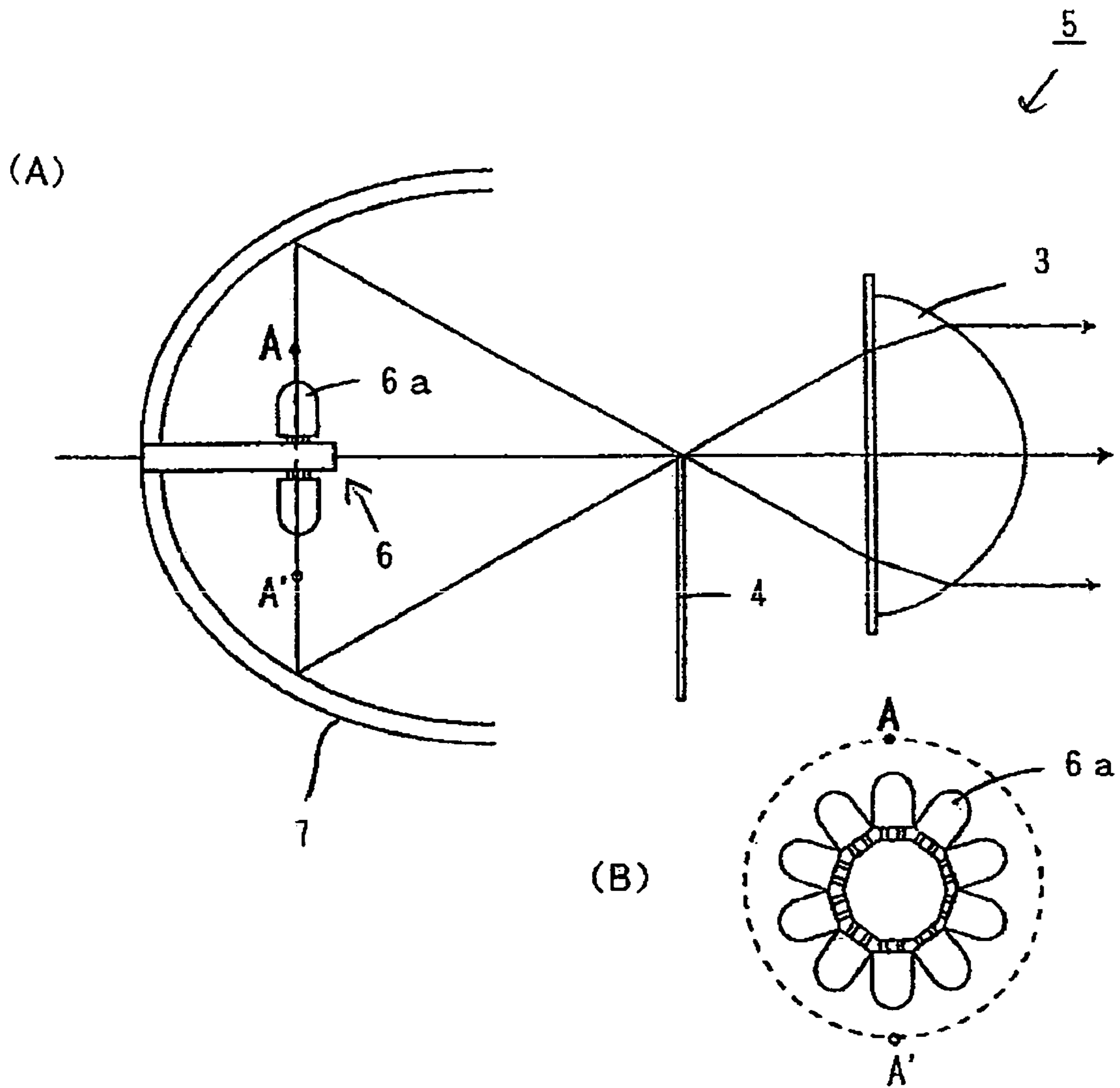
Fig. 27 Conventional Art
