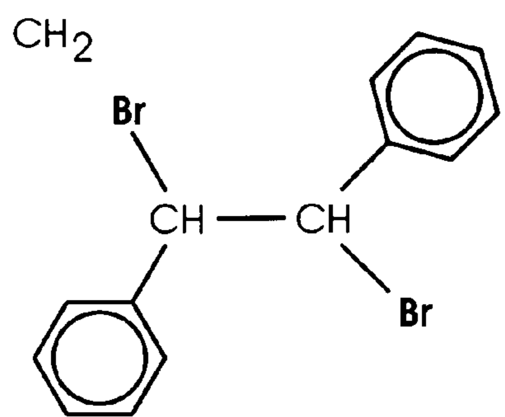
DBDE dibromodiphenylethane
