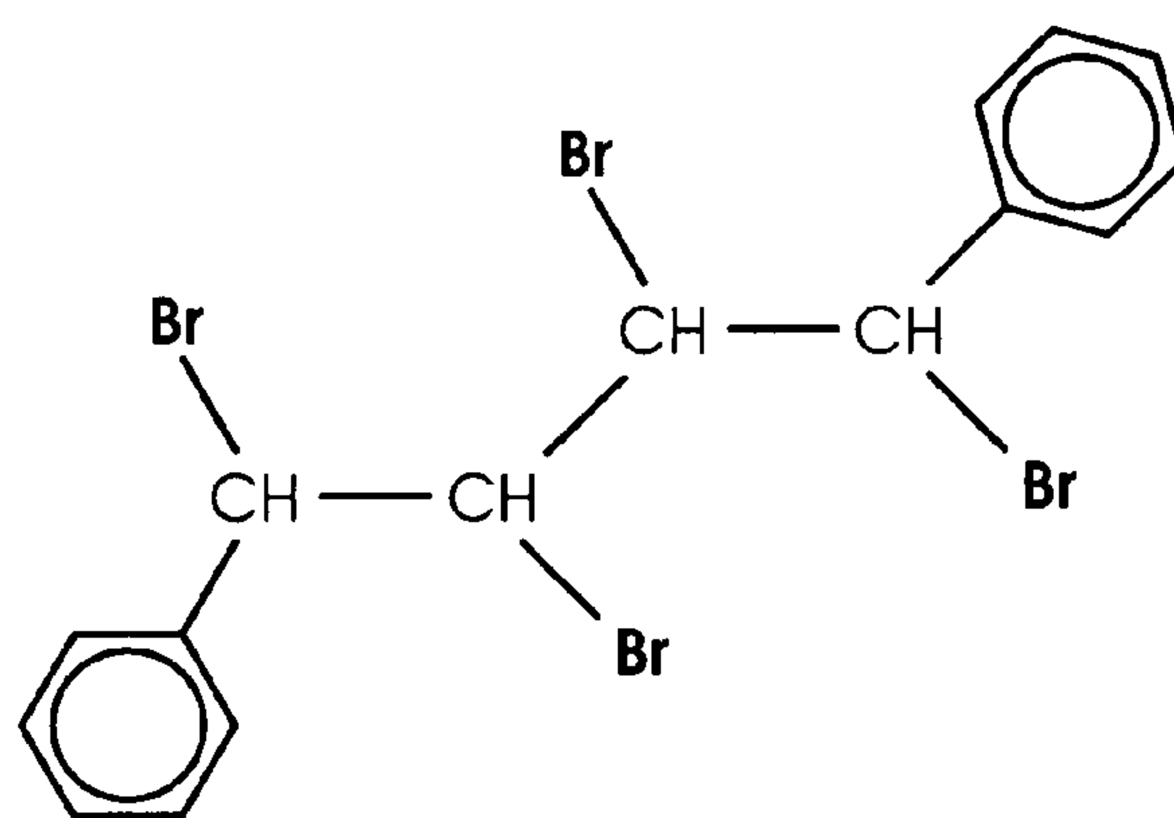
TBDB tetrabromodiphenylbutane
