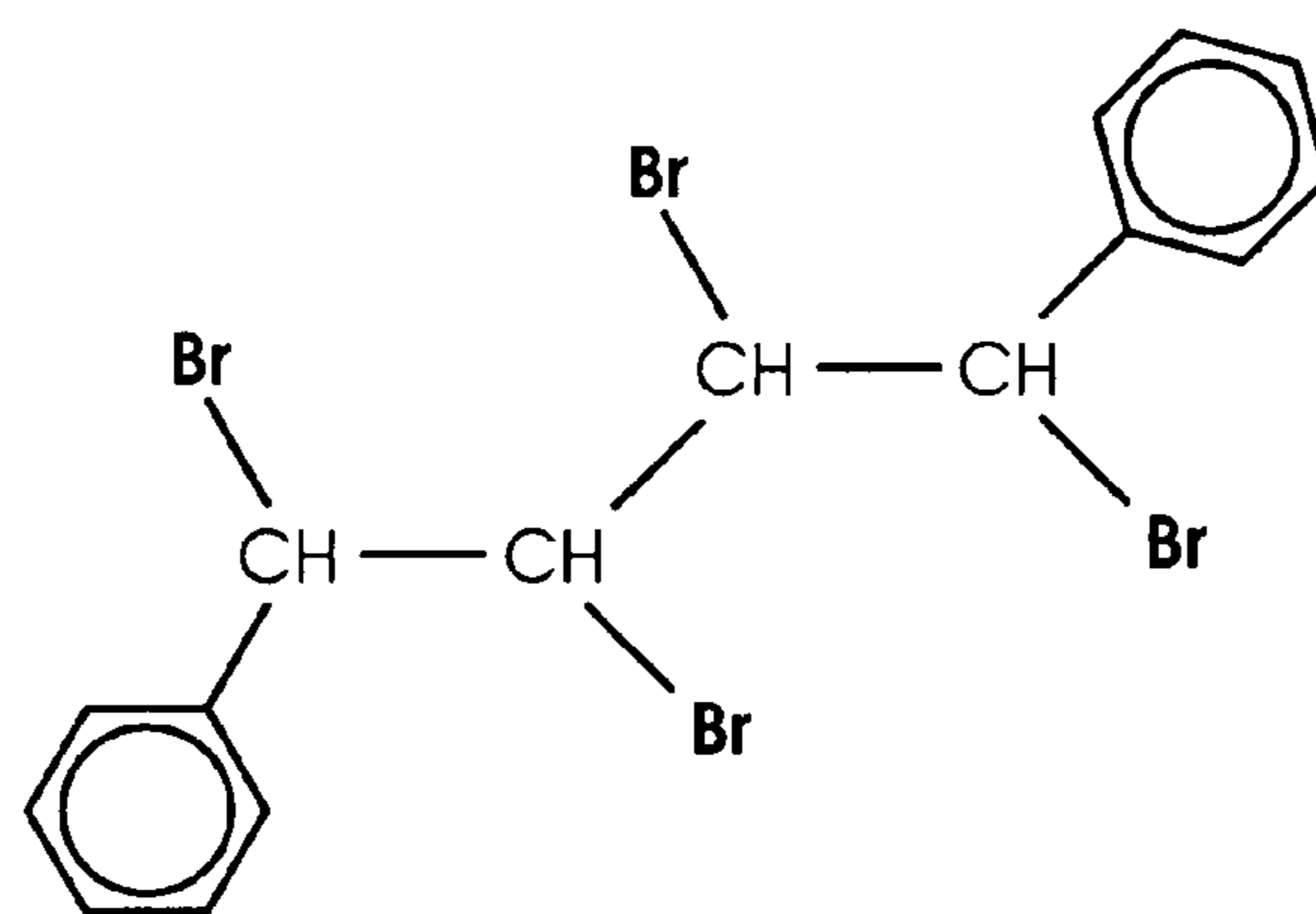
TBDB tetrabromodiphenylbutane
