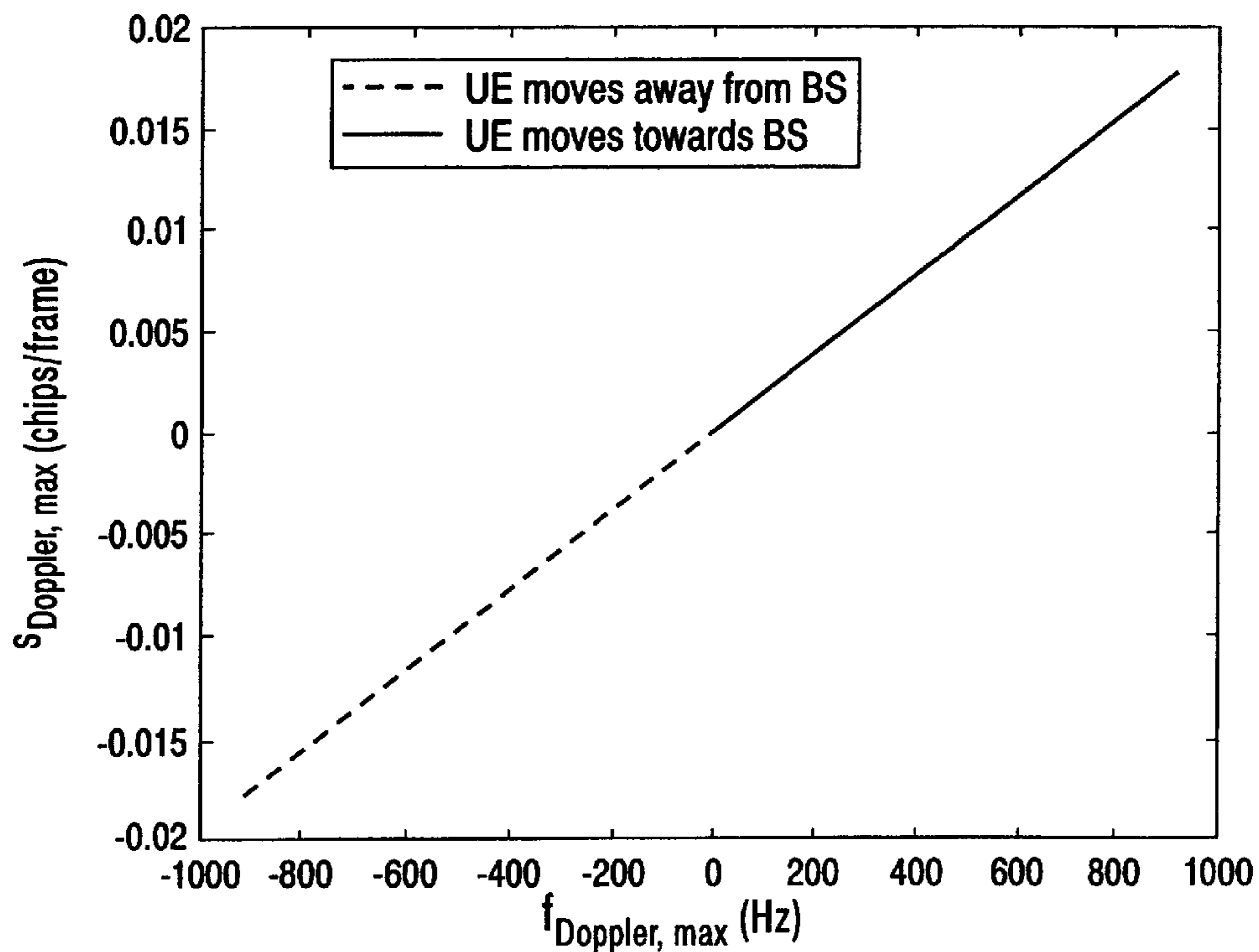
Fig. 10 Maximum Doppler Delay Shift S_{Doppler, max} as a Function of Doppler Frequency f_{Doppler, max}
