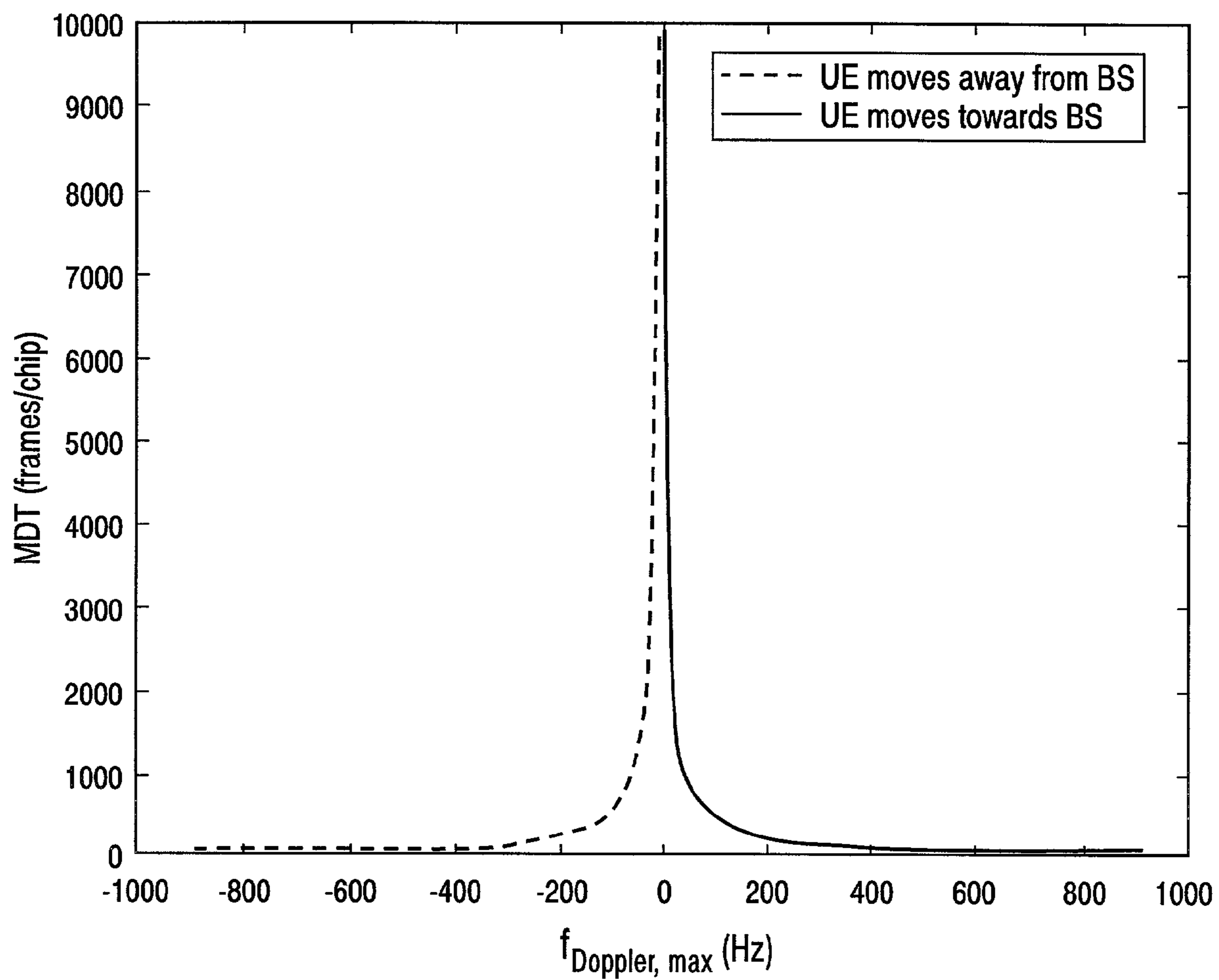
Fig. 11 Minimum Dwell Time as a Function of Doppler Frequency f_{Doppler, max}
