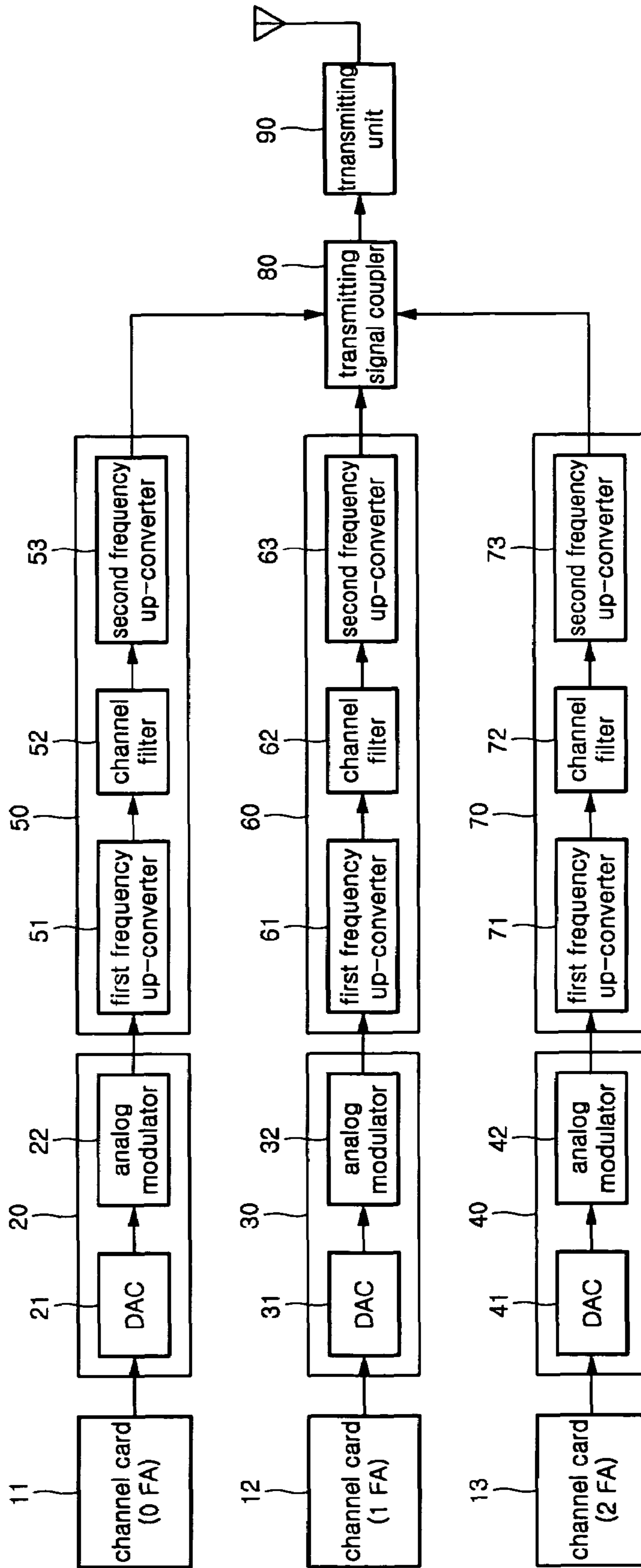
FIG. 2 (PRIOR ART)
