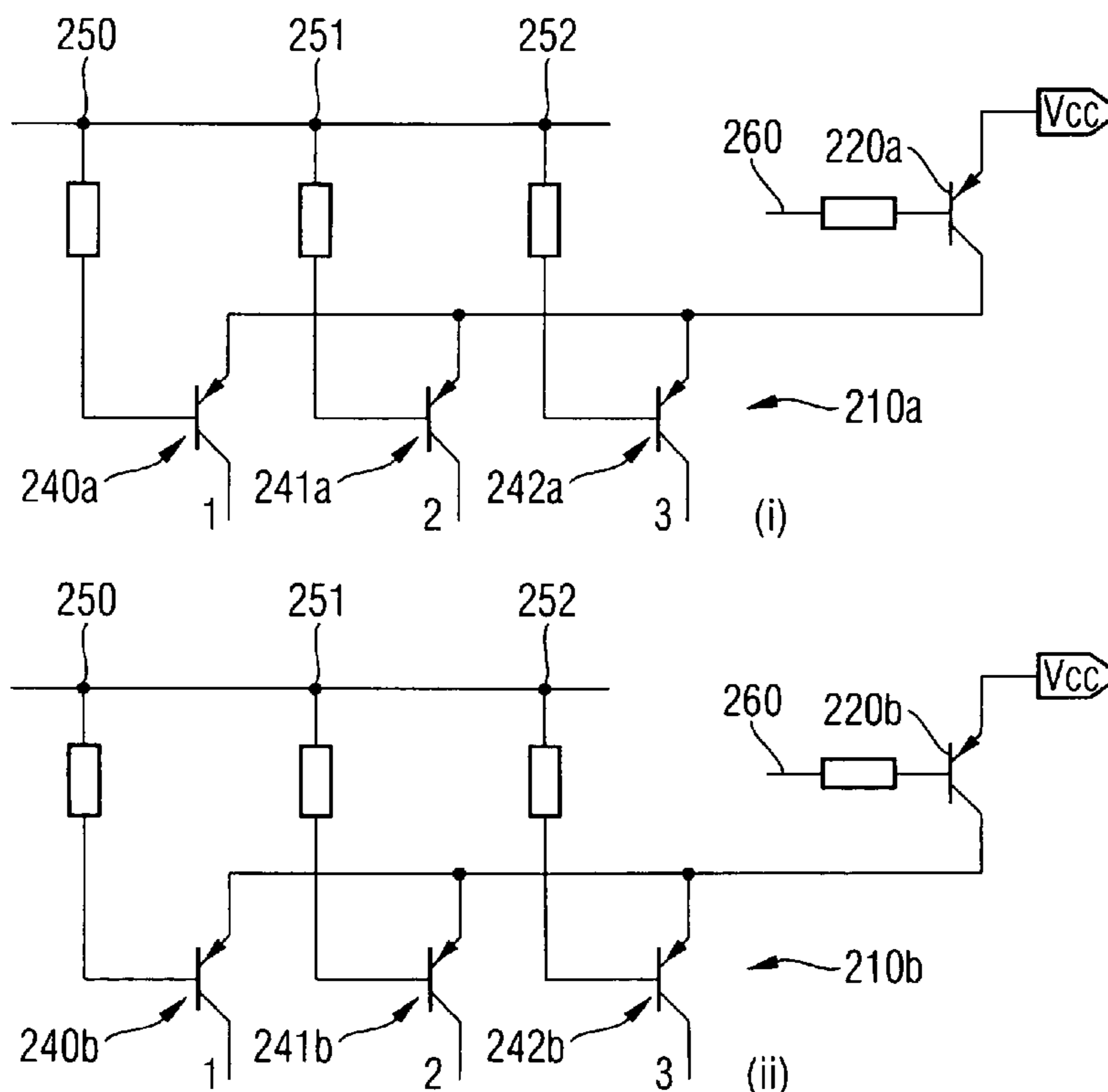
Row Decoding for output lines 1-4
