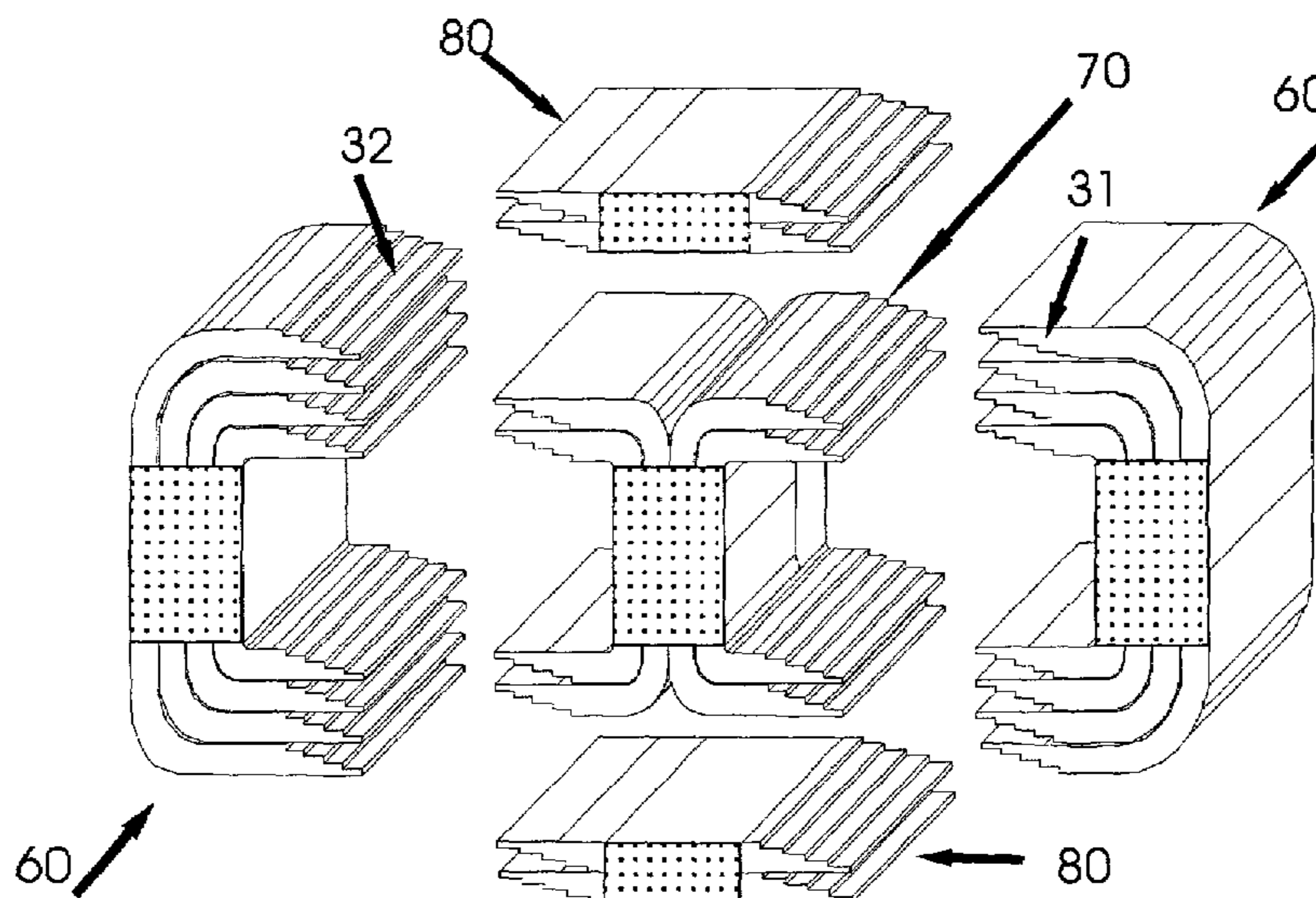
3 Phase / 3 Leg Transformer Core (110)
