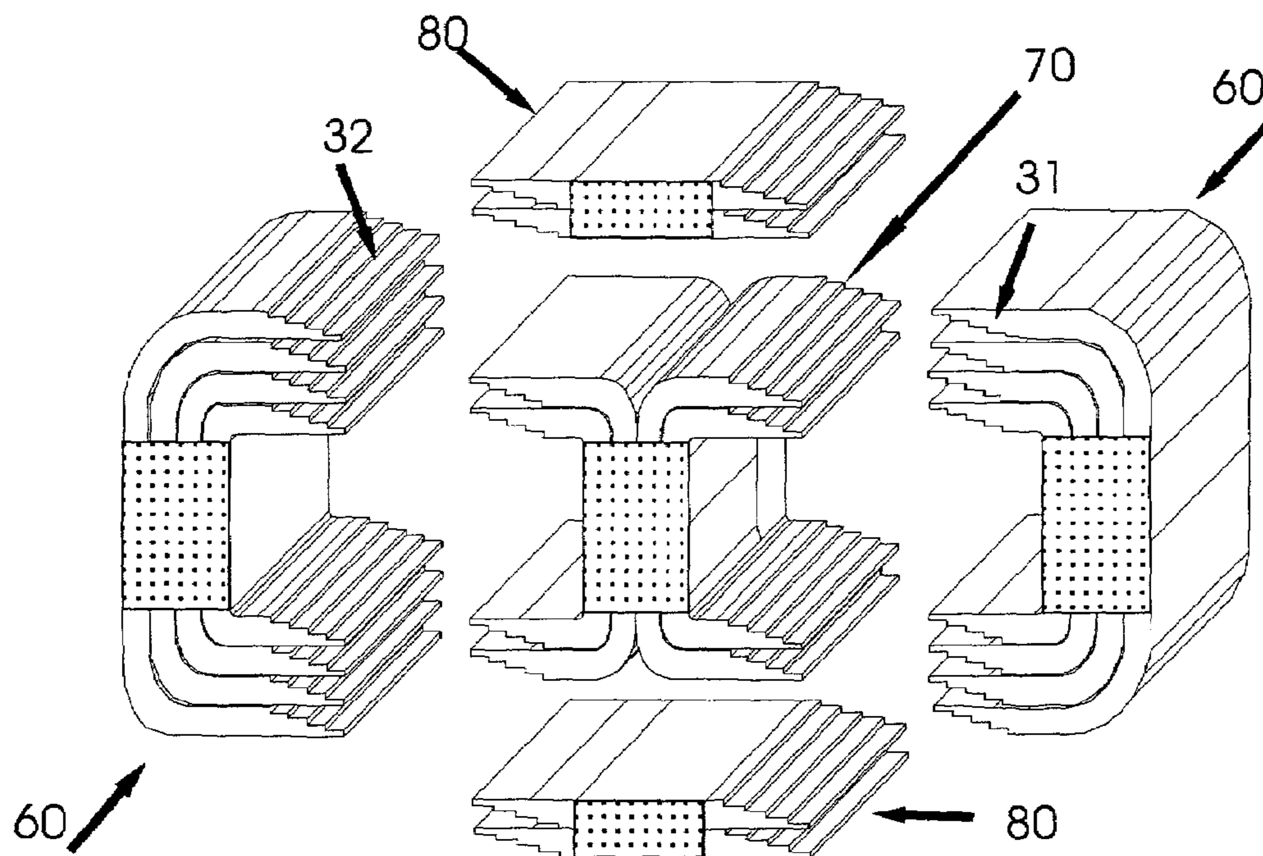
3 Phase / 3 Leg Transformer Core (110)
