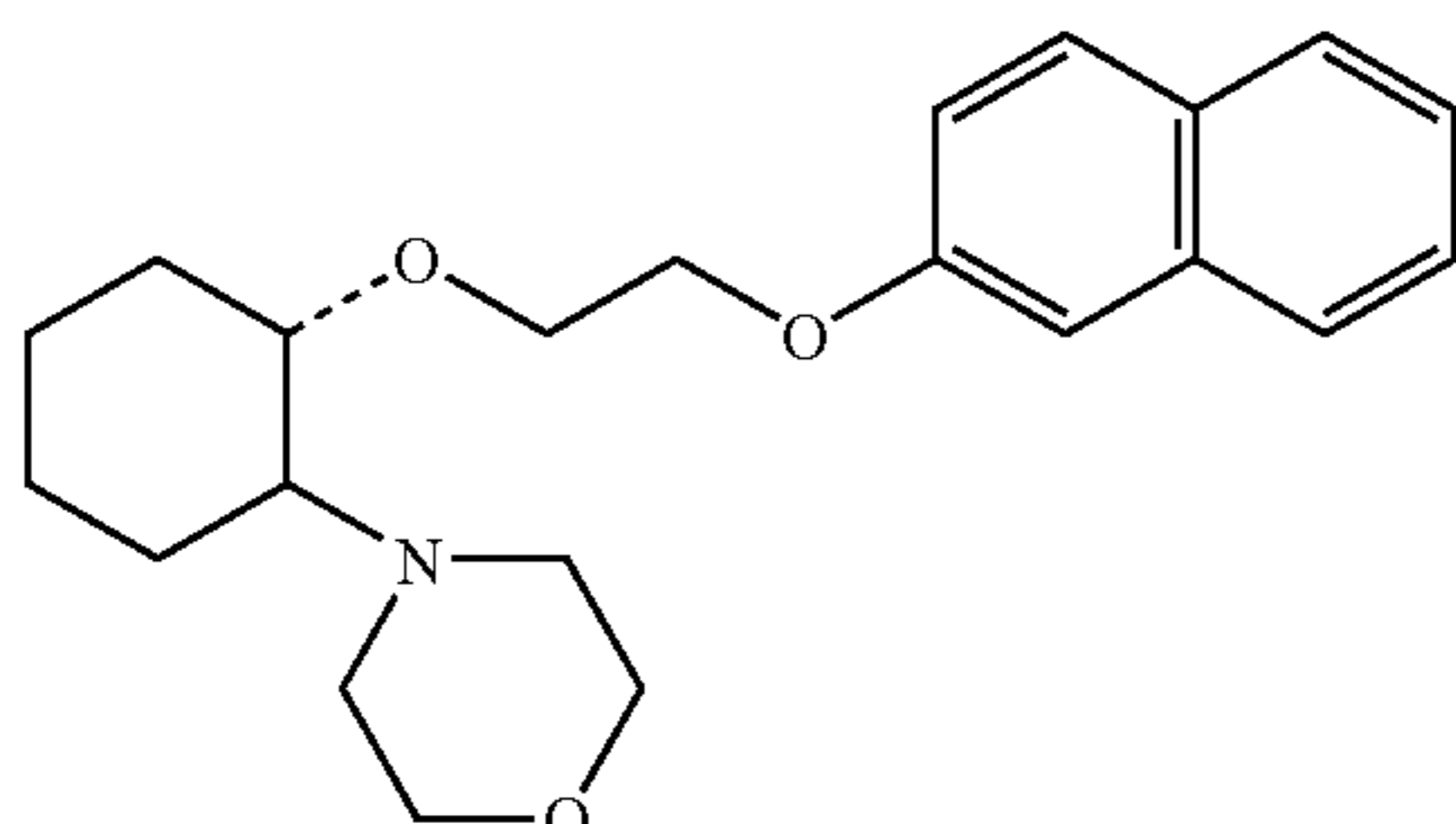
(1R, 2R)/(1S, 2S)-[2-(4-morpholinyl)-1-[2-(2-naphthoxy)ethoxy]]cyclohexane
