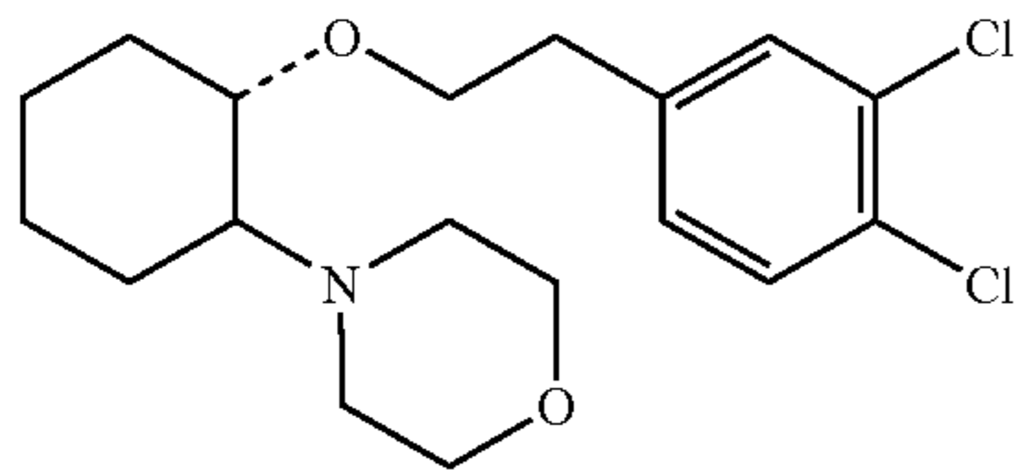
(1R, 2R)/(1S, 2S)-2-(4-morpholinyl)-1-(3,4-dichlorophenethoxy)cyclohexane
