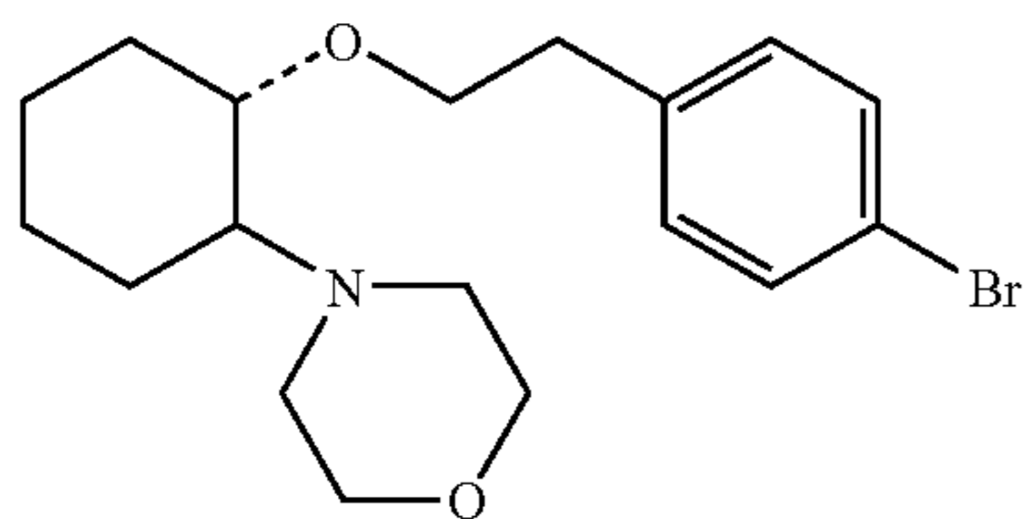
(1R, 2R)/(1S, 2S)-[2-(4-morpholinyl)-1-(4-bromophenethoxy)]cyclohexane
