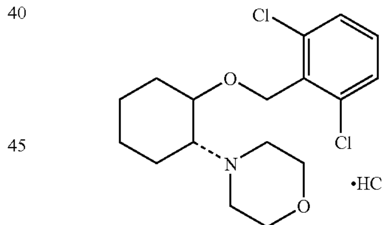
(1R, 2R)/(1S, 2S)-2-(4-morpholinyl)-1-[(2,6-dichlorophenyl)methoxy]cyclohexane monohydrochloride
