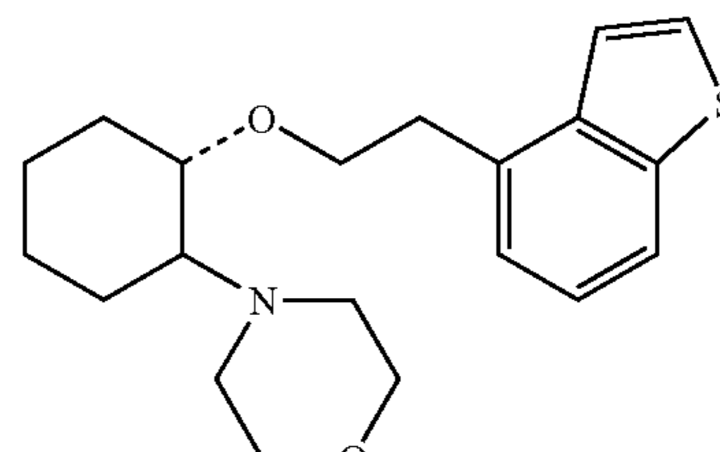
(1R, 2R)/(1S, 2S)-[2-(4-morpholinyl)-1-(2-benzo[b]thiophen-4-yl)]cyclohexane
