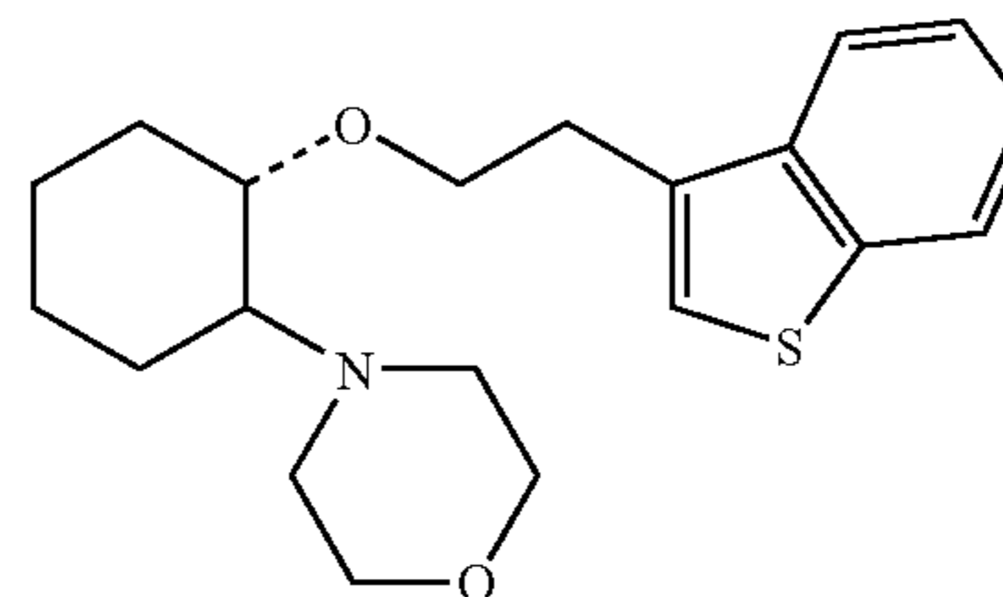
(1R, 2R)/(1S, 2S)-[2-(4-morpholinyl)-1-(2-benzo[b]thiophen-3-yl)]cyclohexane
