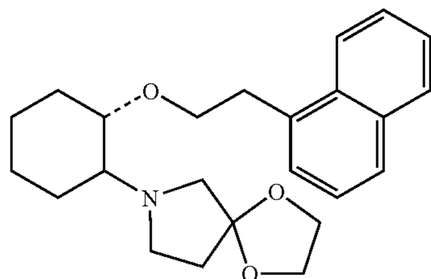
(1R, 2R)/(1S, 2S)-2-[1,4-dioxo-7-azaspiro[4.4]non-7-yl]-1-(1-naphthenethoxy)cyclohexane
