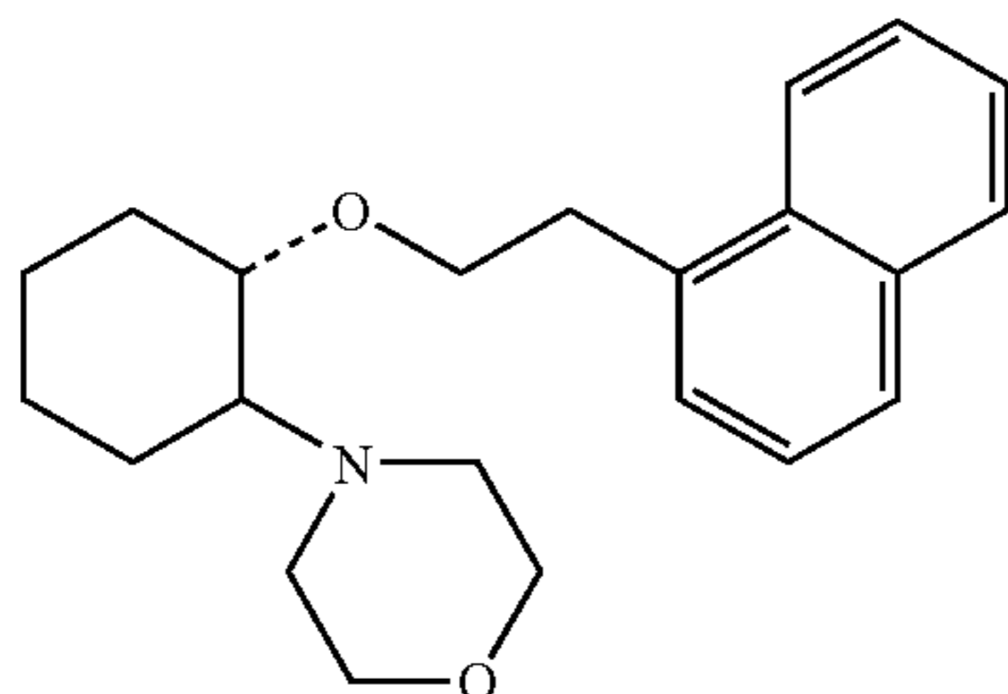
(1R, 2R)/(1S, 2S)-[2-(4-morpholinyl)-1-(1-naphthenethoxy)]cyclohexane
