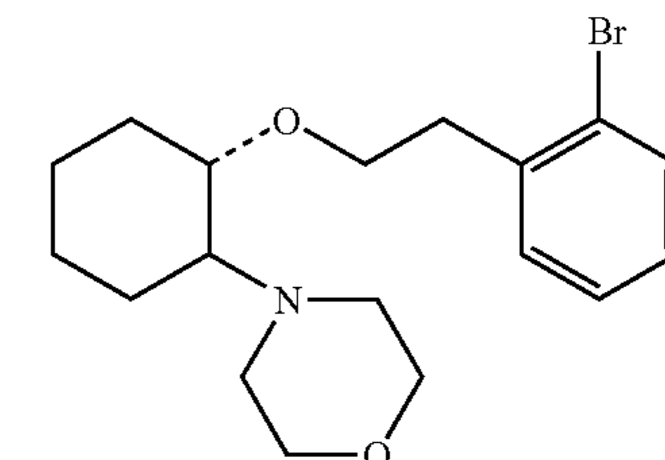
(1R, 2R)/(1S, 2S)-[2-(4-morpholinyl)-1-(2-bromophenethoxy)]cyclohexane
