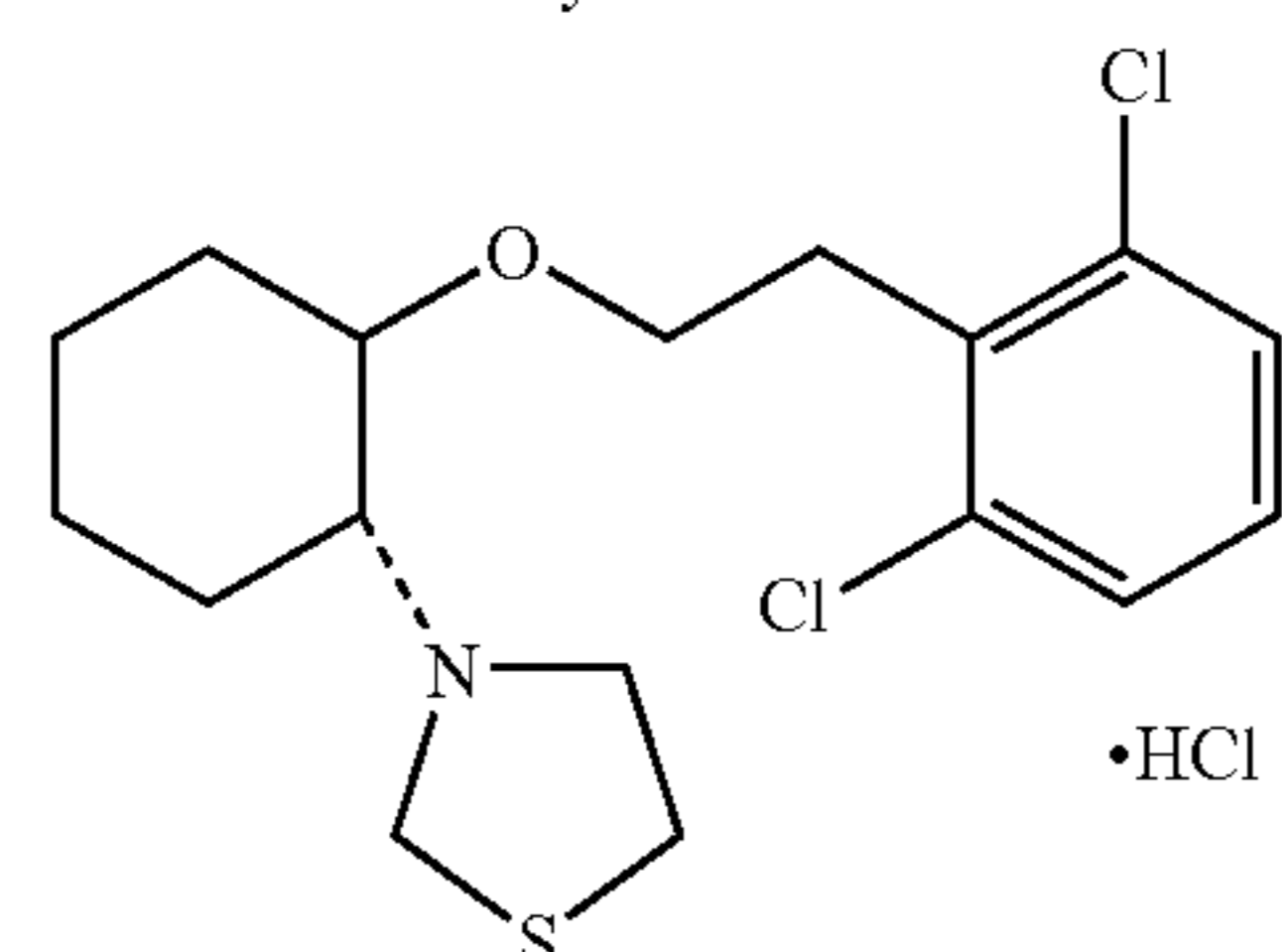
(1R, 2R)/(1S, 2S)-2-(3-thiazolidinyl)-1-(2,6-dichlorophenoxy)cyclohexane monohydrochloride
