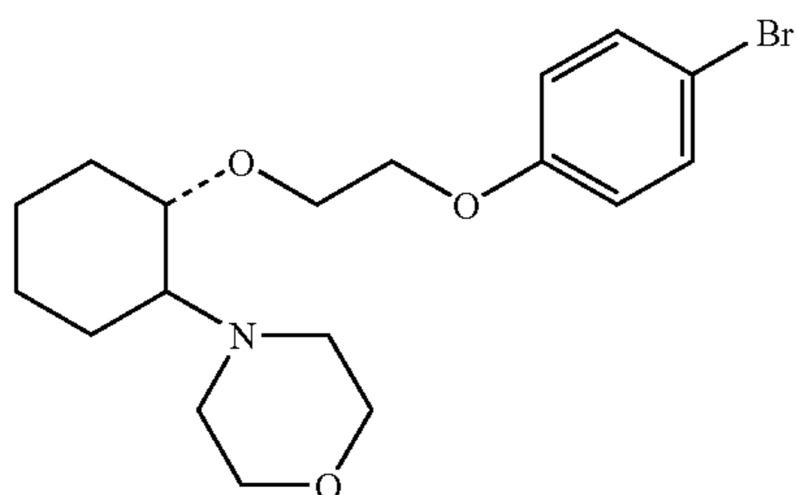
(1R, 2R)/(1S, 2S)-[2-(4-morpholinyl)-1-[2-(4-bromophenoxy)ethoxy]]cyclohexane
