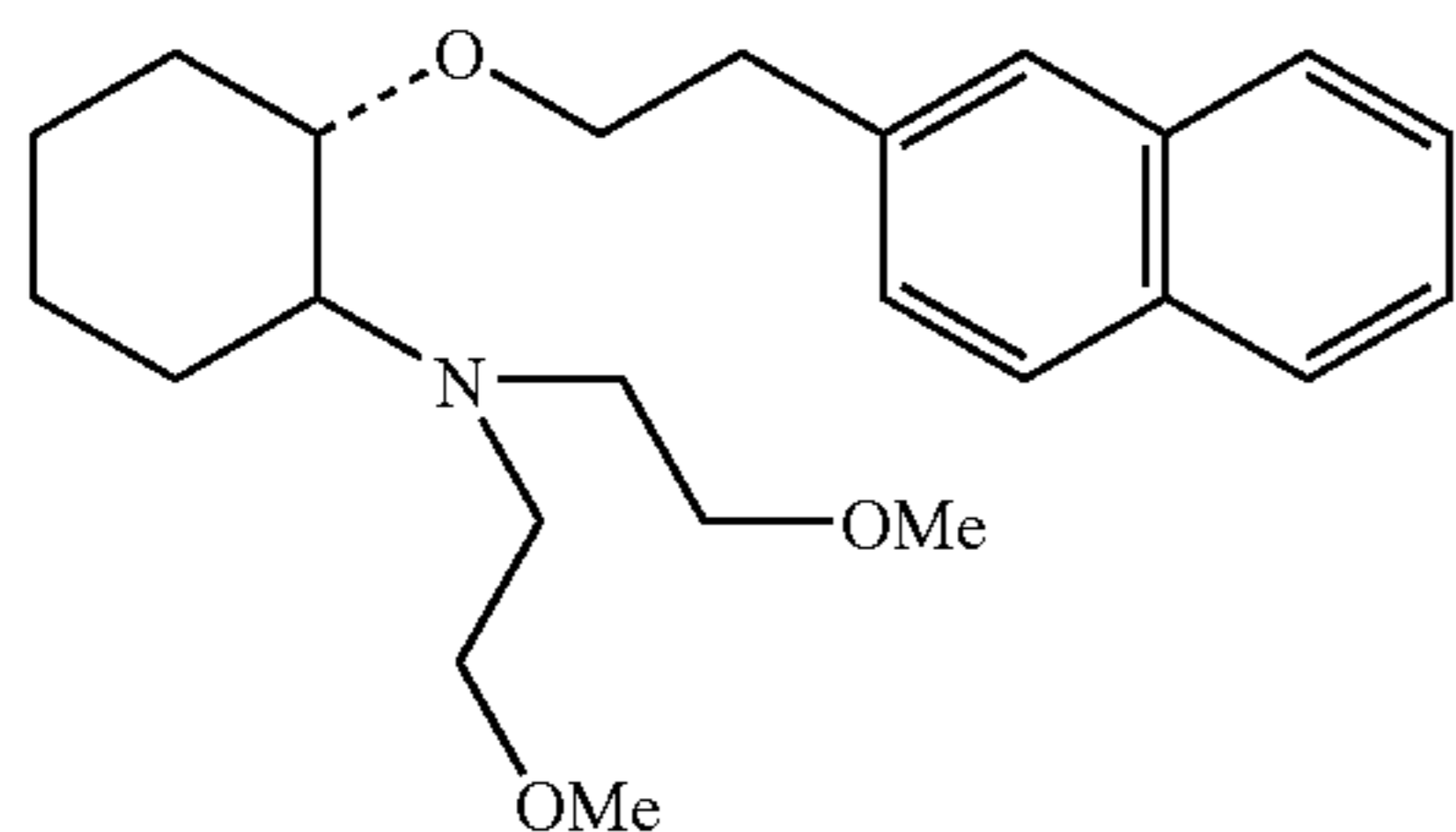
(1R, 2R)/(1S, 2S)-2-[bis(2-methoxyethyl)aminy]-1-(2-naphthenethoxy)cyclohexane
