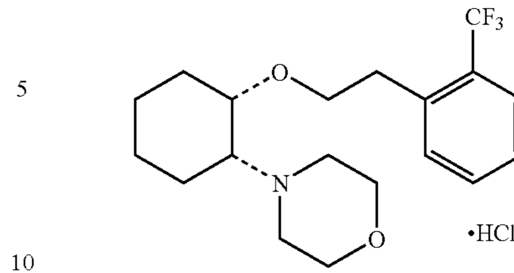
(1R, 2S)/(1S, 2R)-2-(4-morpholinyl)-1-[(2-trifluoromethyl)phenethoxy]cyclohexane monohydrochloride
