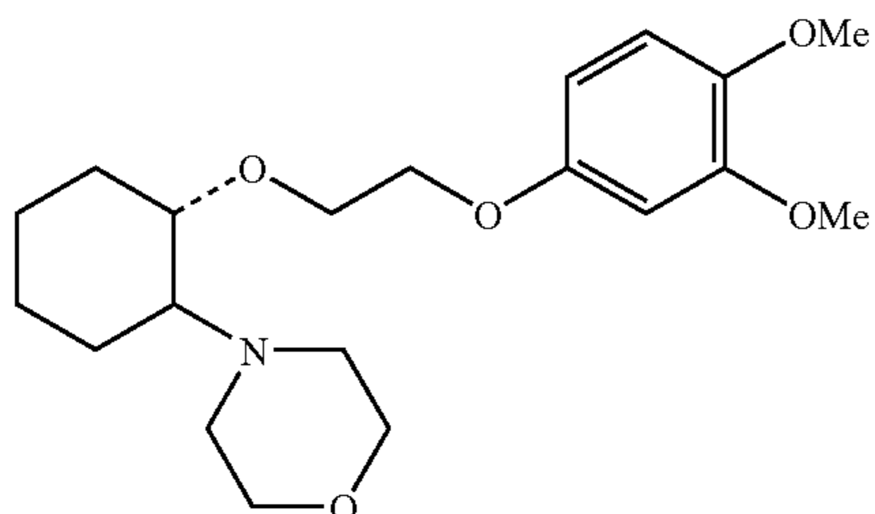
(1R, 2R)/(1S, 2S)-[2-(4-morpholinyl)-1-(3,4-dimethoxyphenethoxy)]cyclohexane
