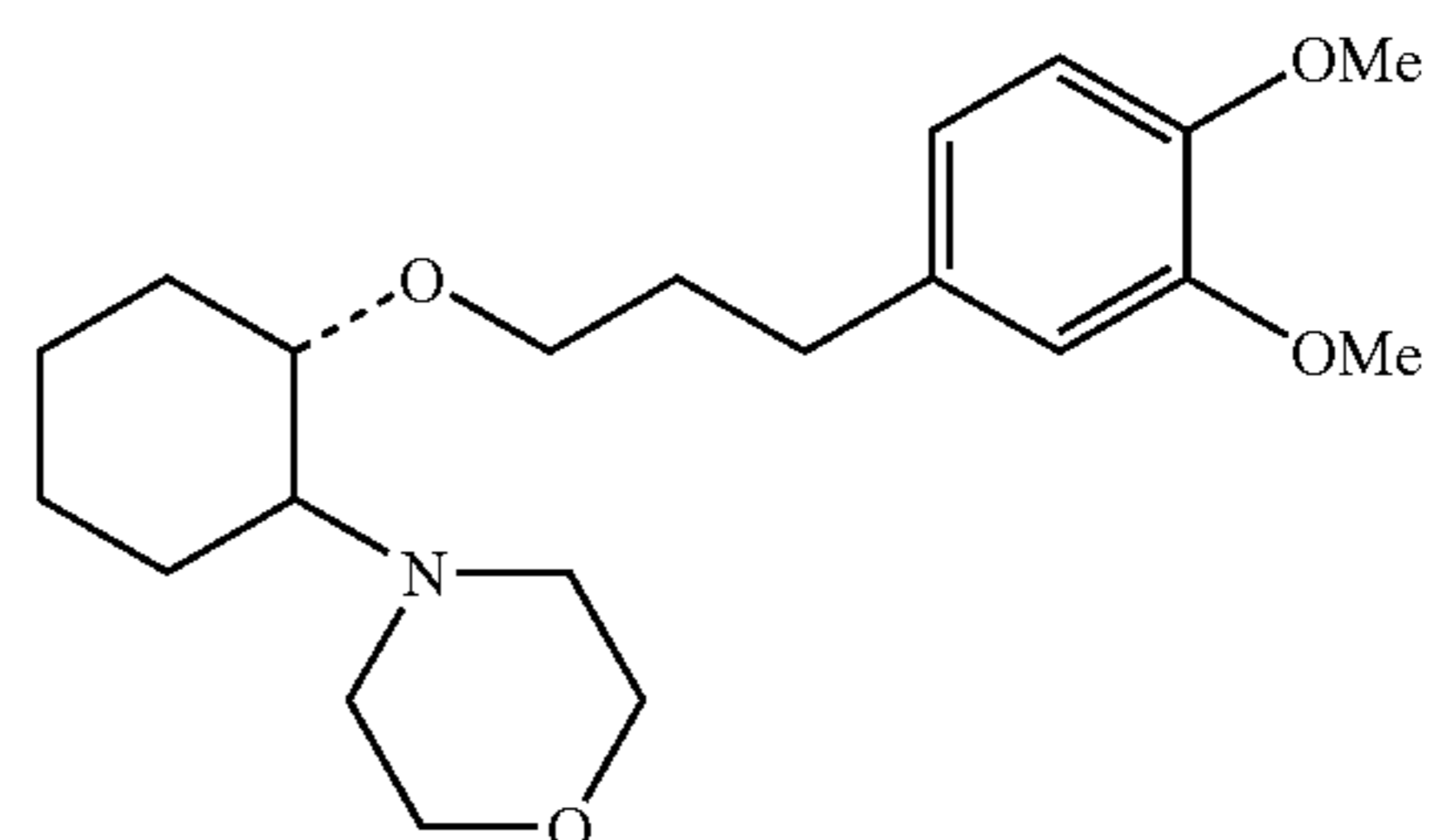
(1R, 2R)/(1S, 2S)-[2-(4-morpholinyl)-1-(3-(3,4-dimethoxyphenyl)propoxy)]cyclohexane
