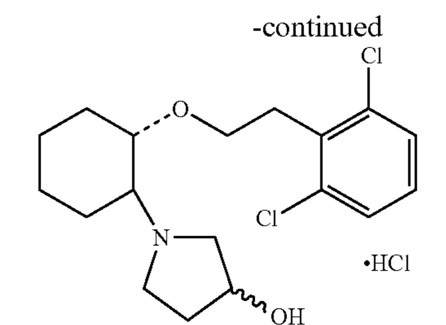
(1R, 2R)/(1S, 2S)-2-(3-hydroxypyrrolidinyl)-1-(2,6-dichlorophenoxy)cyclohexane monohydrochloride
