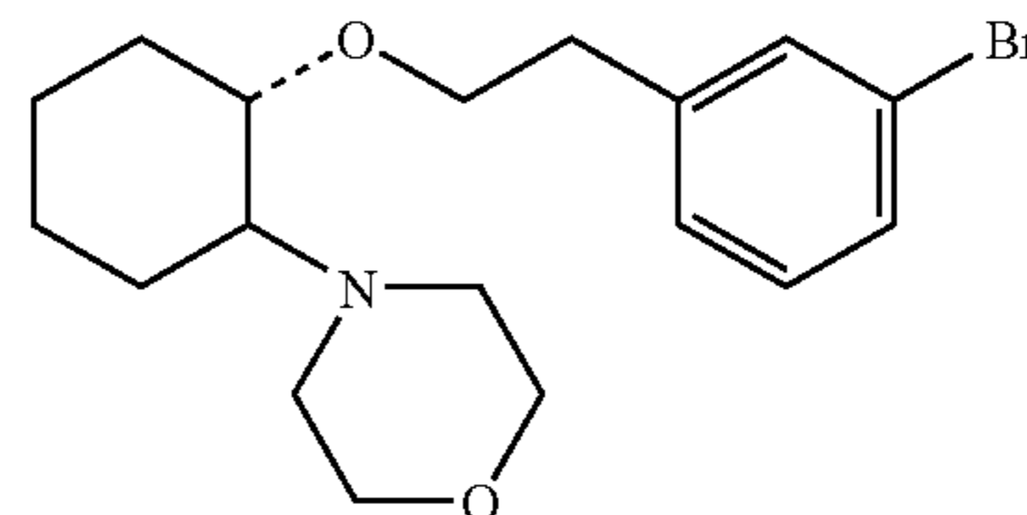
(1R, 2R)/(1S, 2S)-[2-(4-morpholinyl)-1-(3-bromophenethoxy)]cyclohexane
