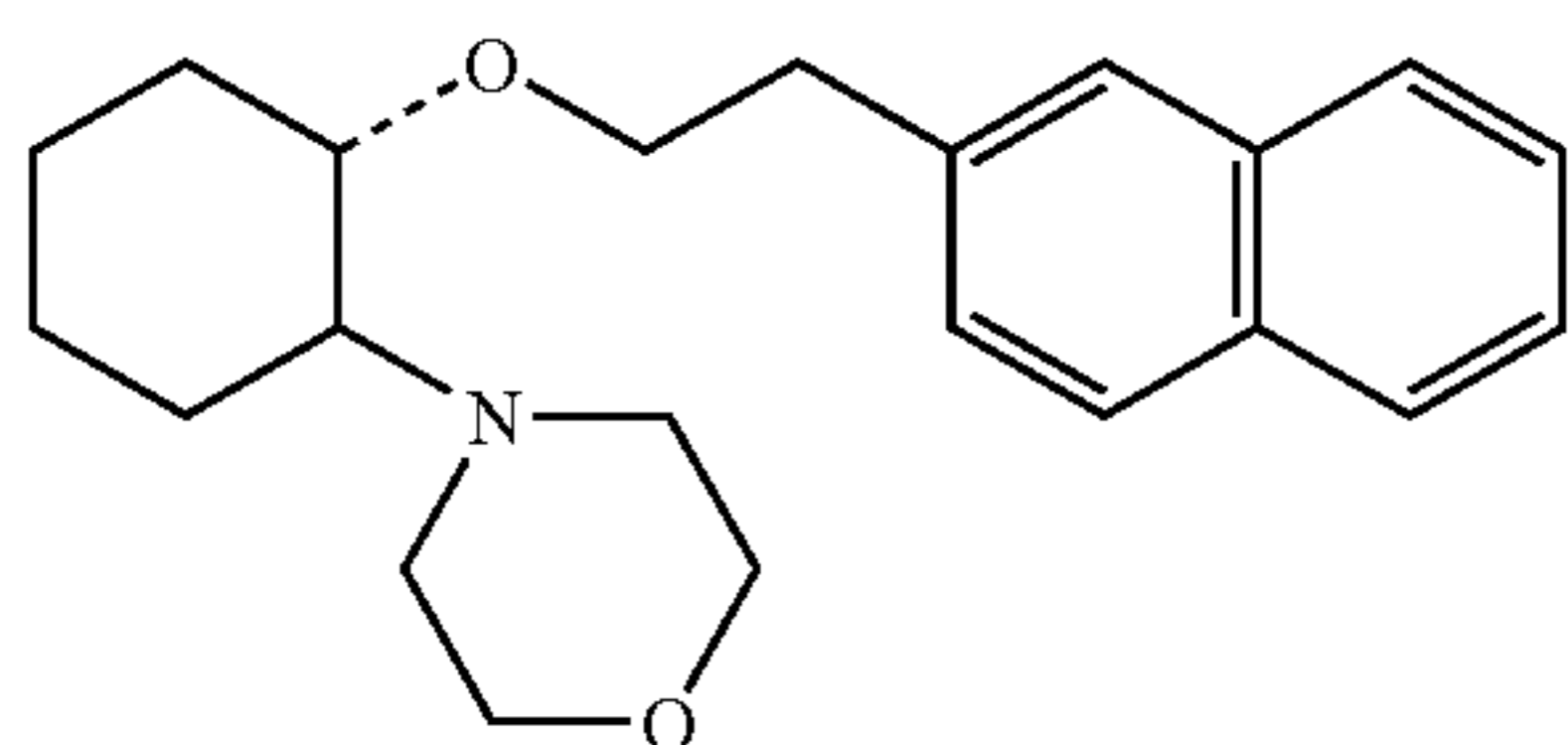
(1R, 2R)/(1S, 2S)-[2-(4-morpholinyl)-1-(2-naphthenethoxy)]cyclohexane
