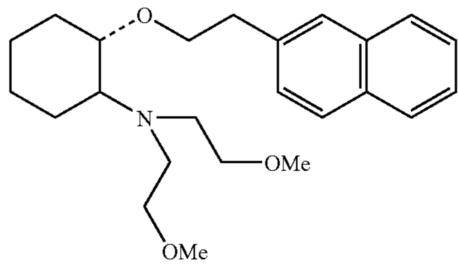
(1R, 2R)/(1S, 2S)-2-[bis(2-methoxyethyl)aminy]-1-(2-naphthenethoxy)cyclohexane
