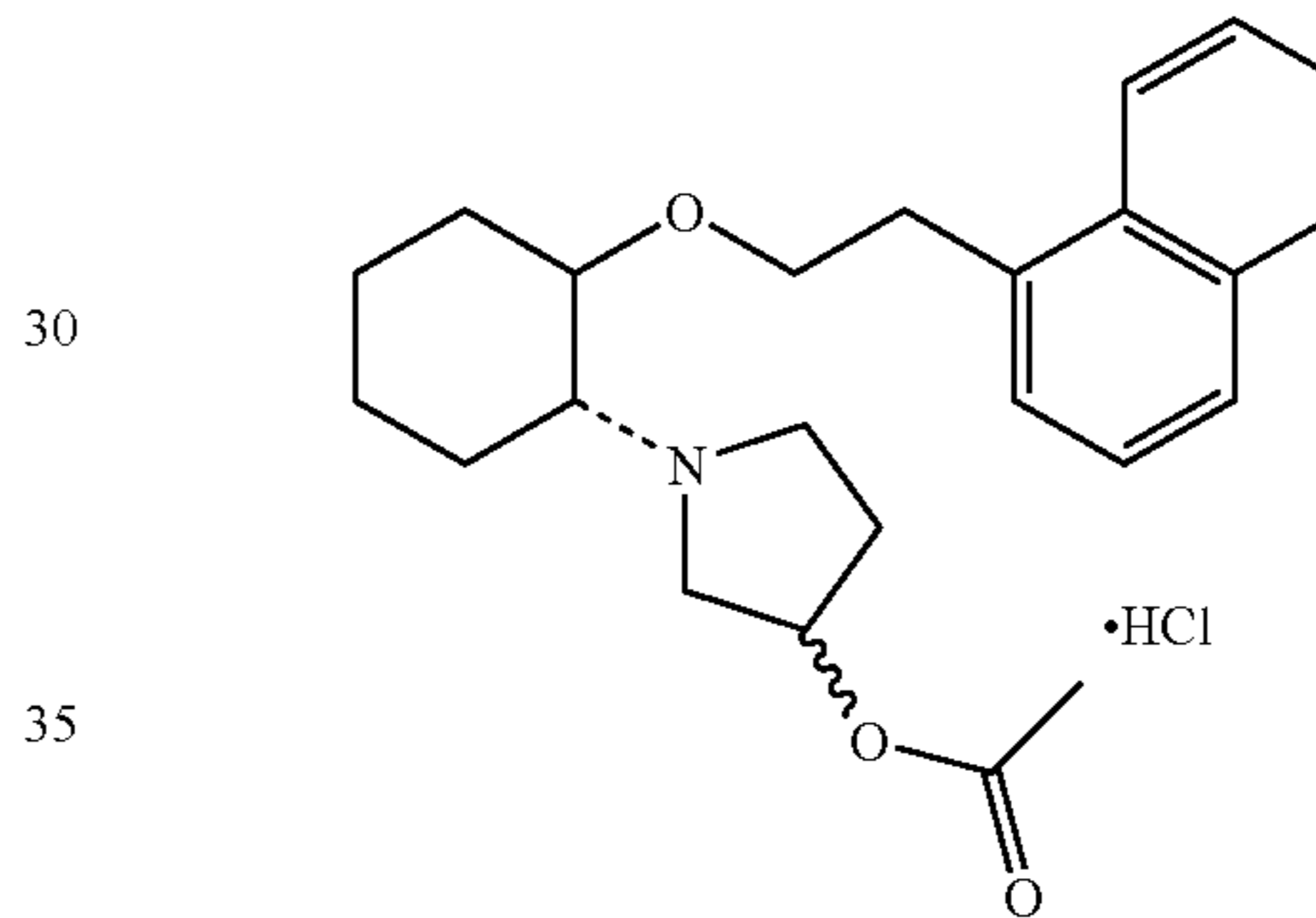
(1R, 2R)/(1S, 2S)-2-(3-acetoxypyrrolidinyl)-1-(1-naphthenethoxy)cyclohexane monohydrochloride
