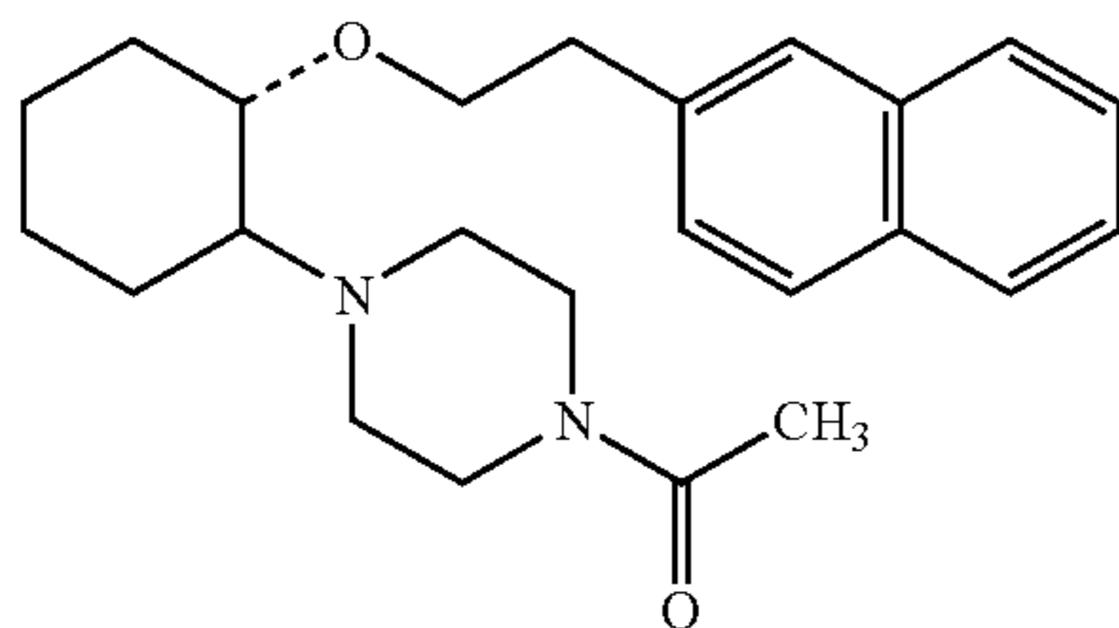
(1R, 2R)/(1S, 2S)-2-(1-acetylpiperazinyl)-1-(2-naphthenethoxy)cyclohexane
