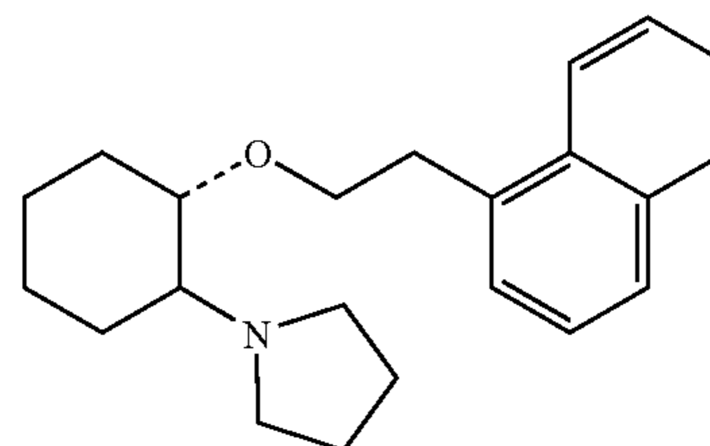
(1R, 2R)/(1S, 2S)-[2-(1-pyrrolidinyl)-1-(1-naphthenethoxy)]cyclohexane
