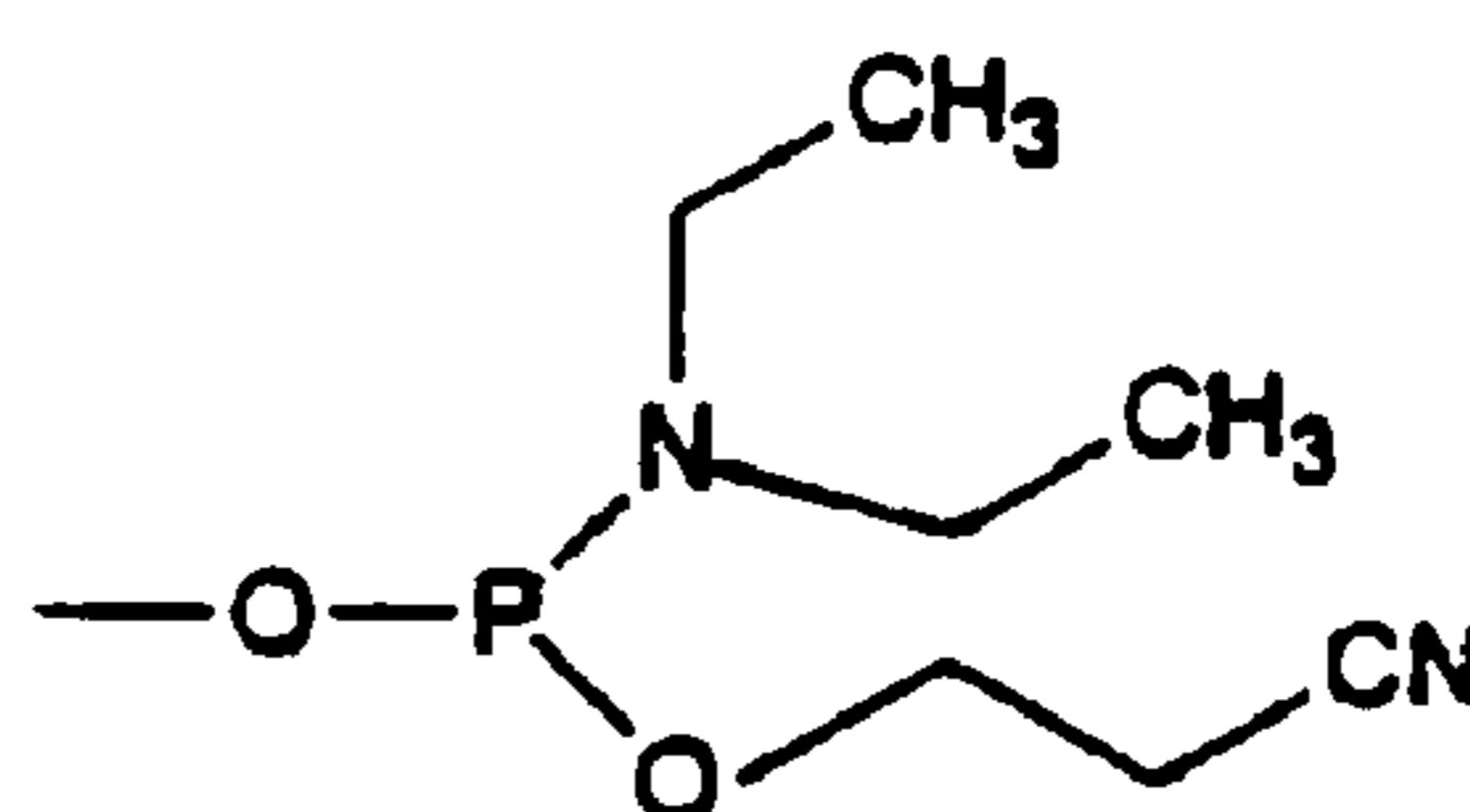
N,N-diethylamino-β-cyanoethoxyphosphine
