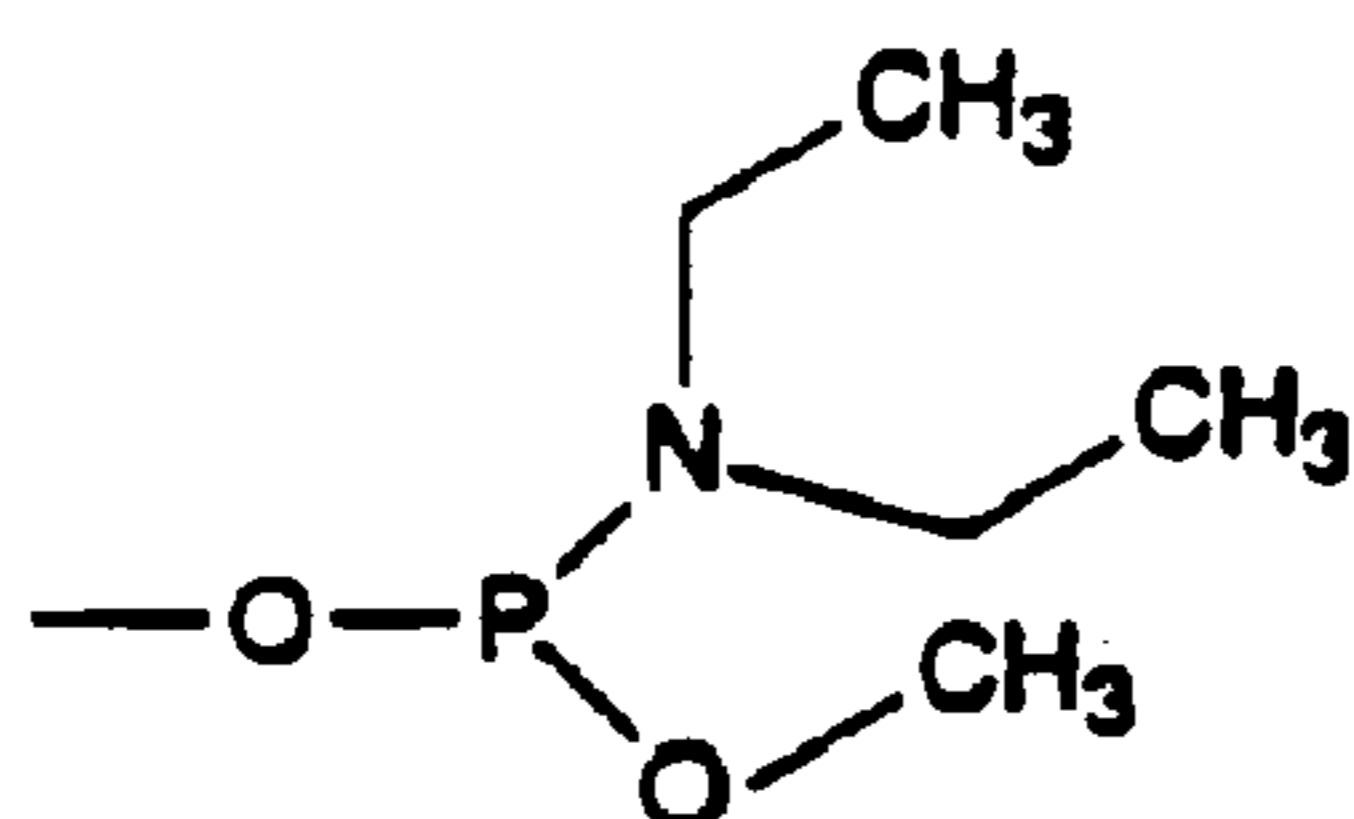
N,N-diethylamino-methoxyphosphine
