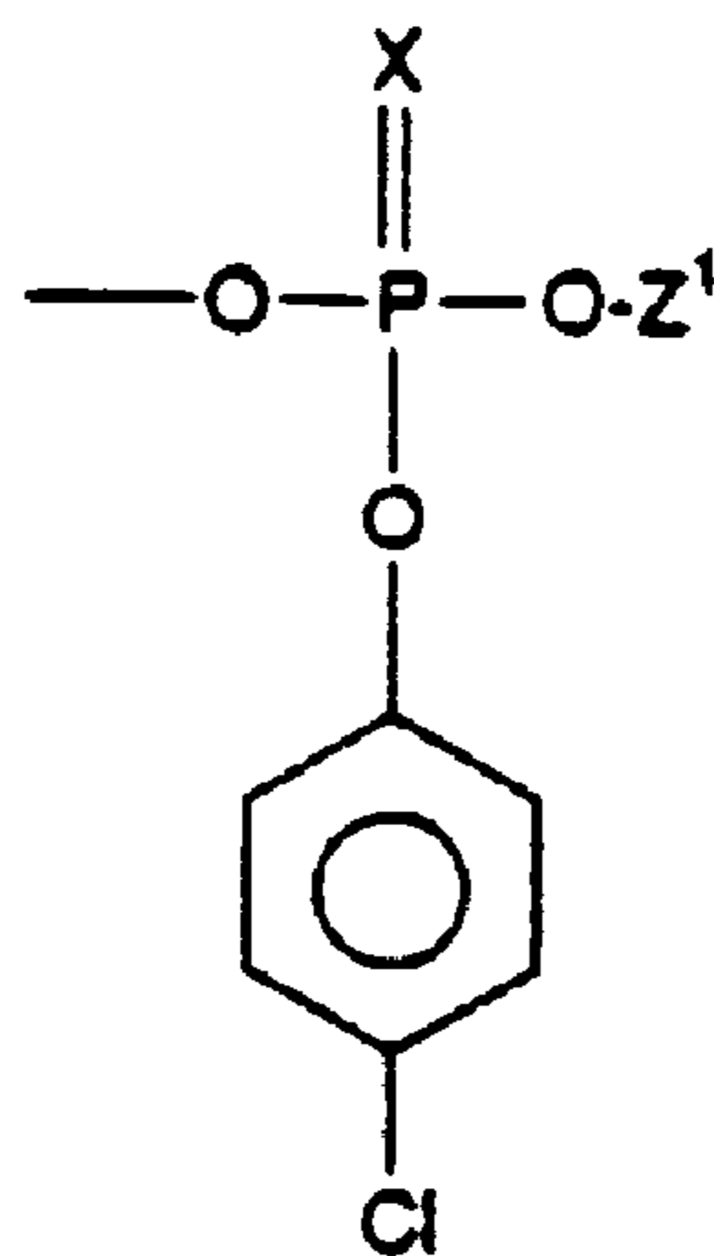
4-chlorophenyl phosphate
