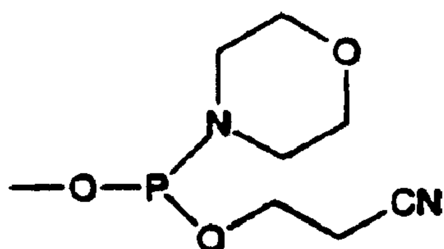
N-morpholino-β-cyanoethoxyphosphine
