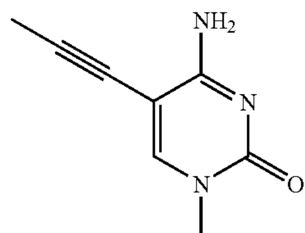
C-5 propynyl cytidine
