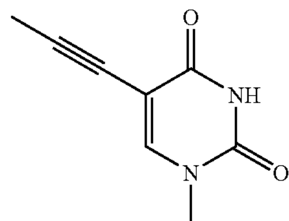
C-5 propynyl thymidine
