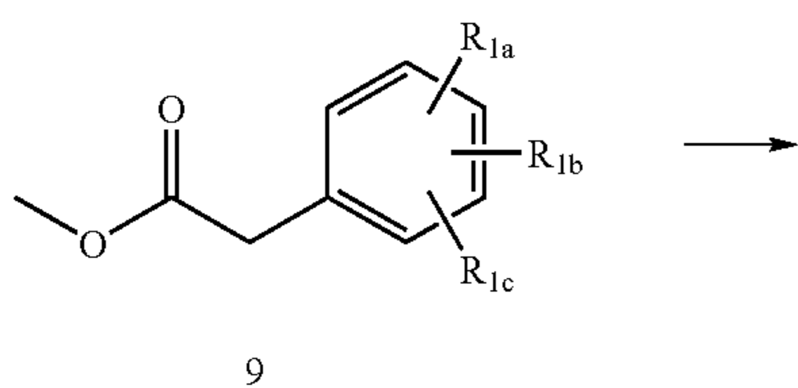
Reaction scheme 3
