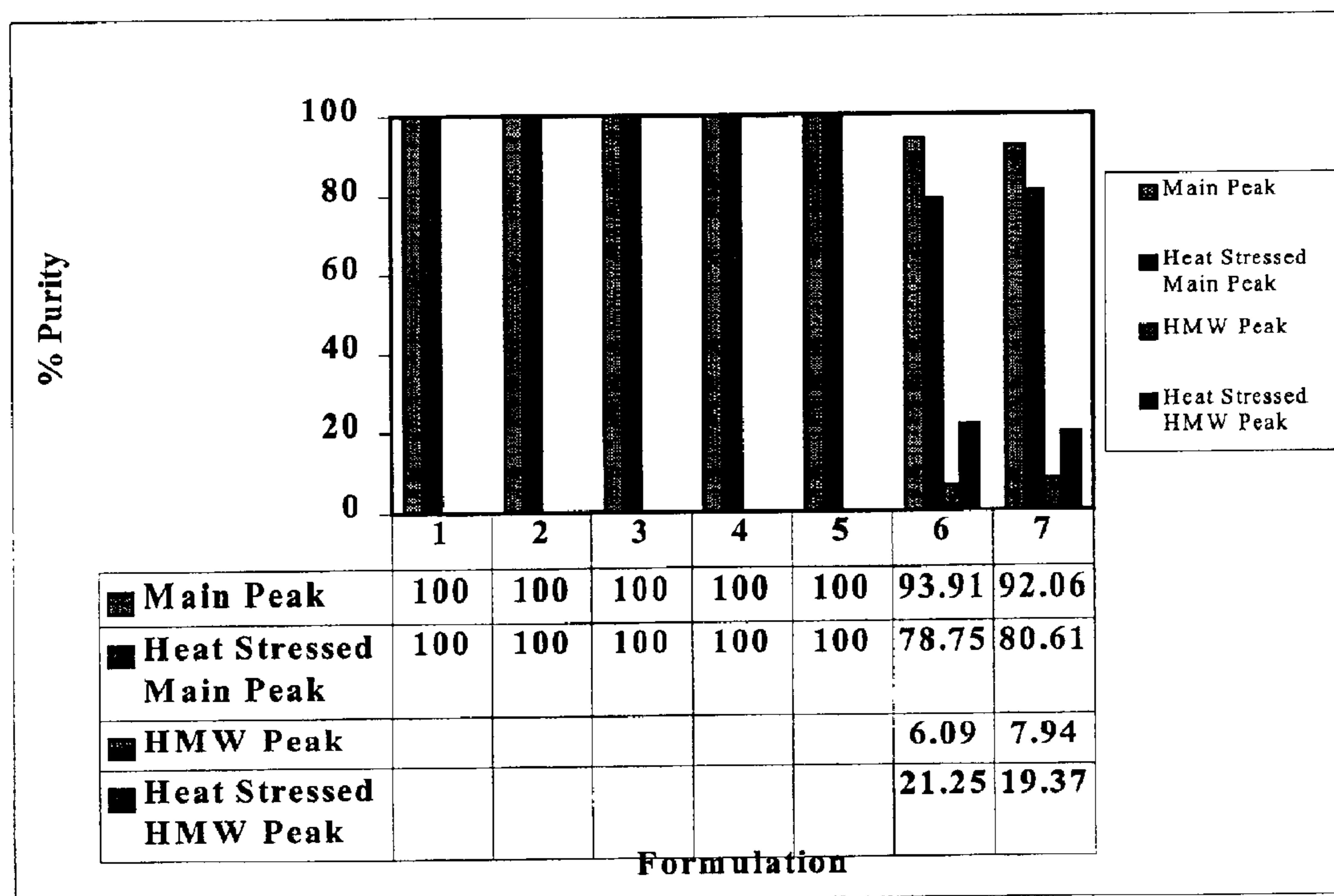
Figure 4. Bulking agents analyzed by SE-HPLC.
