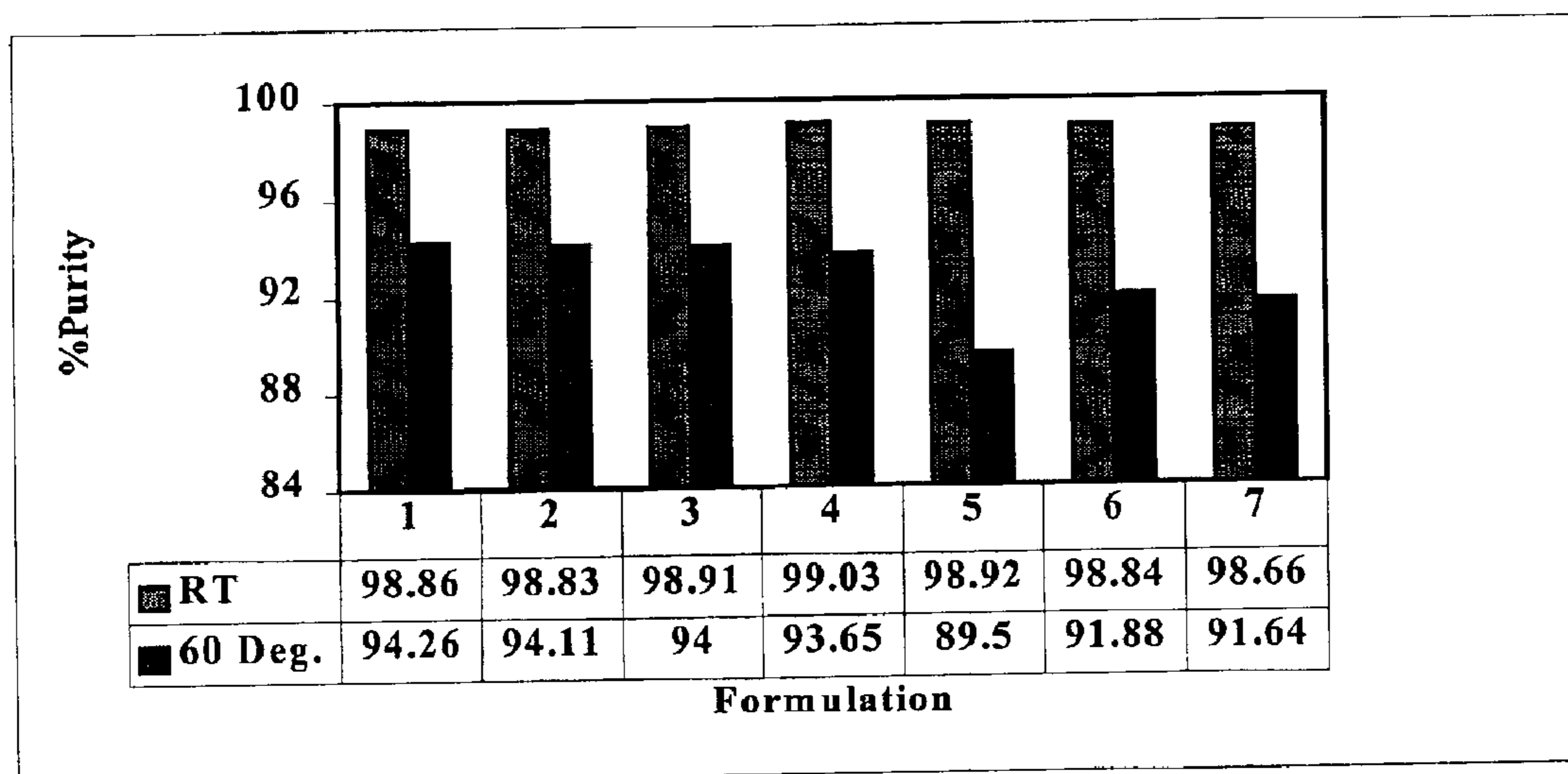
Figure 3. Screening of Bulking agents analyzed by RP-HPLC.
