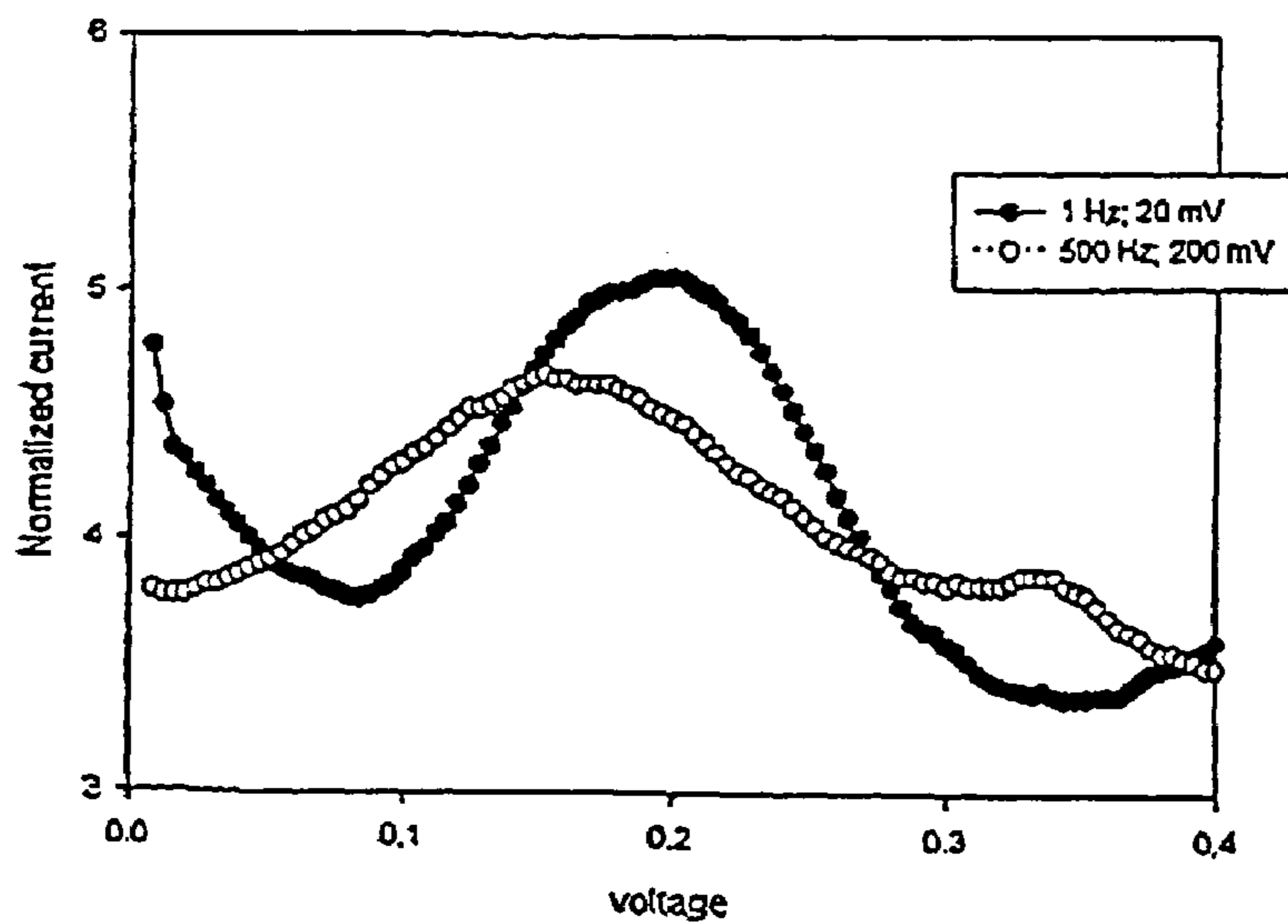
Fc alkane, 1 Hz at 25 mV overpotential 500 Hz at 200 mV overpotential
