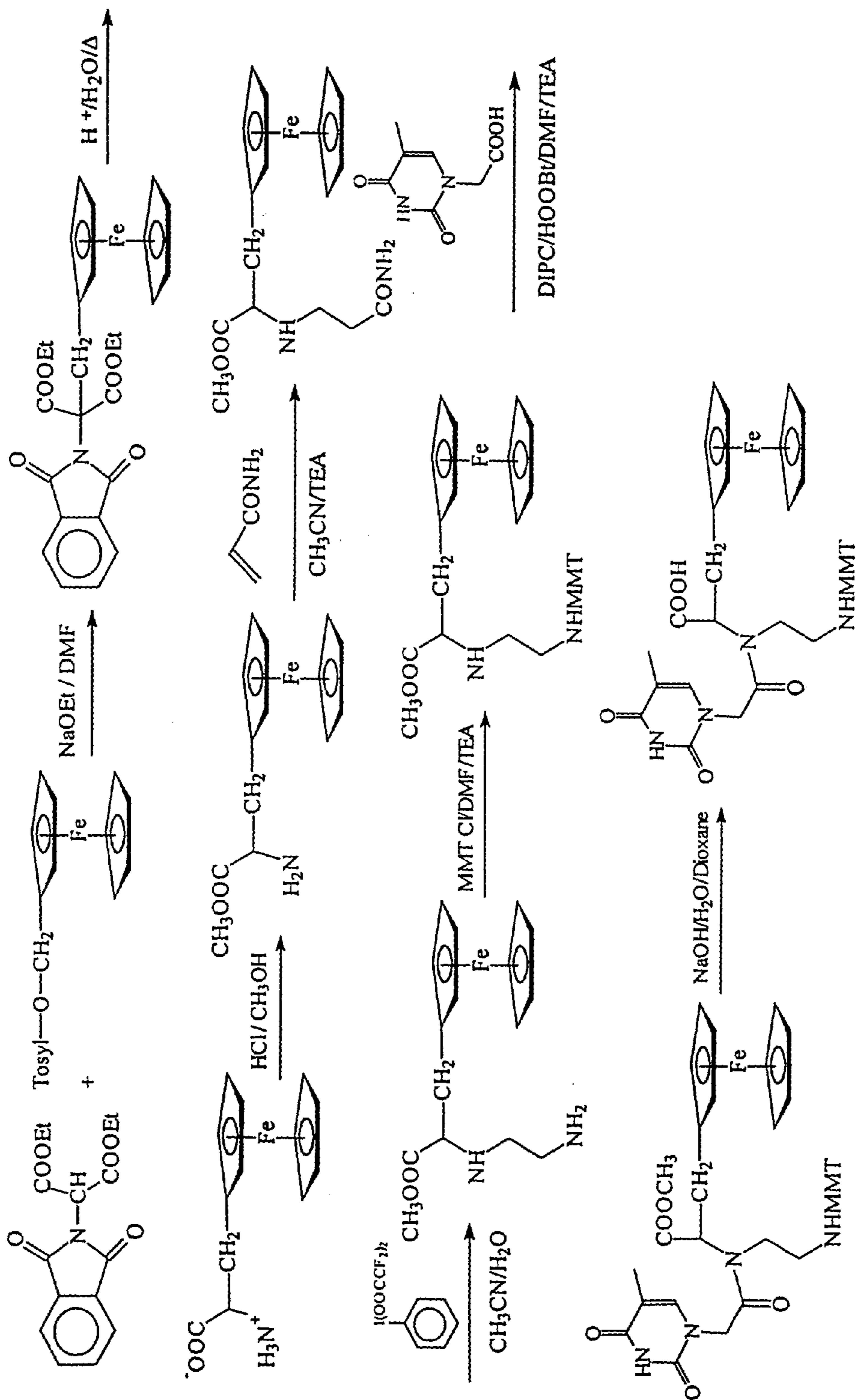
MMT-PNA-Backbone-Ferrocene
