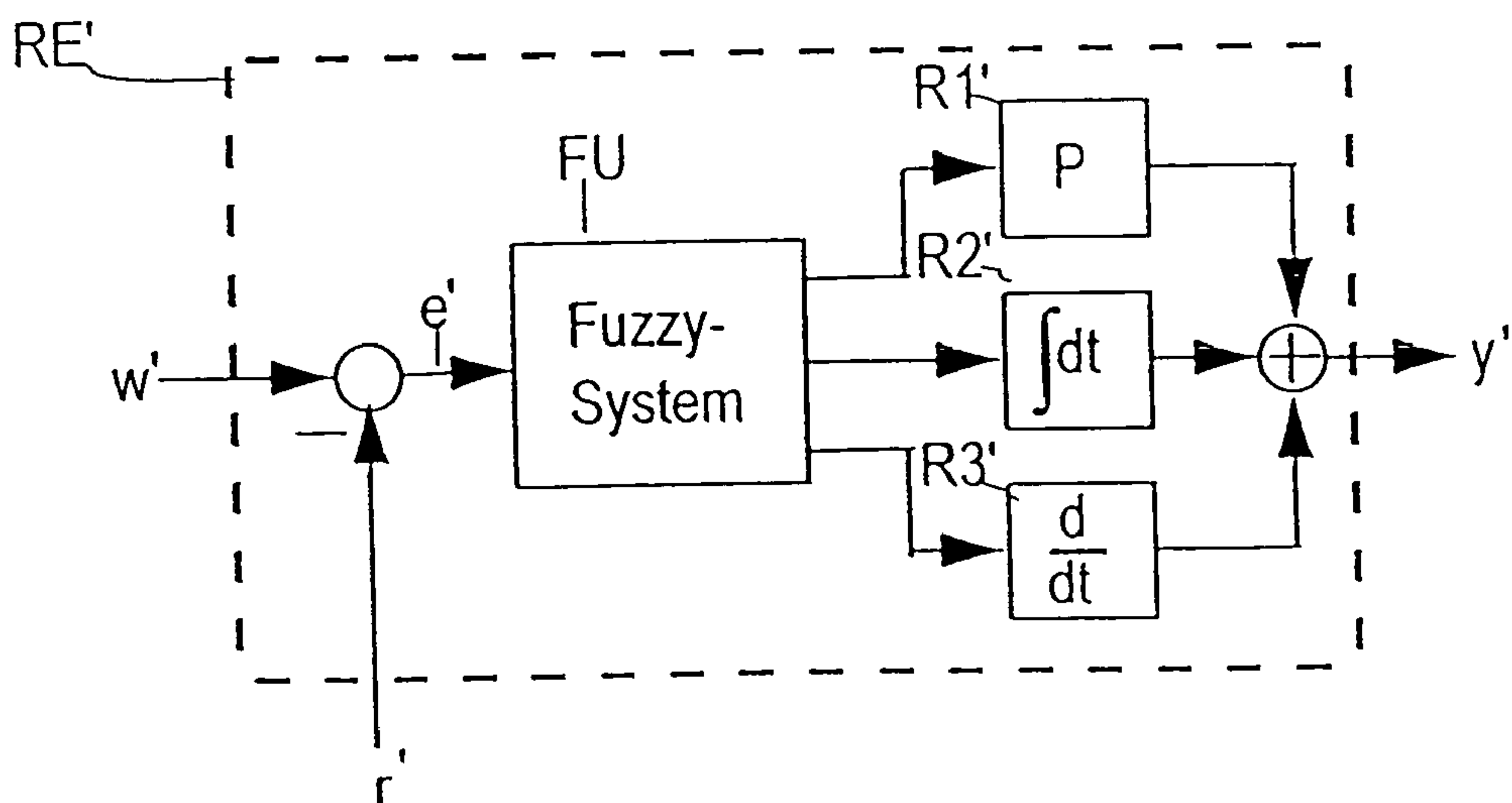
FIG 2 (PRIOR ART)
