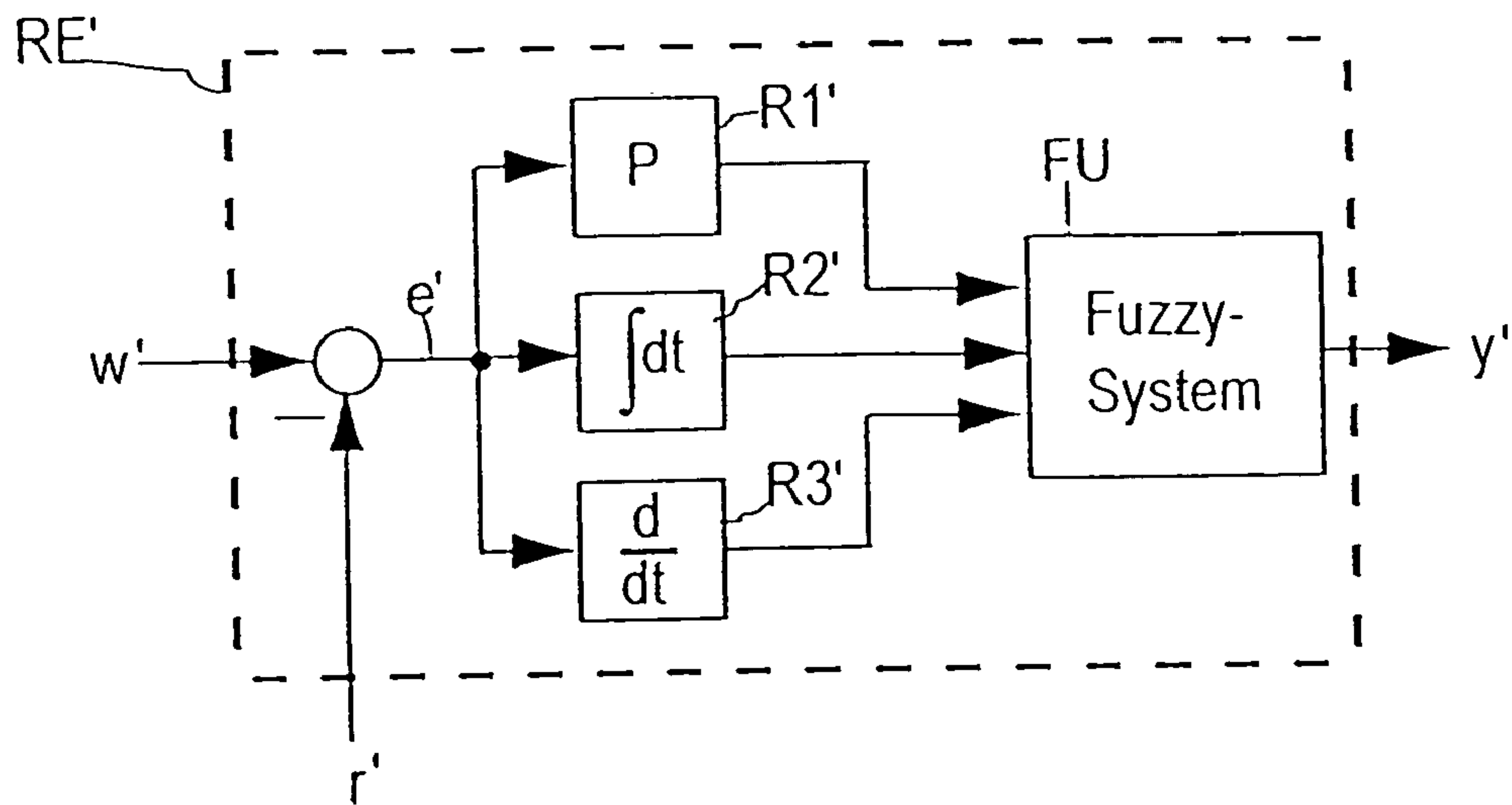
FIG 1 (PRIOR ART)
