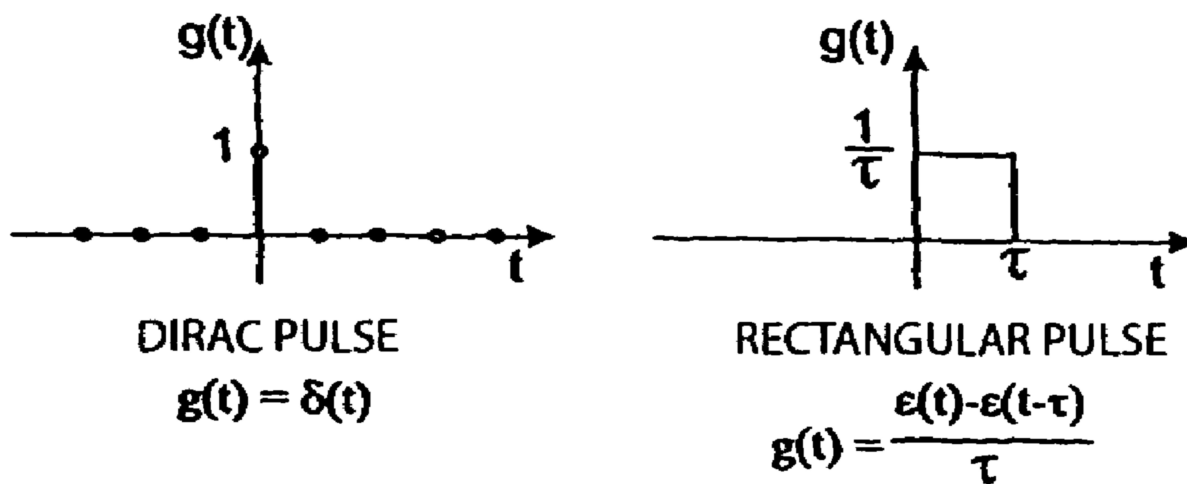
Fig. 2B: DIRAC AND RECTANGULAR PULSES
