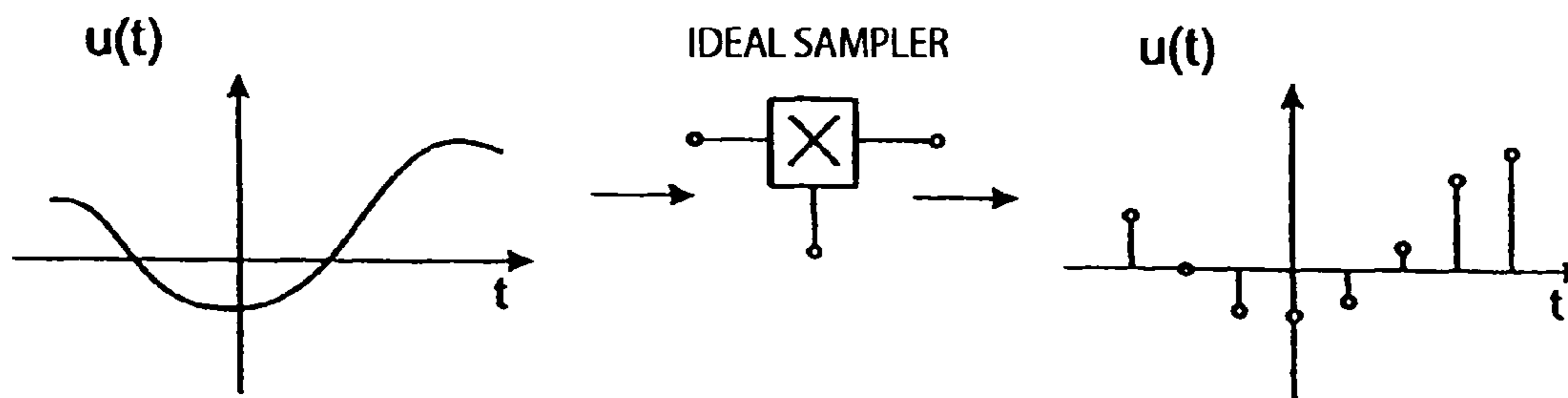
Fig 2D: IDEAL SAMPLER
