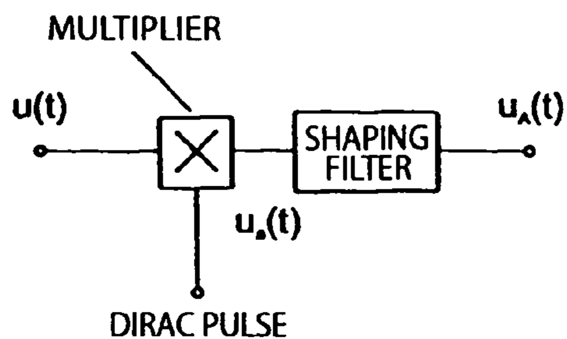
Fig. 2C: MODEL OF A SAMPLER
