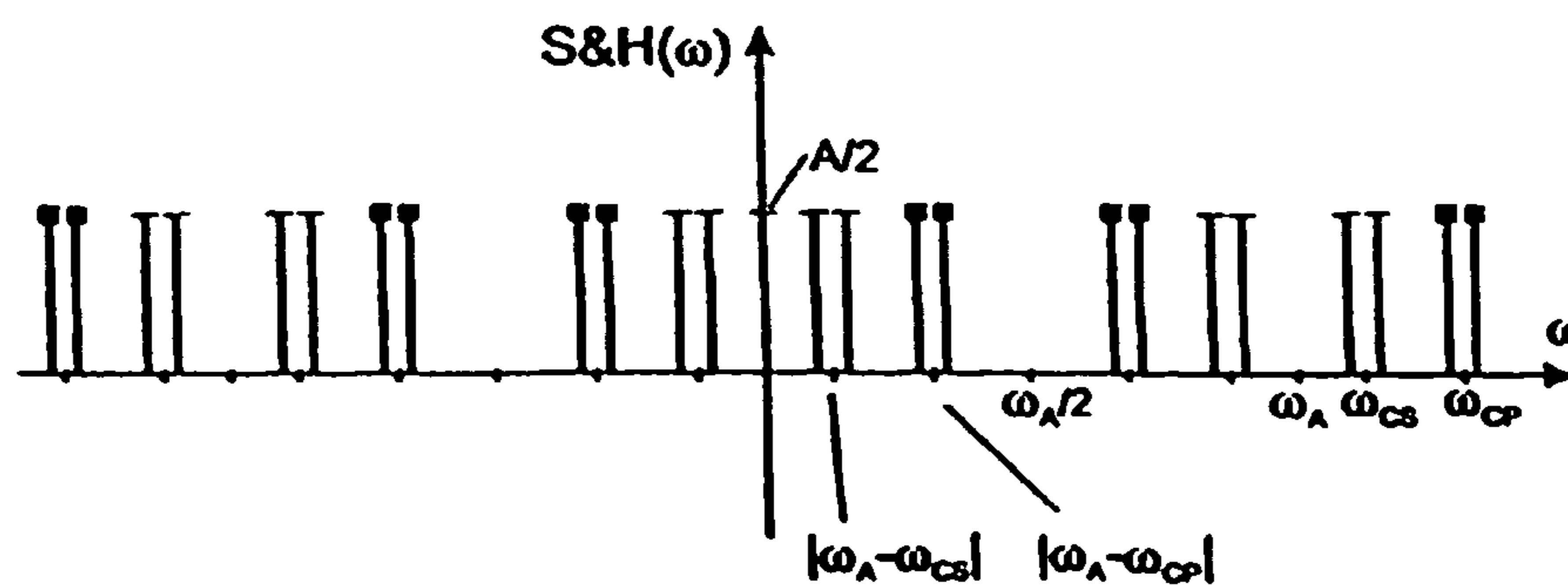
Fig. 2F: INTERMEDIATE MIXING WITH f_A < f_{CS} + f_{drive}
