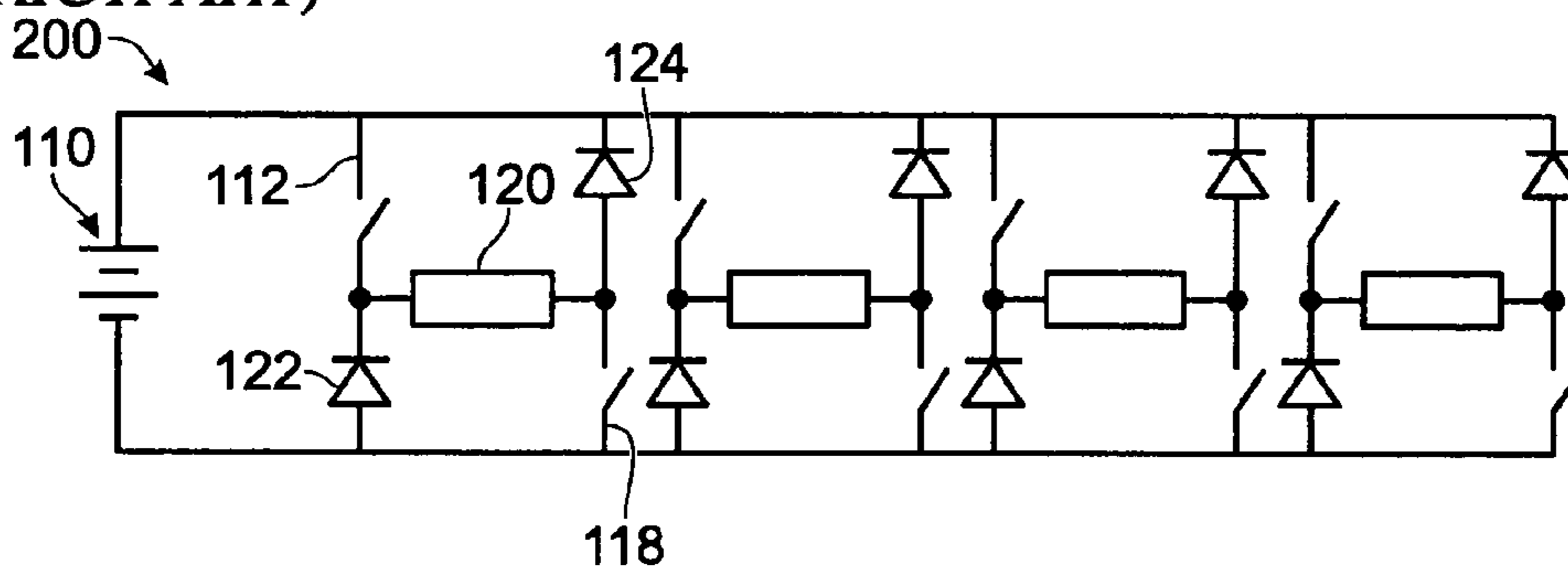
Fig. 2 (PRIOR ART)
