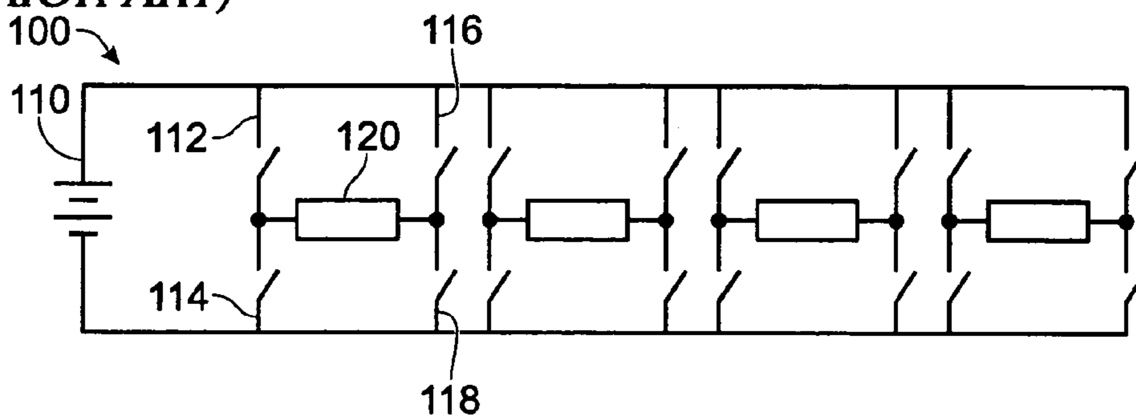
Fig. 1 (PRIOR ART)
