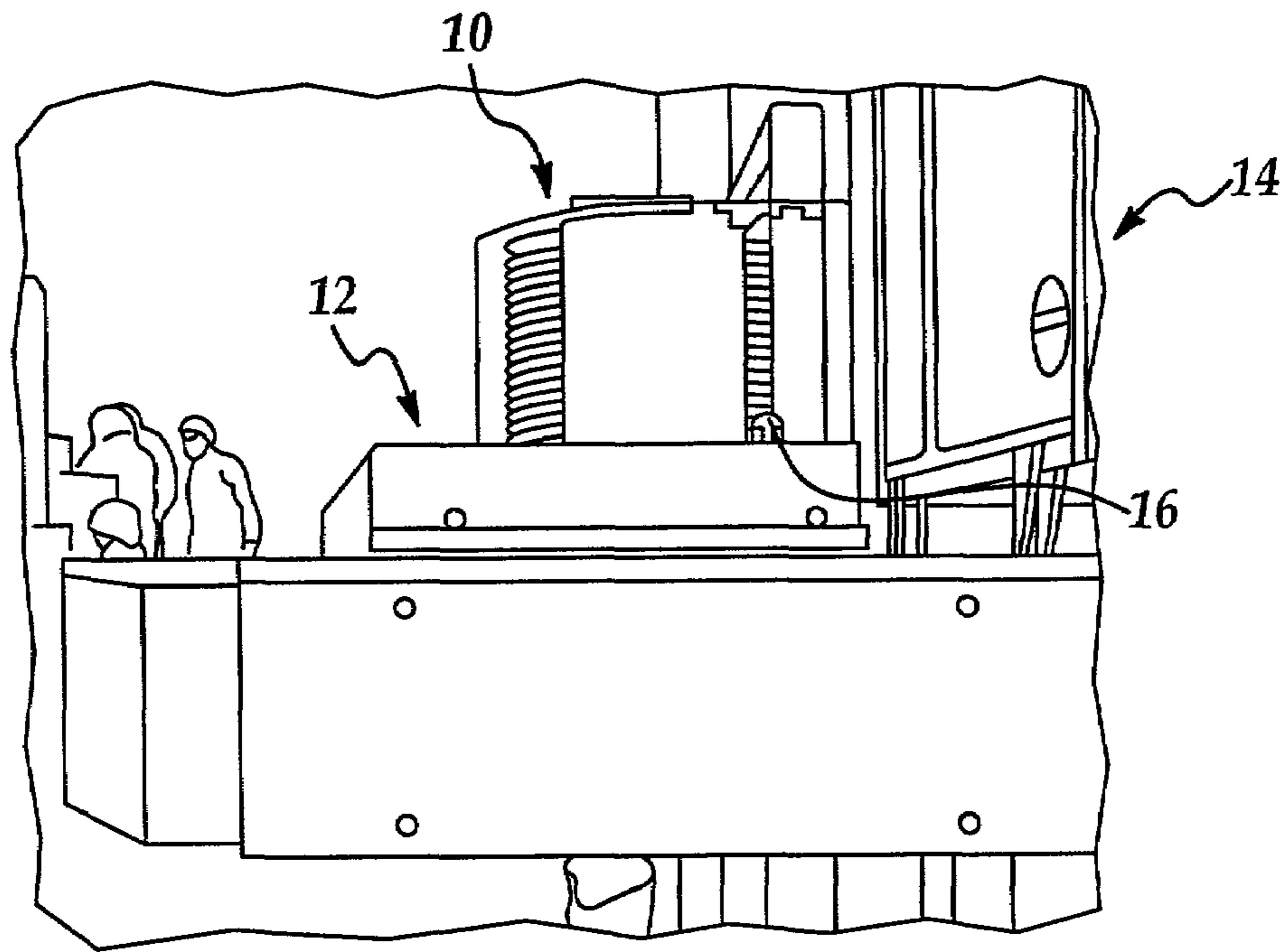
Figure 1 Prior Art
