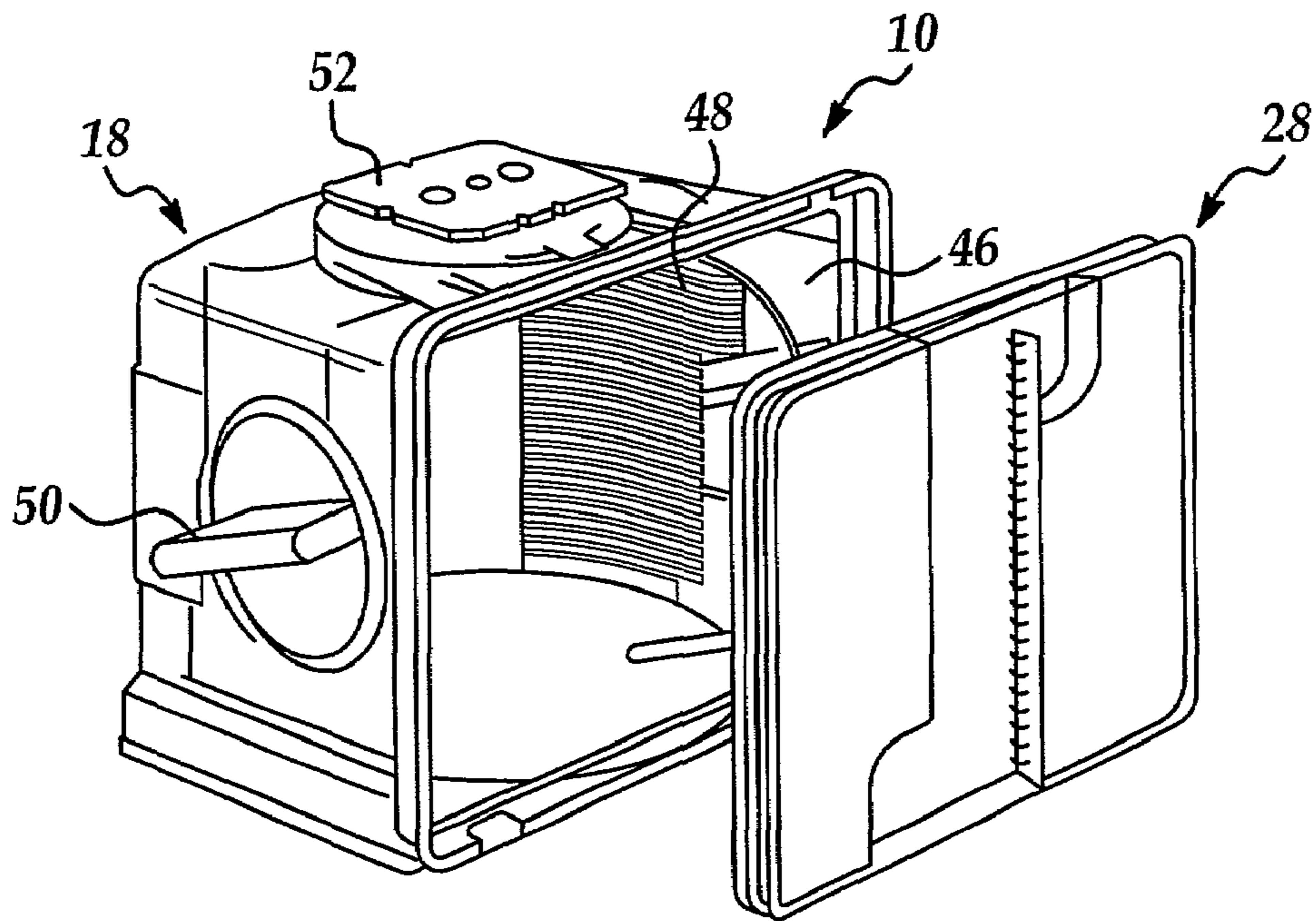
Figure 2 Prior Art
