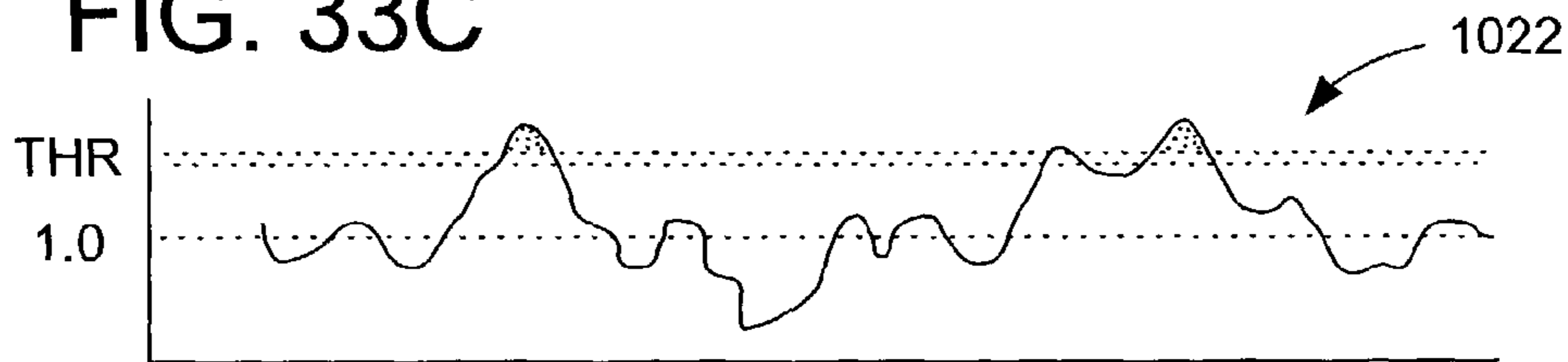
POWER PROFILE ALONG ANGLE A, AS NORMALIZED BY ITS OWN MOVING AVERAGE; ONLY A MINIMAL AMOUNT EXCEEDS THRESHOLD, GIVING A SMALL INTEGRATED VALUE
