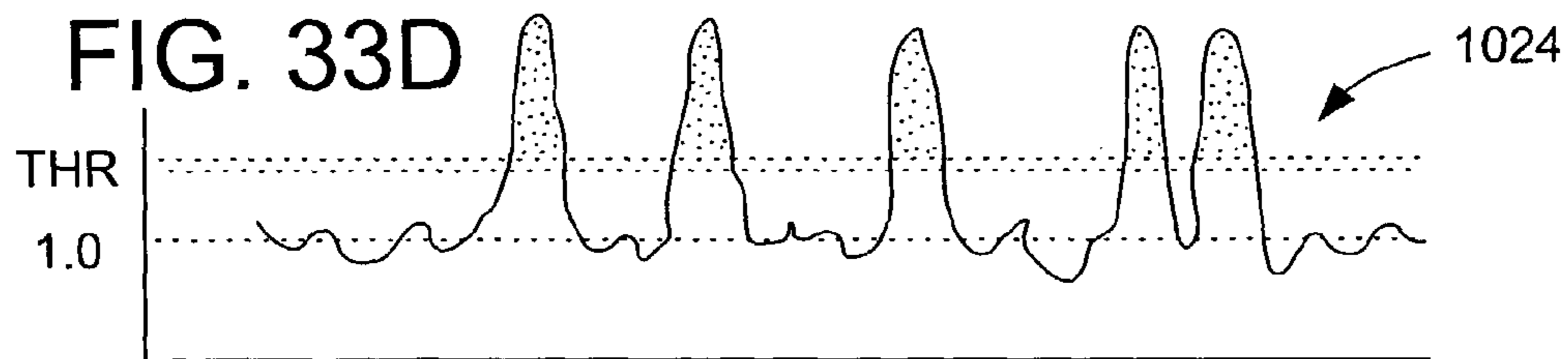
POWER PROFILE ALONG ANGLE B, AS NORMALIZED BY ITS OWN MOVING AVERAGE; THIS FINDS STRONG ENERGY ABOVE THE THRESHOLD
