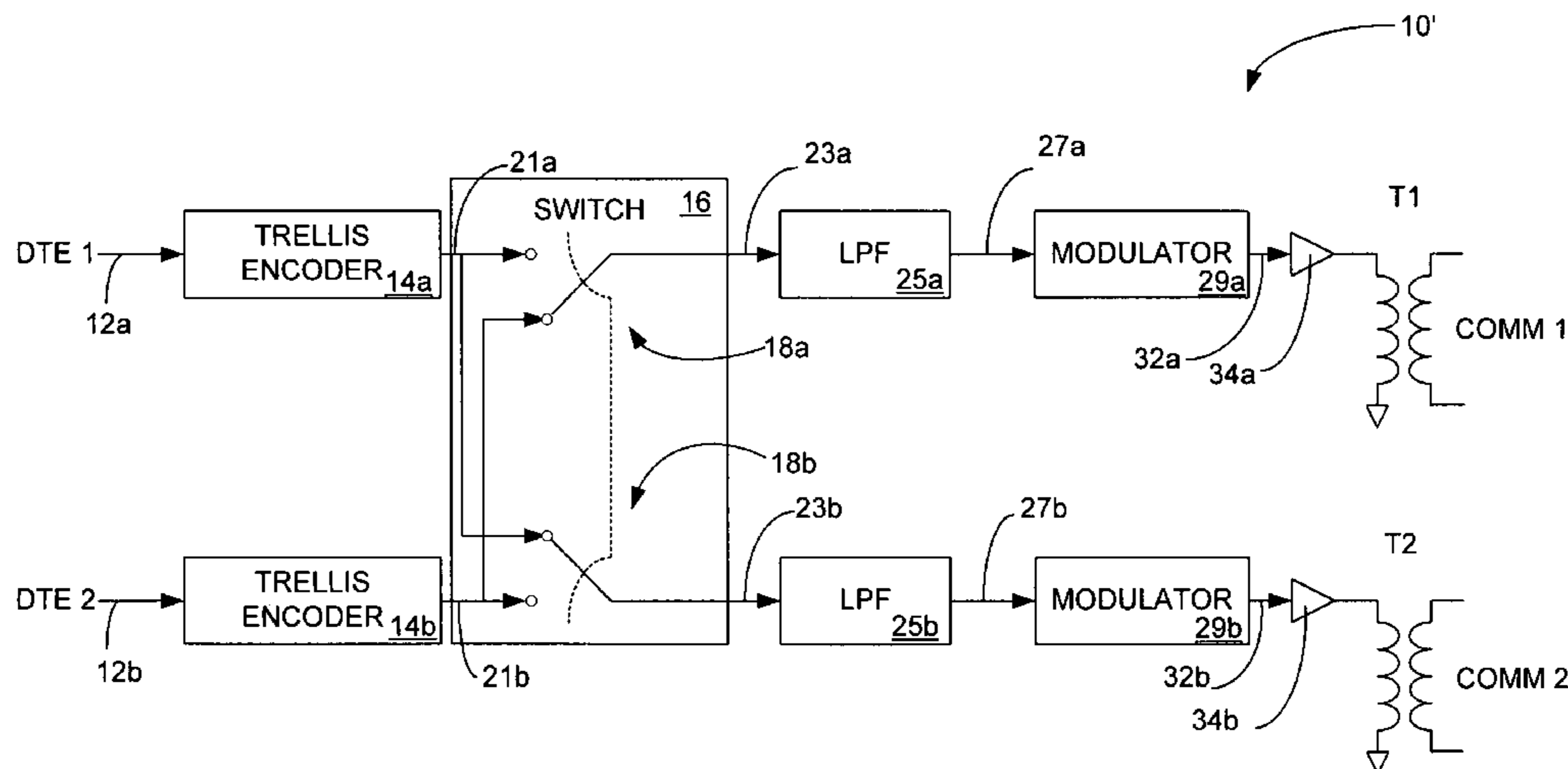
TRANSMITTER (FIRST EMBODIMENT)
