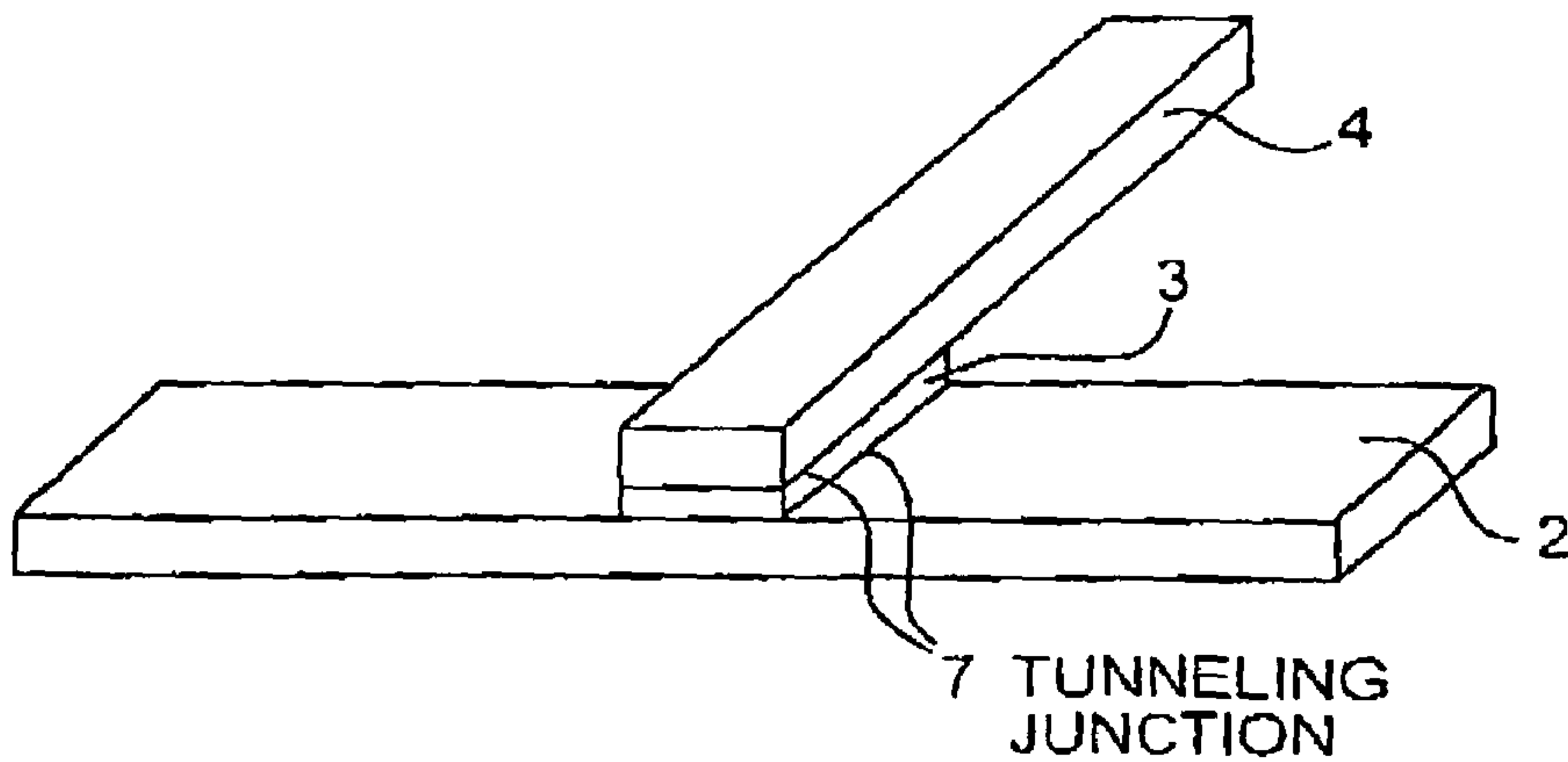
FIG. 13 (PRIOR ART)
