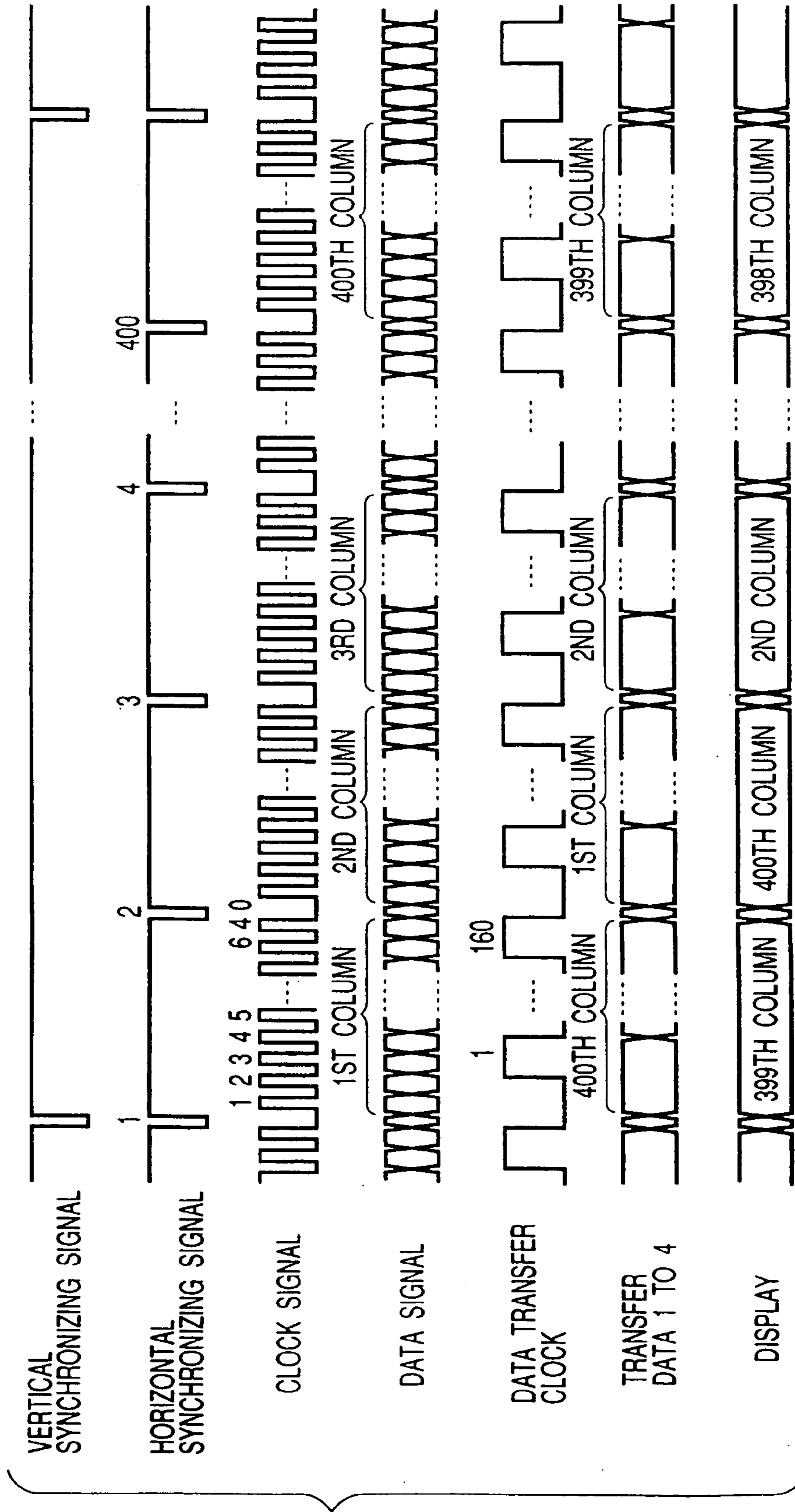
FIG. 25 (PRIOR ART)
