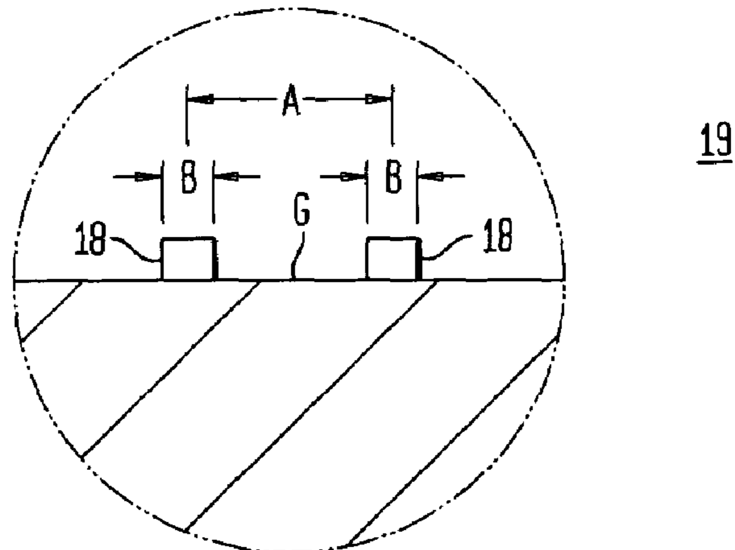
FIG. 1C (PRIOR ART)
