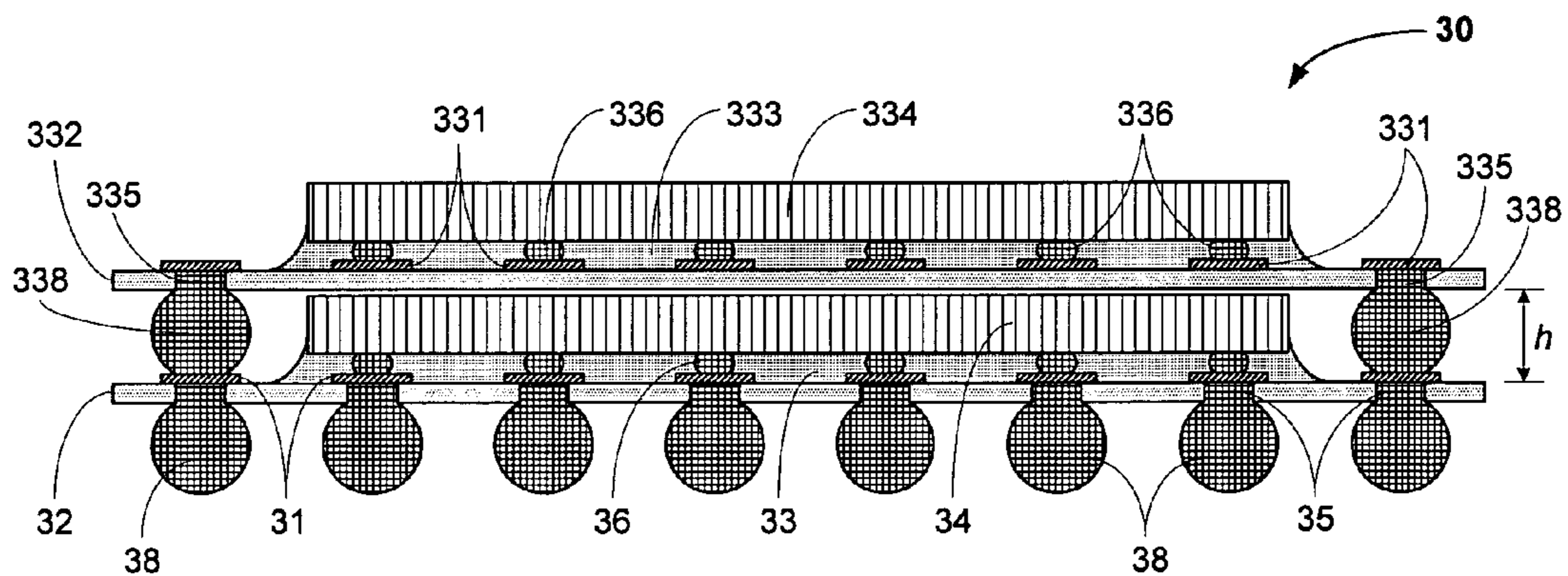
Fig. 3 PRIOR ART
