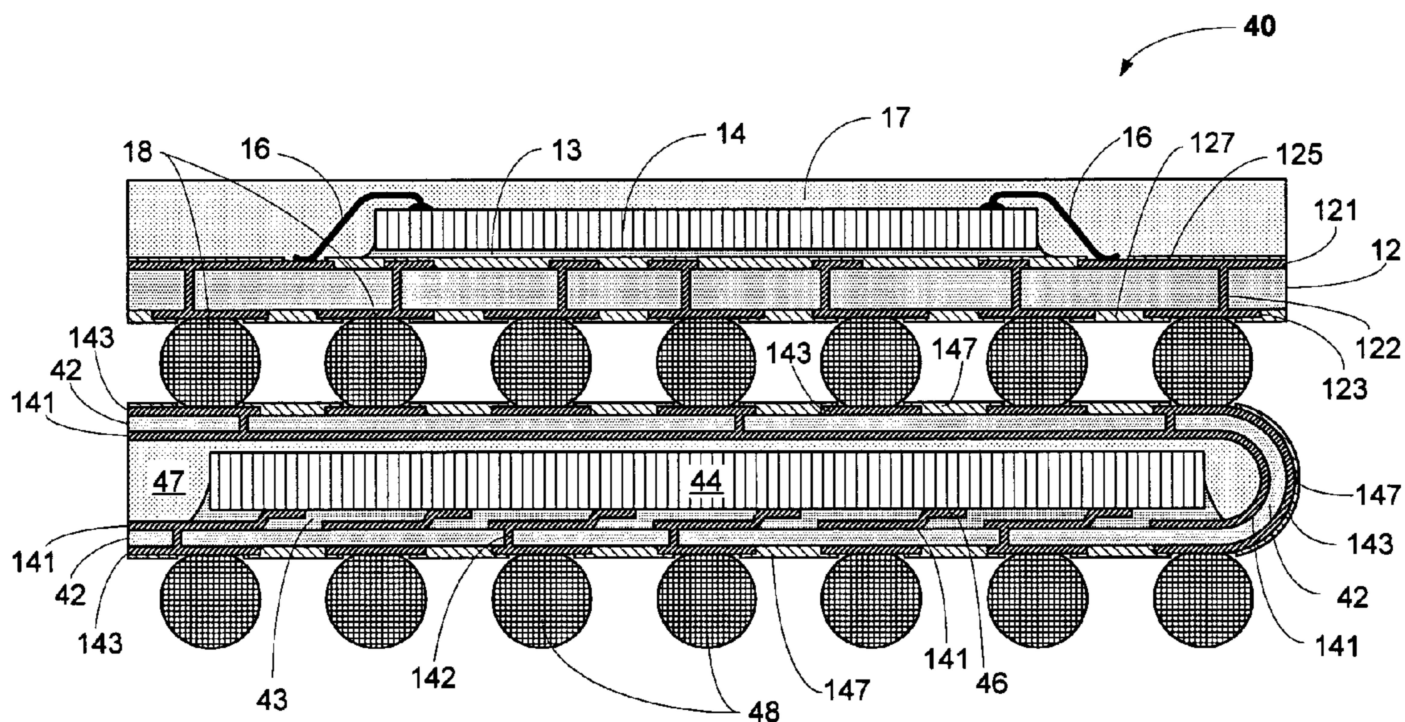
Fig. 4 PRIOR ART
