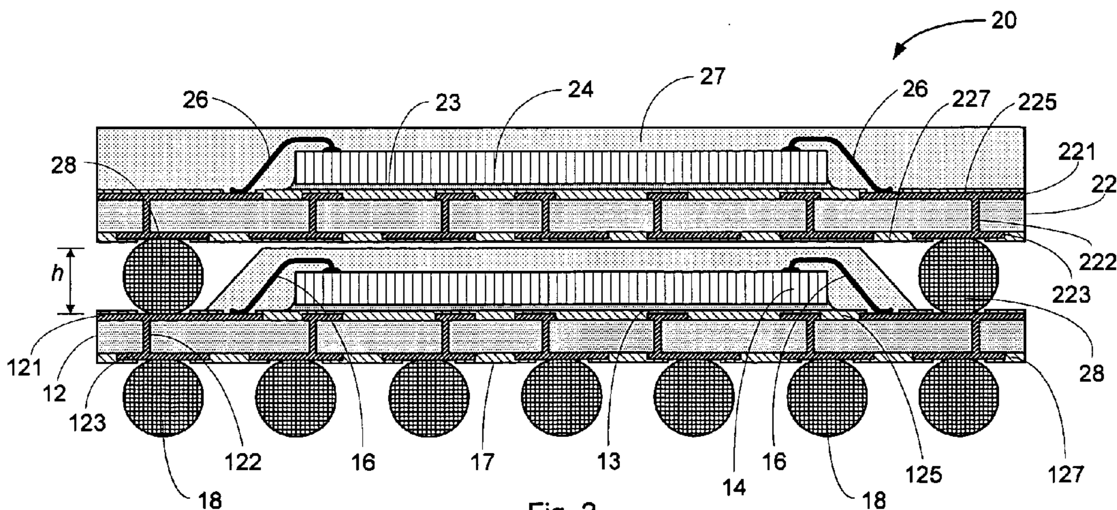
Fig. 2 PRIOR ART
