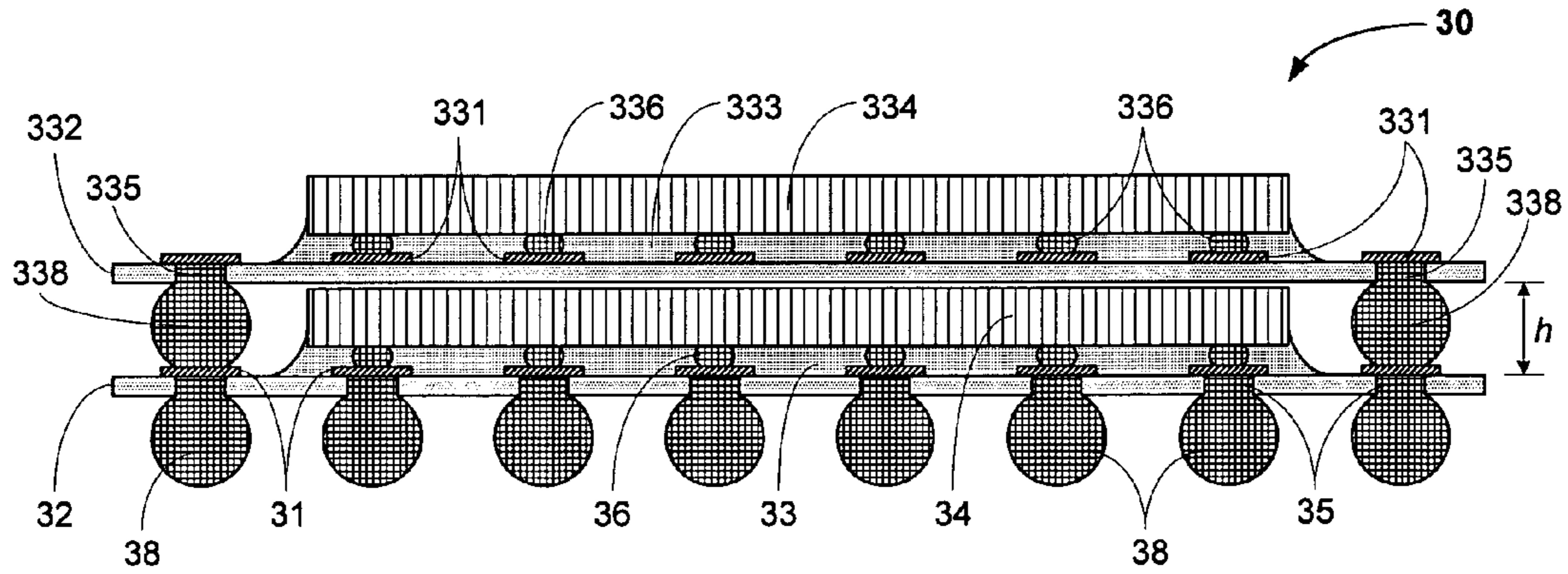
Fig. 3 PRIOR ART
