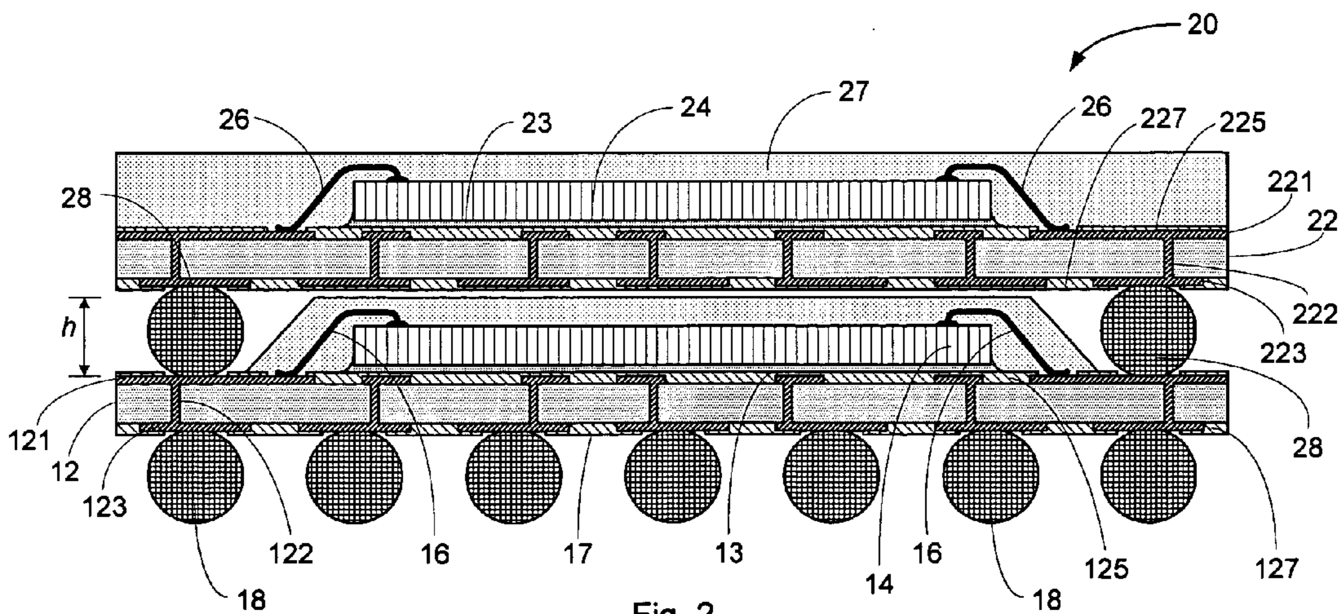
Fig. 2 PRIOR ART
