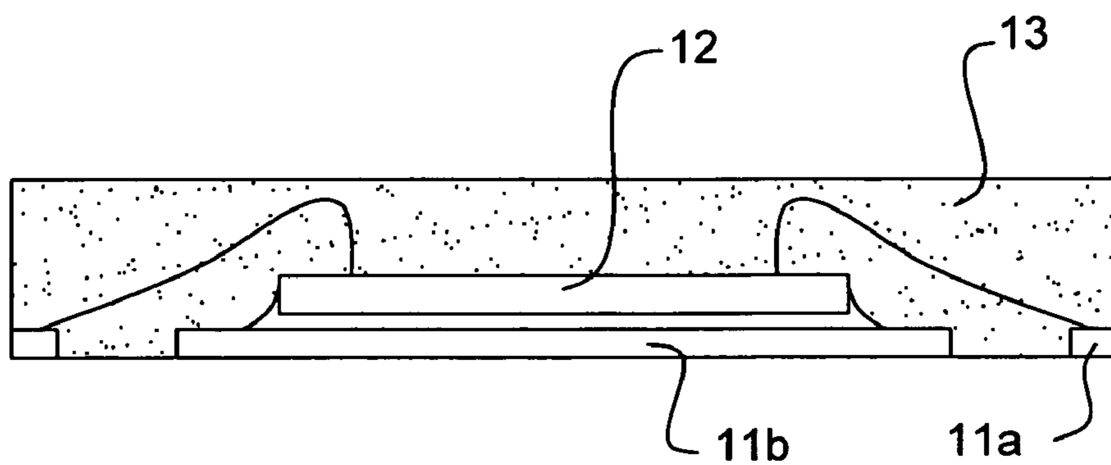
FIG. 2 (PRIOR ART)
