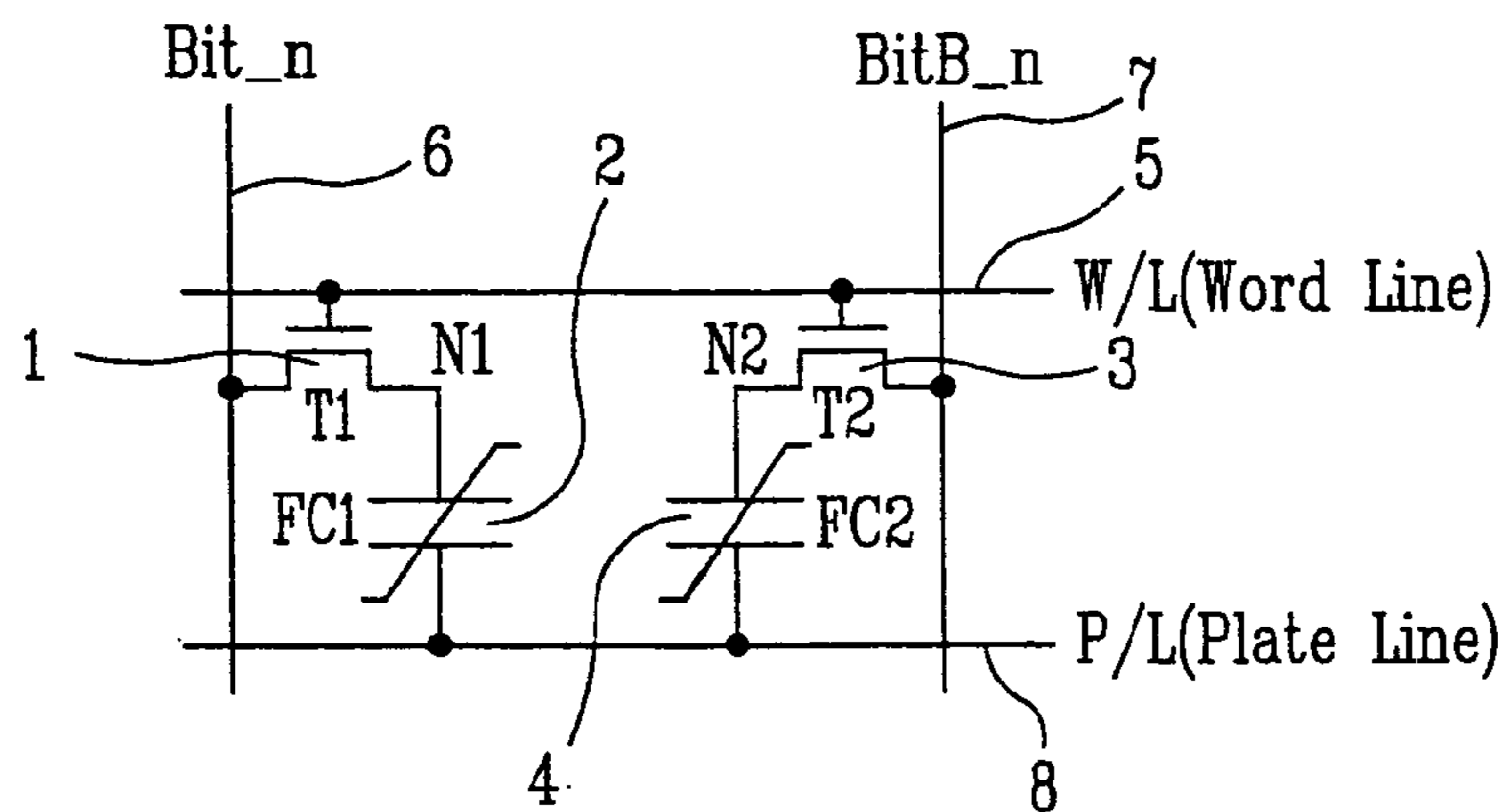
FIG.3 Related Art
