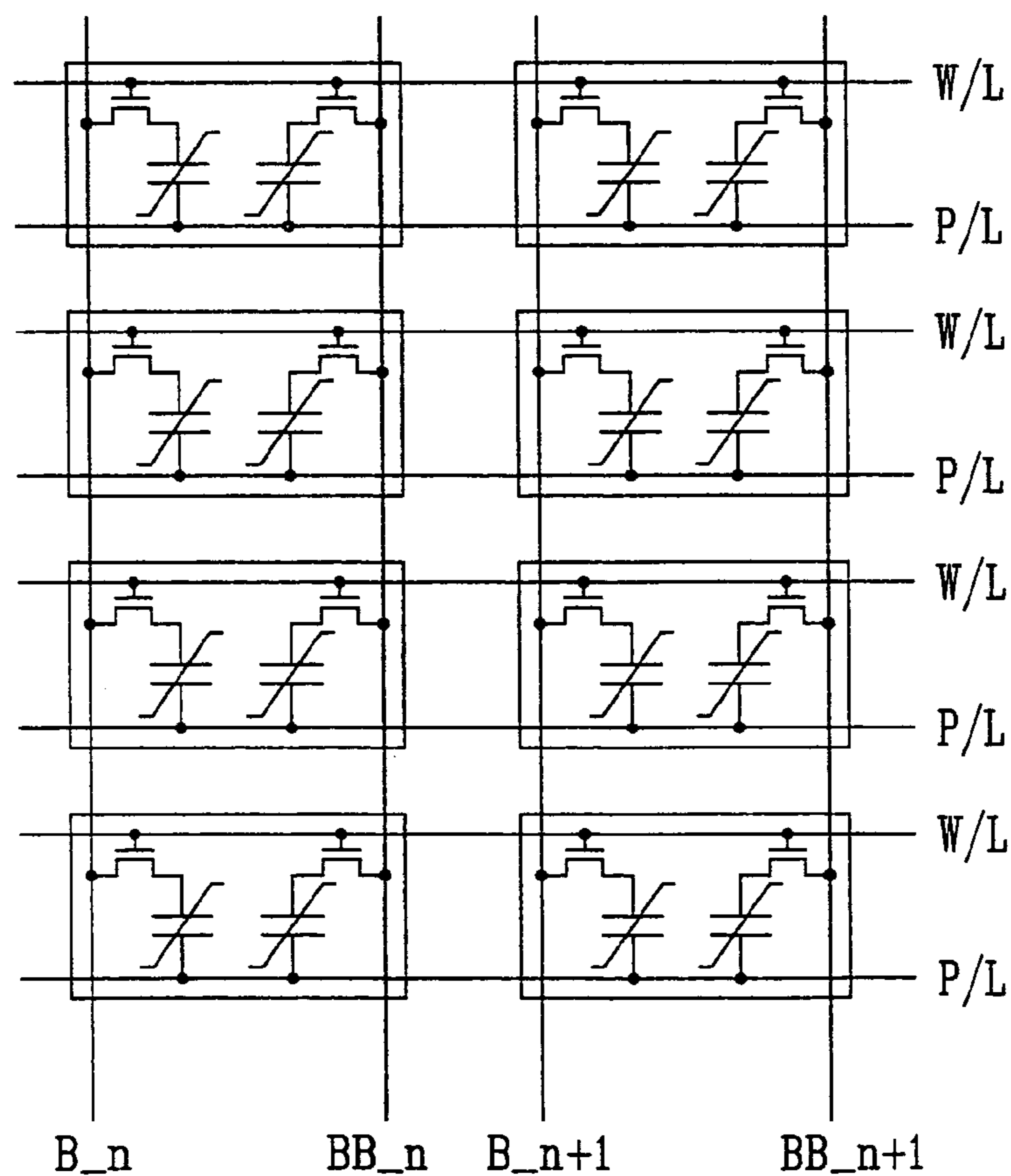
FIG.3 Related Art
