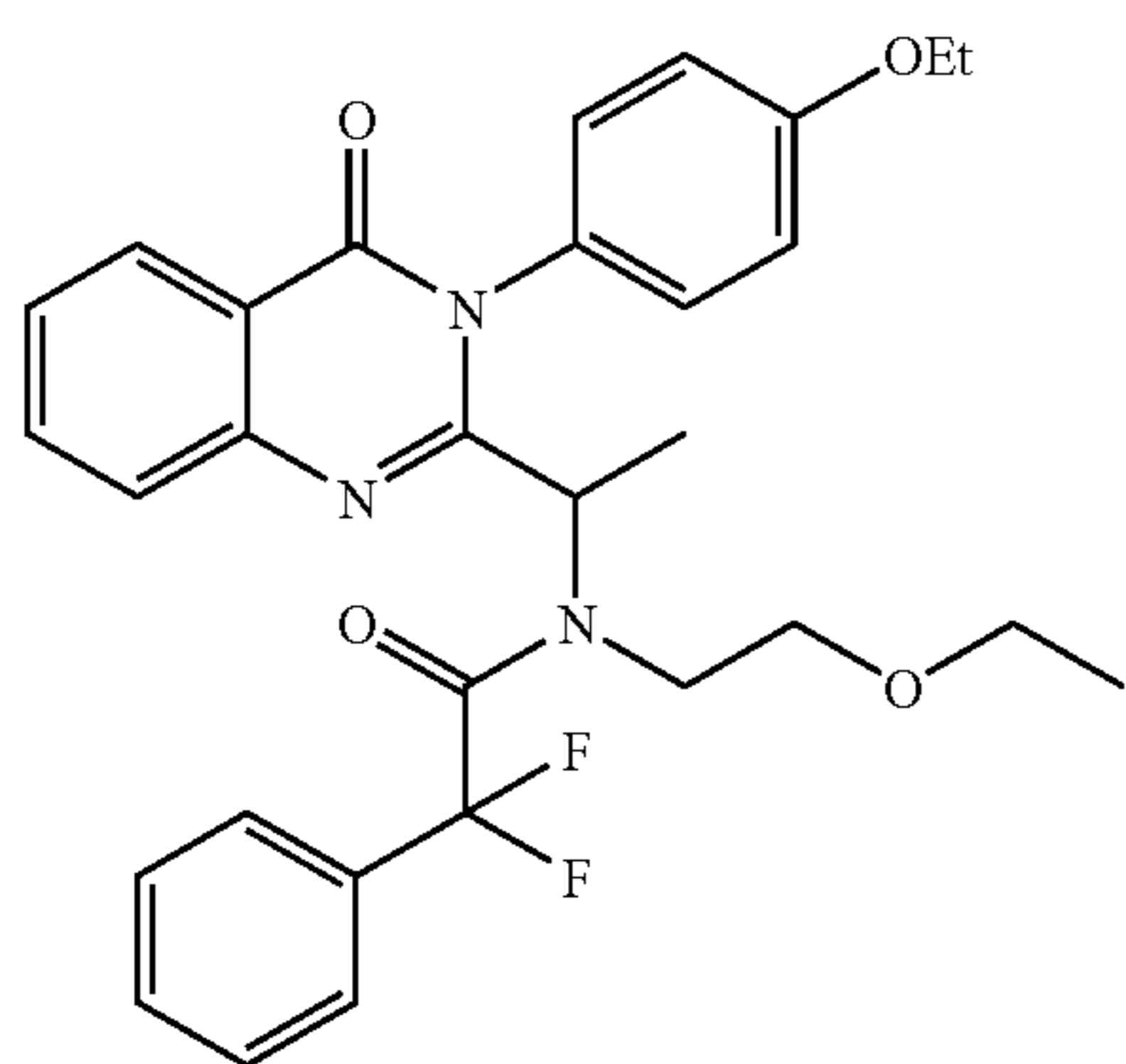
N-(2-Ethoxy-ethyl)-N-{1-[3-(4-ethoxy-phenyl)-4-oxo-3,4-dihydro-quinazolin-2-yl]-ethyl}-2,2-difluoro-2-phenylacetamide
