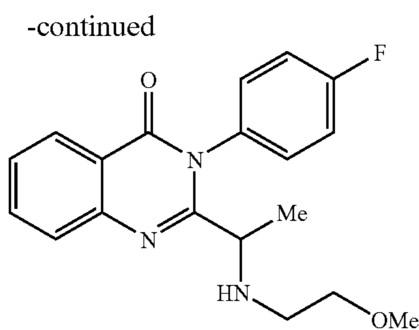
3-(4-Fluoro-phenyl)-2-[1-(2-methoxy-ethylamino)-ethyl]-3H-quinazolin-4-one (VI)
