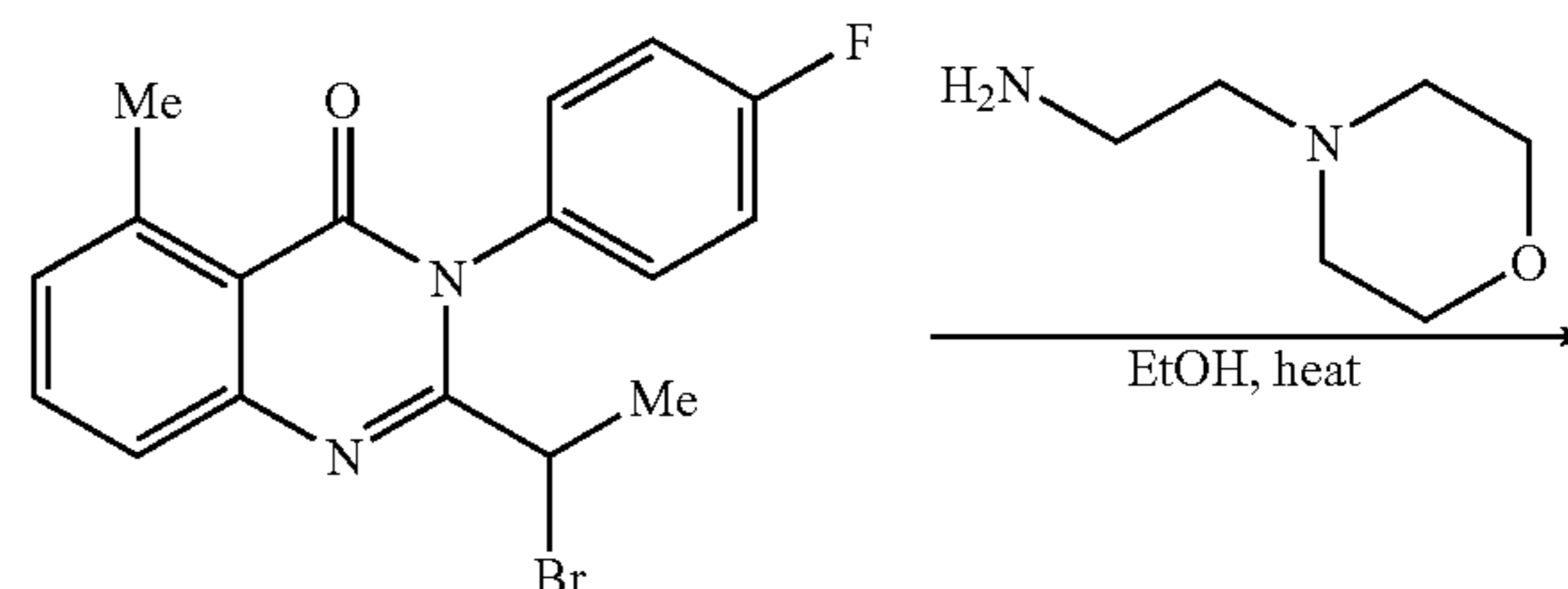
2-(1-Bromo-ethyl)-3-(4-fluoro-phenyl)-5-methyl-3H-quinazolin-4-one (X)
