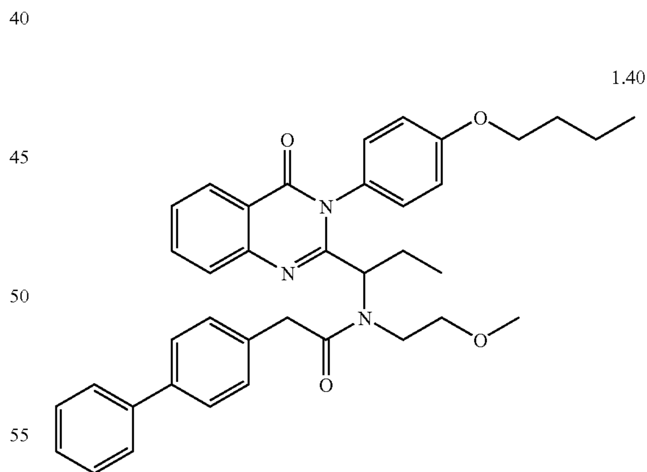
2-Biphenyl-4-yl-N-{1-[3-(4-butoxy-phenyl)-4-oxo-3,4-dihydro-quinazolin-2-yl]-propyl}-N-(2-methoxy-ethyl)-acetamide
