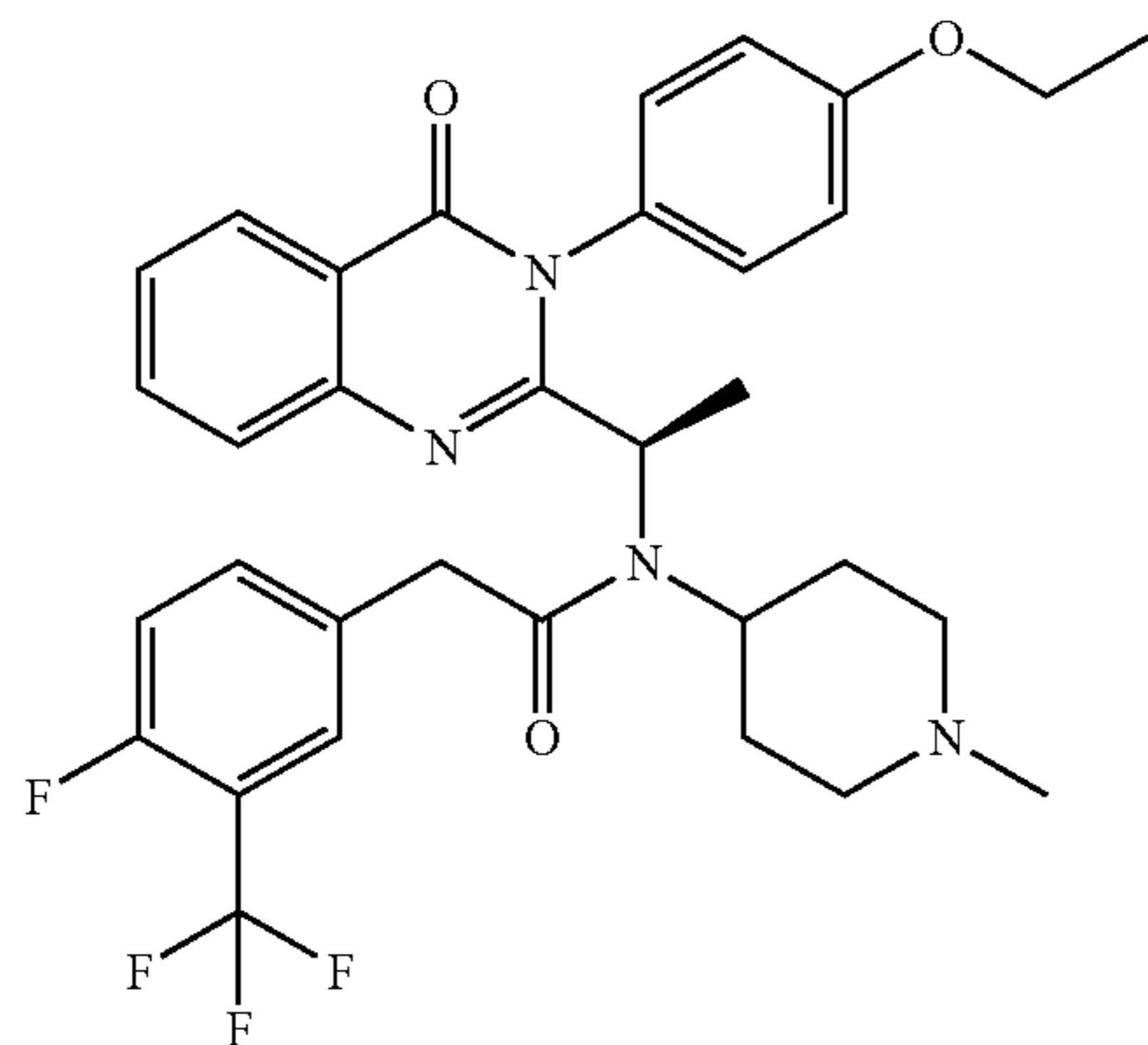
N-{1-[3-(4-Ethoxy-phenyl)-4-oxo-3,4-dihydro-quinazolin-2-yl]-ethyl}-2-(4-fluoro-3-trifluoromethyl-phenyl)-N-(1-methyl-piperidin-4-yl)-acetamide
