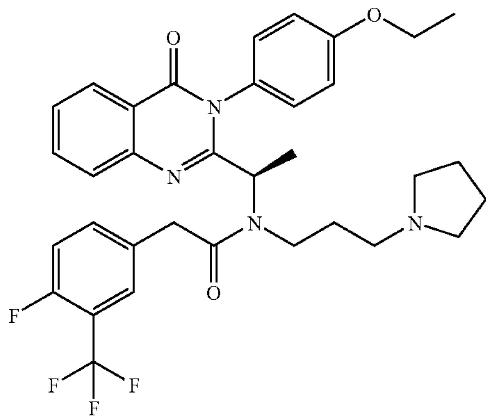
N-{1-[3-(4-Ethoxy-phenyl)-4-oxo-3,4-dihydro-quinazolin-2-yl]-ethyl}-2-(4-fluoro-3-trifluoromethyl-phenyl)-N-(3-pyrrolidin-1-yl-propyl)-acetamide
