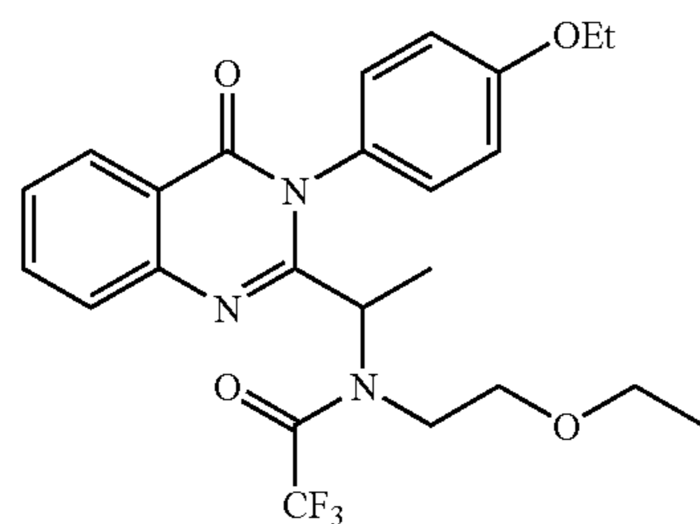
N-(2-Ethoxy-ethyl)-N-{1-[3-(4-ethoxyphenyl)-4-oxo-3,4-dihydro-quinazolin-2-yl]-ethyl}-2,2,2-trifluoroacetamide 1.55
