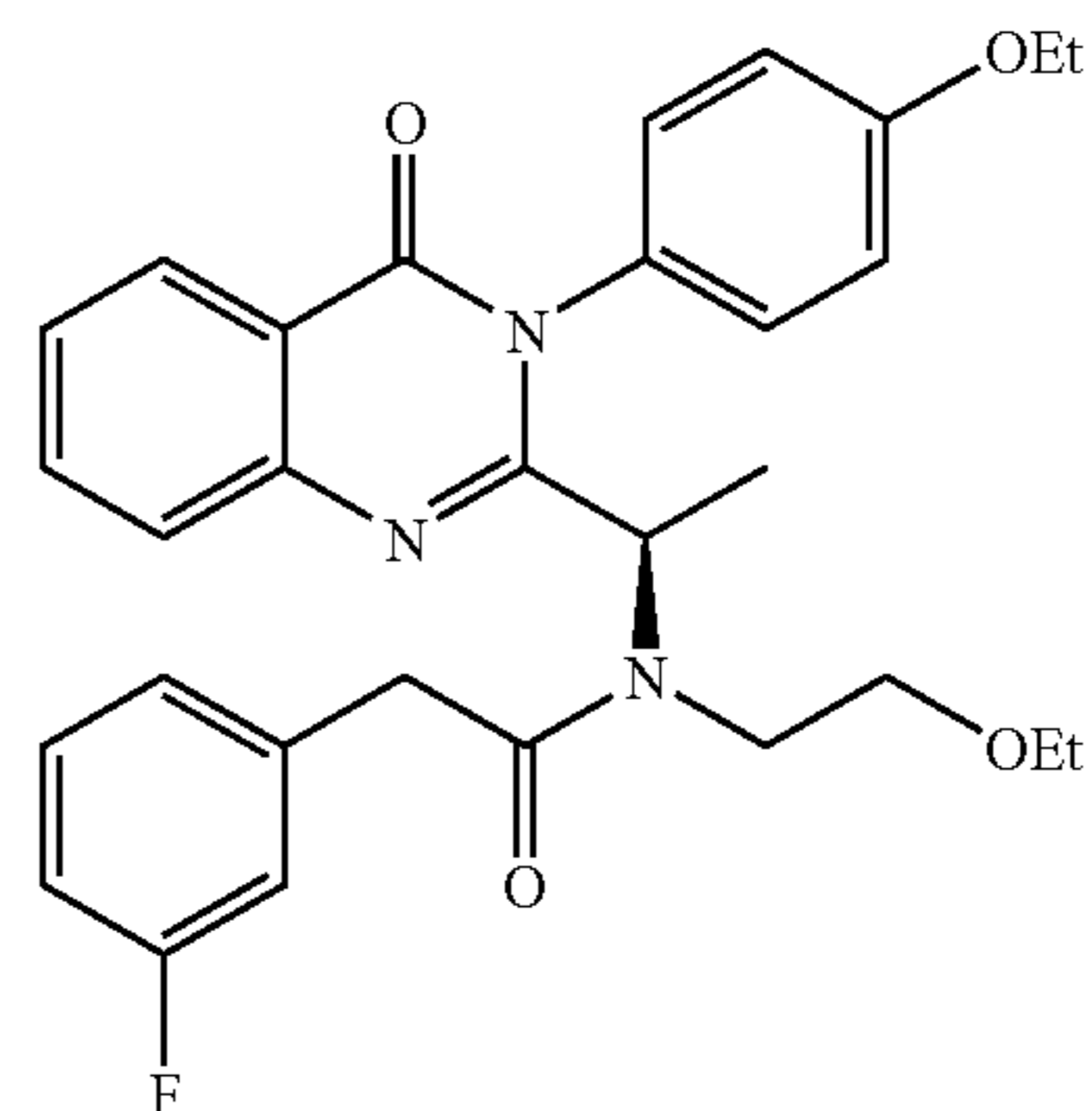
N-(2-Ethoxy-ethyl)-N-{1-[3-(4-ethoxy-phenyl)-4-oxo-3,4-dihydro-quinazolin-2-yl]-ethyl}-2-(3-fluoro-phenyl)-acetamide
