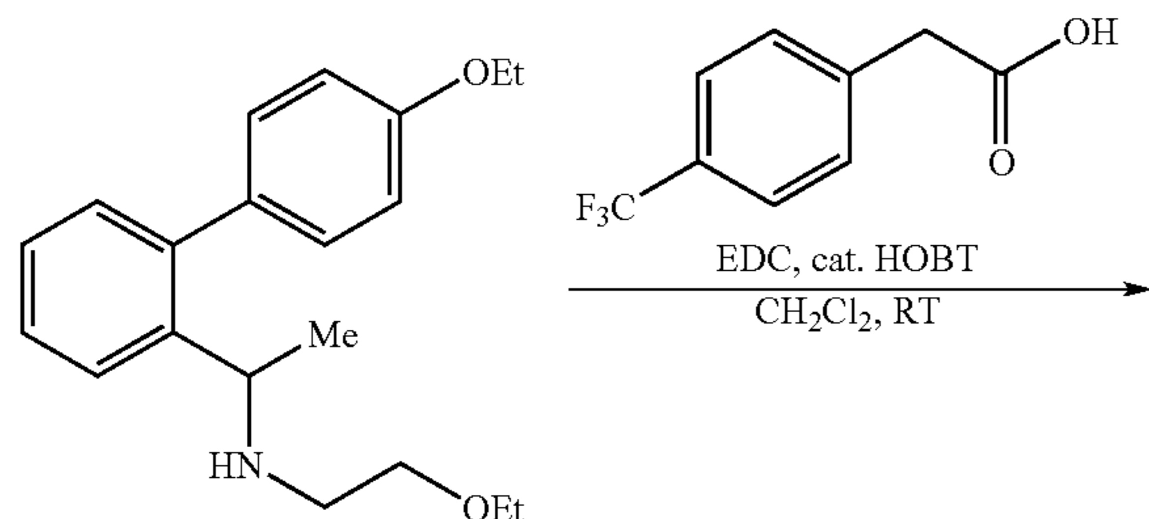
[1-(4'-Ethoxy-biphenyl-2-yl)-ethyl]- (2-ethoxy-ethyl)-amine
