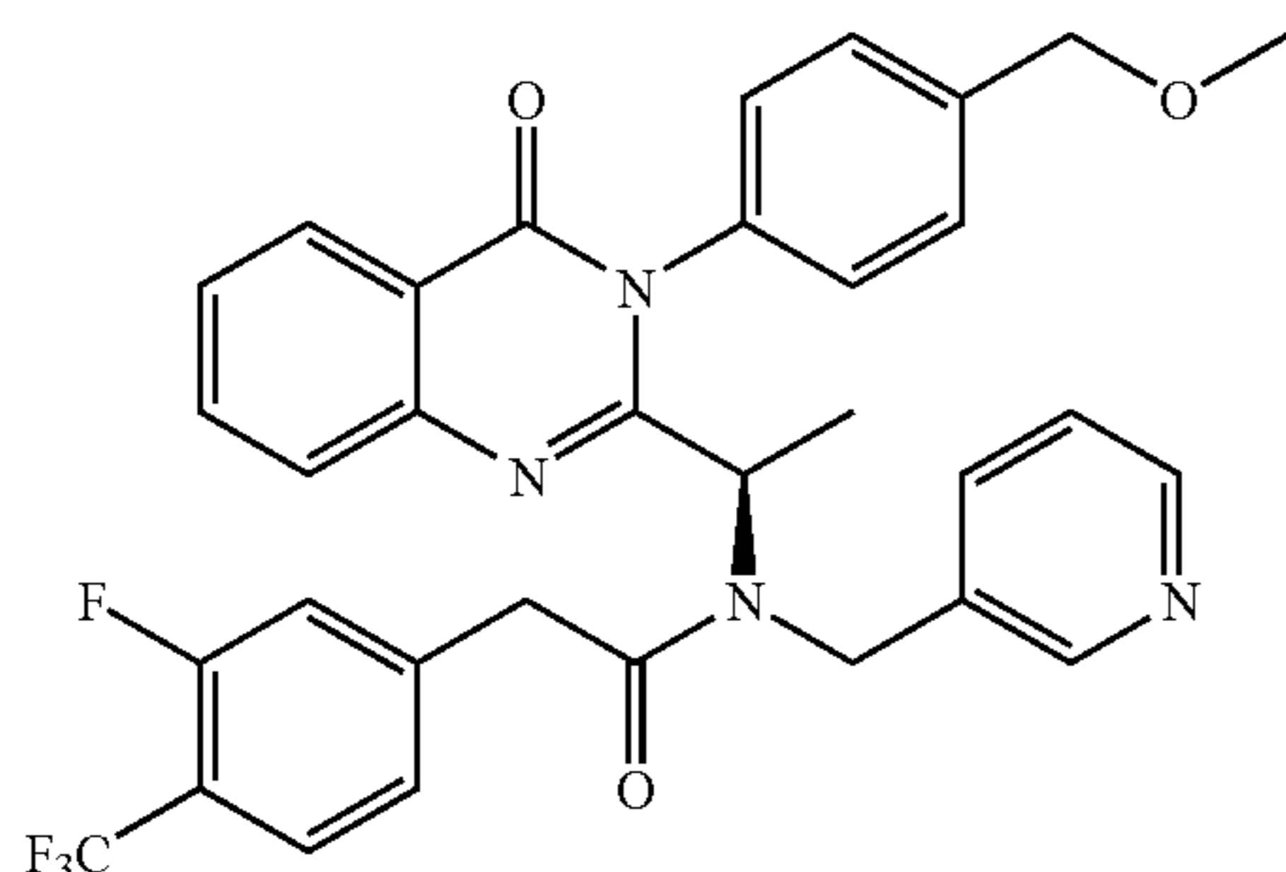
2-(3-Fluoro-4-trifluoromethyl-phenyl)-N-{1-[3-(4-methoxymethyl-phenyl)-4-oxo-3,4-dihydro-quinazolin-2-yl]-ethyl}-N-pyridin-3-ylmethyl-acetamide
