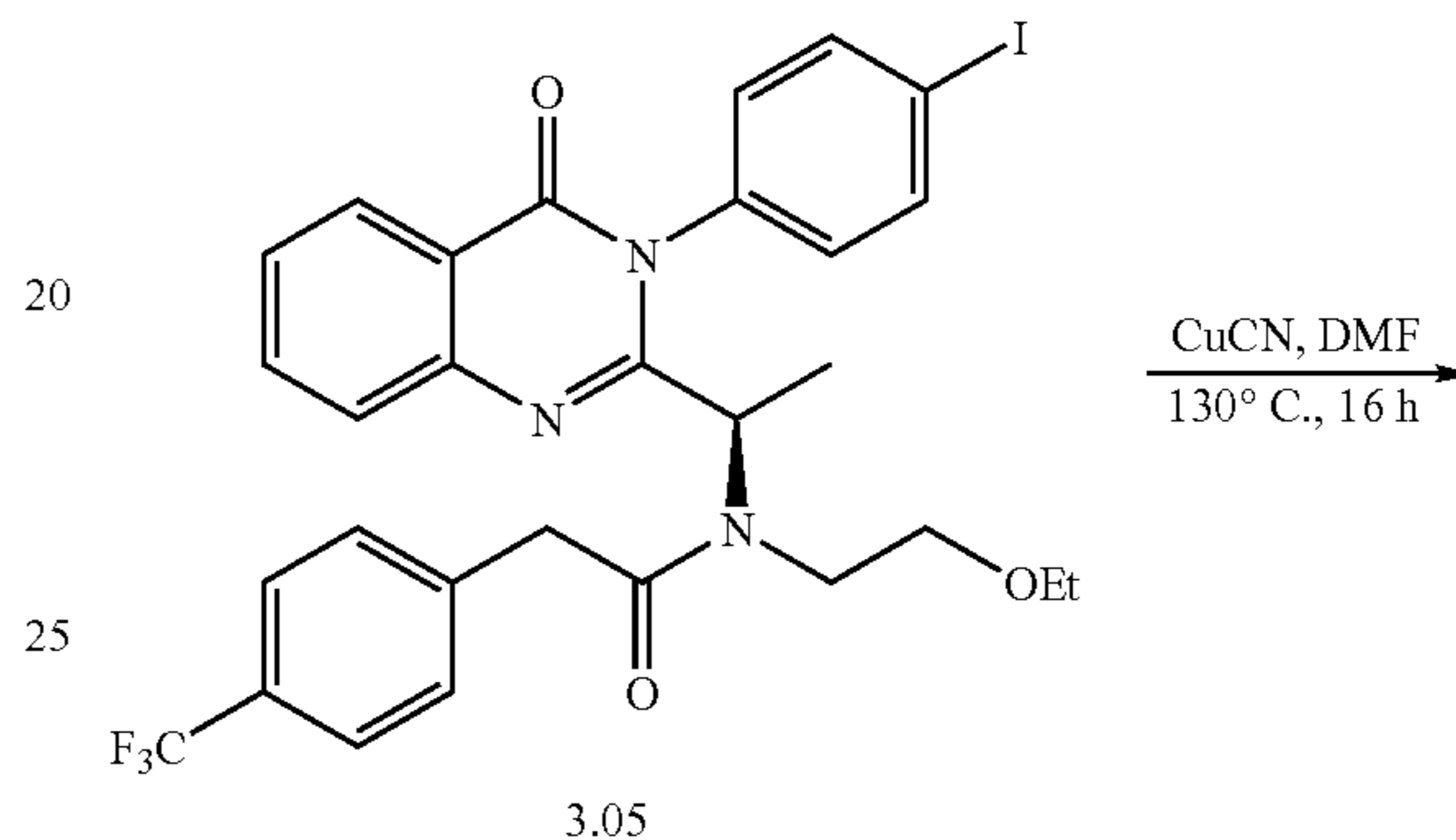
Scheme 6
