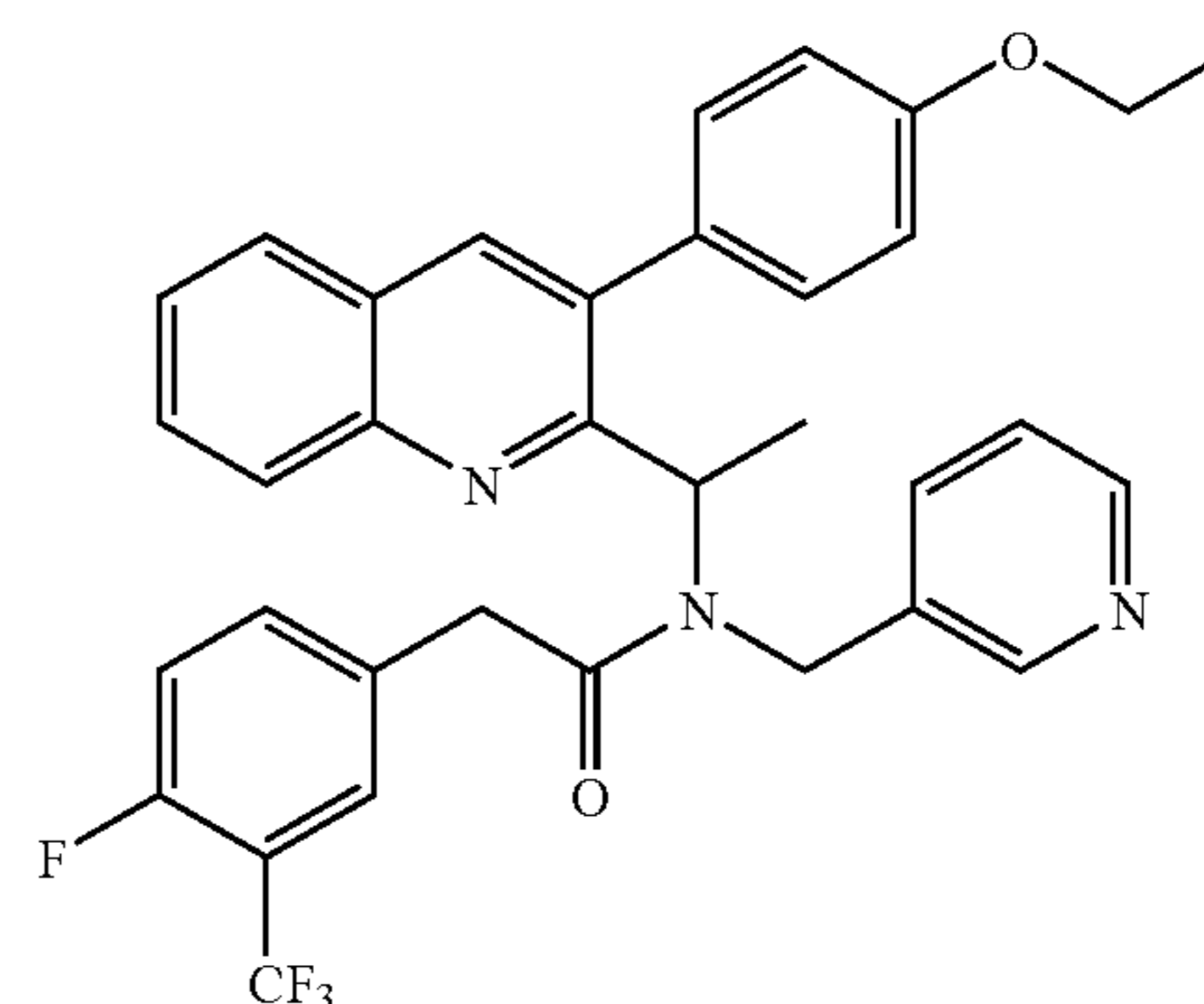
N-{1-[3-(4-Ethoxy-phenyl)-quinolin-2-yl]-ethyl}-2-(4-fluoro-3-trifluoromethyl-phenyl)-N-pyridin-3-ylmethyl-acetamide
