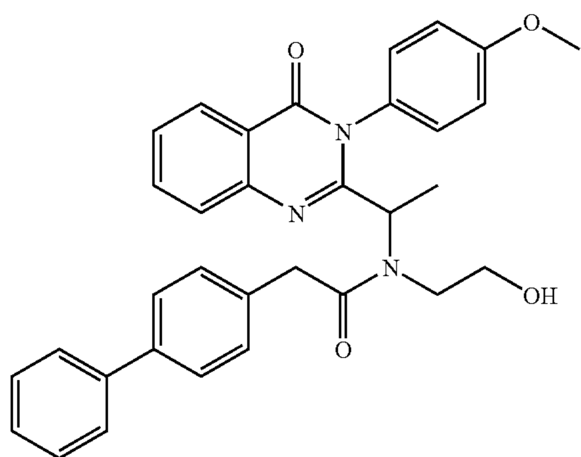
2-Biphenyl-4-yl-N-(2-hydroxy-ethyl)-N-{1-[3-(4-methoxy-phenyl)-4-oxo-3,4-dihydro-quinazolin-2-yl]-ethyl}-acetamide
