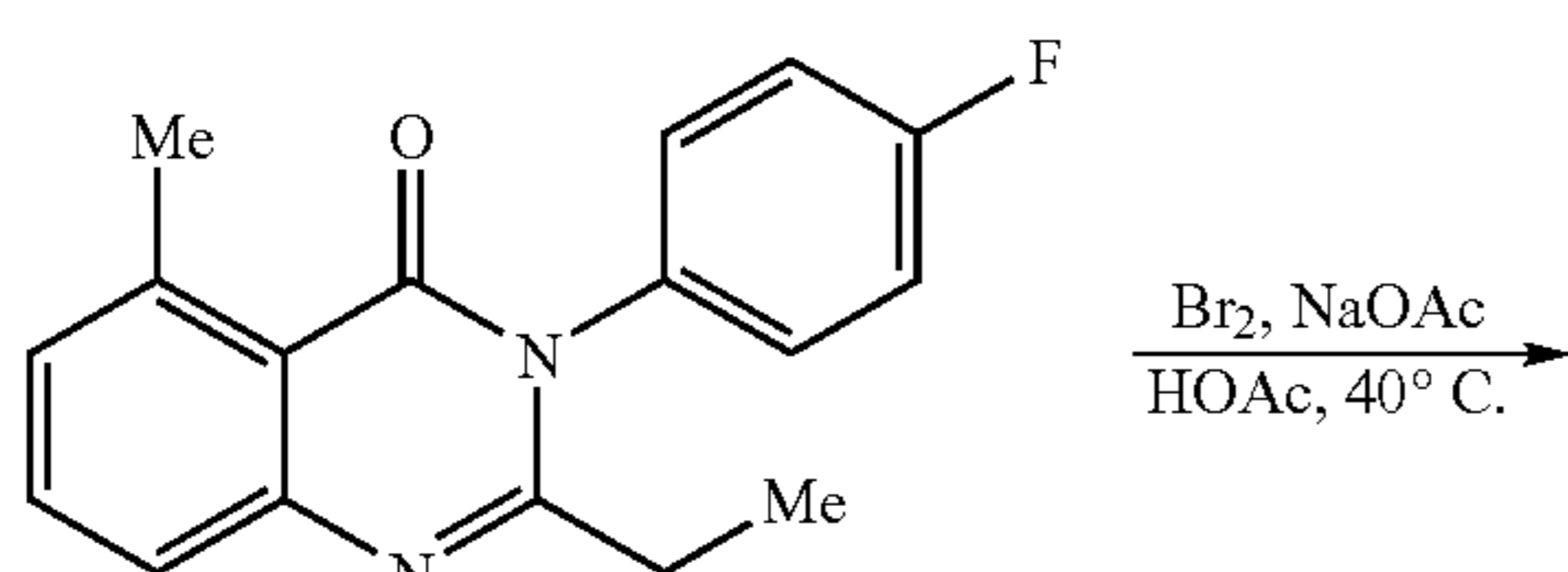
2-Ethyl-3-(4-fluoro-phenyl)-5-methyl-3H-quinazolin-4-one (IX)
