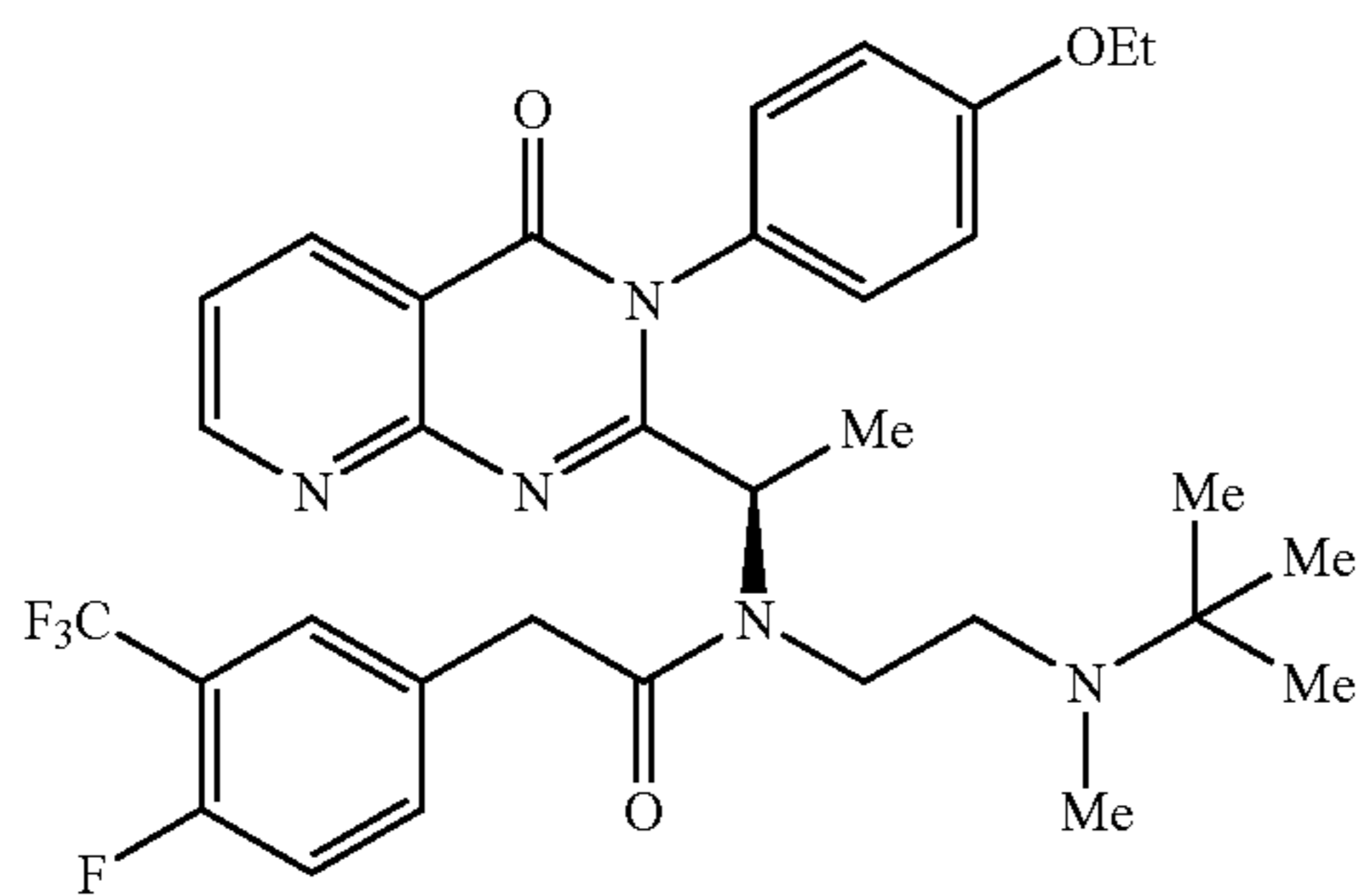
(R)-N-[2-(tert-Butyl-methyl-amino)-ethyl]-N-{1-[3-(4-ethoxy-phenyl)-4-oxo-3,4-dihydro-pyrido[2,3-d]pyrimidin-2-yl]-ethyl}-2-(4-fluoro-3-trifluoromethyl-phenyl)-acetamide
