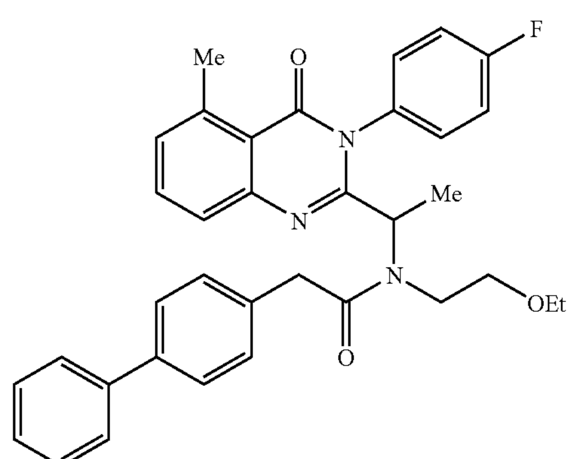
2-Biphenyl-4-yl-N-(2-ethoxy-ethyl)-N-(1-[5-methyl-3-(4-fluoro-phenyl)-4-oxo-3,4-dihydro-quinazolin-2-yl]-ethyl)-acetamide
