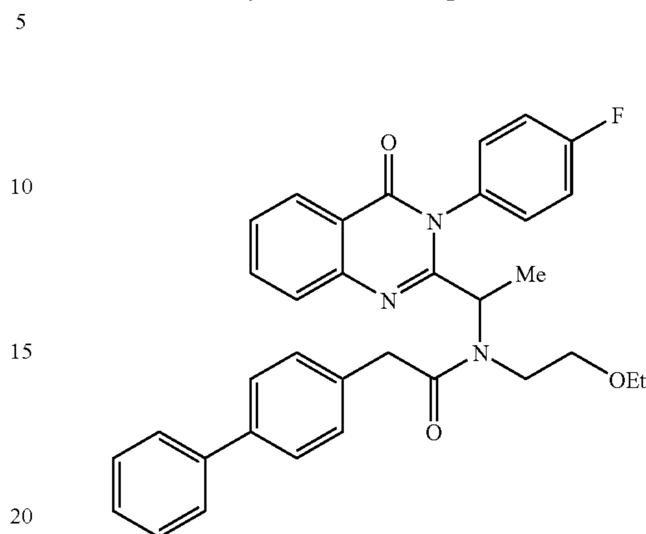
2-Biphenyl-4-yl-N-(2-ethoxy-ethyl)-N-{1-[3-(4-fluoro-phenyl)-4-oxo-3,4-dihydro-quinazolin-2-yl]-ethyl}-acetamide (1.19)
