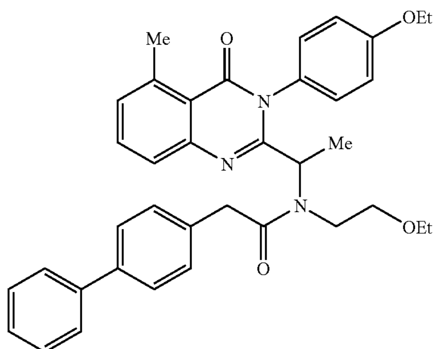
2-Biphenyl-4-yl-N-(2-ethoxy-ethyl)-N-(1-[3-(4-ethoxy-phenyl)-5-methyl-4-oxo-3,4-dihydro-quinazolin-2-yl]-ethyl)-acetamide
