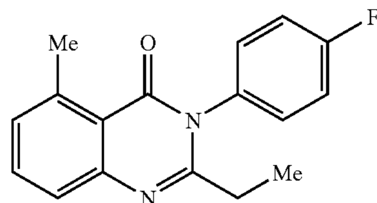
2-Ethyl-3-(4-fluoro-phenyl)-5-methyl-3H-quinazolin-4-one (IX)
