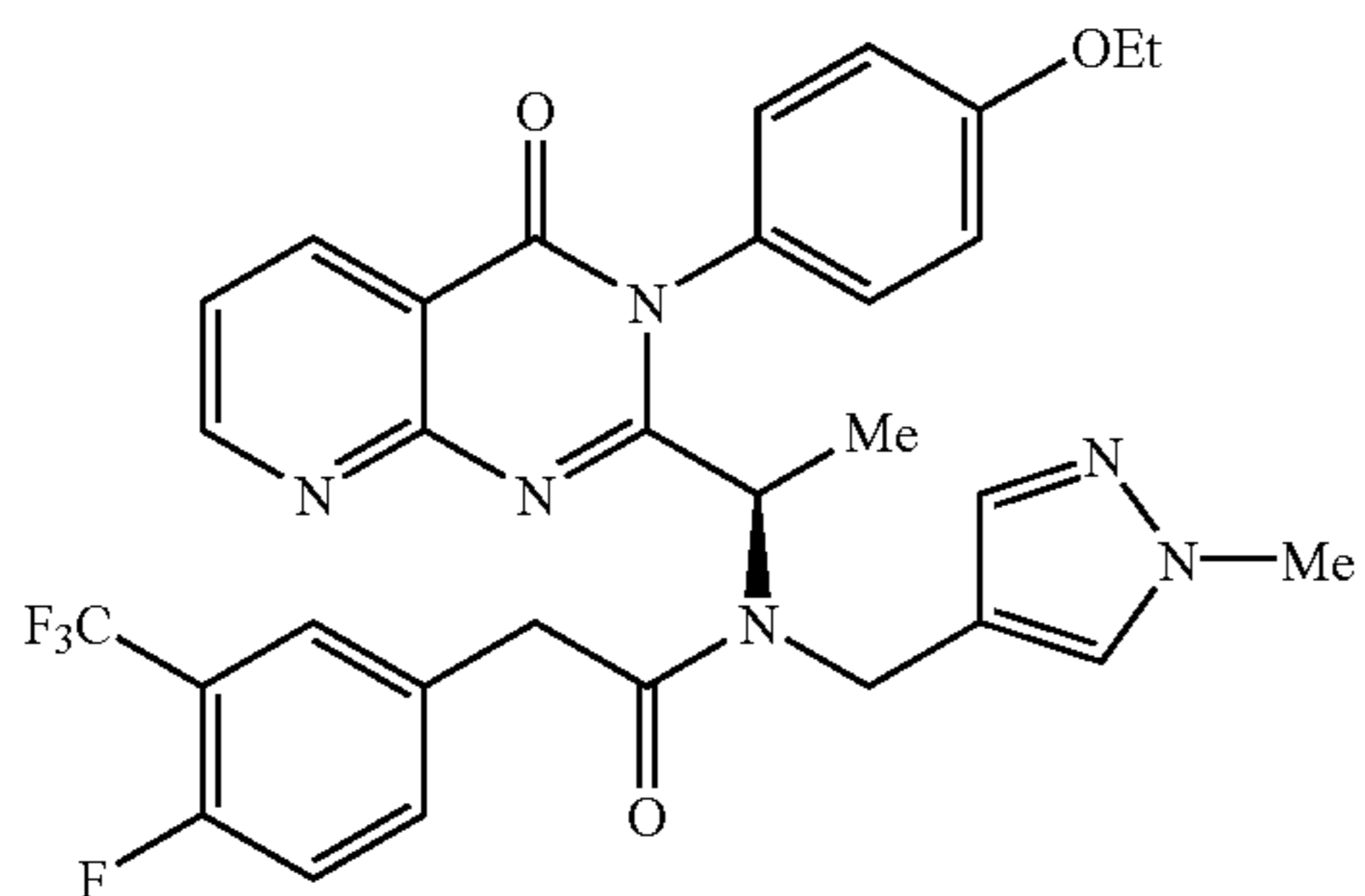
(R)-N-{1-[3-(4-Ethoxy-phenyl)-4-oxo-3,4-dihydro-pyrido[2,3-d]pyrimidin-2-yl]-ethyl}-2-(4-fluoro-3-trifluoromethyl-phenyl)-N-(1-methyl-1H-pyrazol-4-ylmethyl)-acetamide
