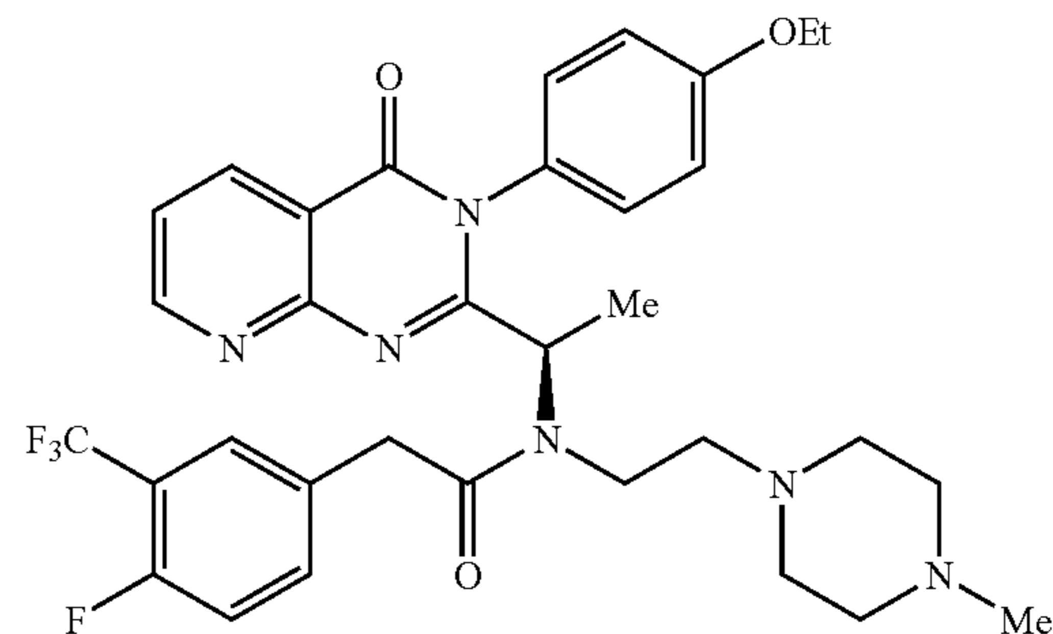
(R)-N-(1-[3-(4-Ethoxy-phenyl)-4-oxo-3,4-dihydro-pyrido[2,3-d]pyrimidin-2-yl]-ethyl)-2-(4-fluoro-3-trifluoromethyl-phenyl)-N-[2-(4-methyl-piperazin-1-yl)-ethyl]-acetamide
