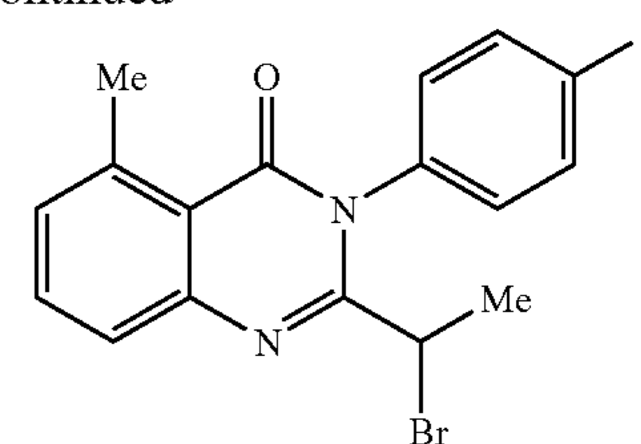
2-(1-Bromo-ethyl)-3-(4-fluoro-phenyl)-5-methyl-3H-quinazolin-4-one (X)
