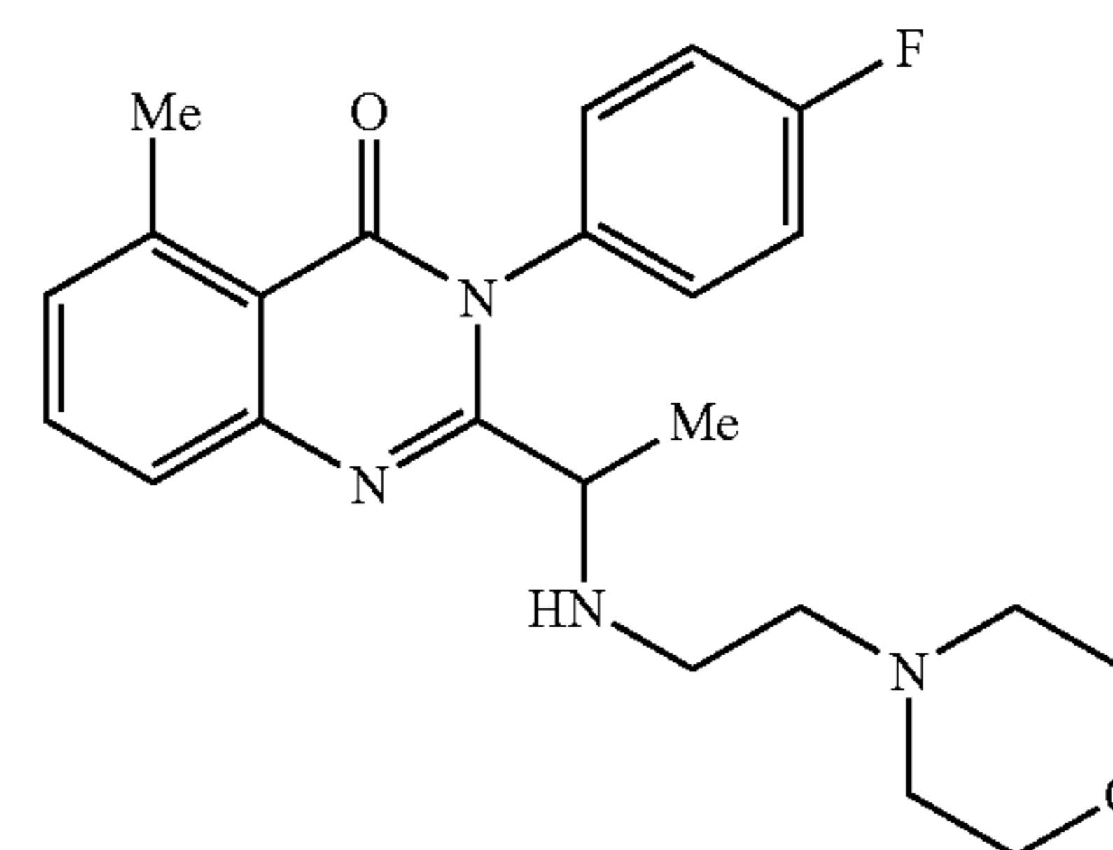
3-(4-Fluoro-phenyl)-5-methyl-2-[1-(2-morpholin-4-yl-ethylamino)-ethyl]-3H-quinazolin-4-one (XI)
