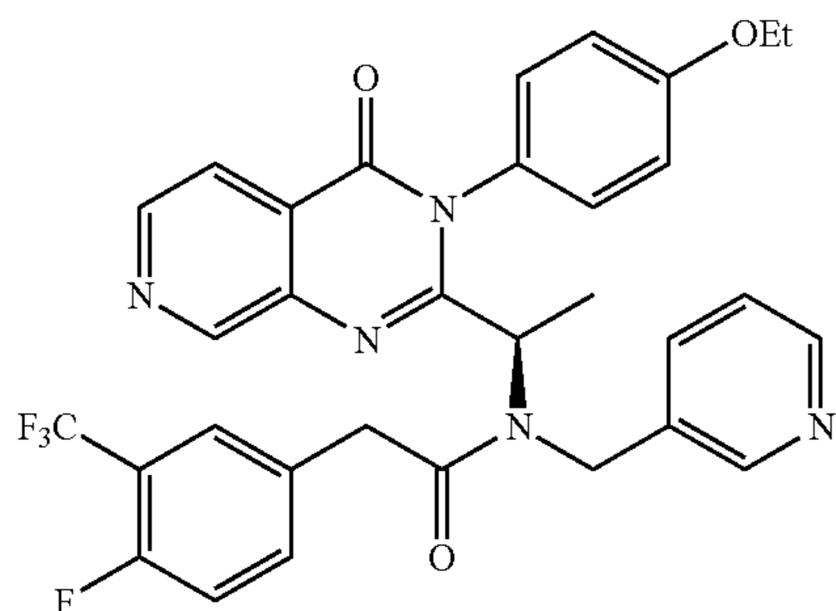
N-{1-[3-(4-Ethoxy-phenyl)-4-oxo-3,4-dihydro-pyrido[3,4-d]pyrimidin-2-yl]-ethyl}-2-(4-fluoro-3-trifluoromethyl-phenyl)-N-pyridin-3-ylmethyl-acetamide
