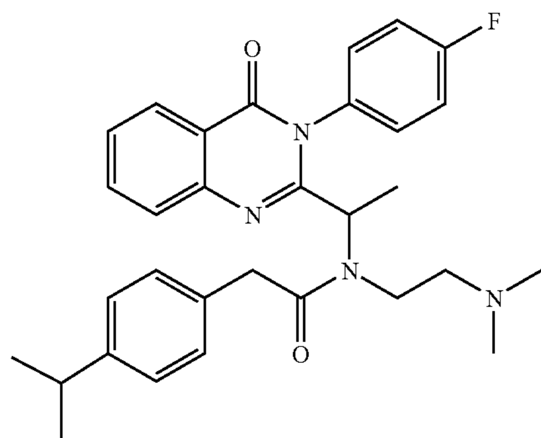
N-(2-Dimethylamino-ethyl)-N-{1-[3-(4-fluorophenyl)-4-oxo-3,4-dihydro-quinazolin-2-yl]-ethyl}-2-(4-isopropyl-phenyl)-acetamide
