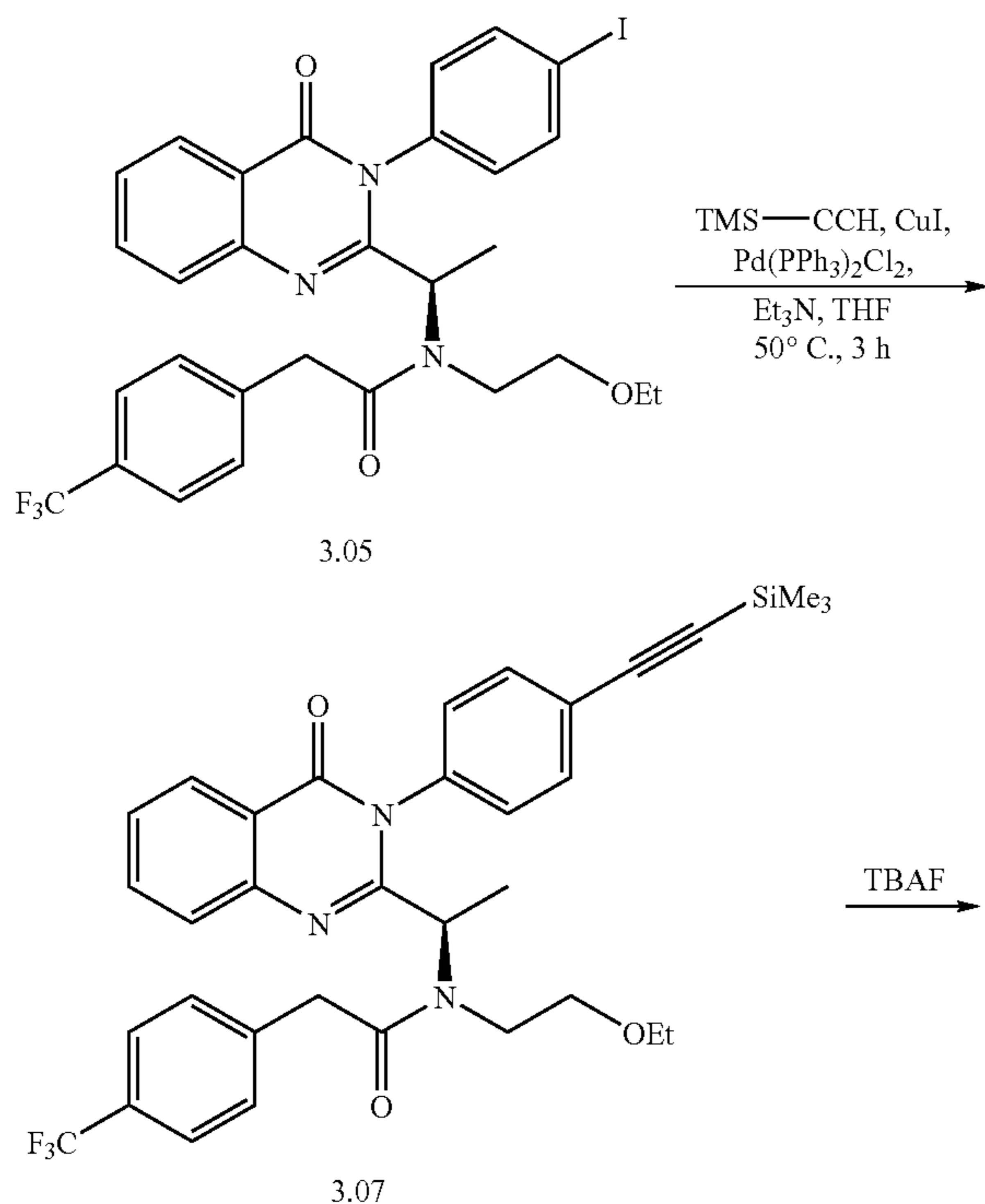
Scheme 7
