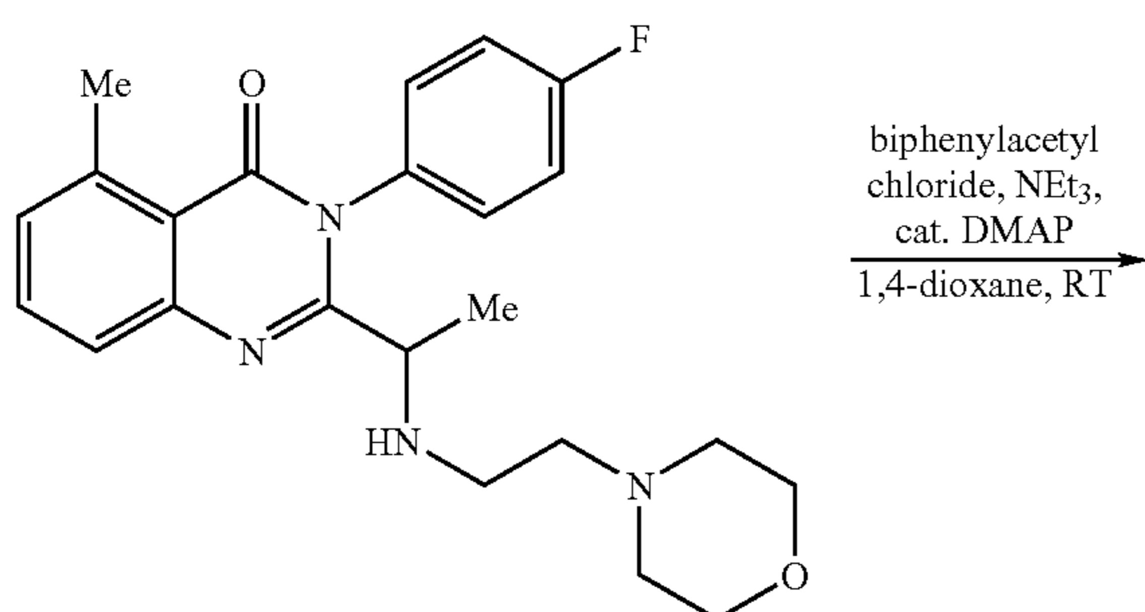
3-(4-Fluoro-phenyl)-5-methyl-2-[1-(2-morpholin-4-yl-ethylamino)-ethyl]-3H-quinazolin-4-one (XI)
