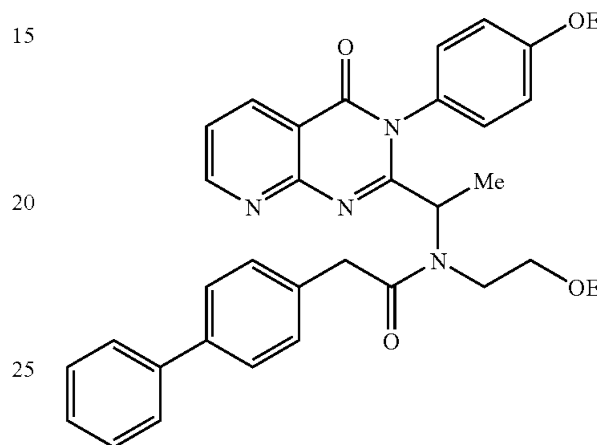
2-Biphenyl-4-yl-N-(2-ethoxy-ethyl)-N-(1-[3-(4-ethoxy-phenyl)-4-oxo-3,4-dihydro-pyrido[2-3-d]pyrimidin-2-yl]-ethyl)-acetamide
