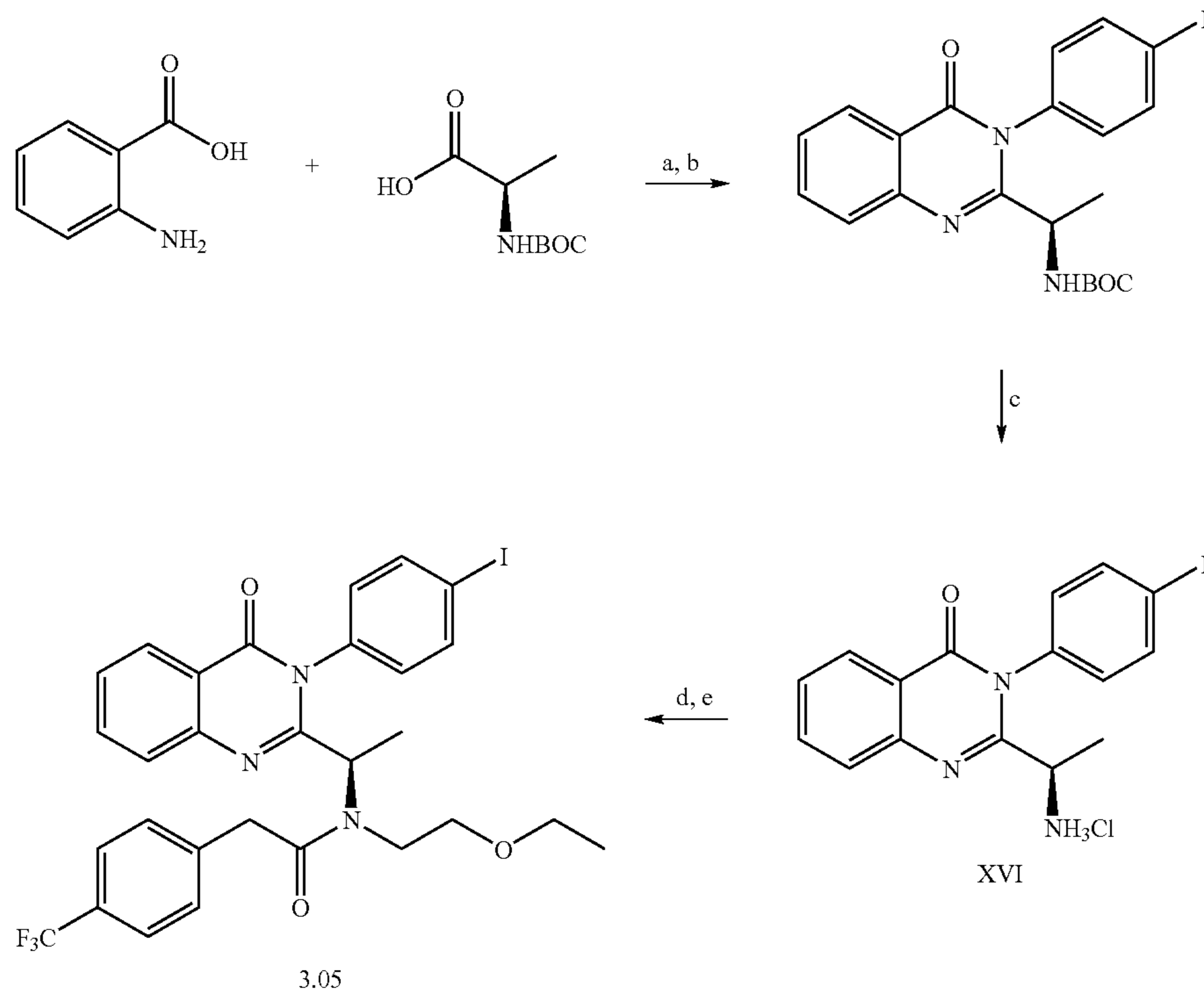
Scheme 5
