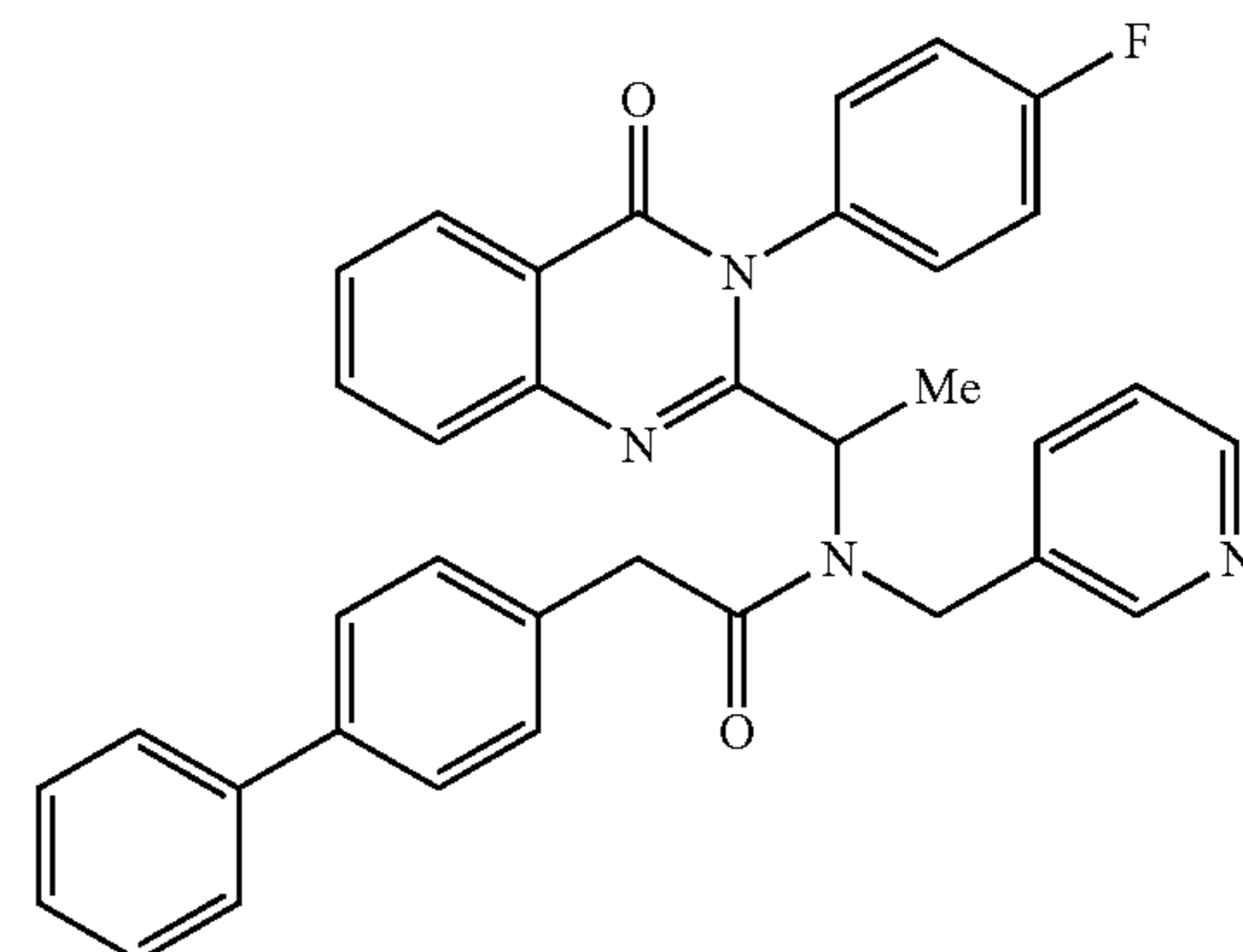
2-Biphenyl-4-yl-N-(1-[3-(4-fluoro-phenyl)-4-oxo-3,4-dihydro-quinazolin-2-yl]-ethyl)-N-pyridin-3-ylmethyl-acetamide
