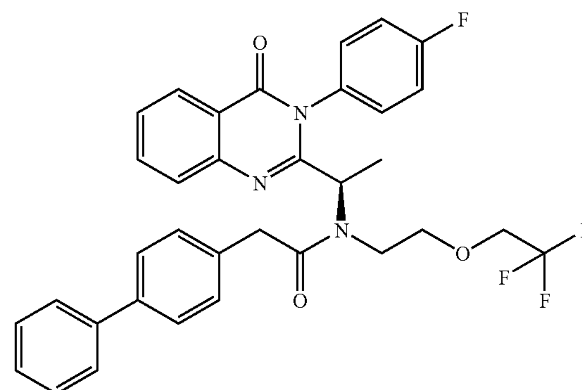
2-Biphenyl-4-yl-N-{1-[3-(4-fluoro-phenyl)-4-oxo-3,4-dihydro-quinazolin-2-yl]-ethyl}-N-[2-(2,2,2-trifluoroethoxy)-ethyl]-acetamide
