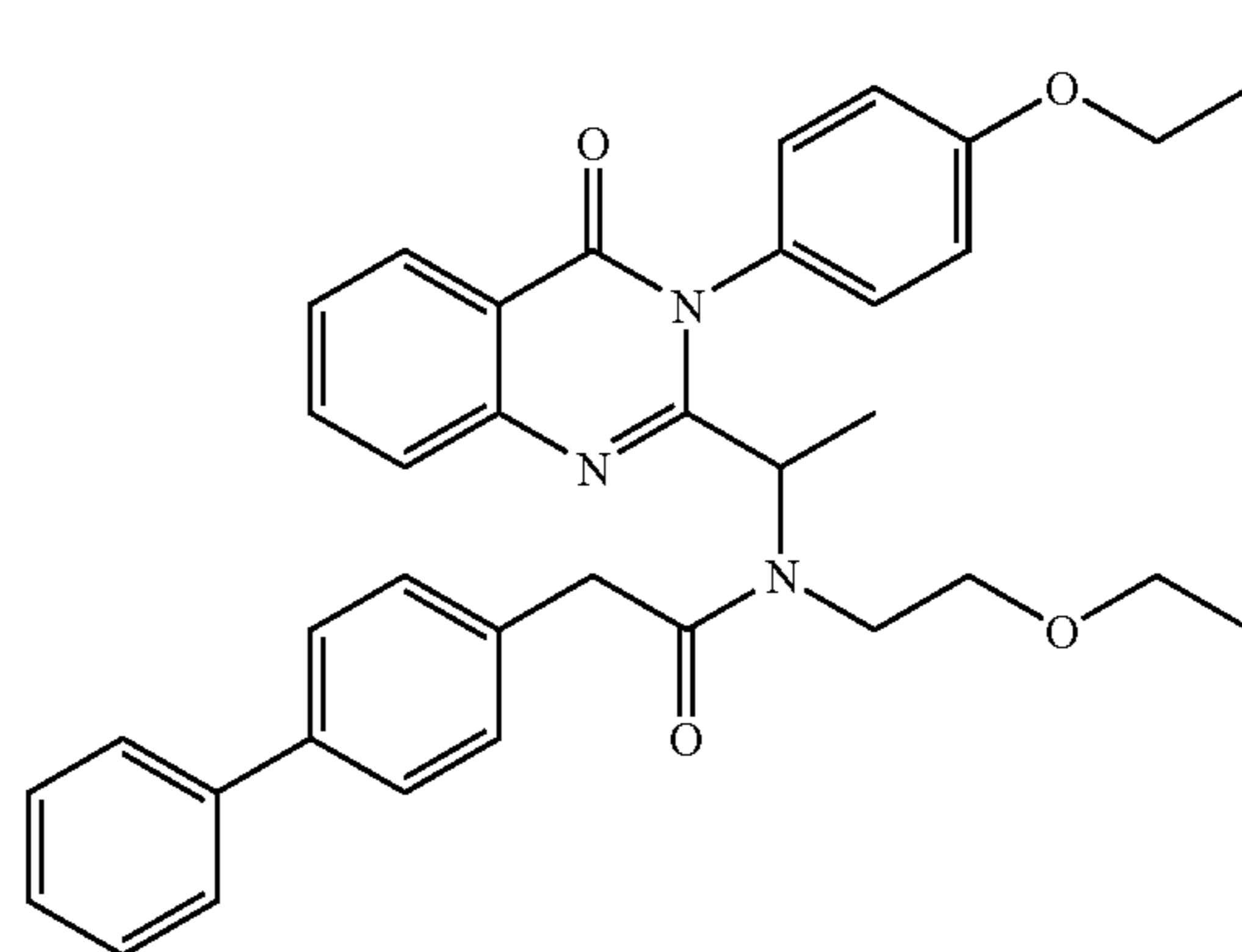
2-Biphenyl-4-yl-N-(2-ethoxy-ethyl)-N-{1-[3-(4-ethoxy-phenyl)-4-oxo-3,4-dihydro-quinazolin-2-yl]-ethyl}-acetamide
