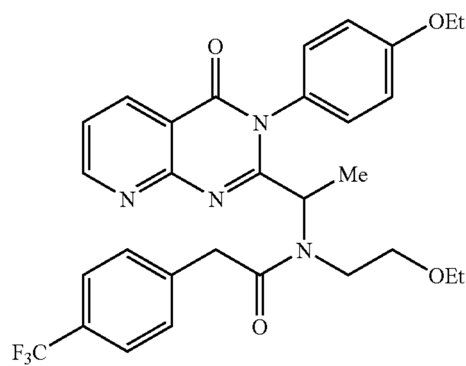
N-(2-Ethoxy-ethyl)-N-(1-[3-(4-ethoxy-phenyl)4-oxo-3,4-dihydro-pyrido[2,3-0]pyrimidin-2-yl]-ethyl)-2-(4-trifluoromethyl-phenyl)-acetamide
