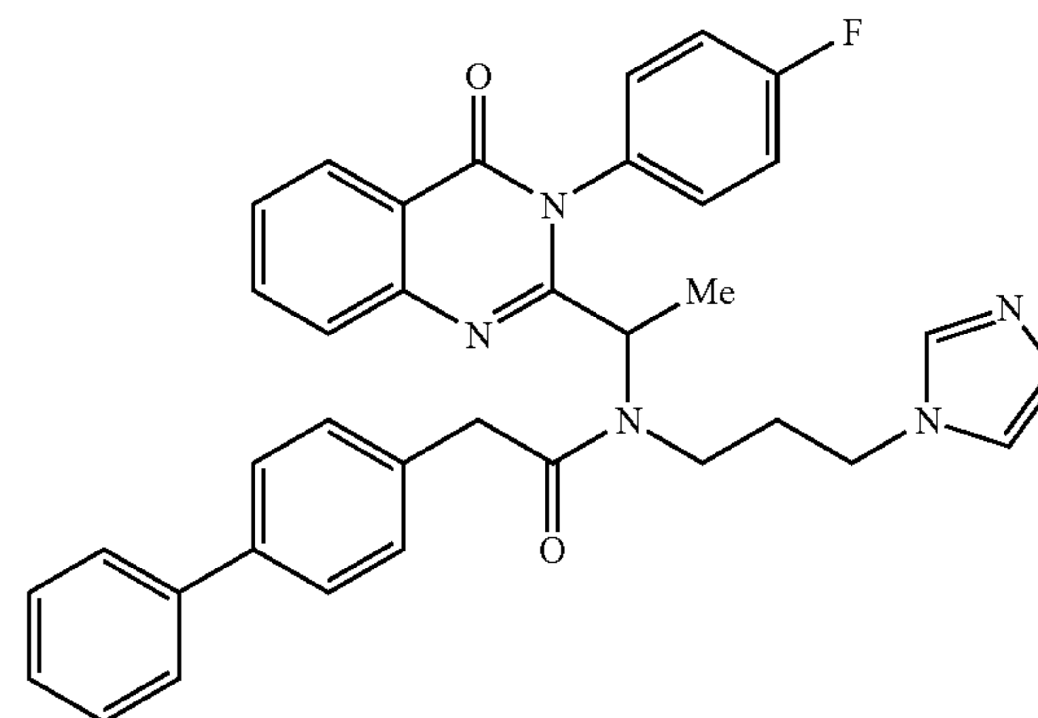
2-Biphenyl-4-yl-N-(1-[3-(4-fluoro-phenyl)-4-oxo-3,4-dihydro-quinazolin-2-yl]-ethyl)-N-(3-imidazol-1-yl-propyl)-acetamide
