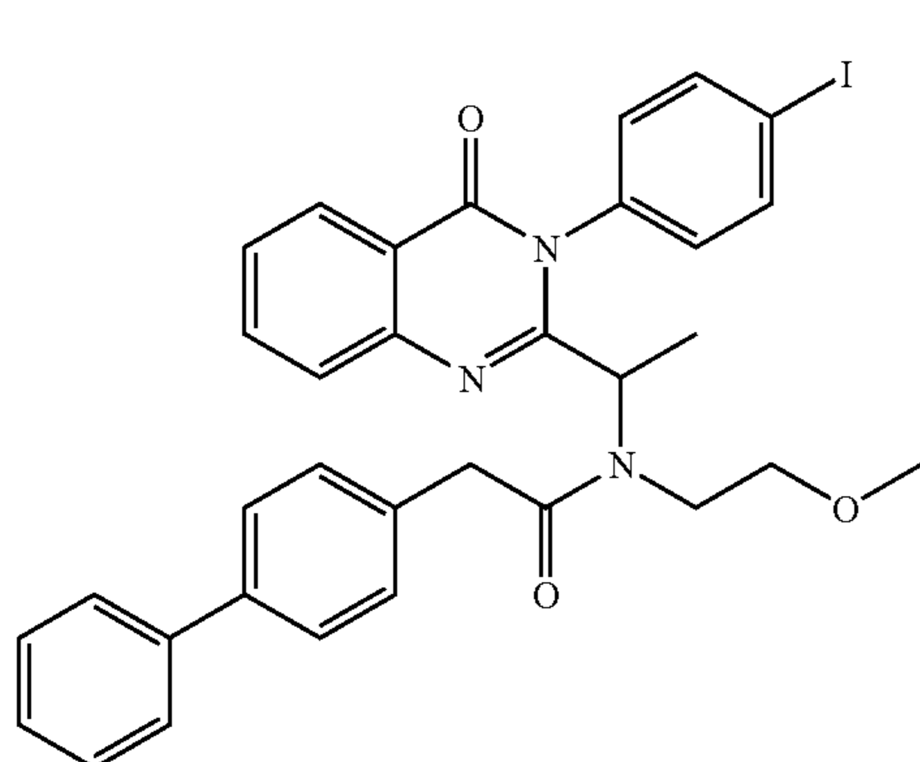
2-Biphenyl-4-yl-N-(1-[3-(4-iodo-phenyl)-4-oxo-3,4-dihydro-quinazolin-2-yl]-ethyl)-N-(2-methoxy-ethyl)-acetamide
