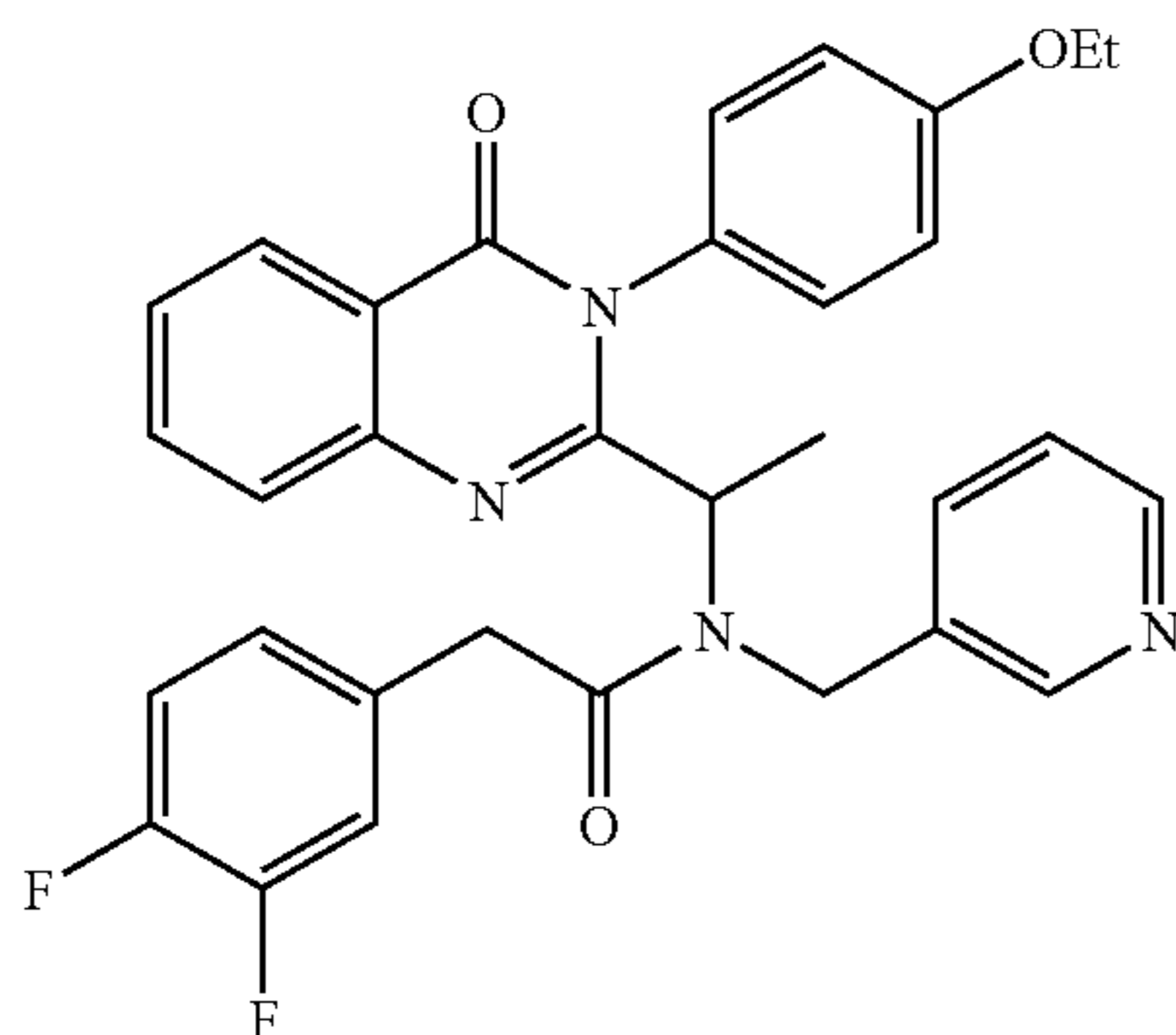
2-(3,4-Difluoro-phenyl)-N-{1-[3-(4-ethoxy-phenyl)-4-oxo-3,4-dihydro-quinazolin-2-yl]-ethyl}-N-pyridin-3-ylmethyl-acetamide
