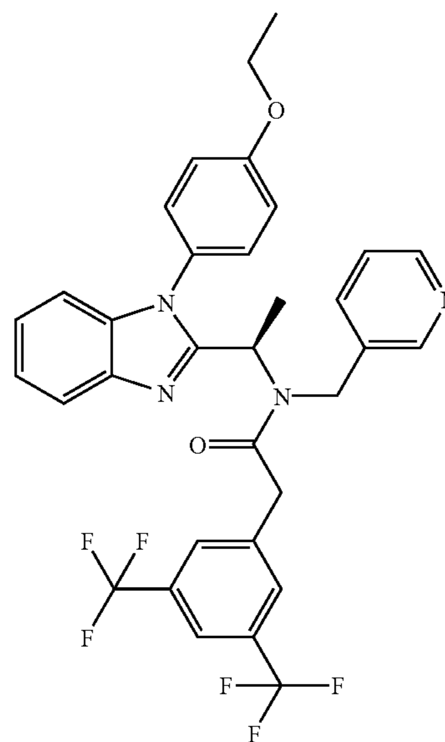
2-(3,5-Bis-trifluoromethyl-phenyl)-N-{1-[1-(4-ethoxy-phenyl)-1H-benzoimidazol-2-yl]-ethyl}-N-pyridin-3-ylmethyl-acetamide
