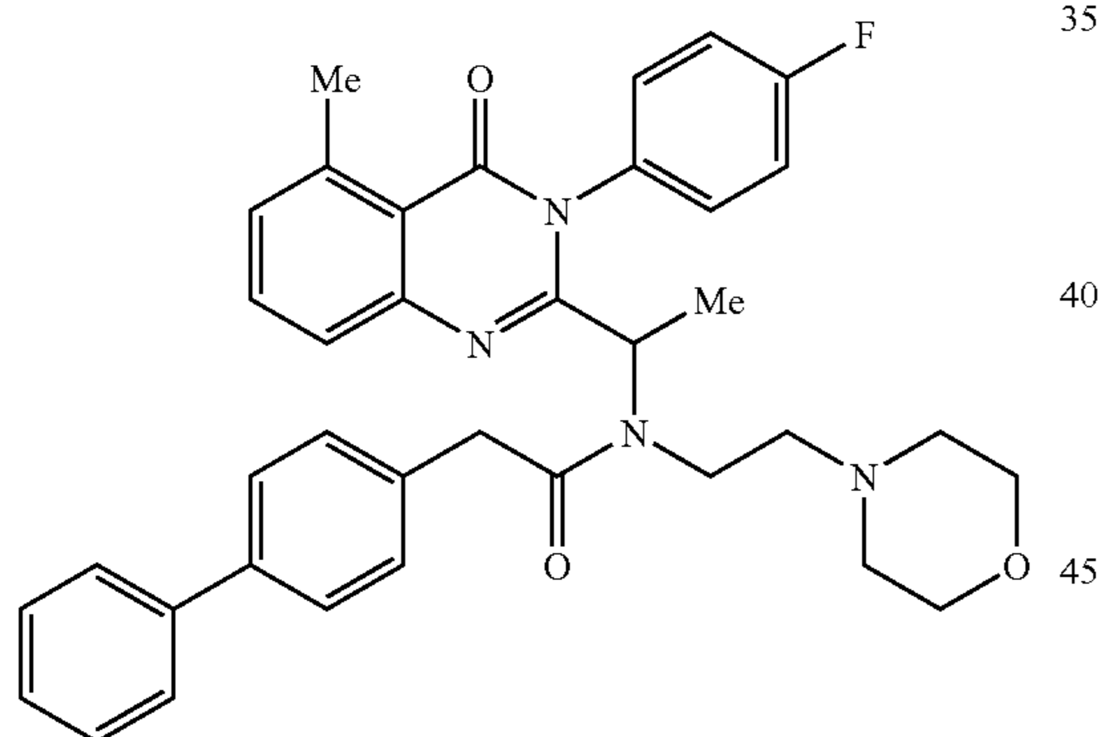
2-Biphenyl-4-yl-N-{1-[3-(4-fluoro-phenyl)-5-methyl-4-oxo-3,4-dihydro-quinazolin-2-yl]-ethyl}-N-(2-morpholin-4-yl-ethyl)-acetamide (2.01)
