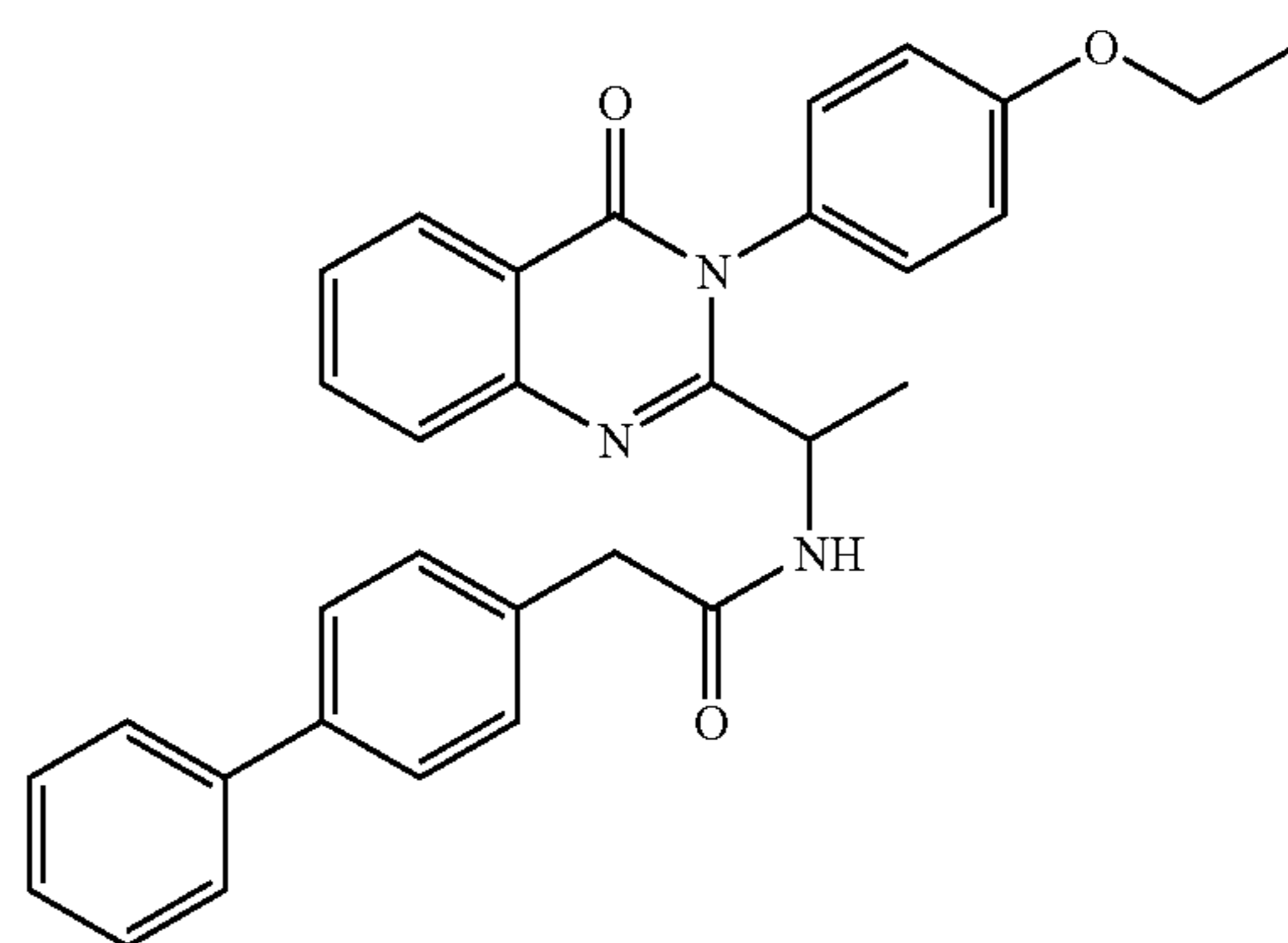
2-Biphenyl-4-yl-N-{1-[3-(4-ethoxy-phenyl)-4-oxo-3,4-dihydro-quinazolin-2-yl]-ethyl}-acetamide
