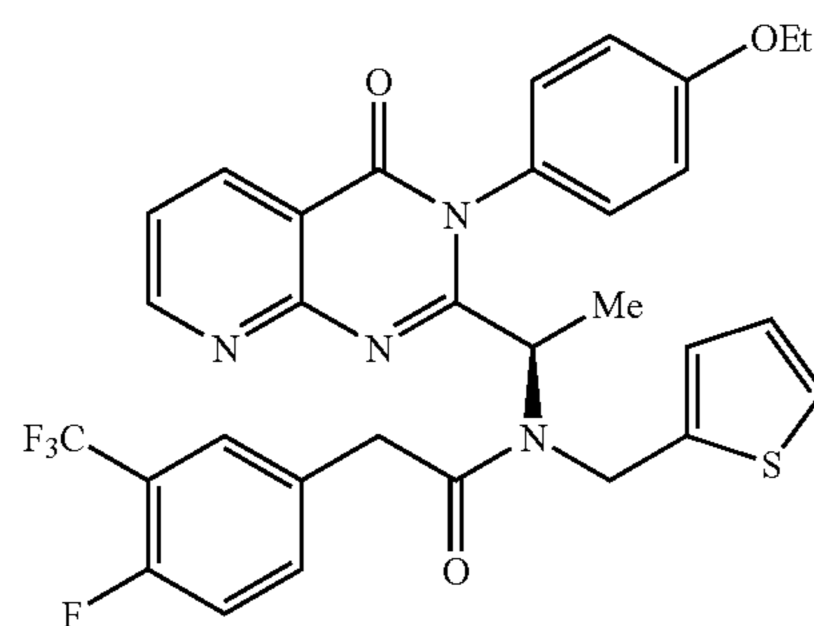
(R)-N-(1-[3-(4-Ethoxy-phenyl)-4-oxo-3,4-dihydro-pyrido[2,3-d]pyrimidin-2-yl]-ethyl)-2-(4-fluoro-3-trifluoromethyl-phenyl)-N-thiophen-2-ylmethyl-acetamide
