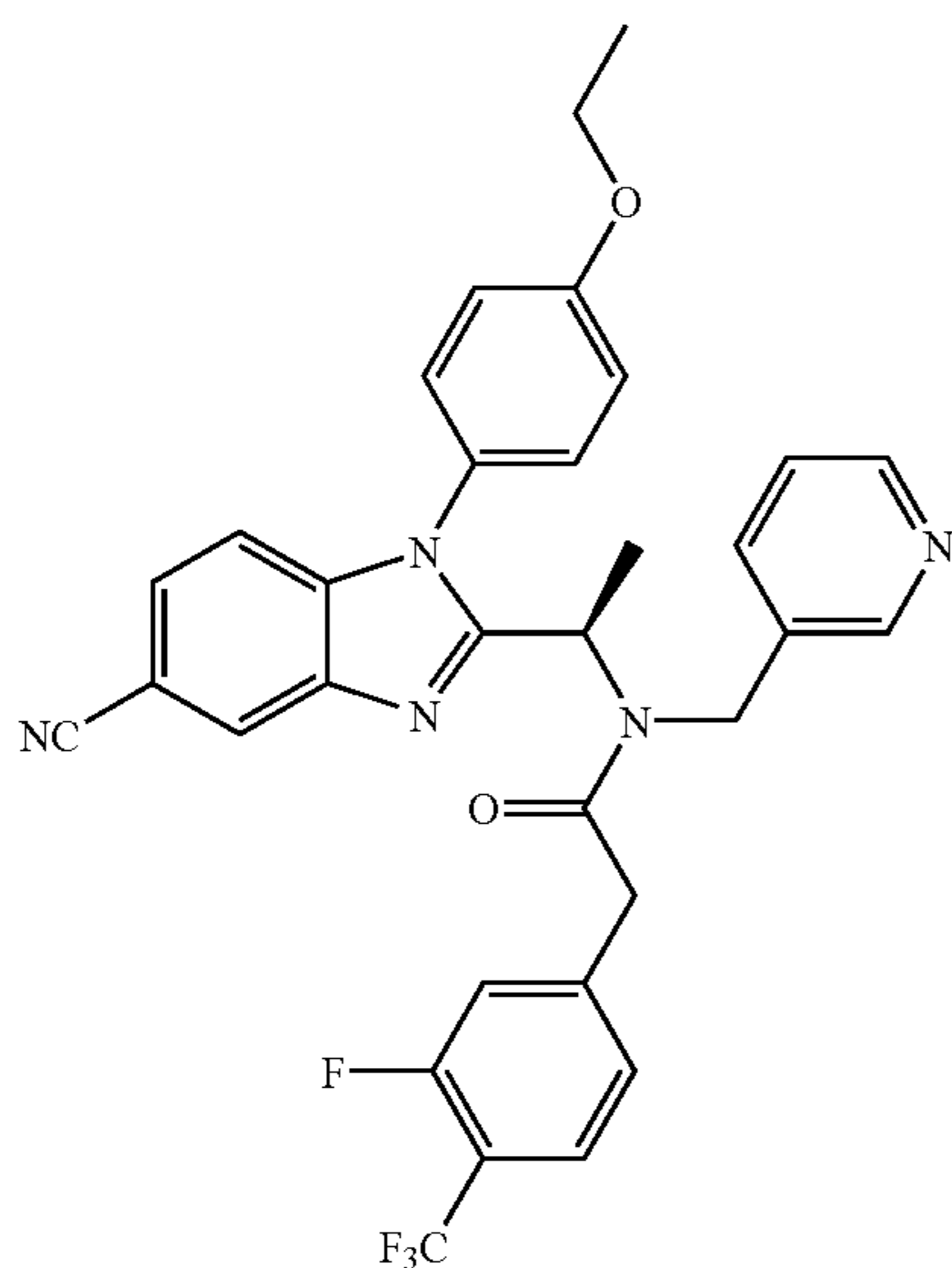
N-{1-[5-Cyano-1-(4-ethoxy-phenyl)-1H-benzimidazol-2-yl]-ethyl}-2-(3-fluoro-4-trifluoromethyl-phenyl)-N-pyridin-3-ylmethyl-acetamide
