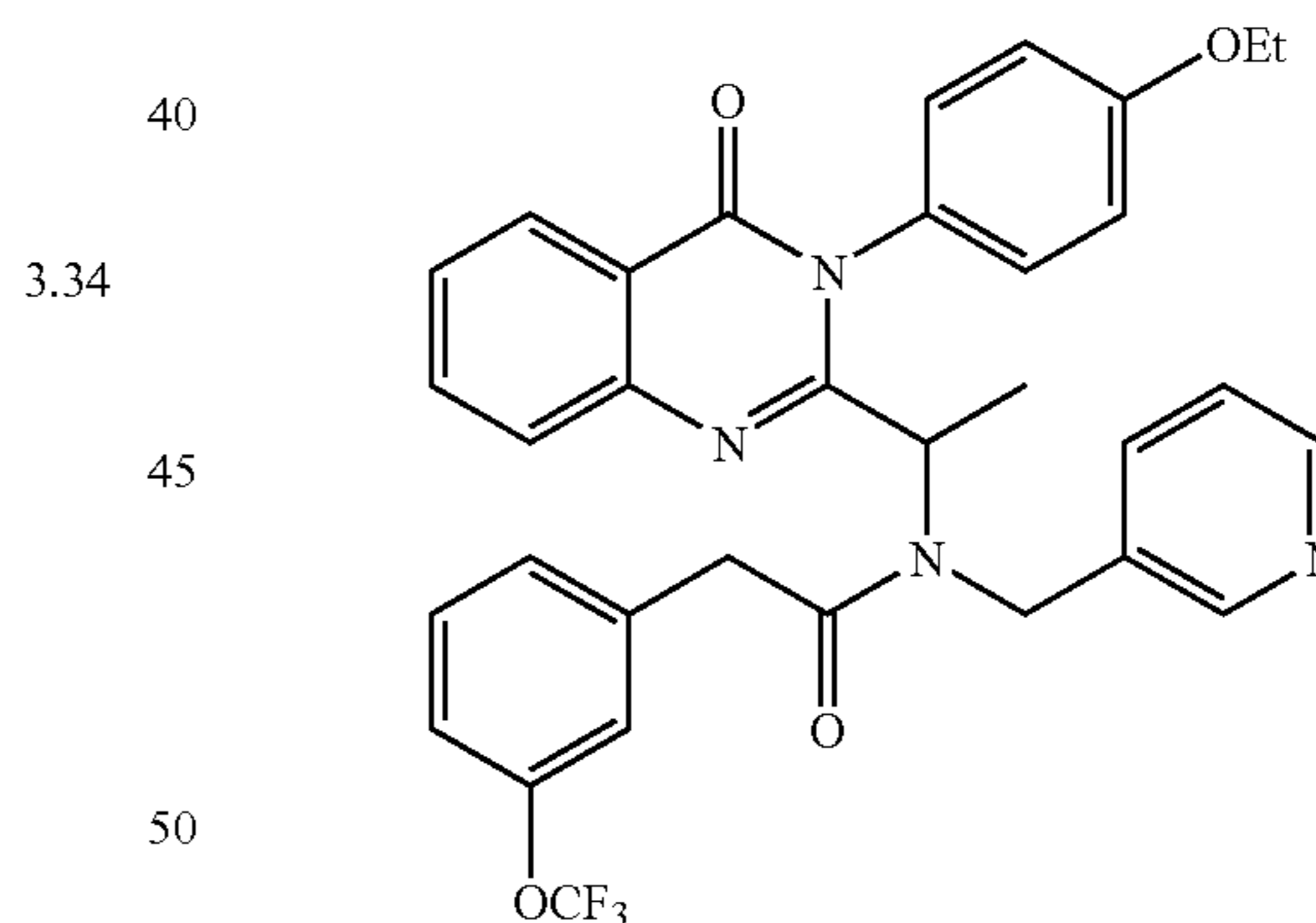
N-{1-[3-(4-Ethoxy-phenyl)-4-oxo-3,4-dihydro-quinazolin-2-yl]-ethyl}-N-pyridin-3-ylmethyl-2-(3-trifluoromethoxy-phenyl)-acetamide
