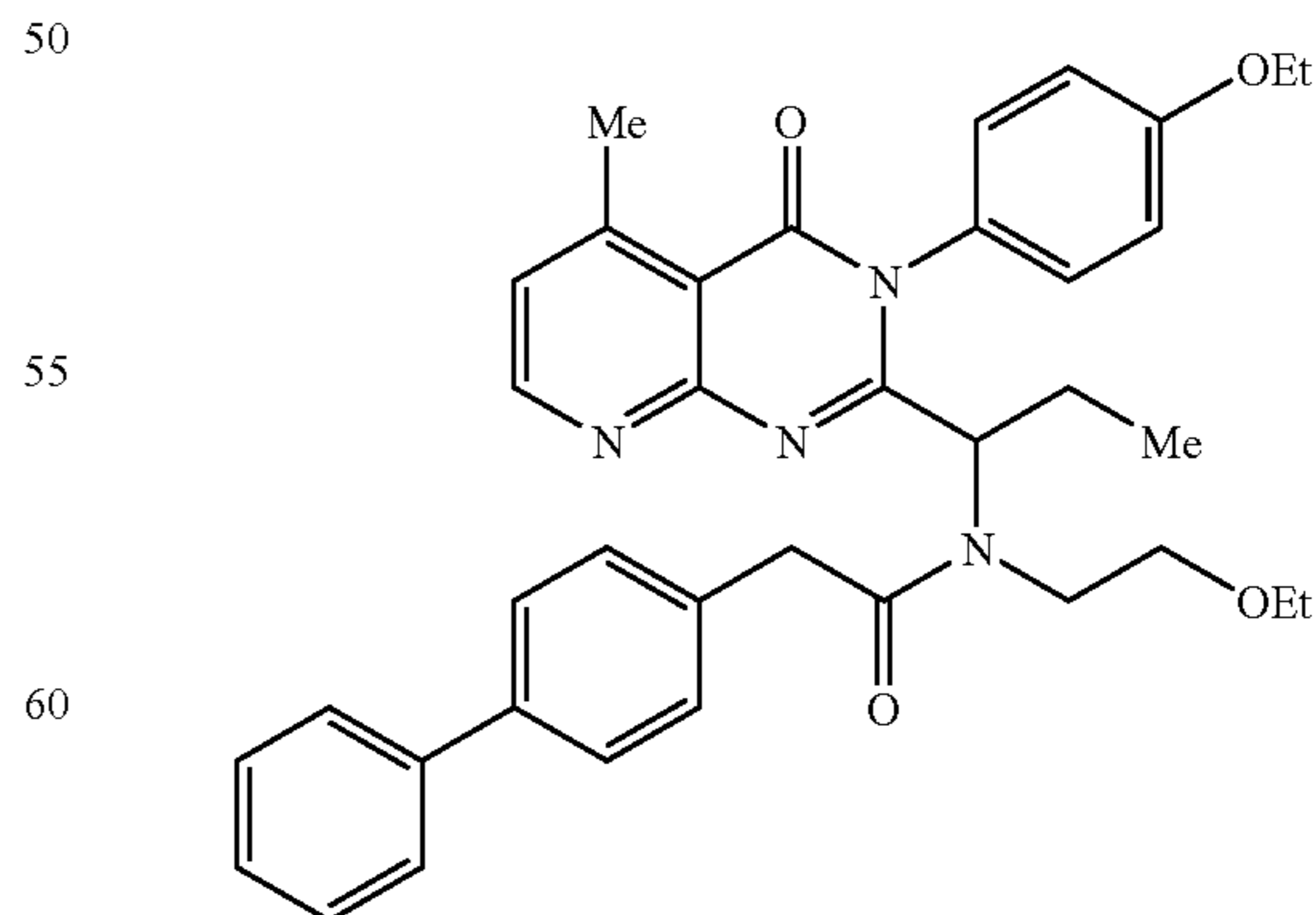
2-Biphenyl-4-yl-N-(2-ethoxy-ethyl)-N-(1-[3-(4-ethoxy-phenyl)-5-methyl-4-oxo-3,4-dihydro-quinazolin-2-yl]-propyl)-acetamide
