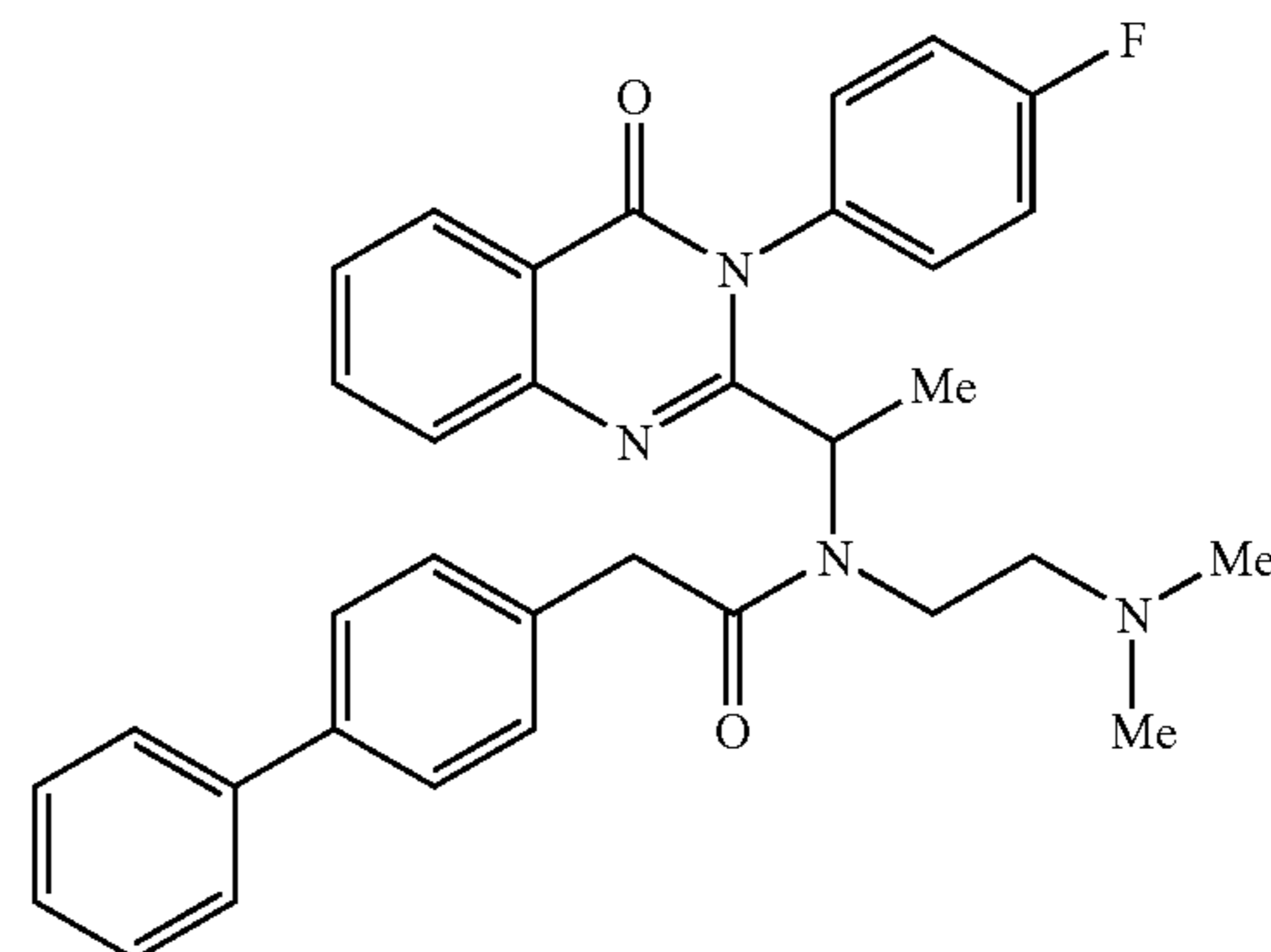
2-Biphenyl-4-yl-N-(2-dimethylamino-ethyl)-N-{1-[3-(4-fluoro-phenyl)-4-oxo-3,4-dihydro-quinazolin-2-yl]-ethyl}-acetamide (1.05)
