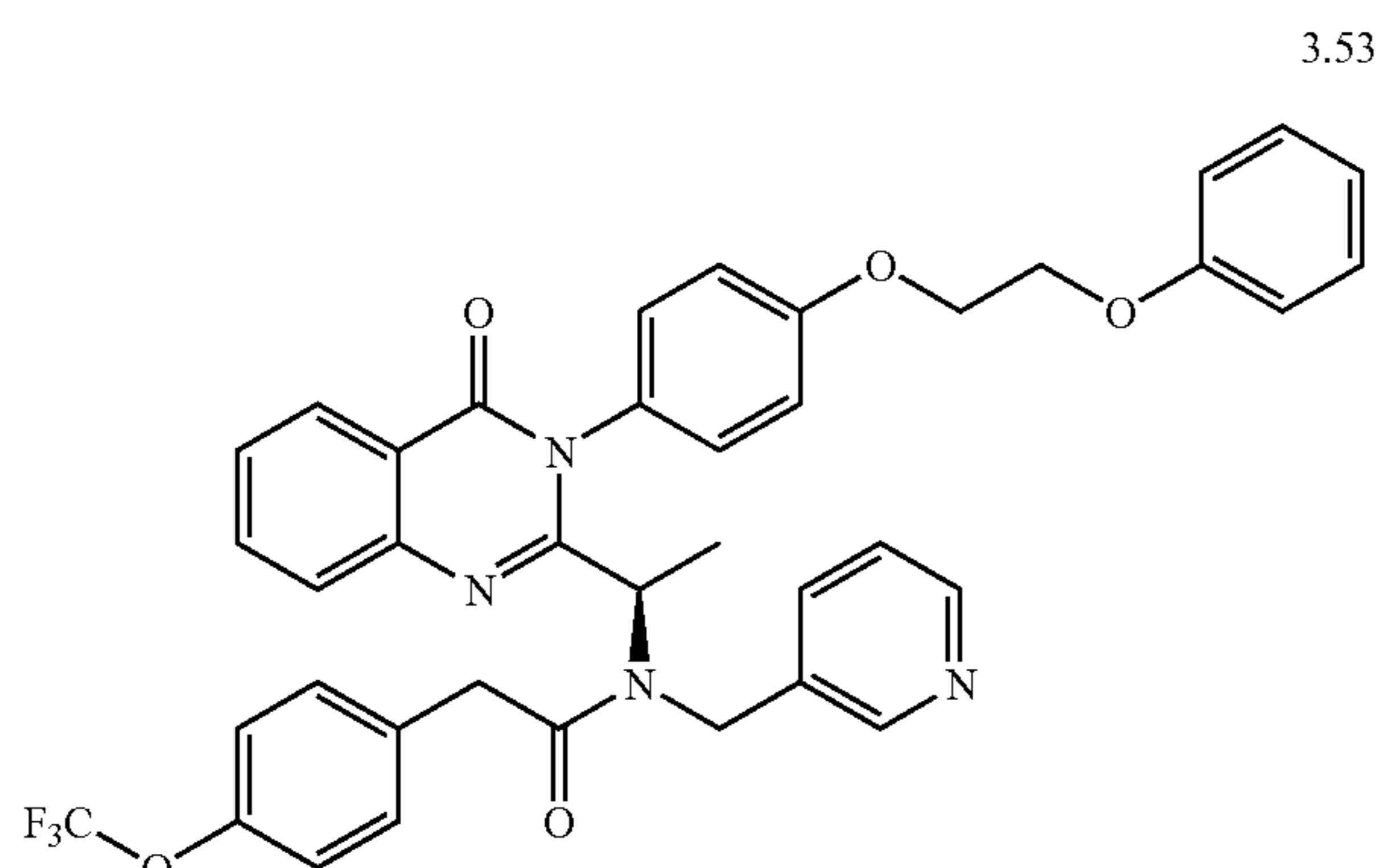
N-(1-(4-Oxo-3-[4-(2-phenoxy-ethoxy)-phenyl]-3,4-dihydro-quinazolin-2-yl)-ethyl)-N-pyridin-3-ylmethyl-2-(4-trifluoromethoxy-phenyl)-acetamide
