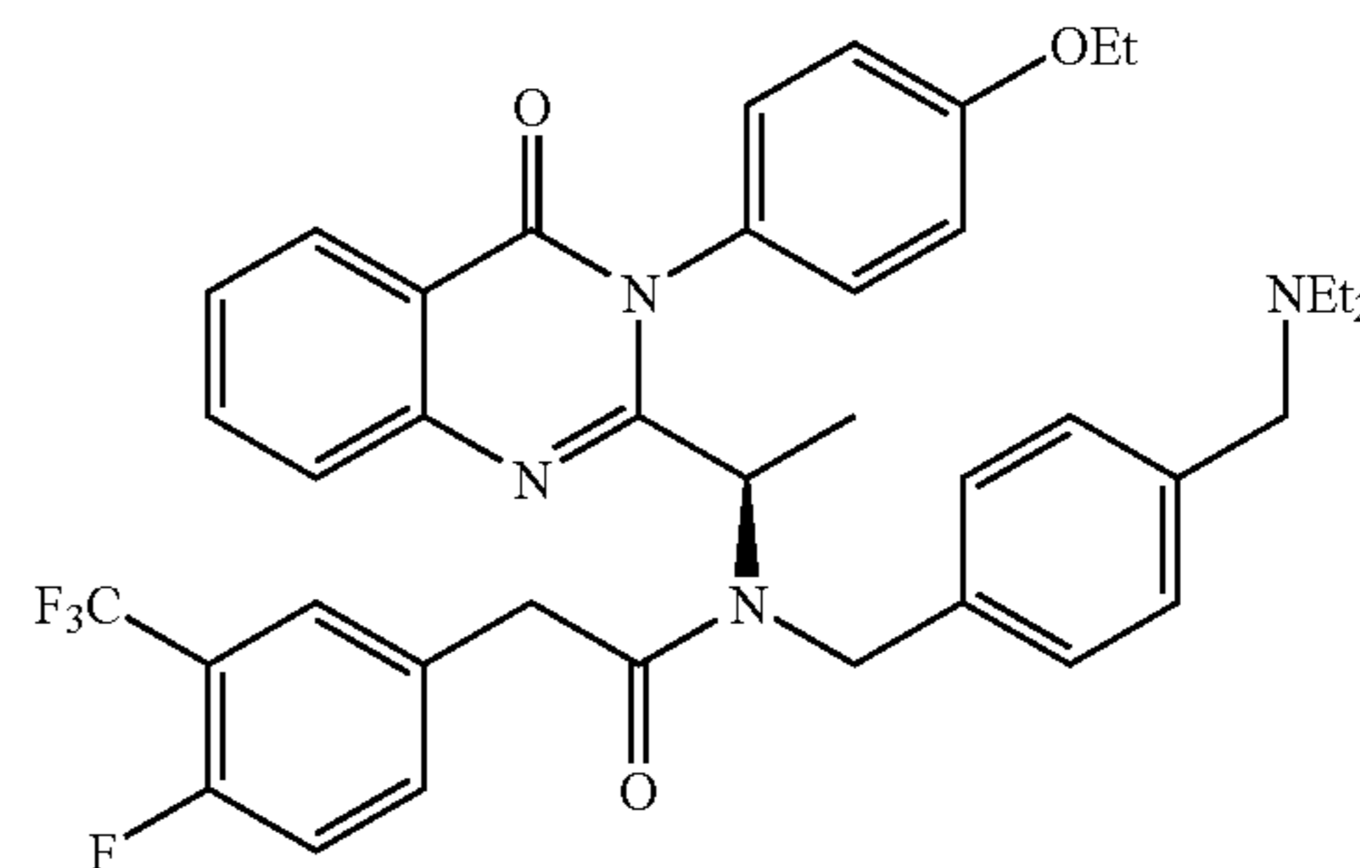
N-(4-Diethylaminomethyl-benzyl)-N-{1-[3-(4-ethoxy-phenyl)-4-oxo-3,4-dihydroquinazolin-2-yl]-ethyl}-2-(4-fluoro-3-trifluoromethyl-phenyl)-acetamide
