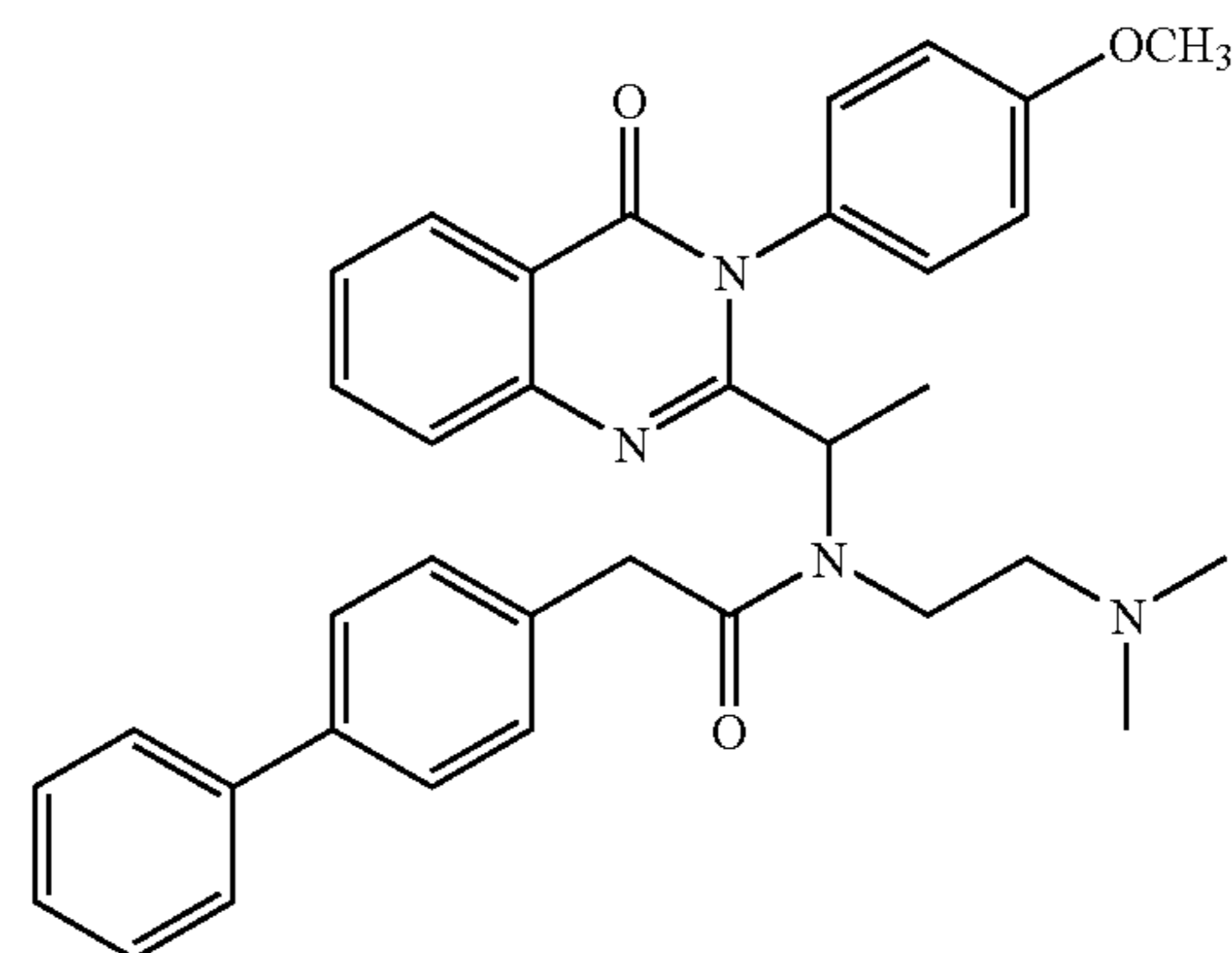
2-Biphenyl-4-yl-N-(2-dimethylamino-ethyl)-N-{1-[3-(4-methoxy-phenyl)-4-oxo-3,4-dihydro-quinazolin-2-yl]-ethyl}-acetamide
