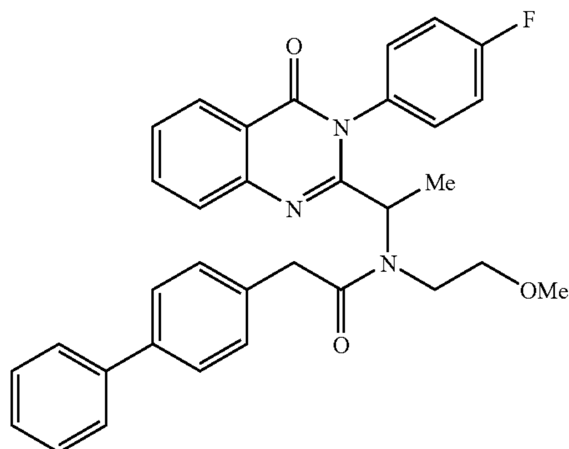
2-Biphenyl-4-yl-N-{1-[3-(4-fluoro-phenyl)-4-oxo-3,4-dihydro-quinazolin-2-yl]-ethyl}-N-(2-methoxy-ethyl)-acetamide (1.17)
