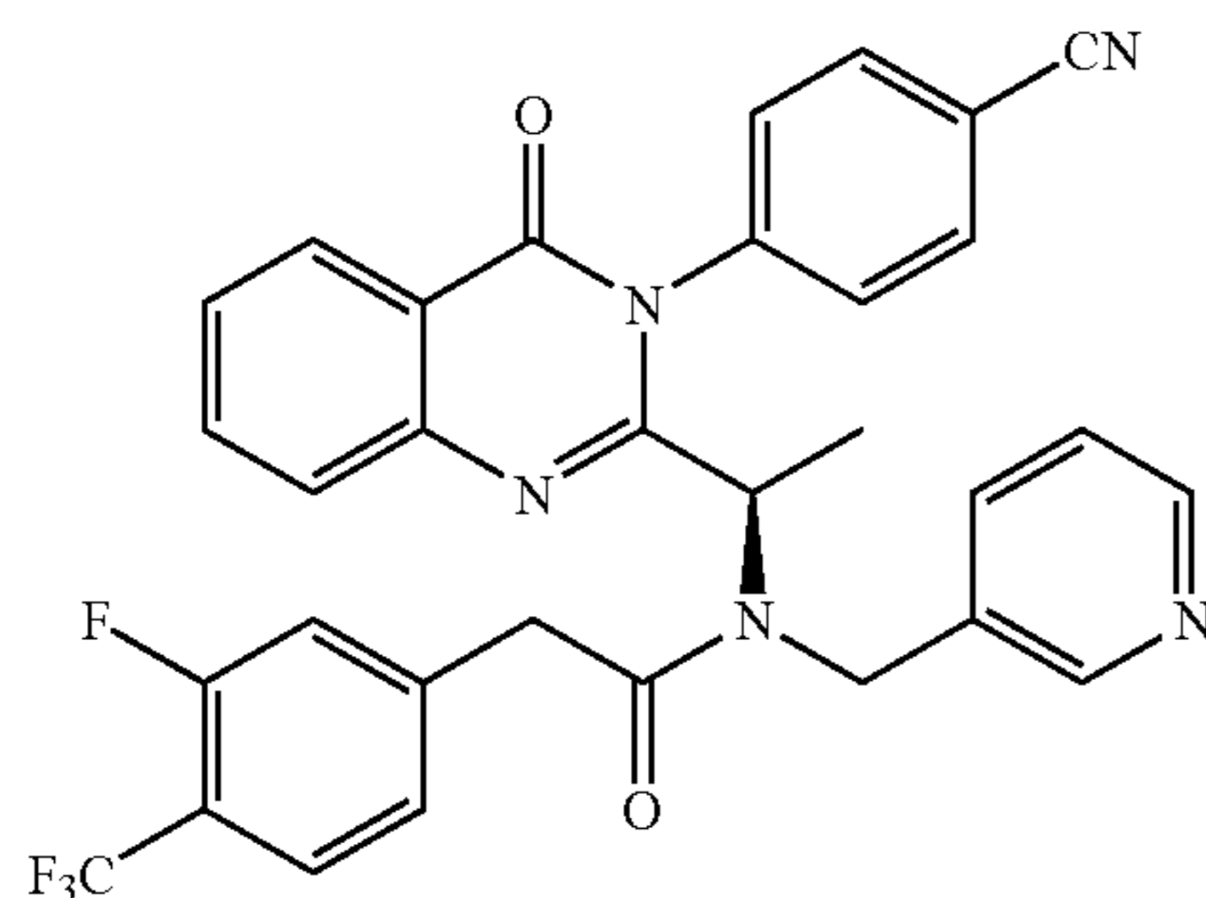
N-{1-[3-(4-Cyano-phenyl)-4-oxo-3,4-dihydro-quinazolin-2-yl]-ethyl}-2-(3-fluoro-4-trifluoromethyl-phenyl)-N-pyridin-3-ylmethyl-acetamide
