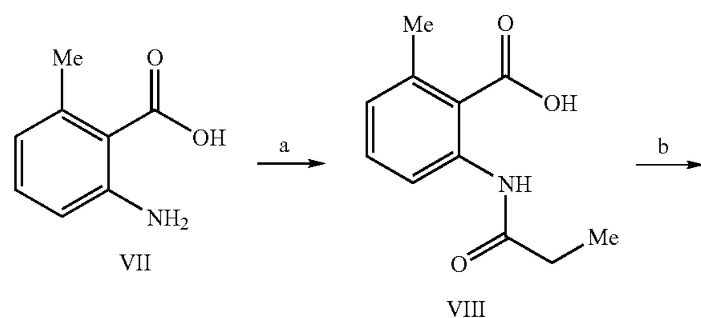
Scheme 2
