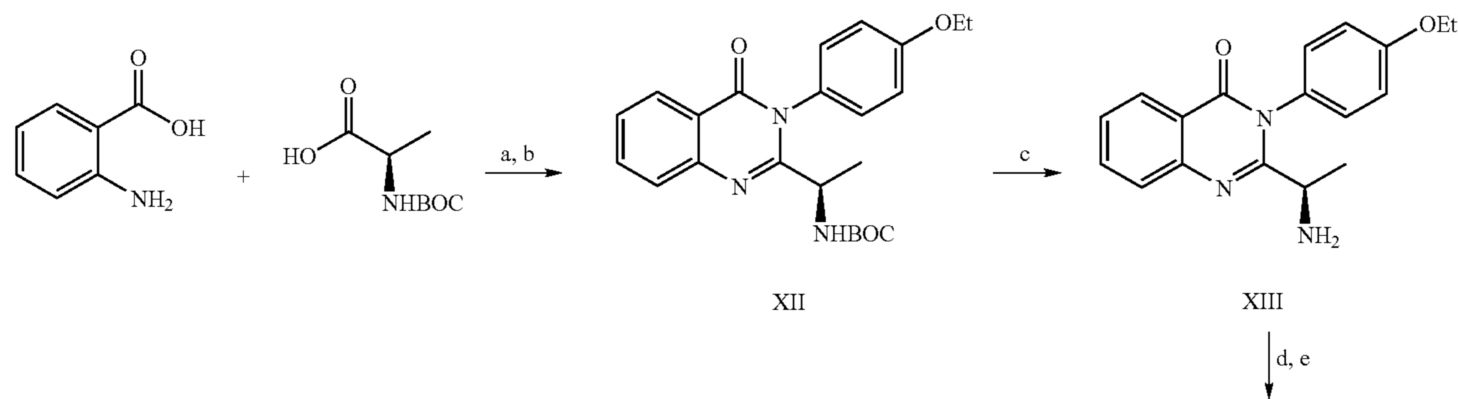
Scheme 3
