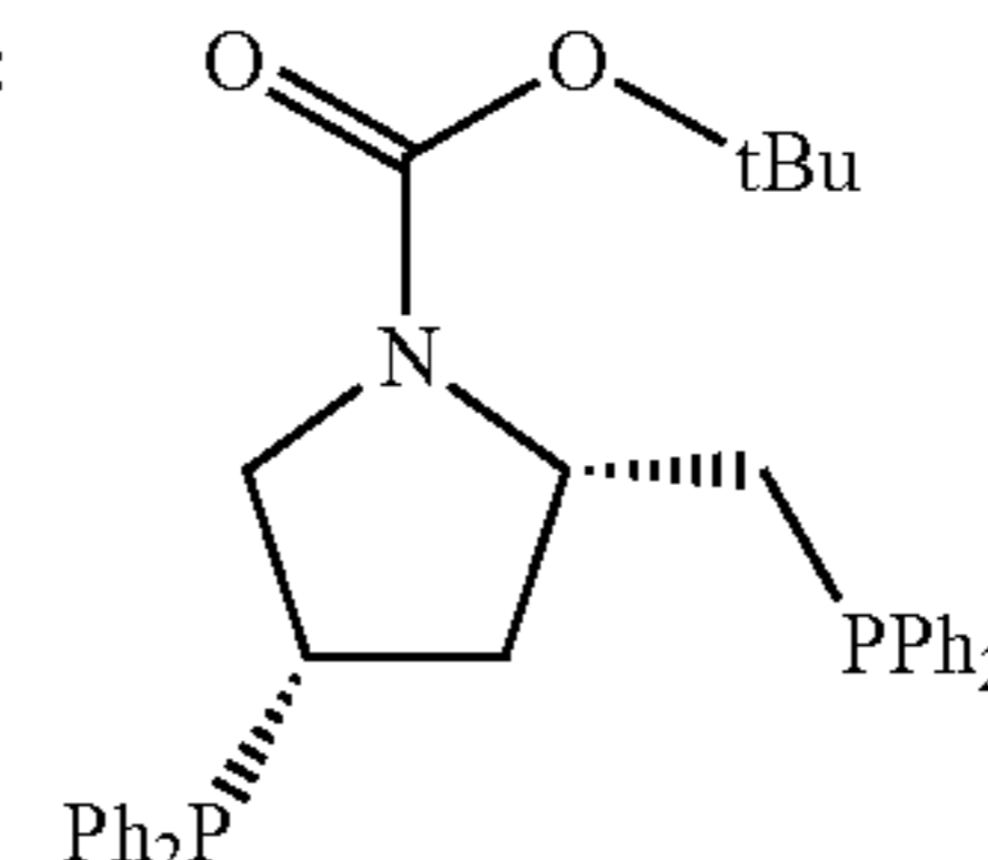
(S,S)-BPPM:
