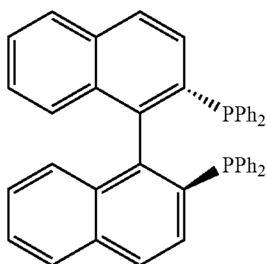
(S)-BINAP:
