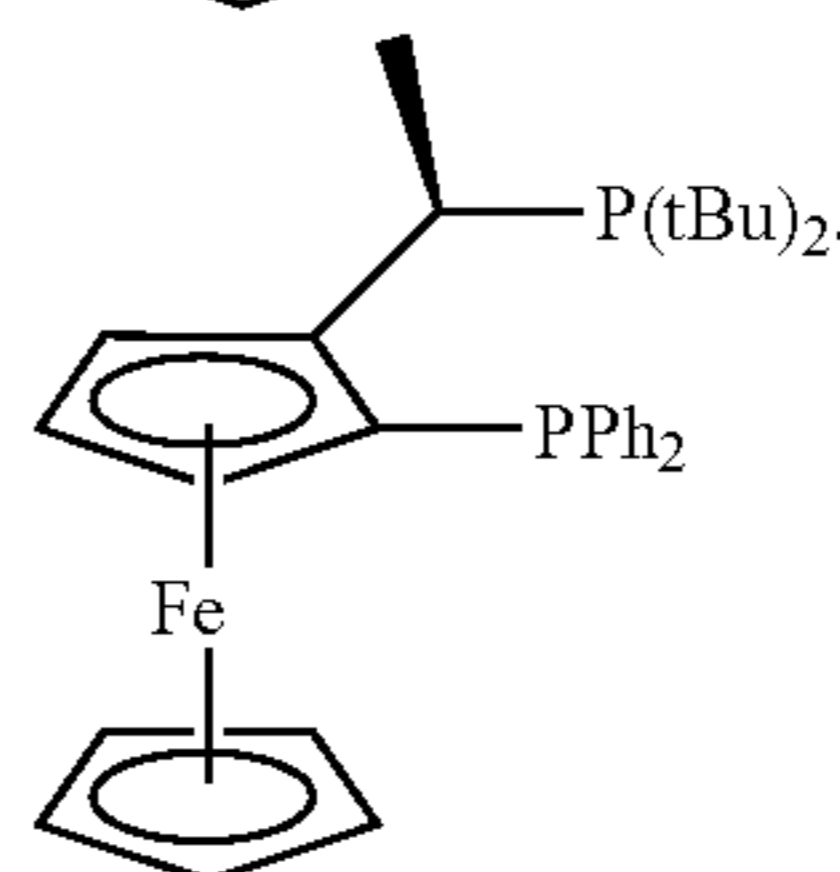
(S,R)-PFctBu:
