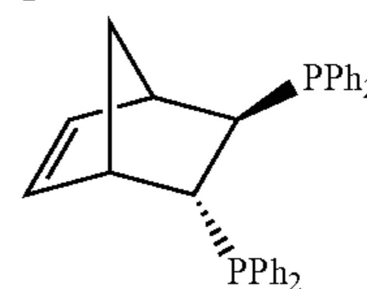
(R,R)-Norphos:
