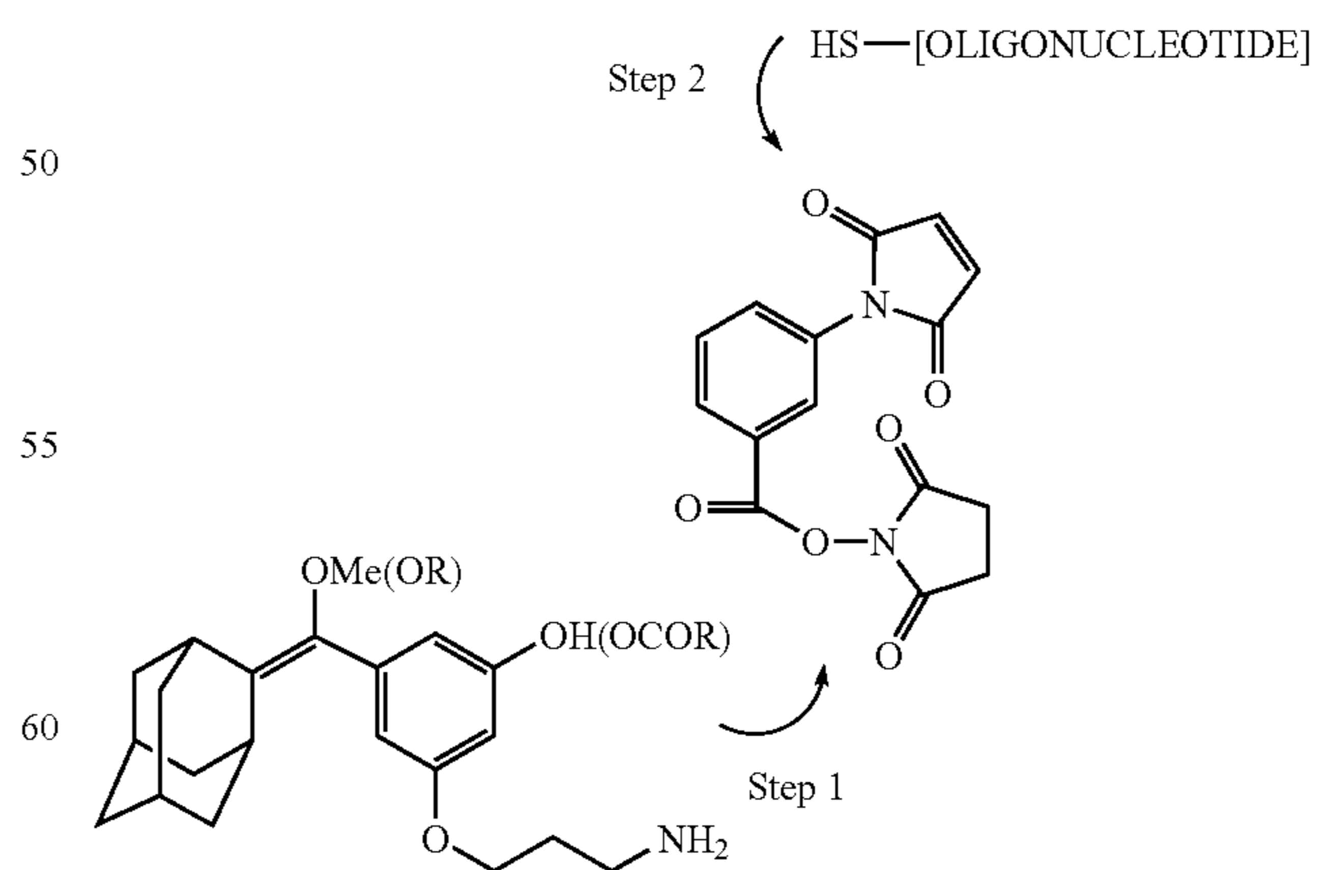
Assembly of enol ether-labeled oligonucleotide
