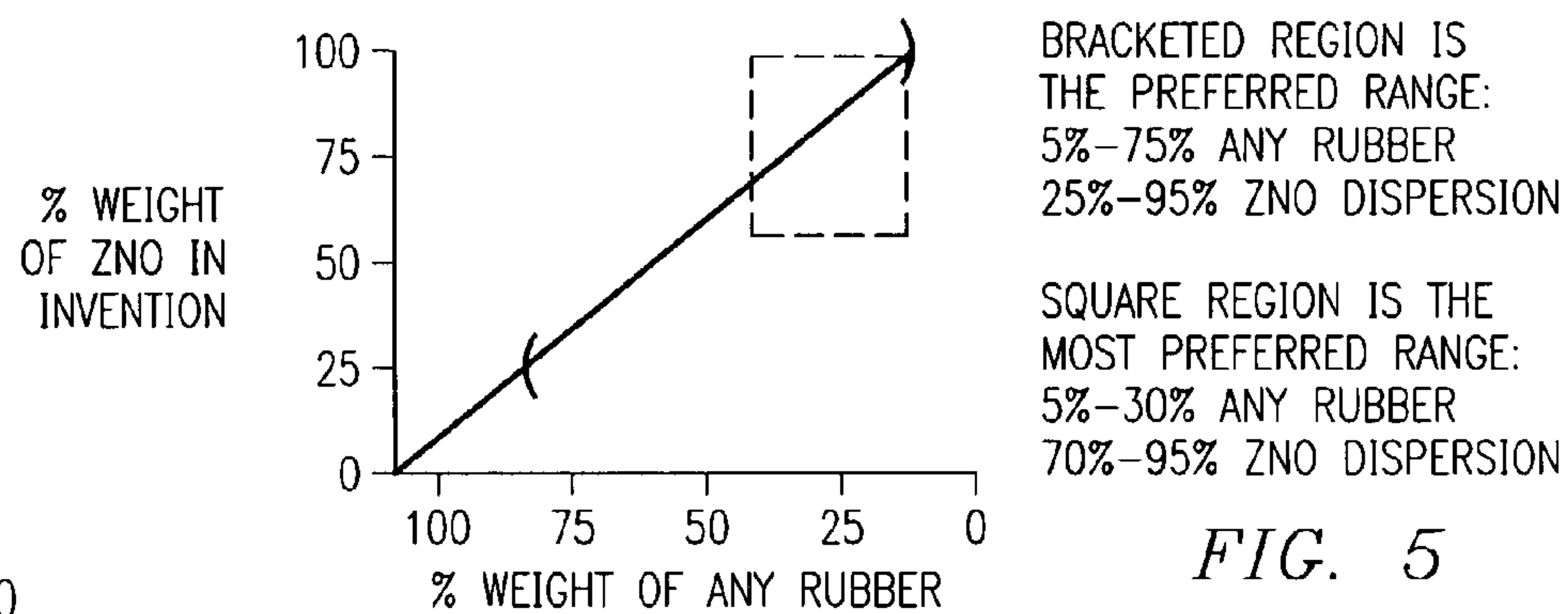
% BY WEIGHT OF ANY RUBBER BASE VERSUS % BY WEIGHT OF ZNO DISPERSION
