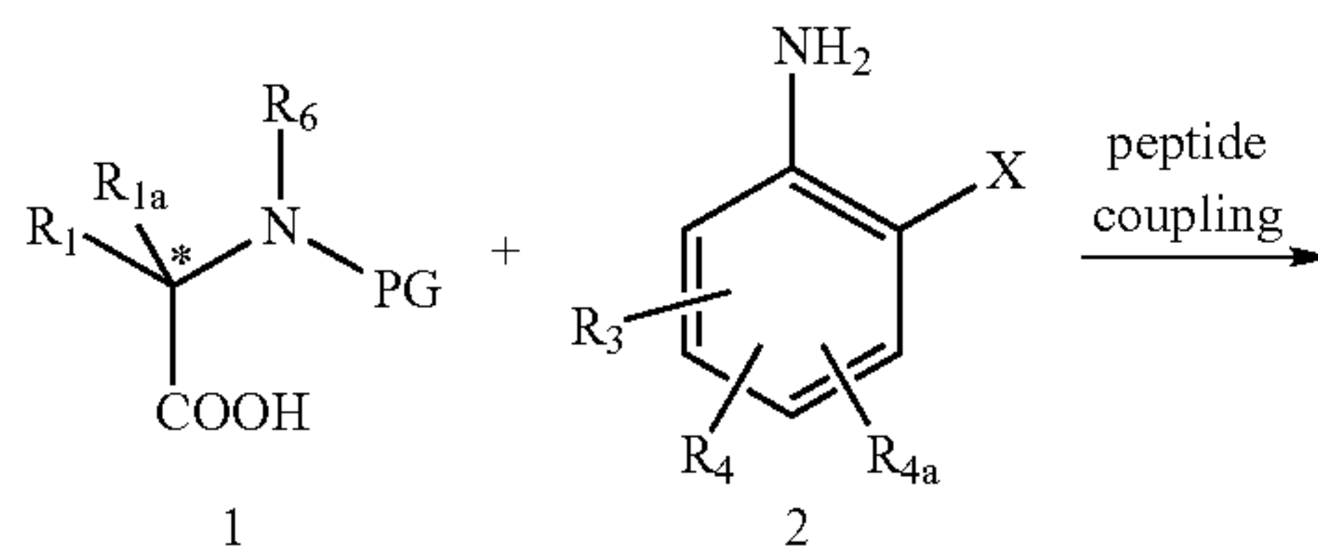
Scheme 1
