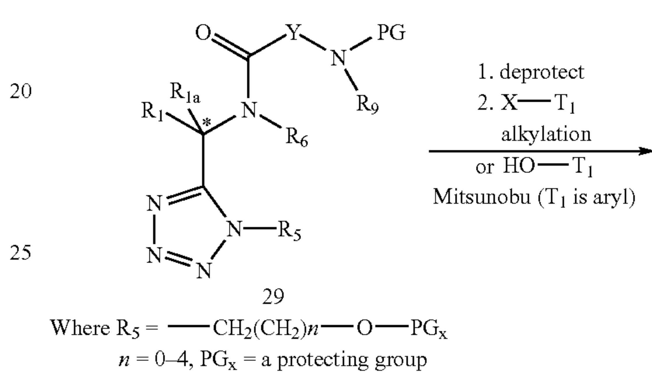
Scheme 3h
