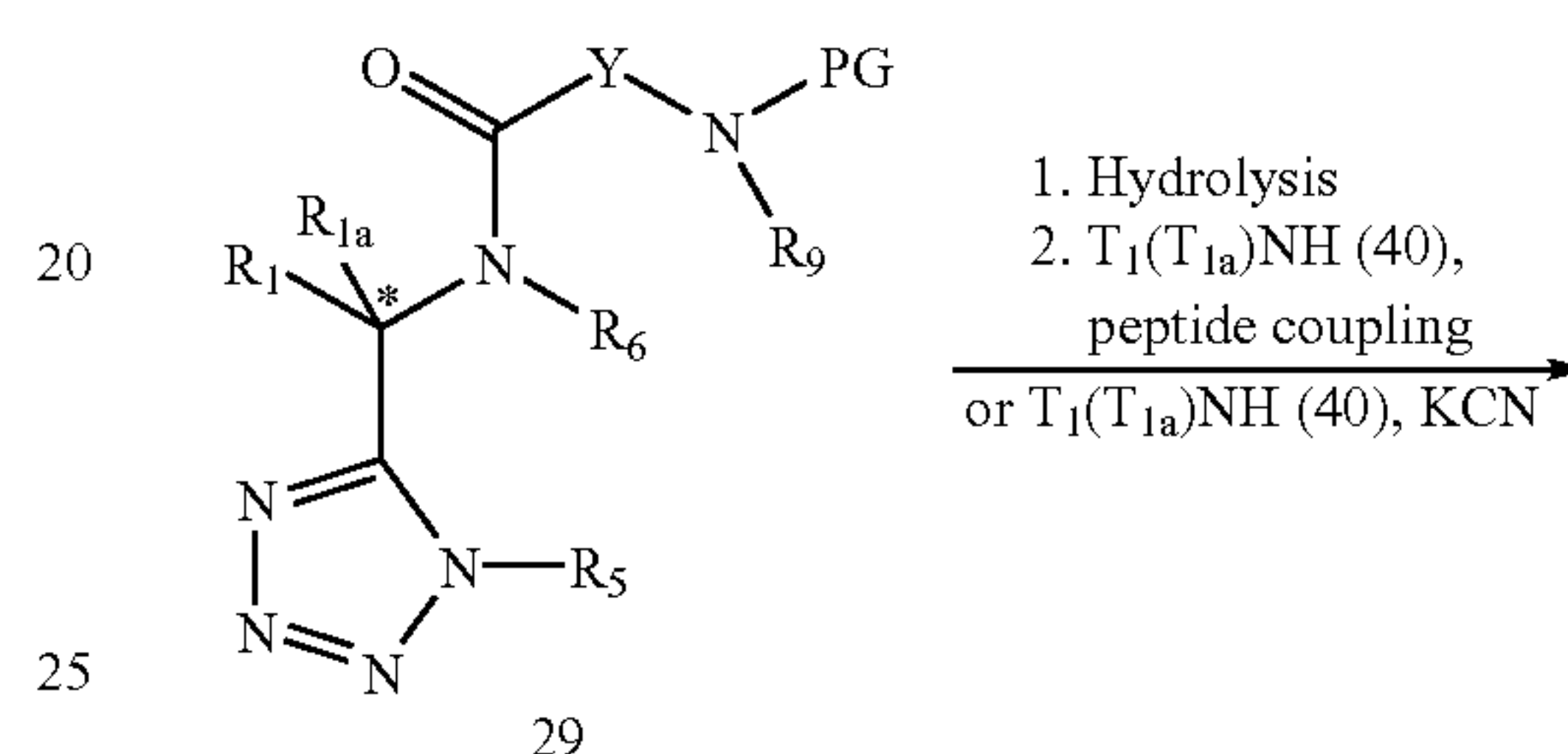
Scheme 3d
