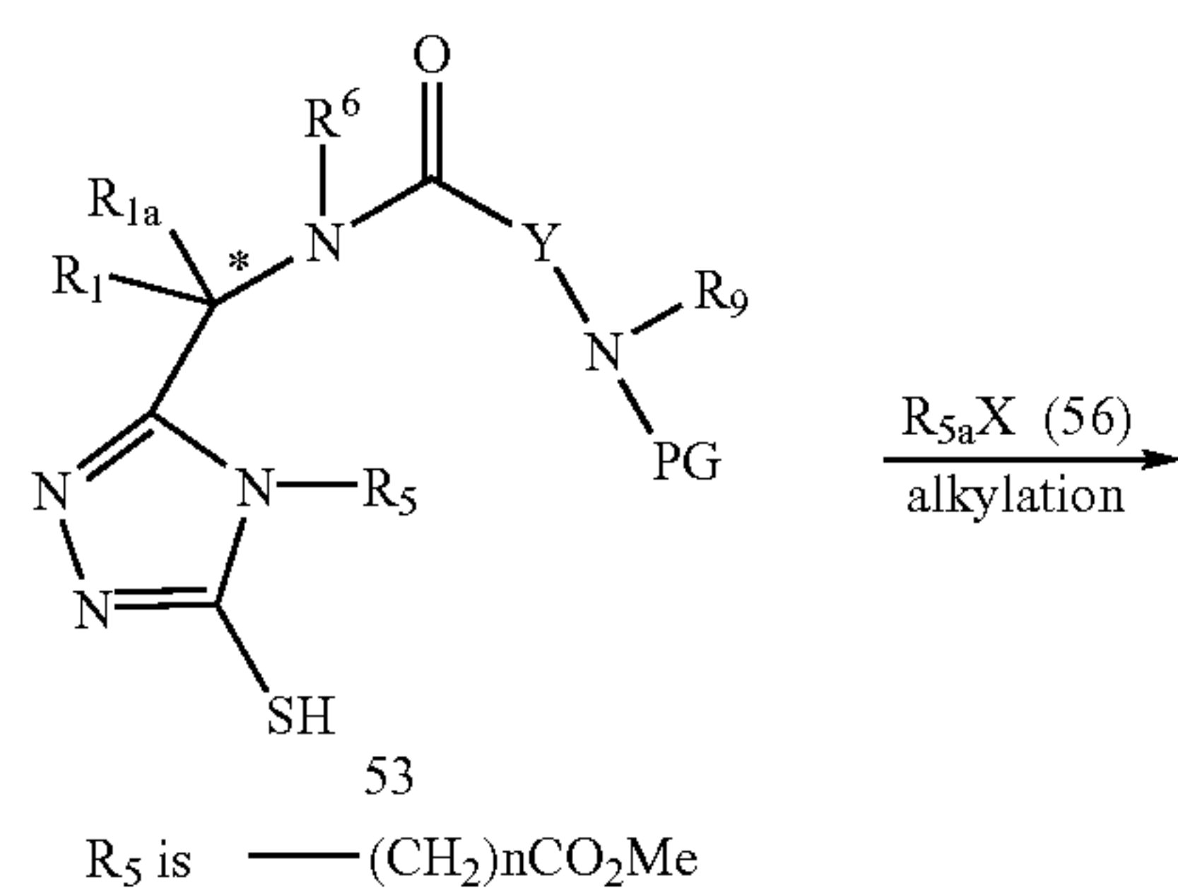
Scheme 4d
