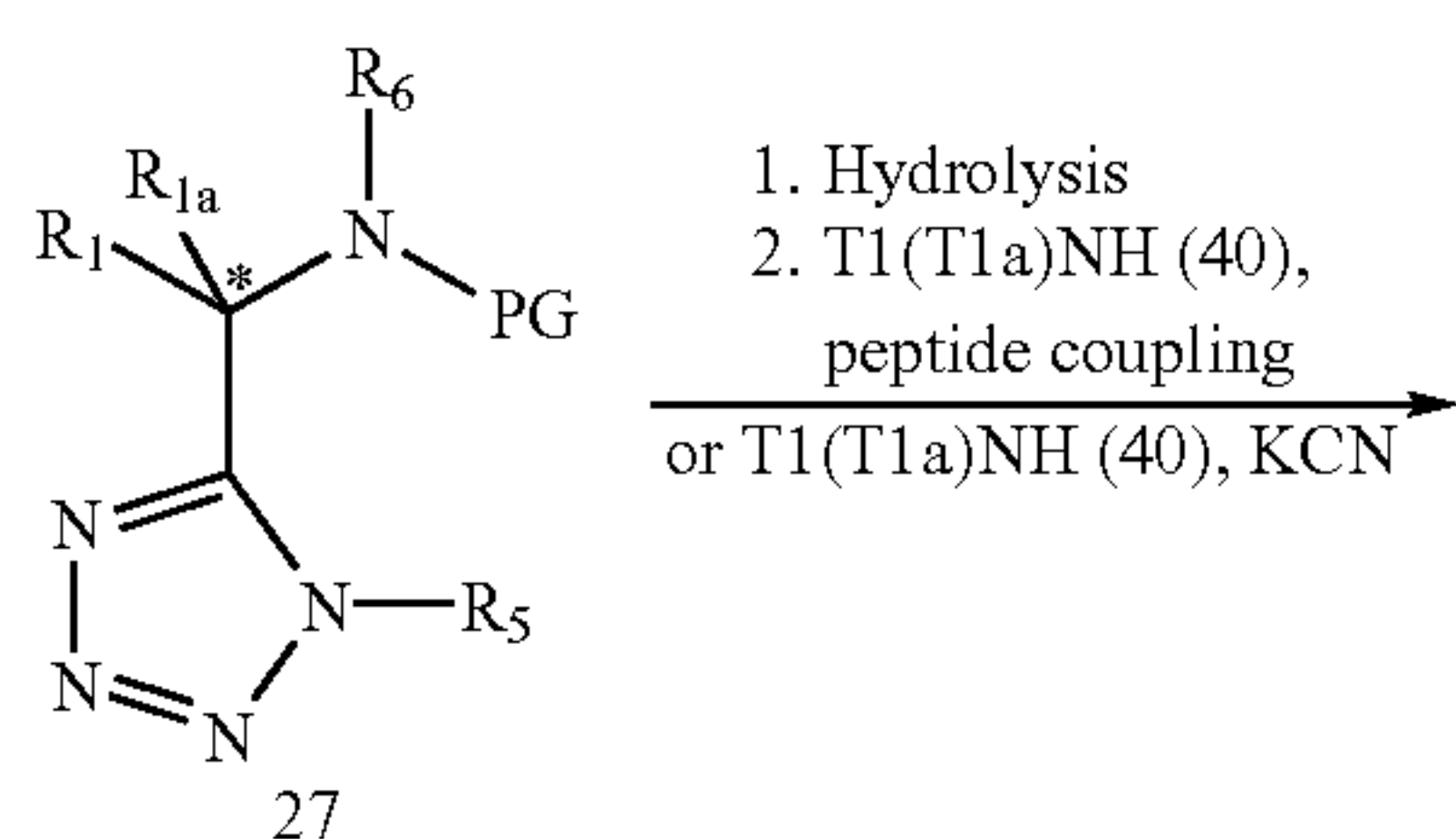
Scheme 3c
