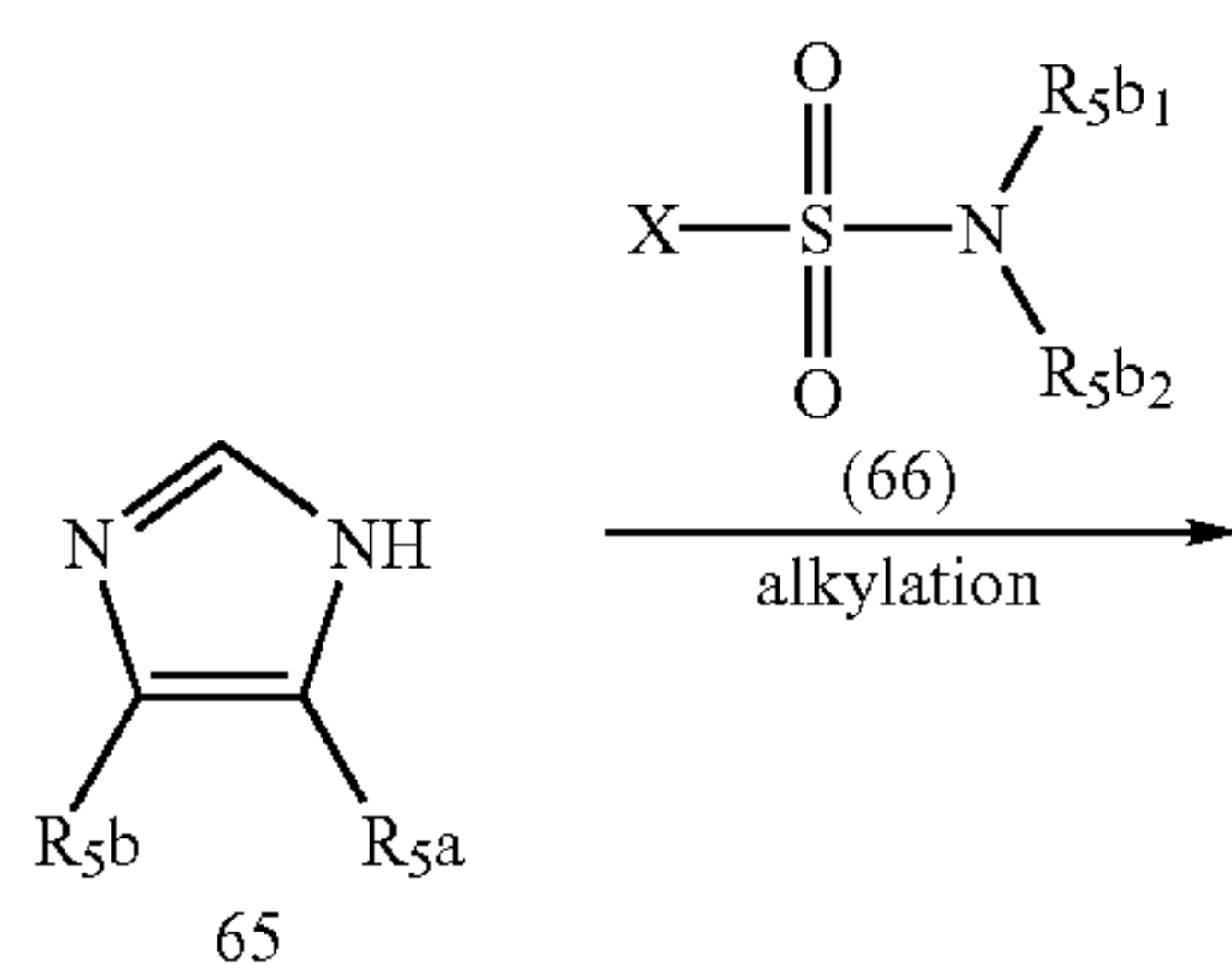
Scheme 5: Imidazoles
