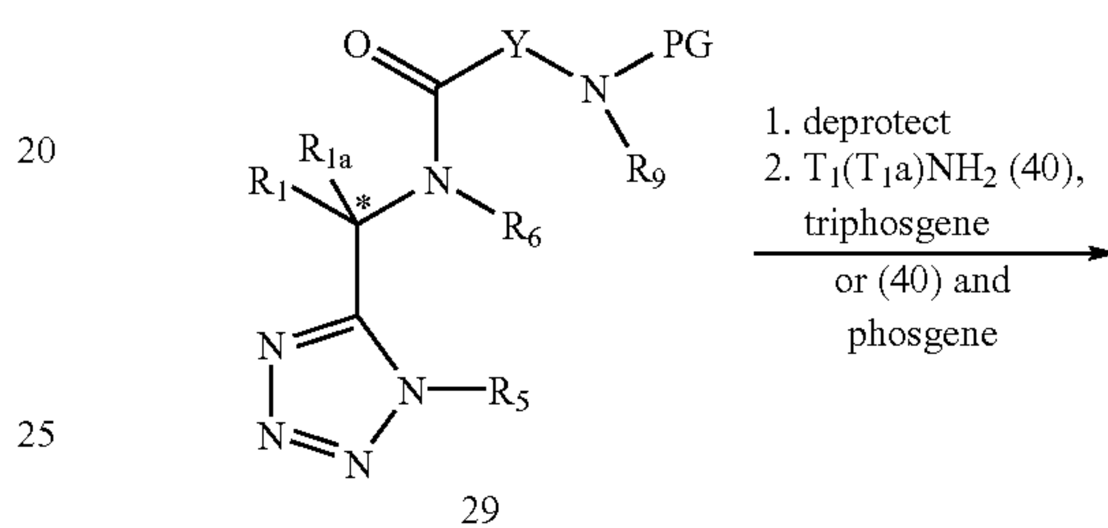
Scheme 3f
