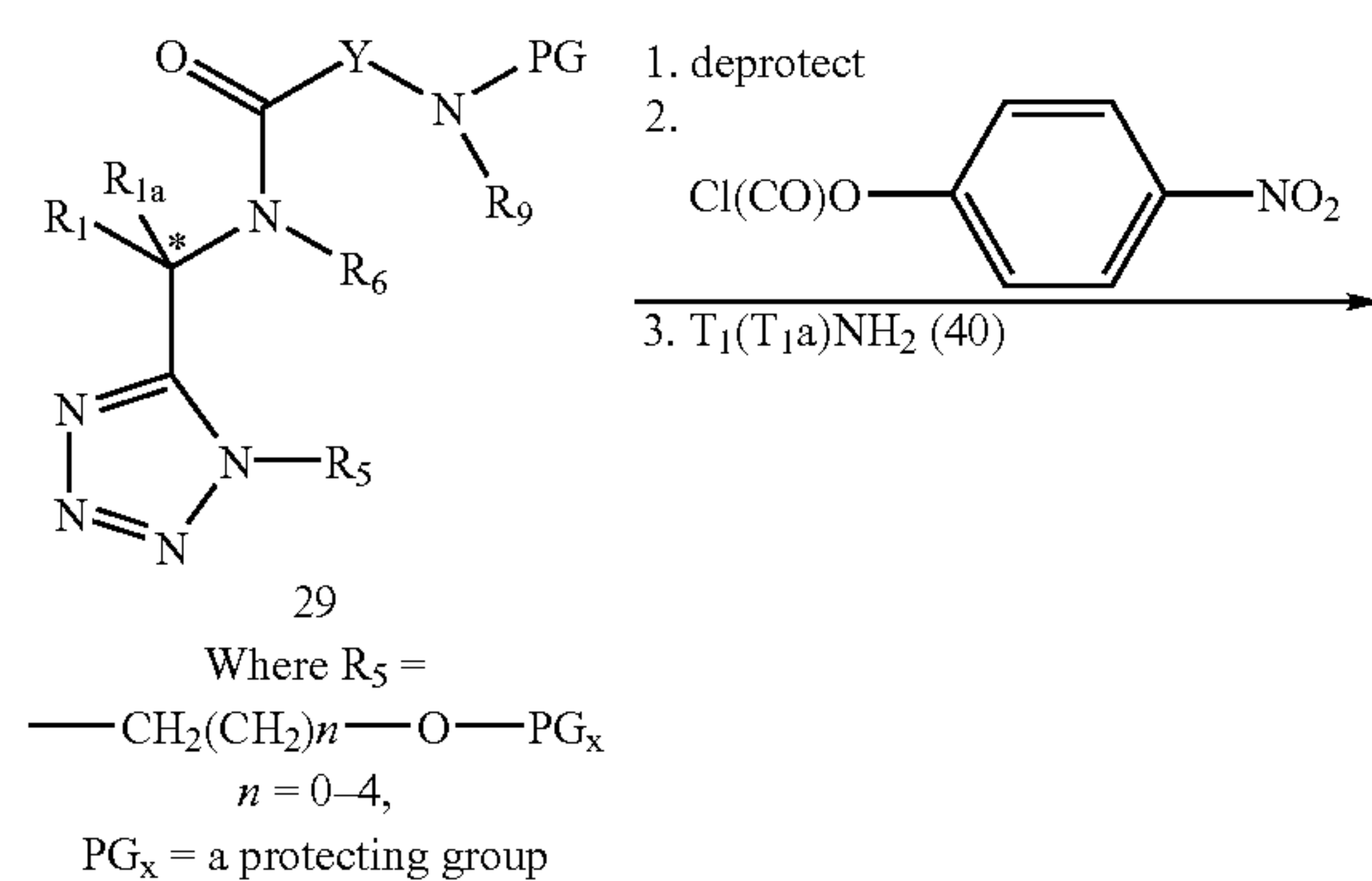
Scheme 3g
