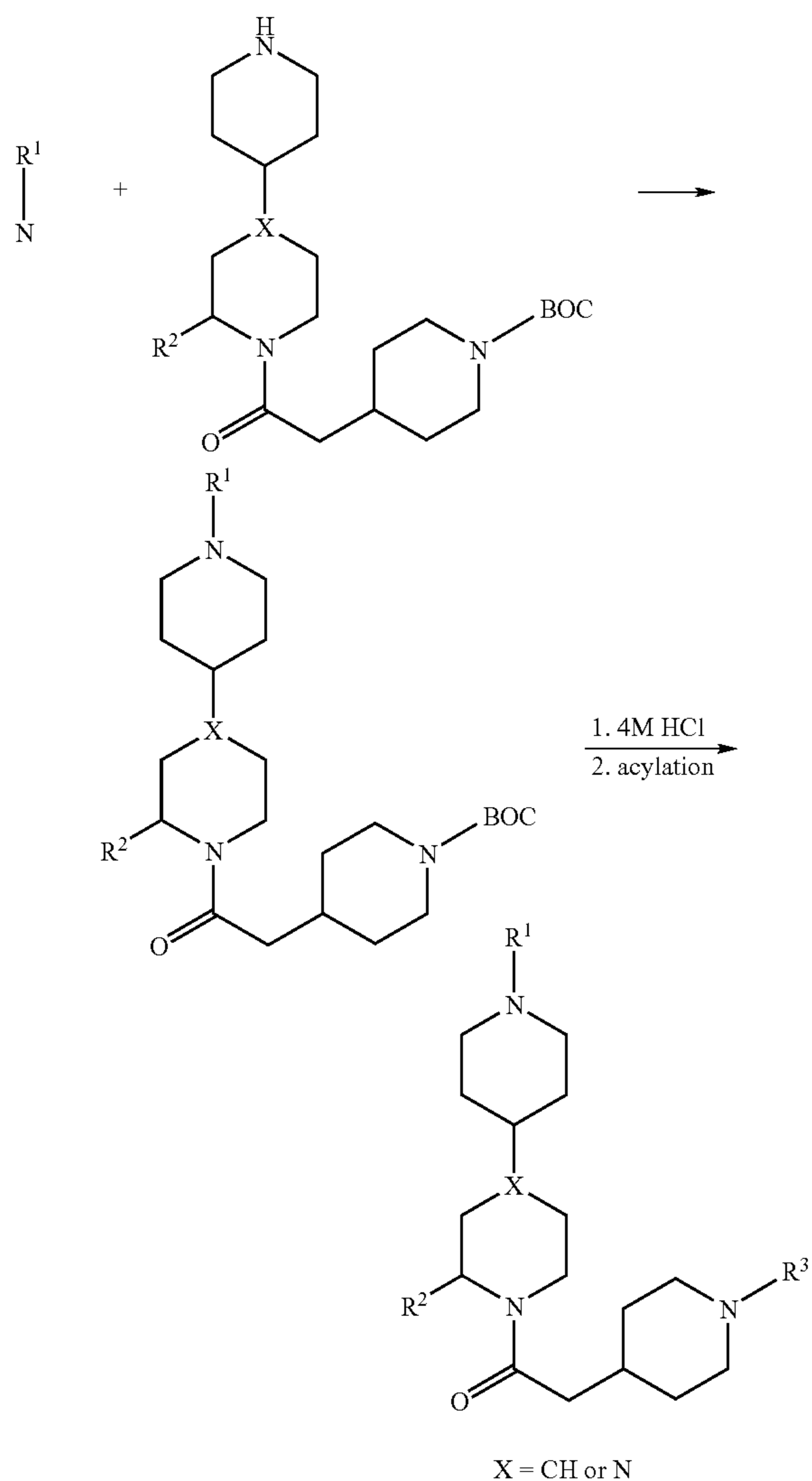
Scheme 3
