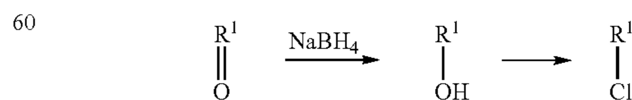
Scheme 5
