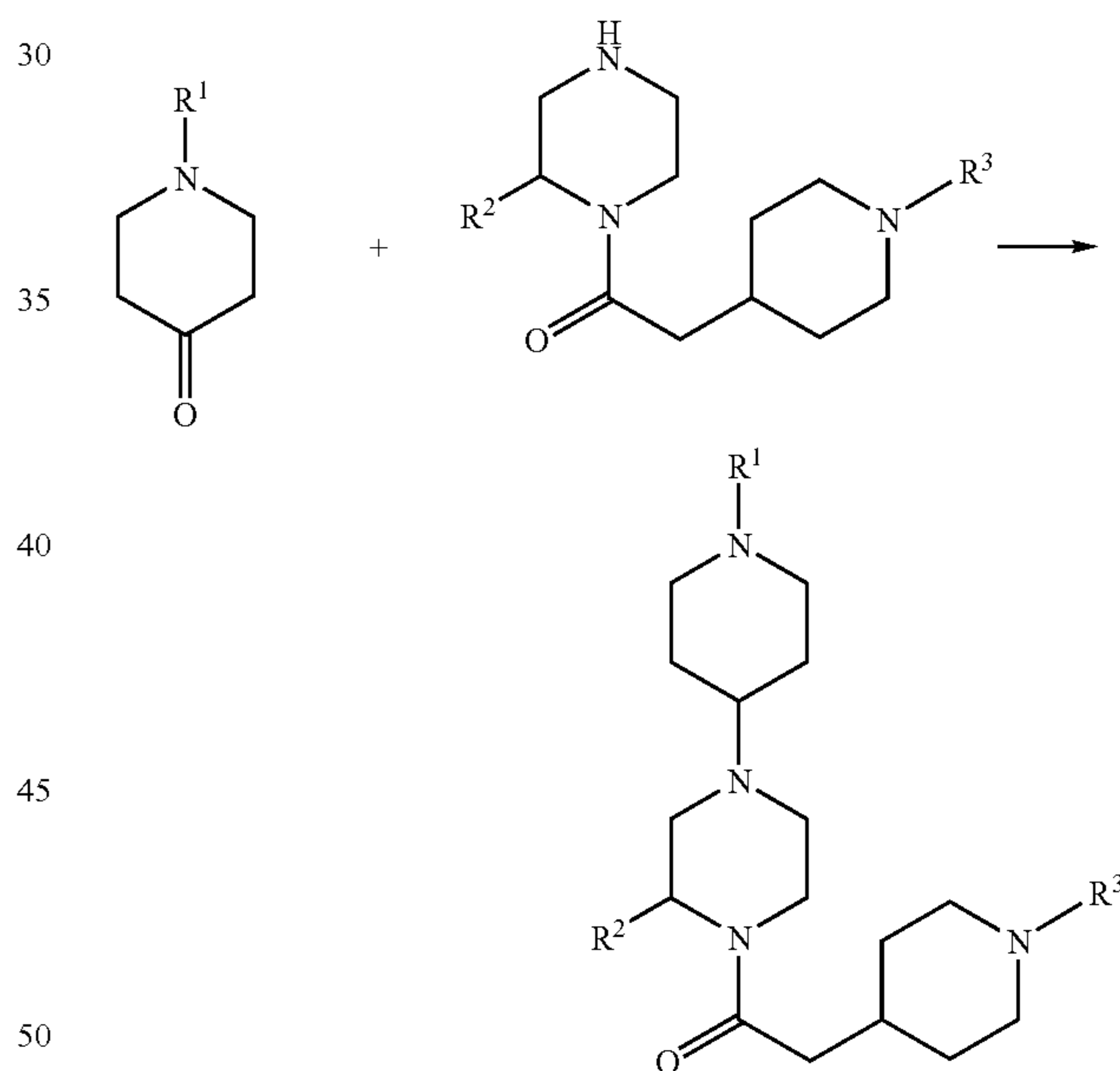
Scheme 4
