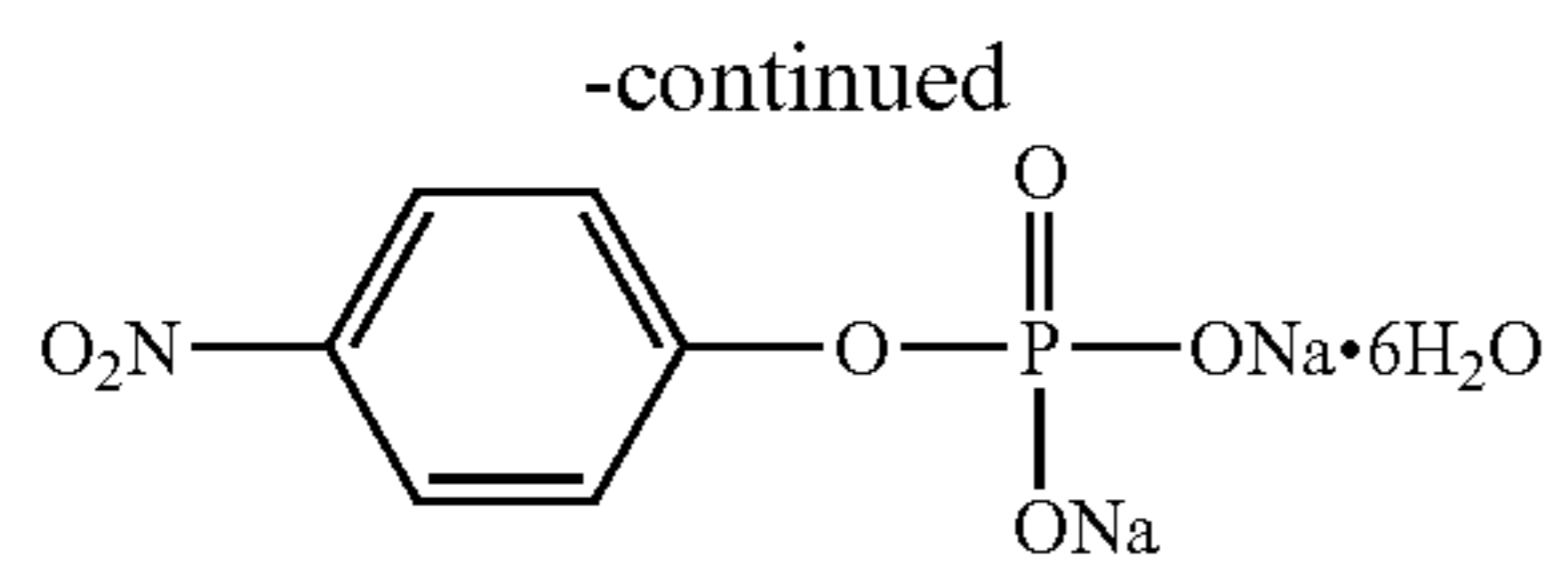
p-nitrophenyl phosphate
