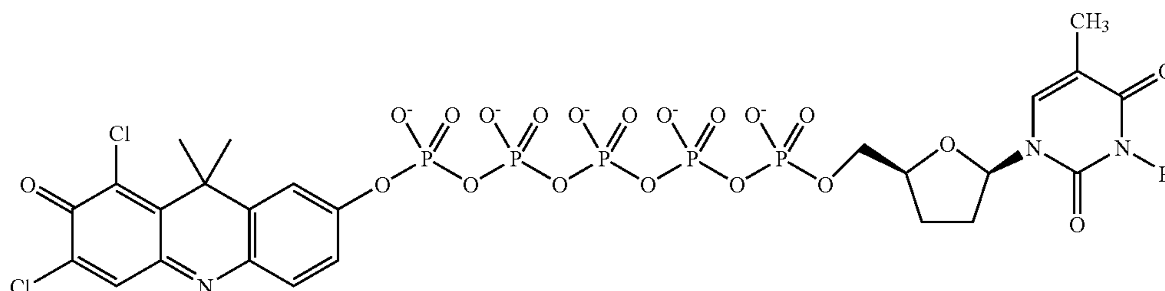
dd-T5P-DDAO
