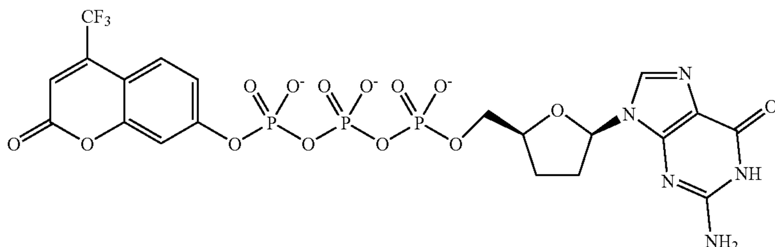
\gamma -(4-trifluoromethylcoumarinyl)dideoxyguanosine-5'-triphosphate ( \gamma CF 3 Coumarin-ddGTP)
