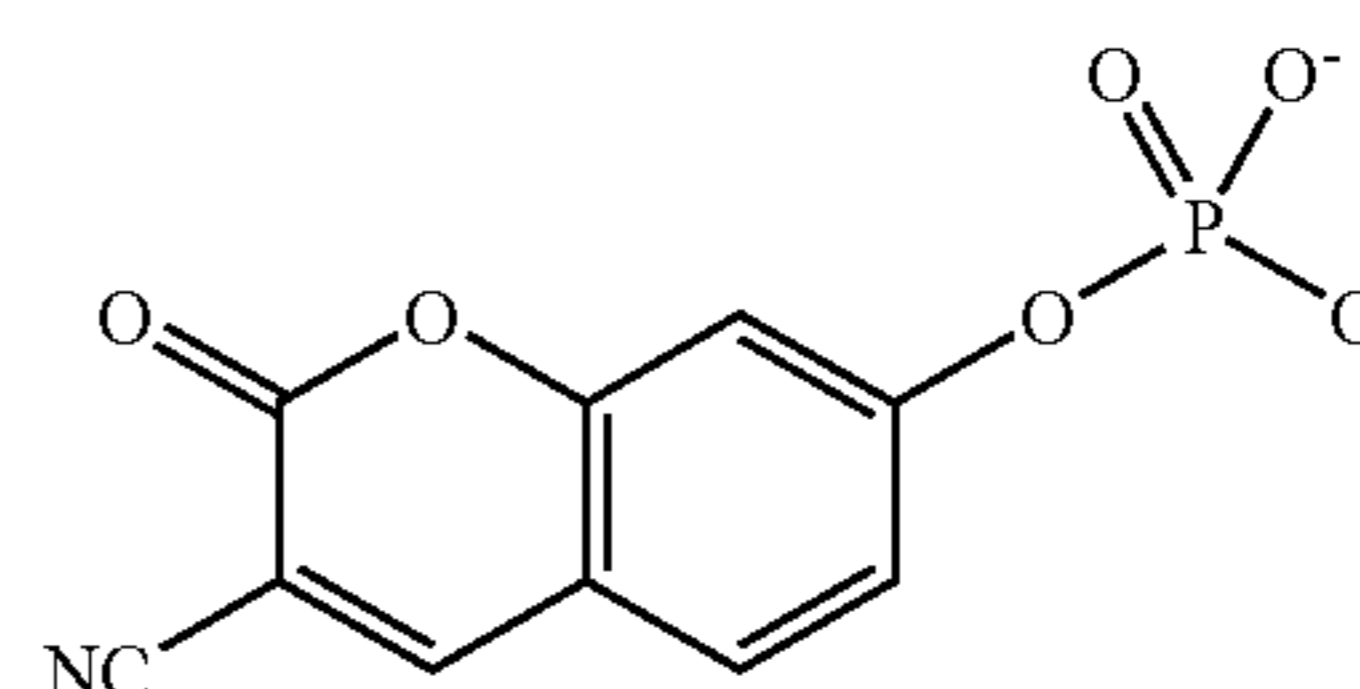
3-Cyanoumbelliferyl phosphate
