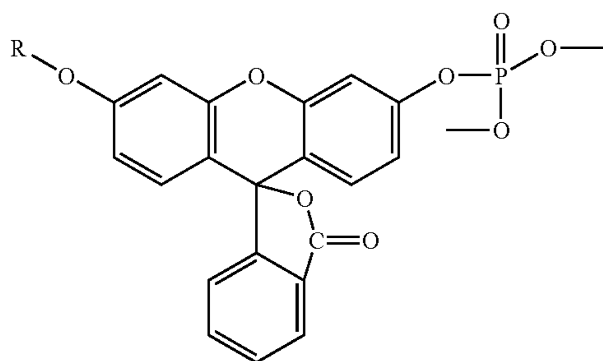
fluorescein 3'-(6')-O-alkyl-6'-(3')-phosphate
