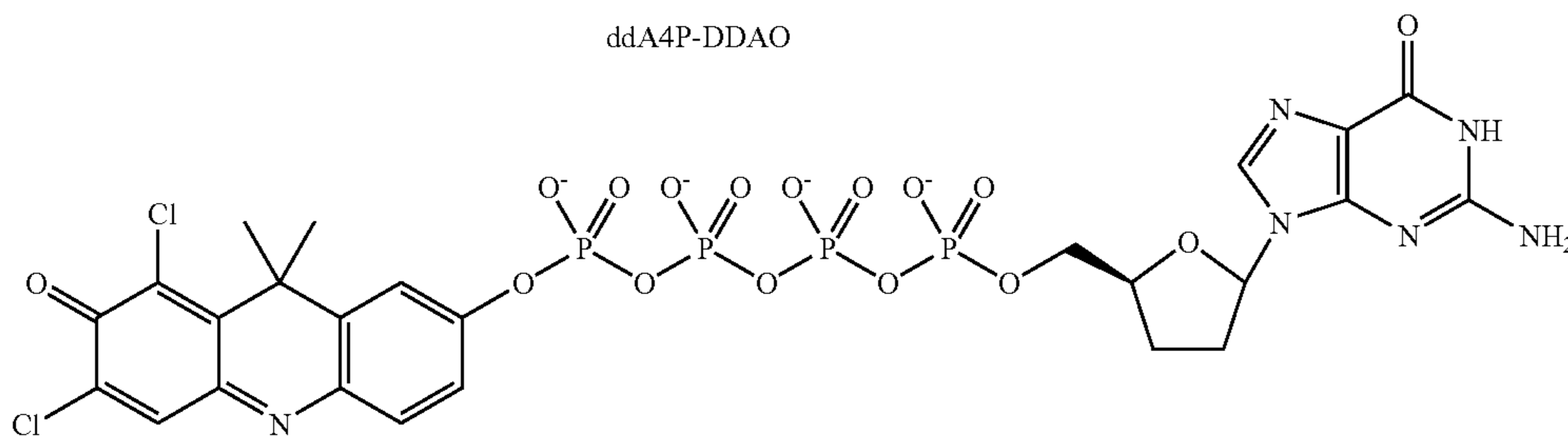
ddG4P-DDAO
