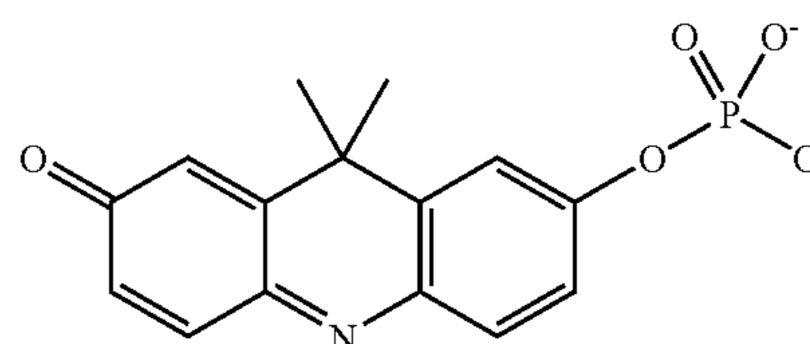
9,9-dimethylacridin-2-one-7-yl phosphate
