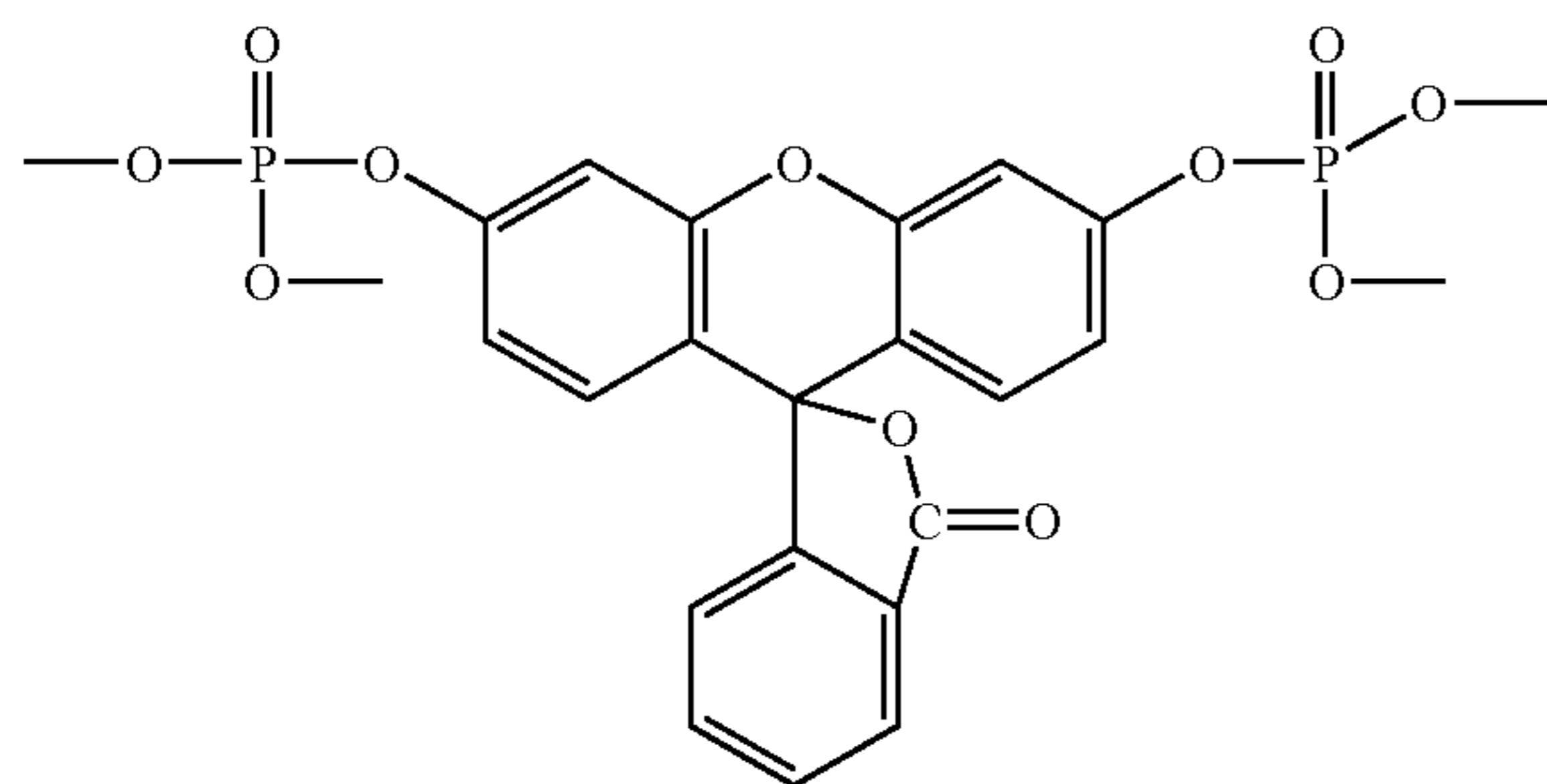
fluorescein diphosphate
