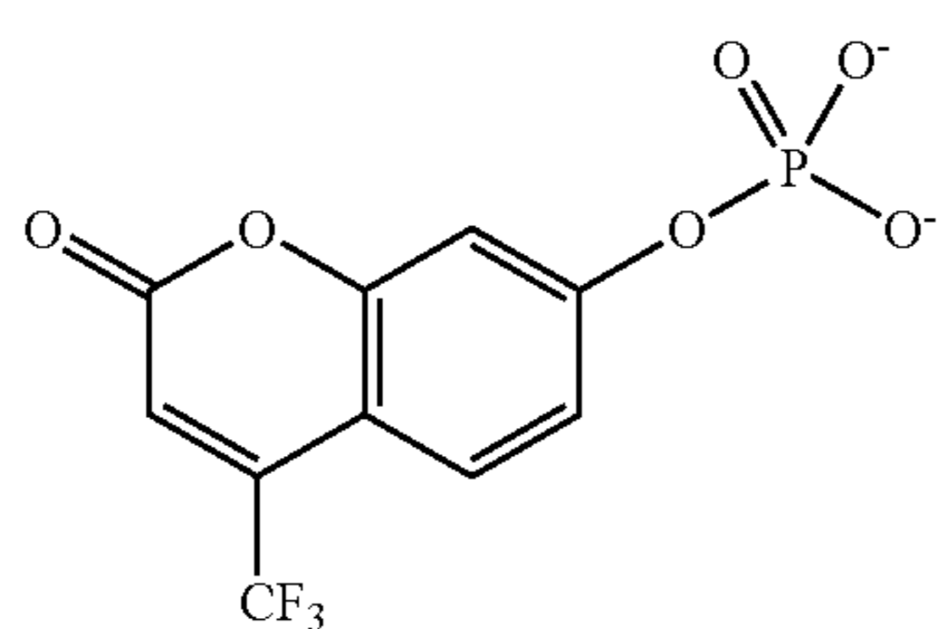
4-Trifluoromethylumbelliferyl phosphate
