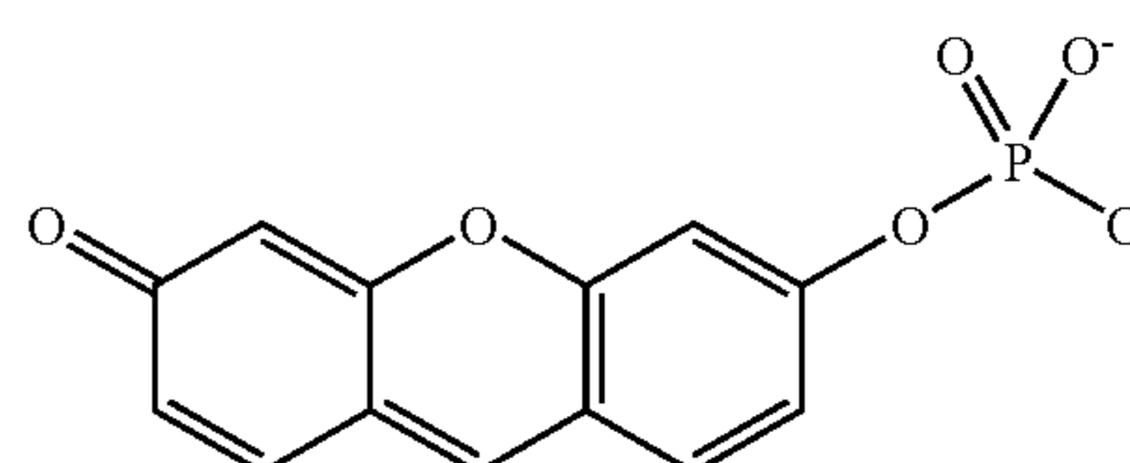
Resorufin phosphate
