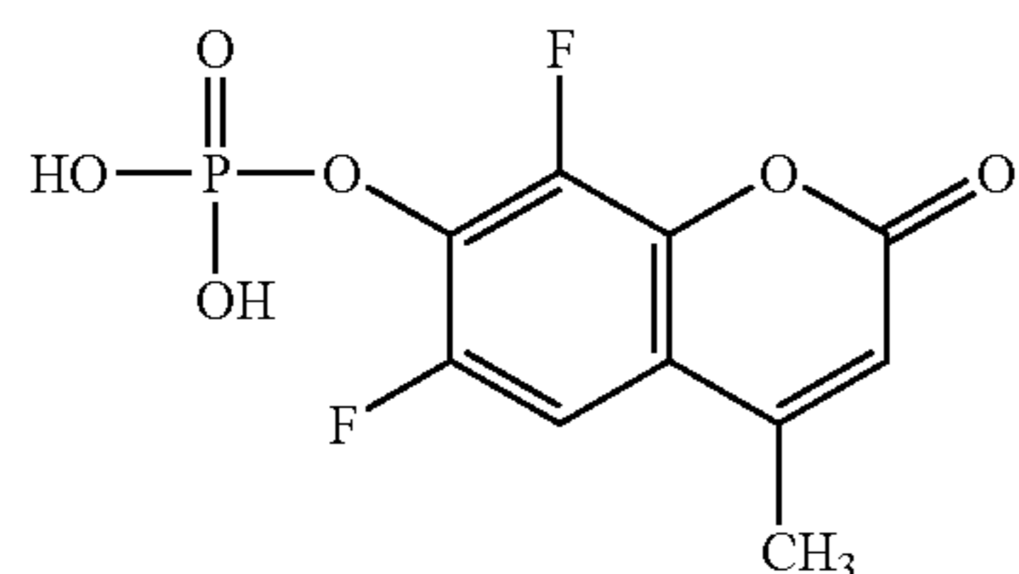
6,8-difluoro-4-methylumbelliferyl phosphate
