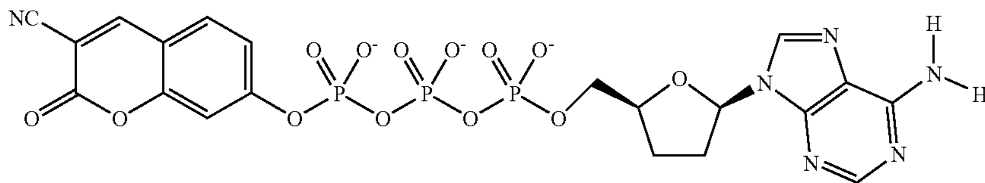
\gamma -(3-cyanocoumarinyl)dideoxyadenosine-5'-triphosphate ( \gamma CNCoumarin-ddATP)
