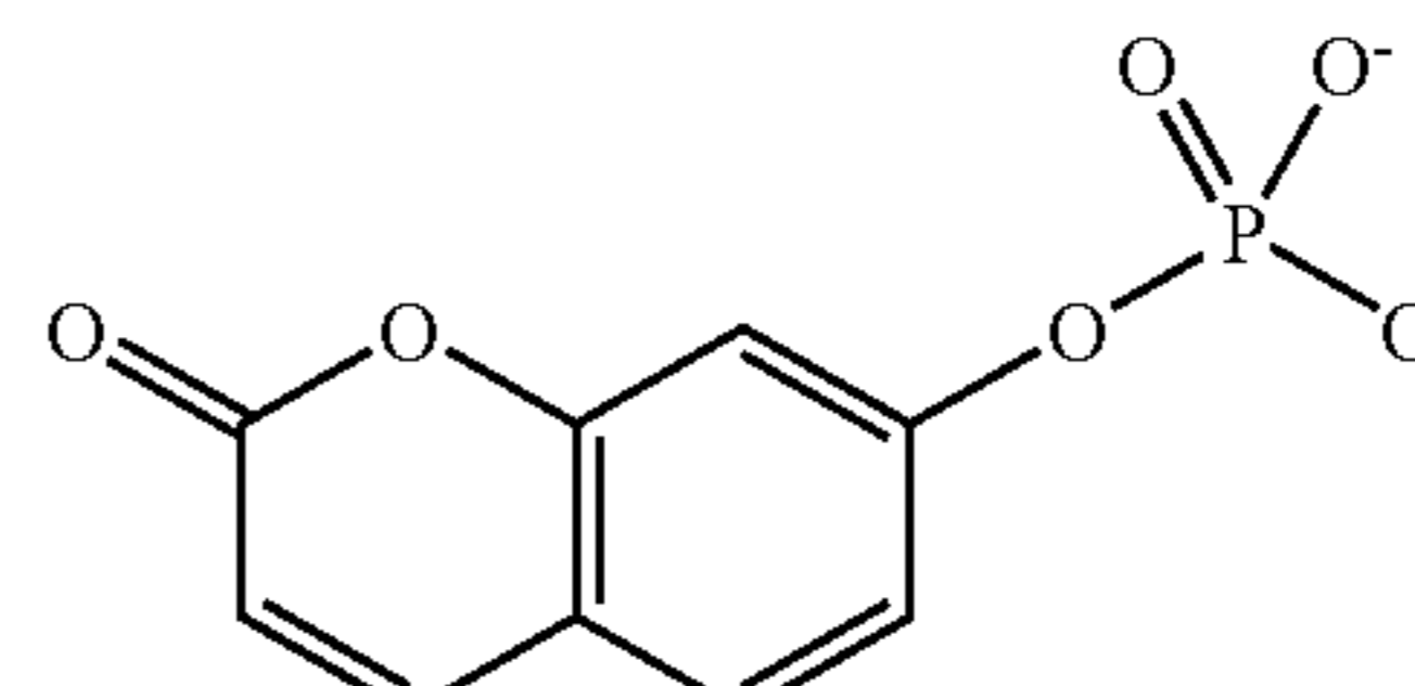
Umbelliferyl phosphate
