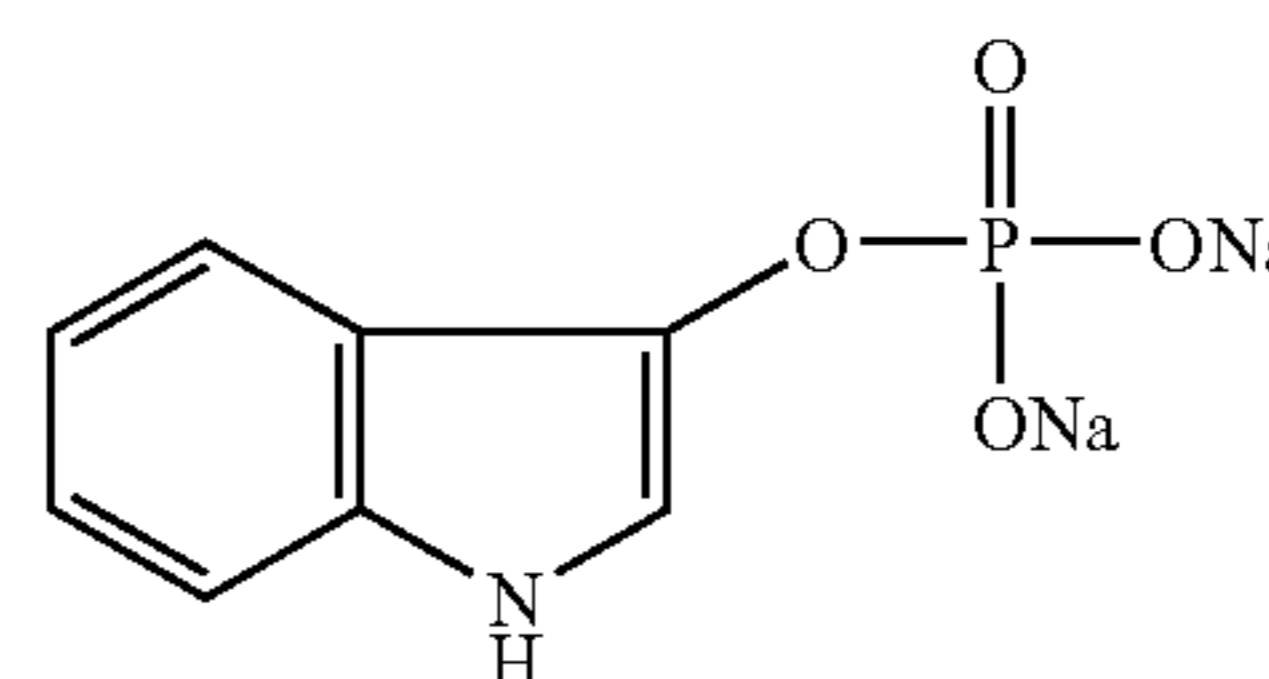
5-bromo-4-chloro-3-indolyl phosphate (disodium salt)
