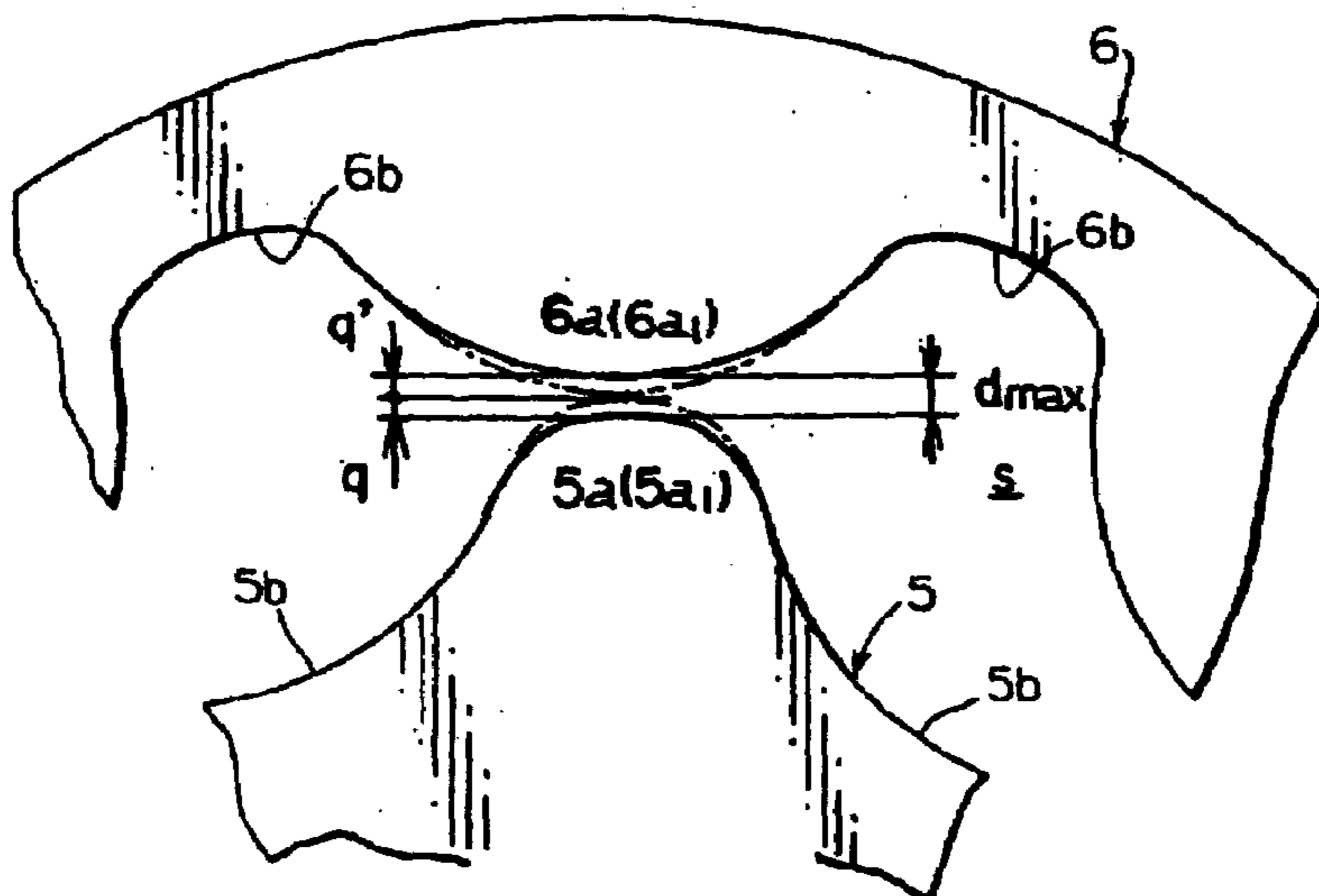
FIG. 11 (C)
