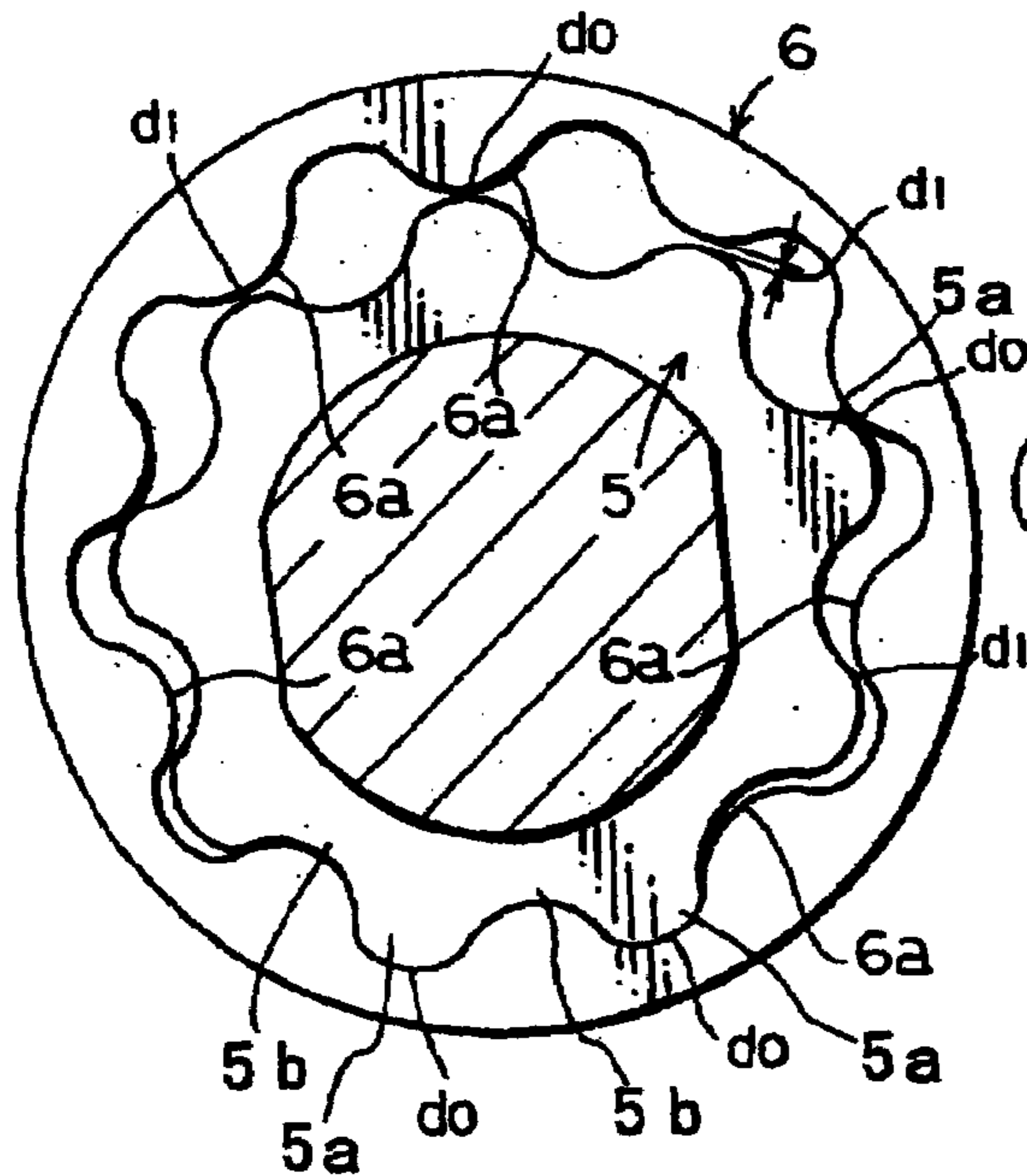
FIG. 6 (A)
