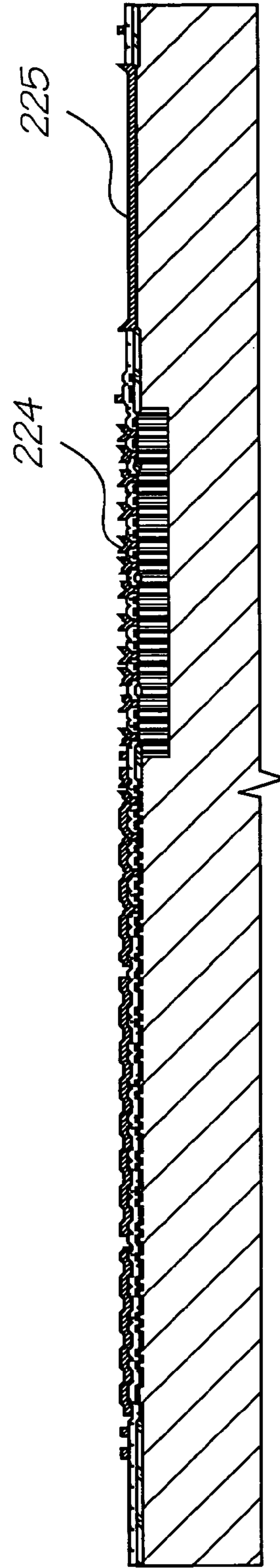
Deposit Metal 1
