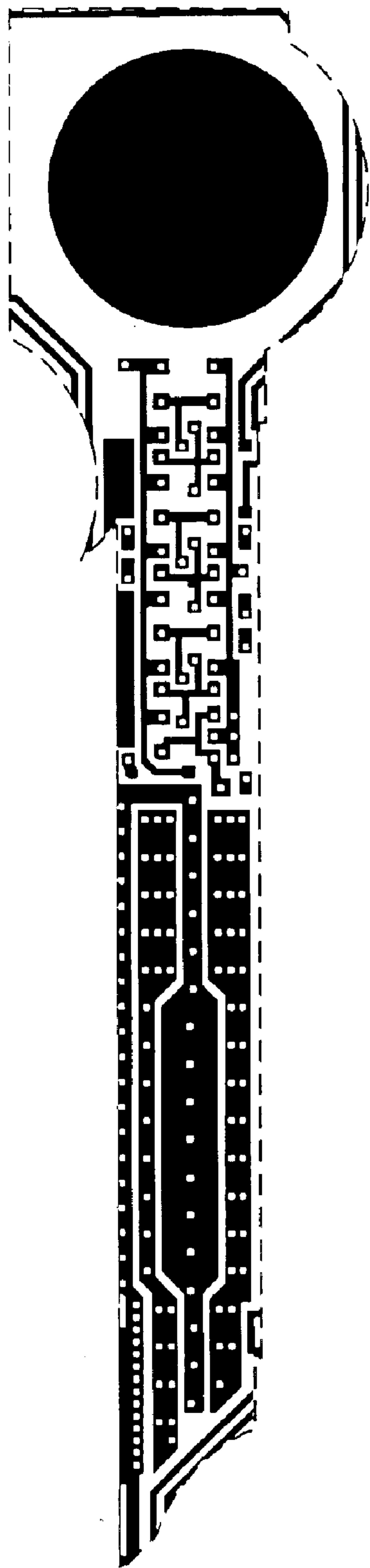
Metal 1 mask
