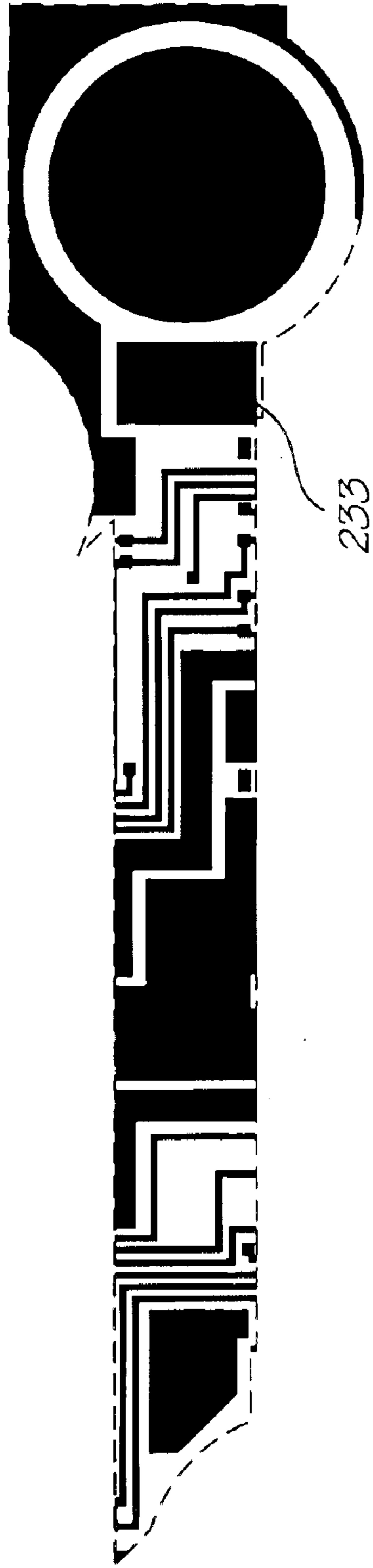
Metal 2 mask
