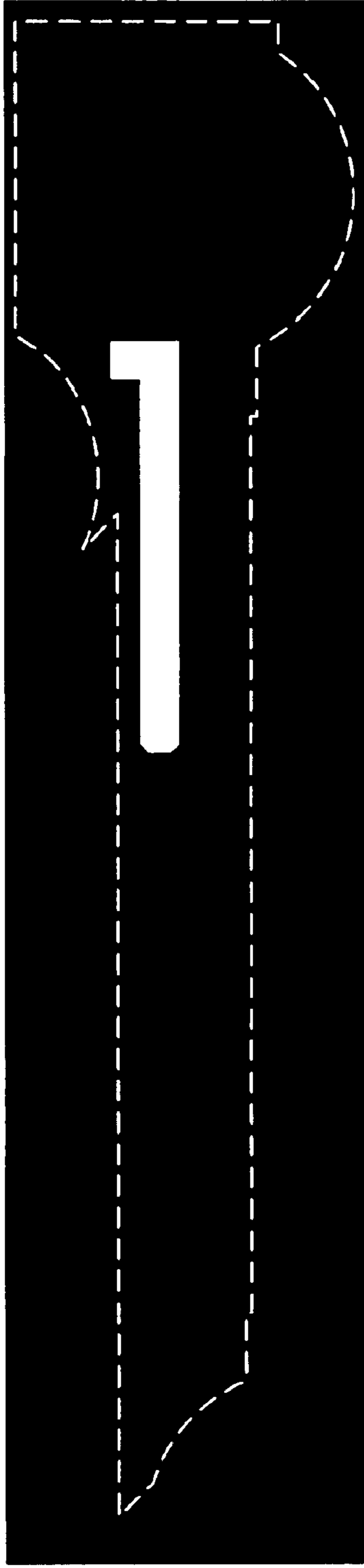
N-Well mask
