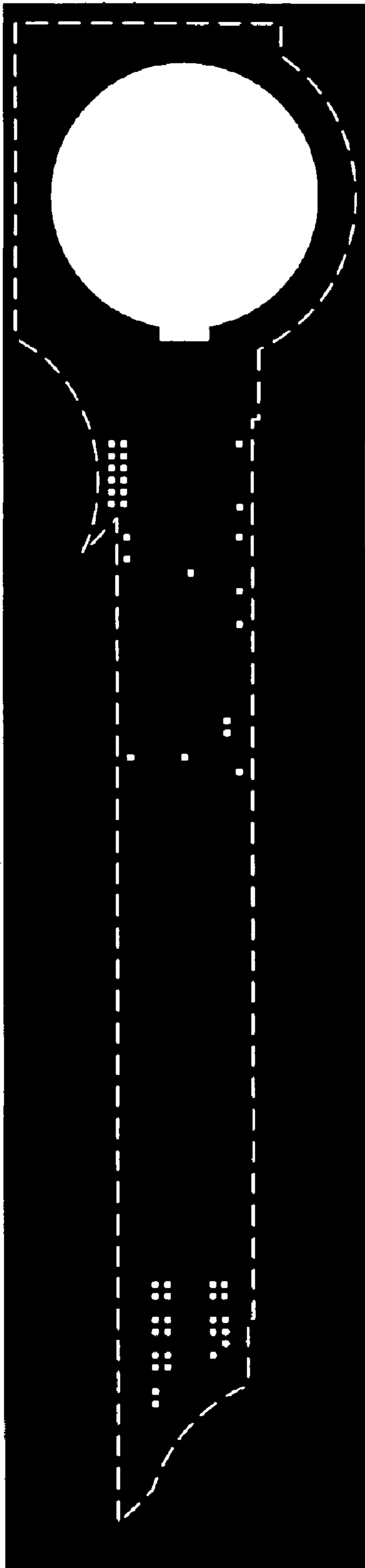
Via 1 mask
