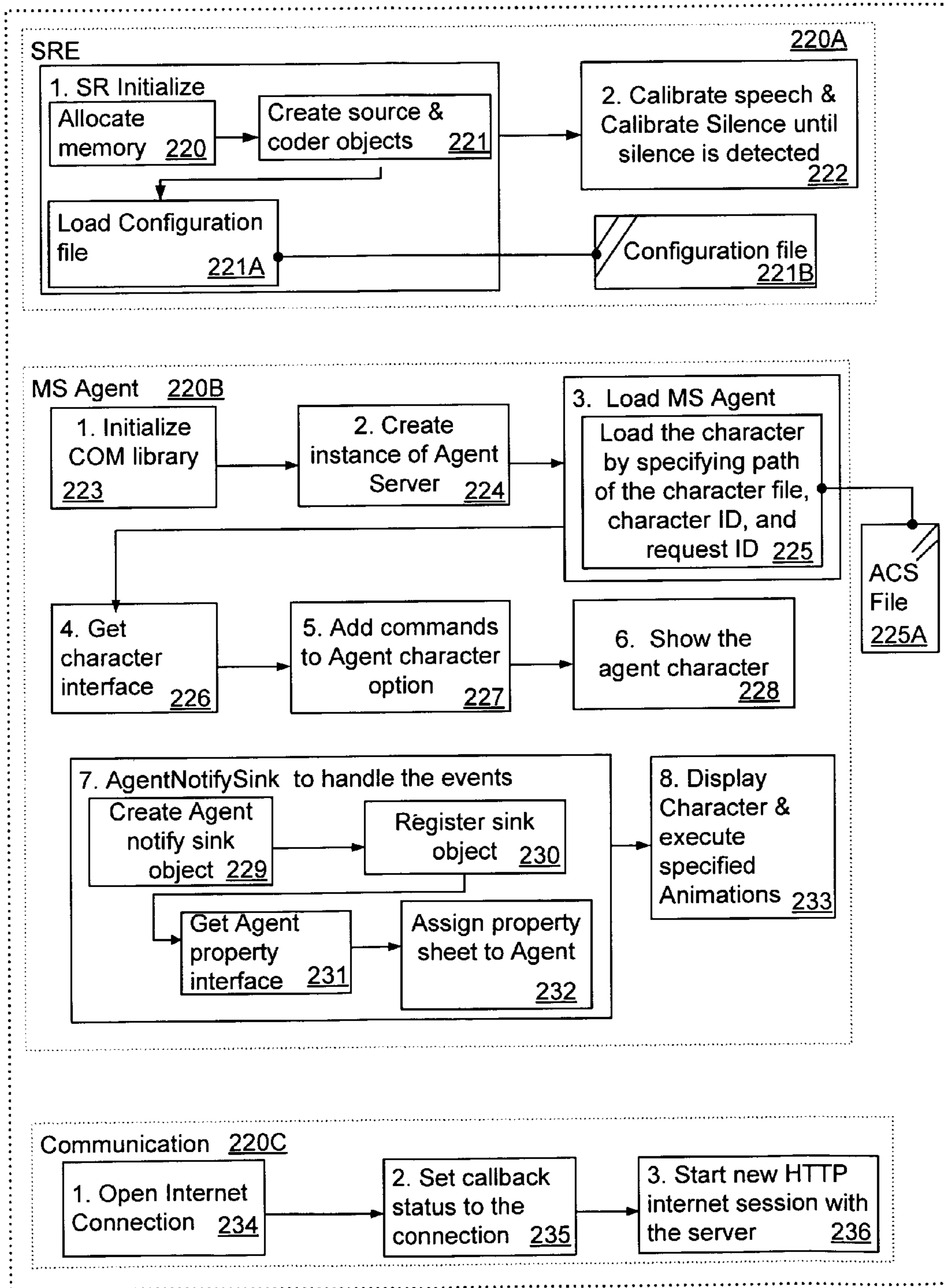
Fig. 2-2 client-side Initialization
