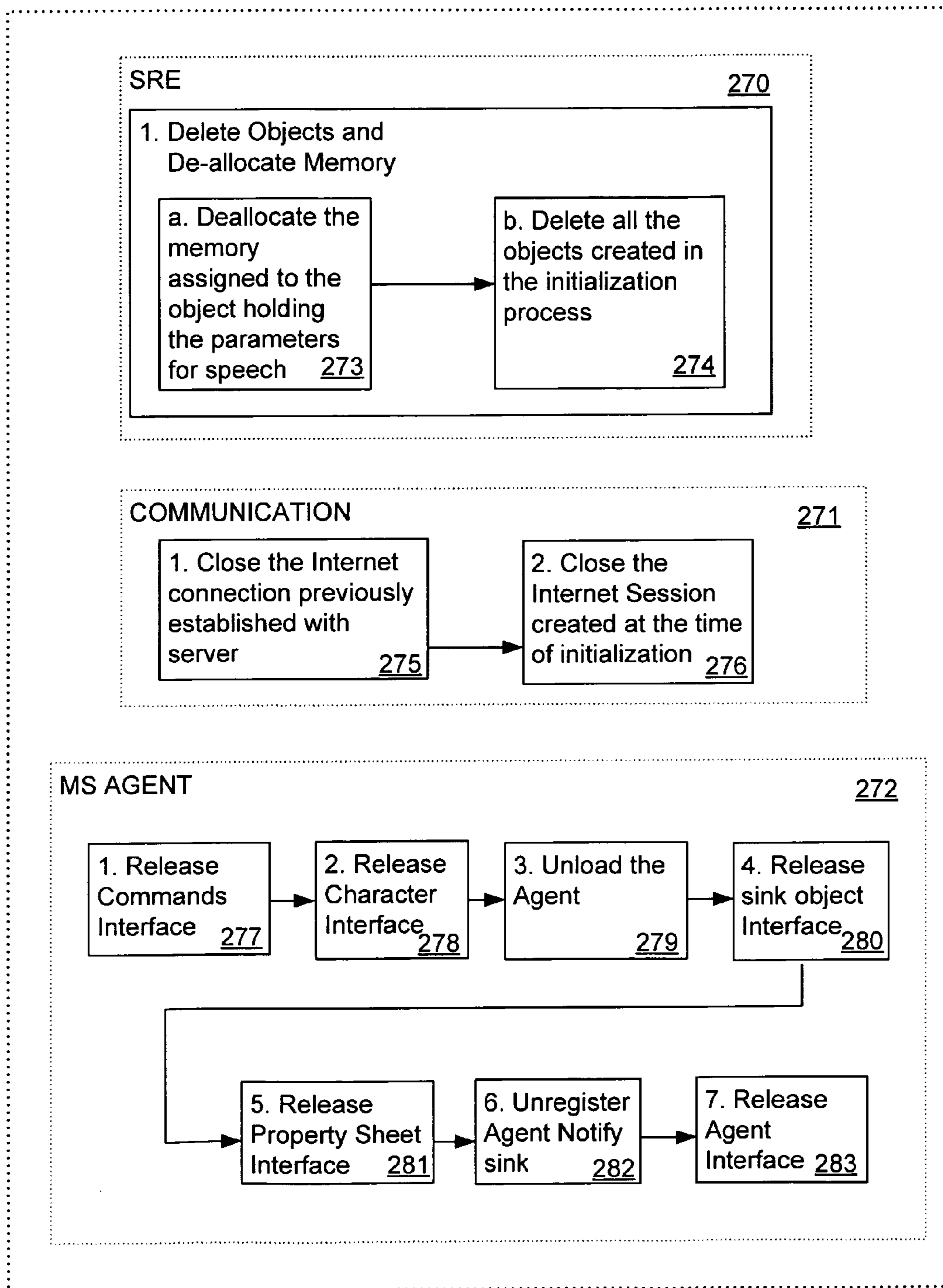
Fig. 4 Client-side Un-Initialization
