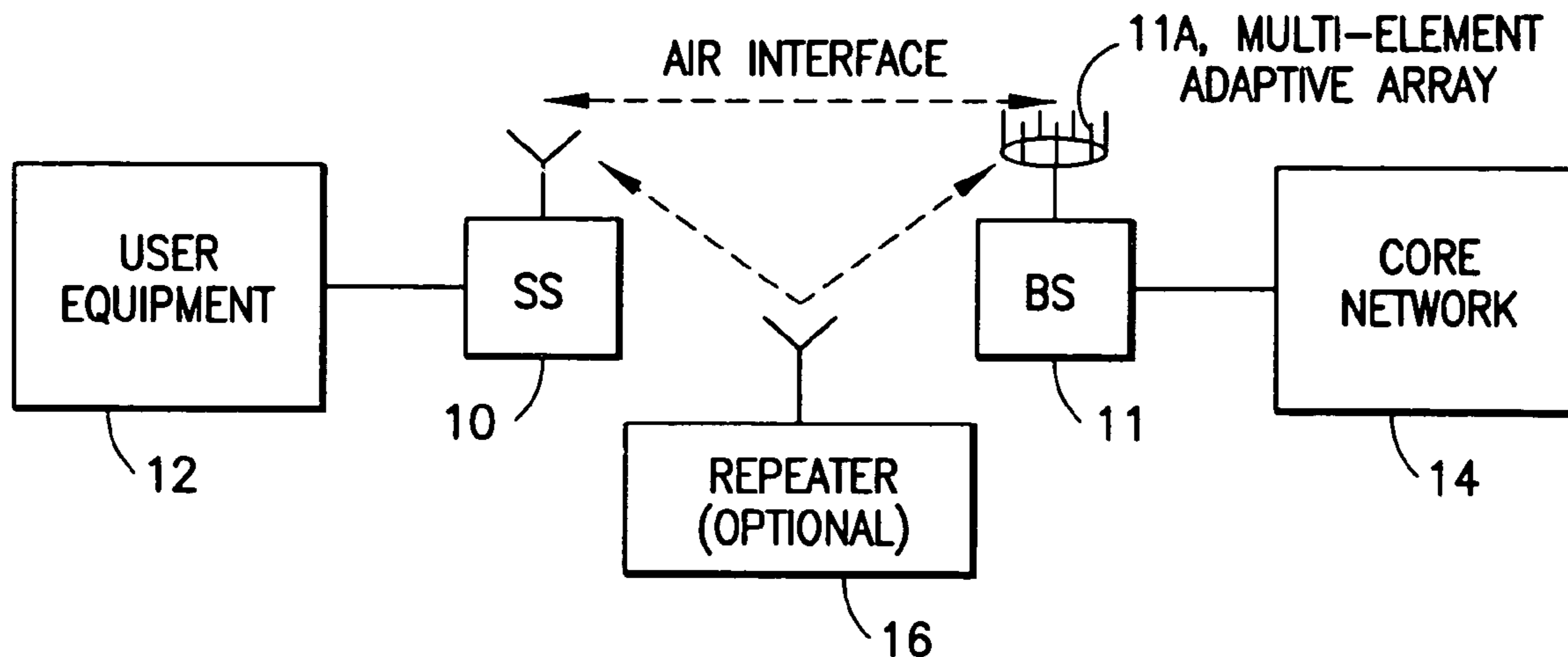
WIRELESS ACCESS REFERENCE MODEL
