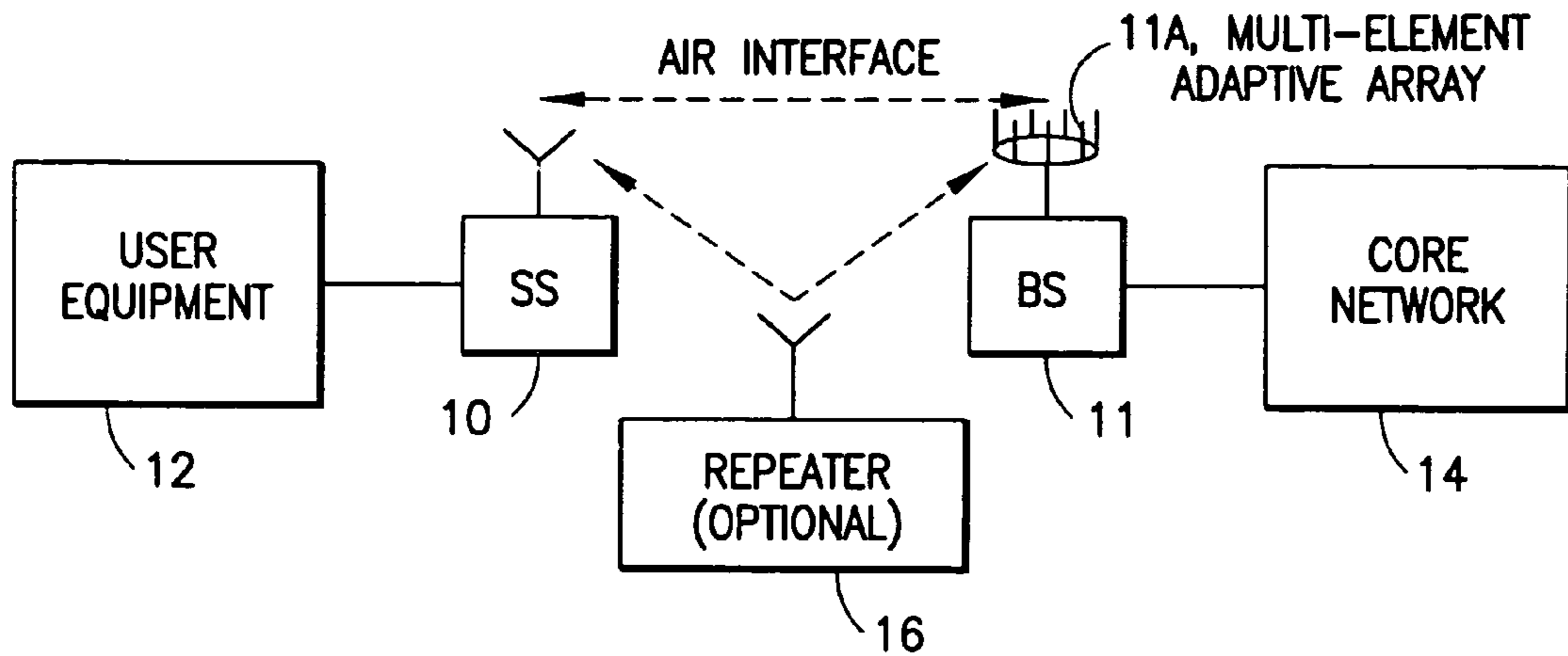
FIG. 1 WIRELESS ACCESS REFERENCE MODEL
