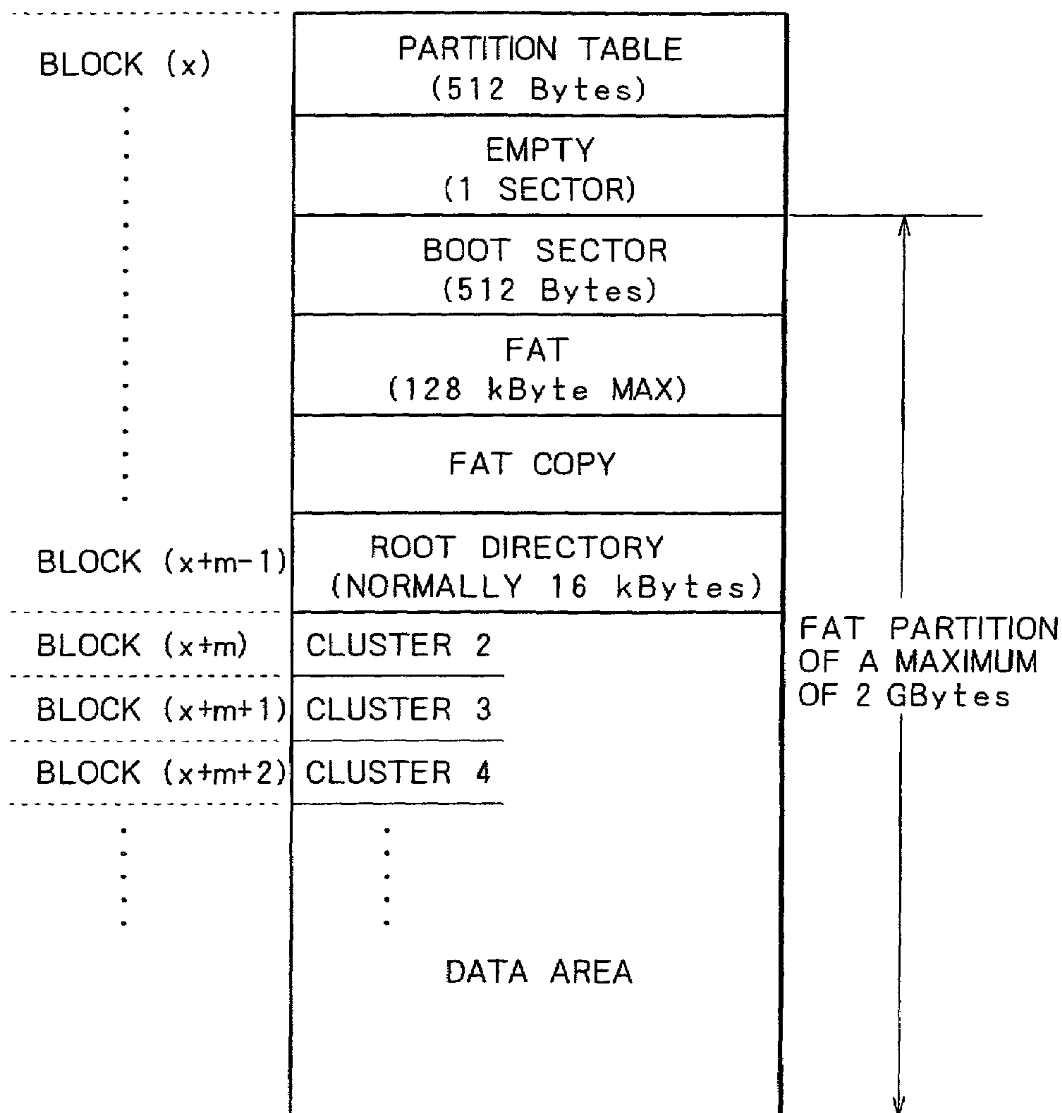
FAT STRUCTURE OUTLINE
