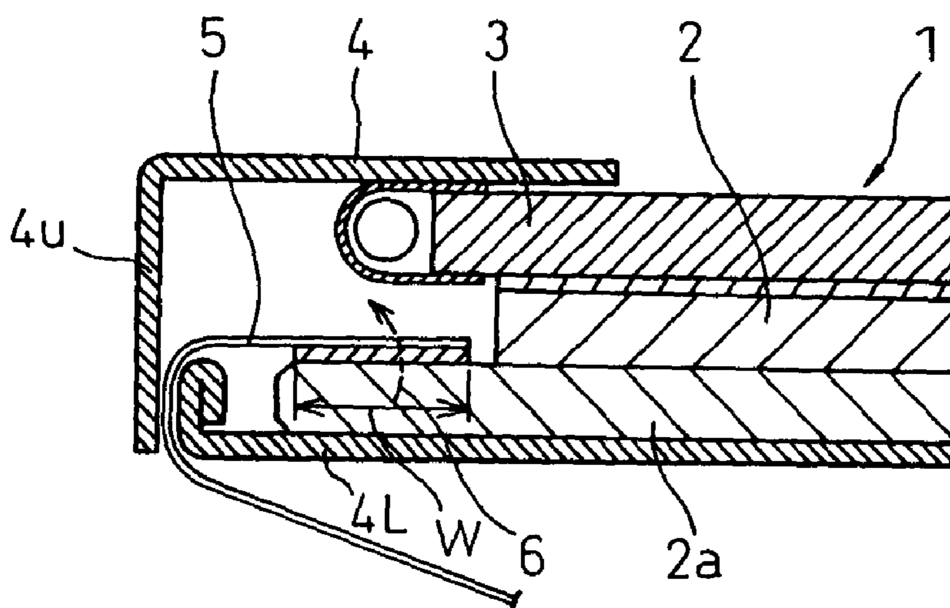
Fig. 9 PRIOR ART
