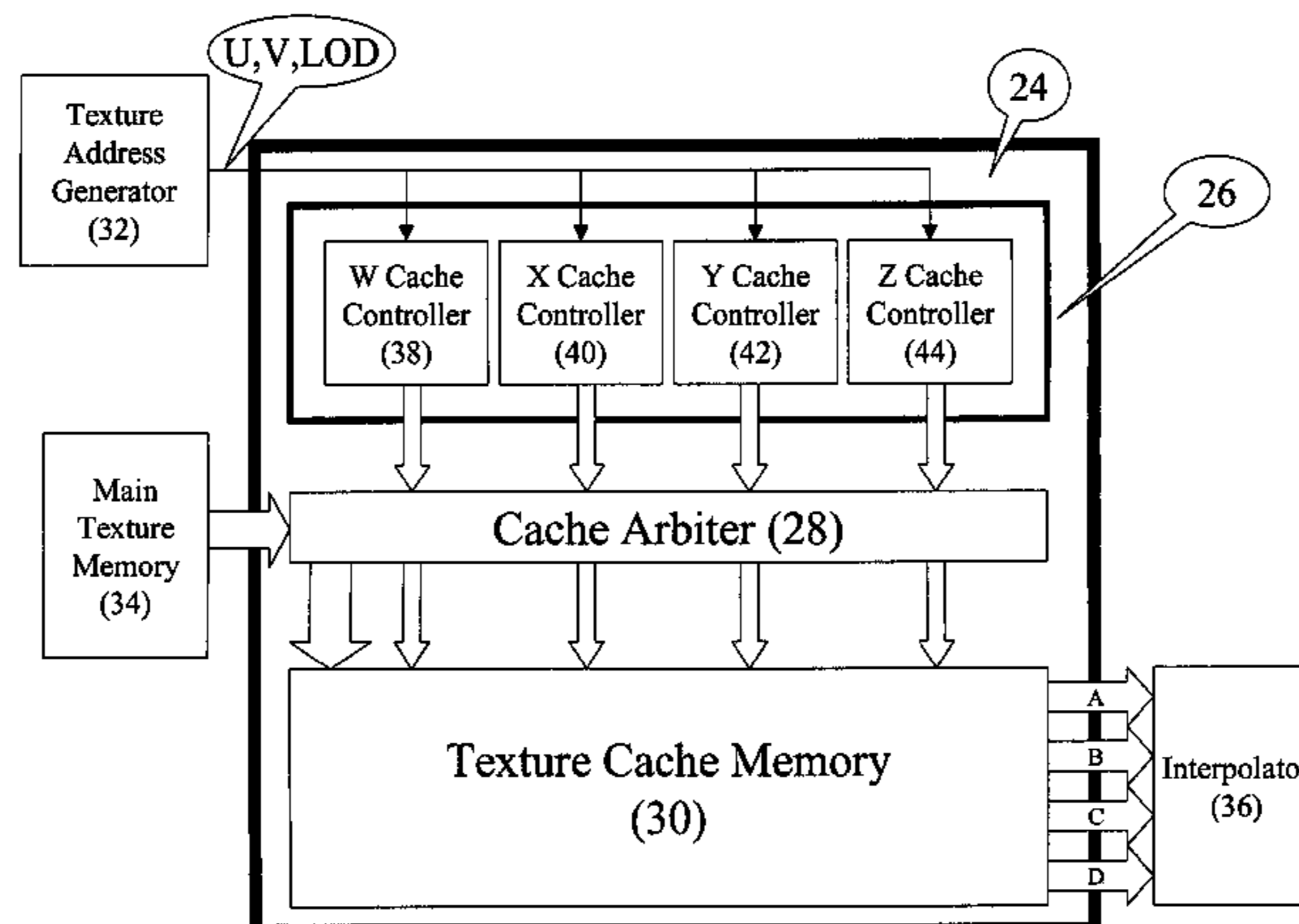
Texture Cache System
