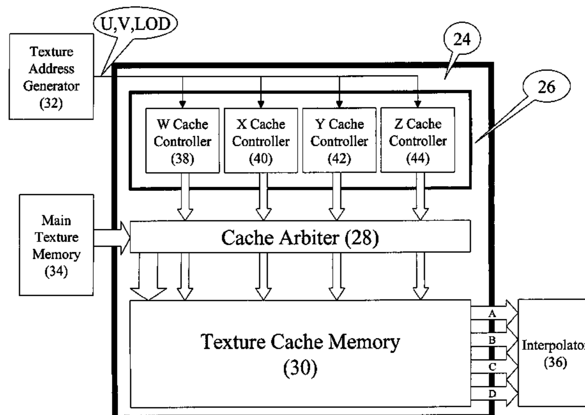
Texture Cache System
