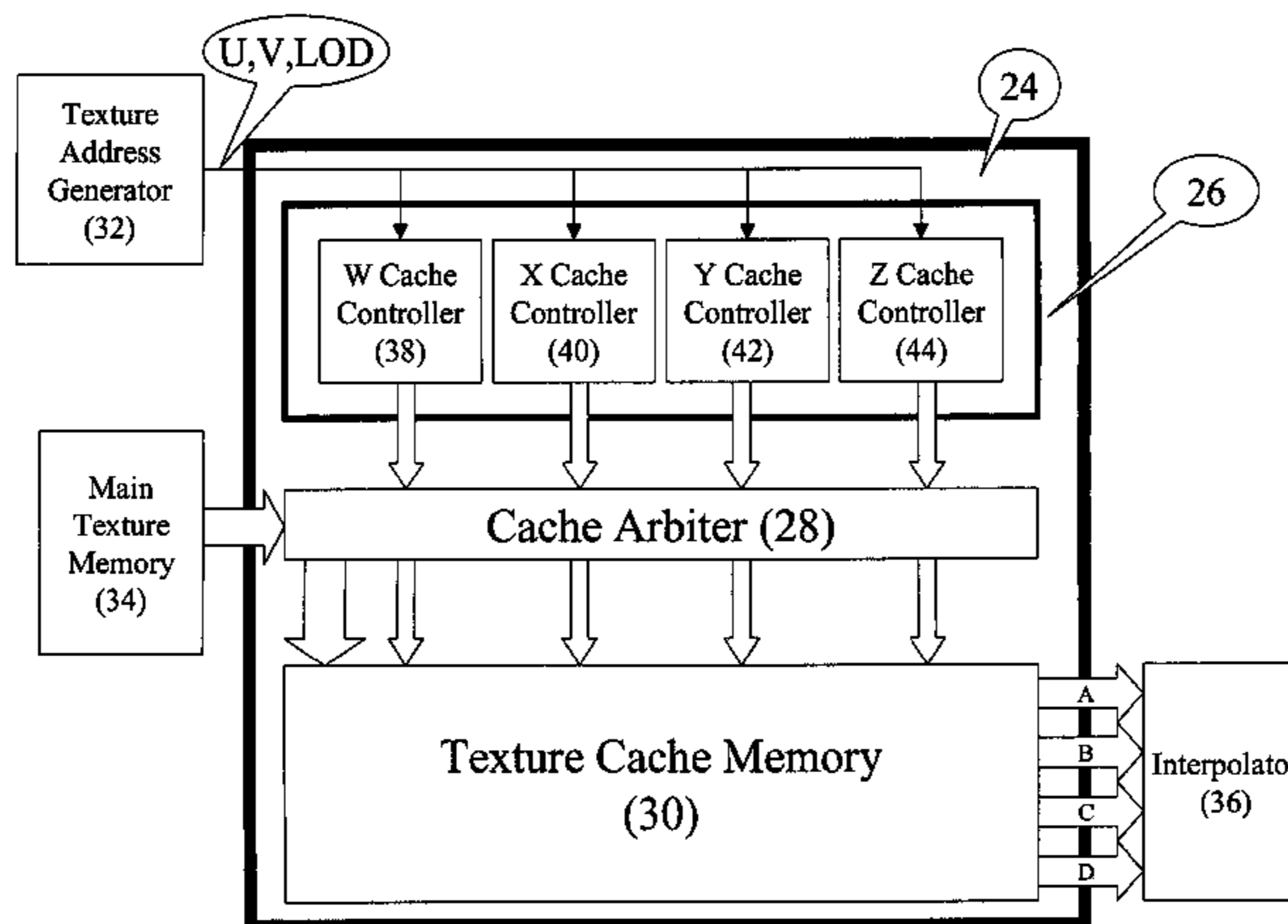
Texture Cache System
