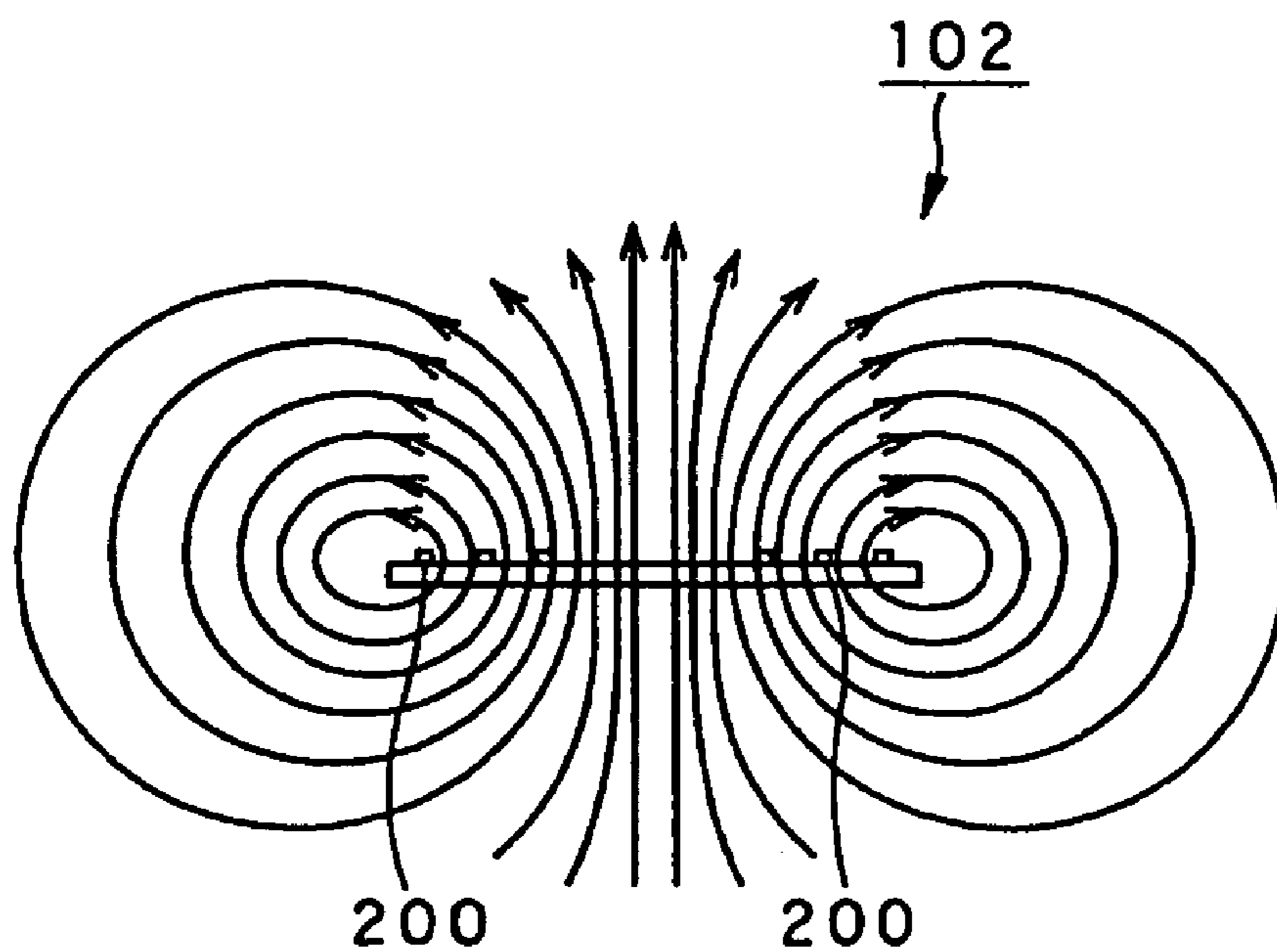
FIG. 3 (PRIOR ART)
