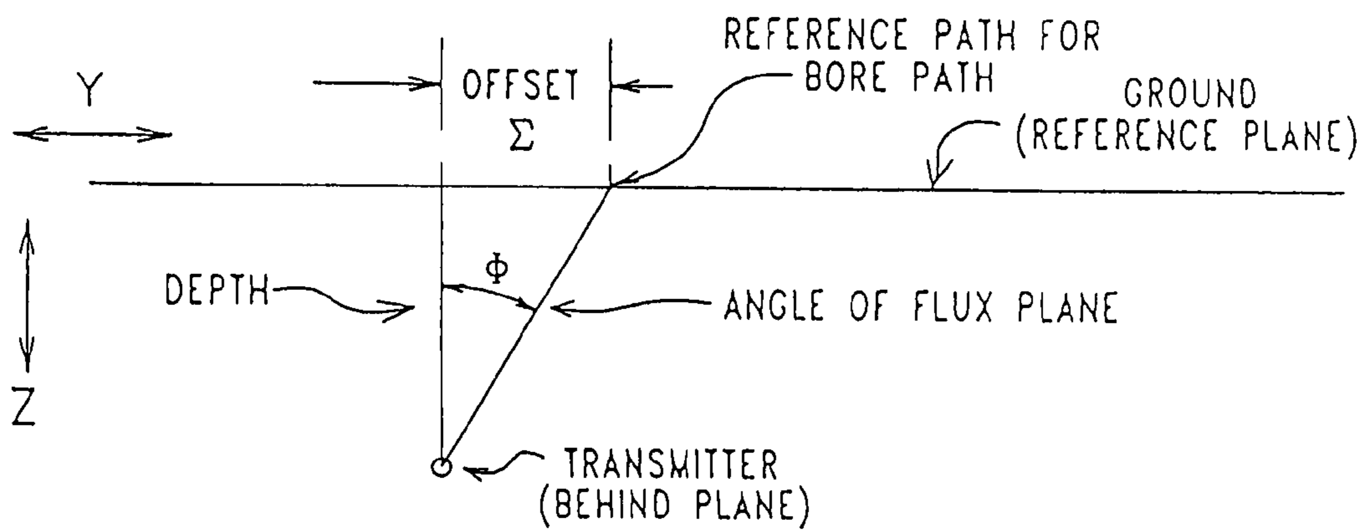
FRONT VIEW FIG. 13
