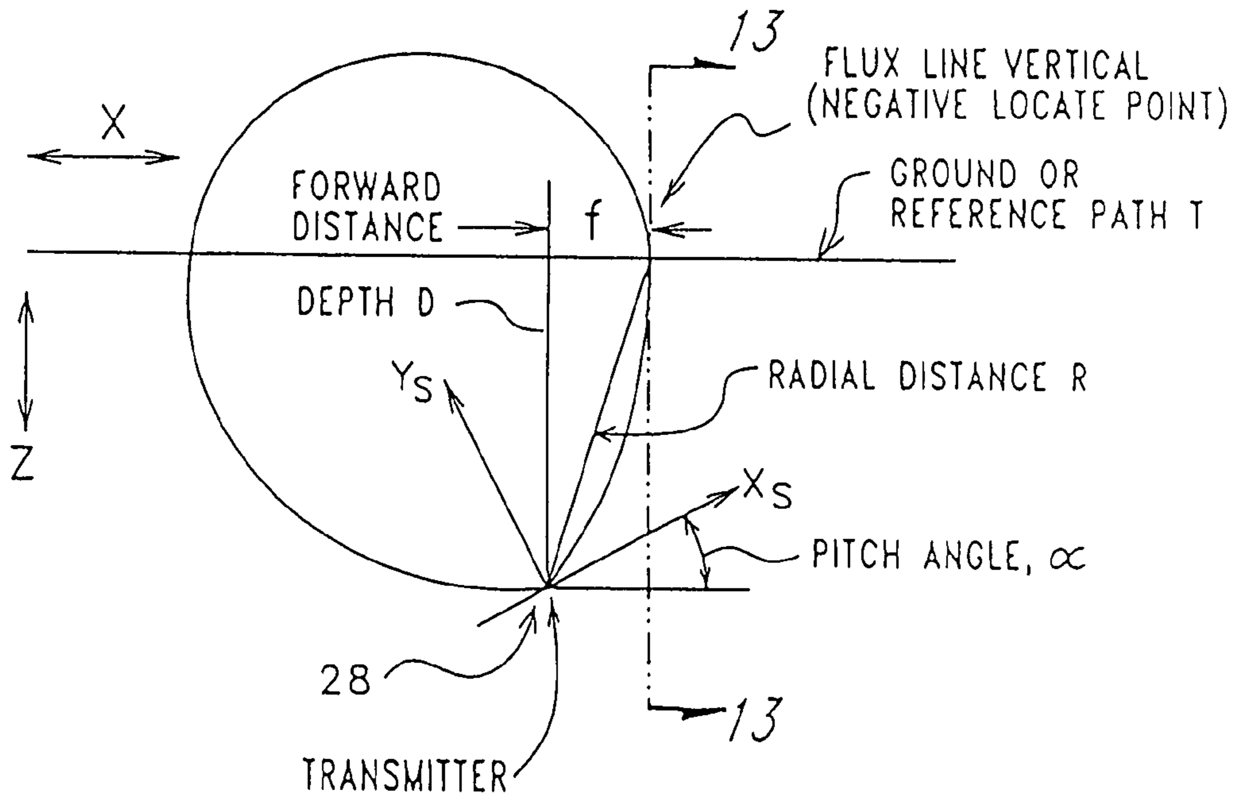
SIDE VIEW FIG. 12
