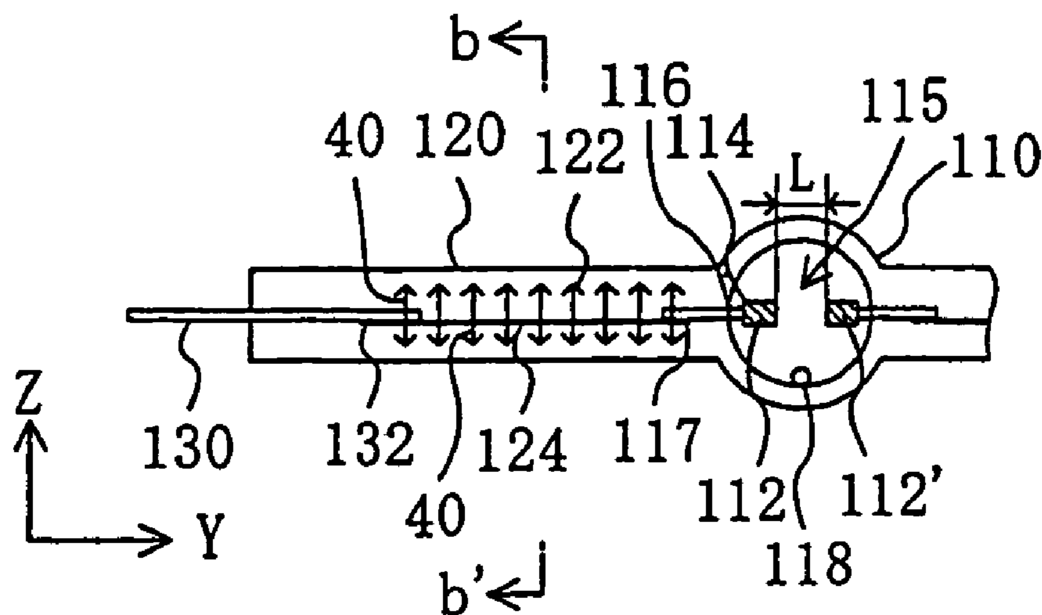
PRIOR ART FIG. 22A
