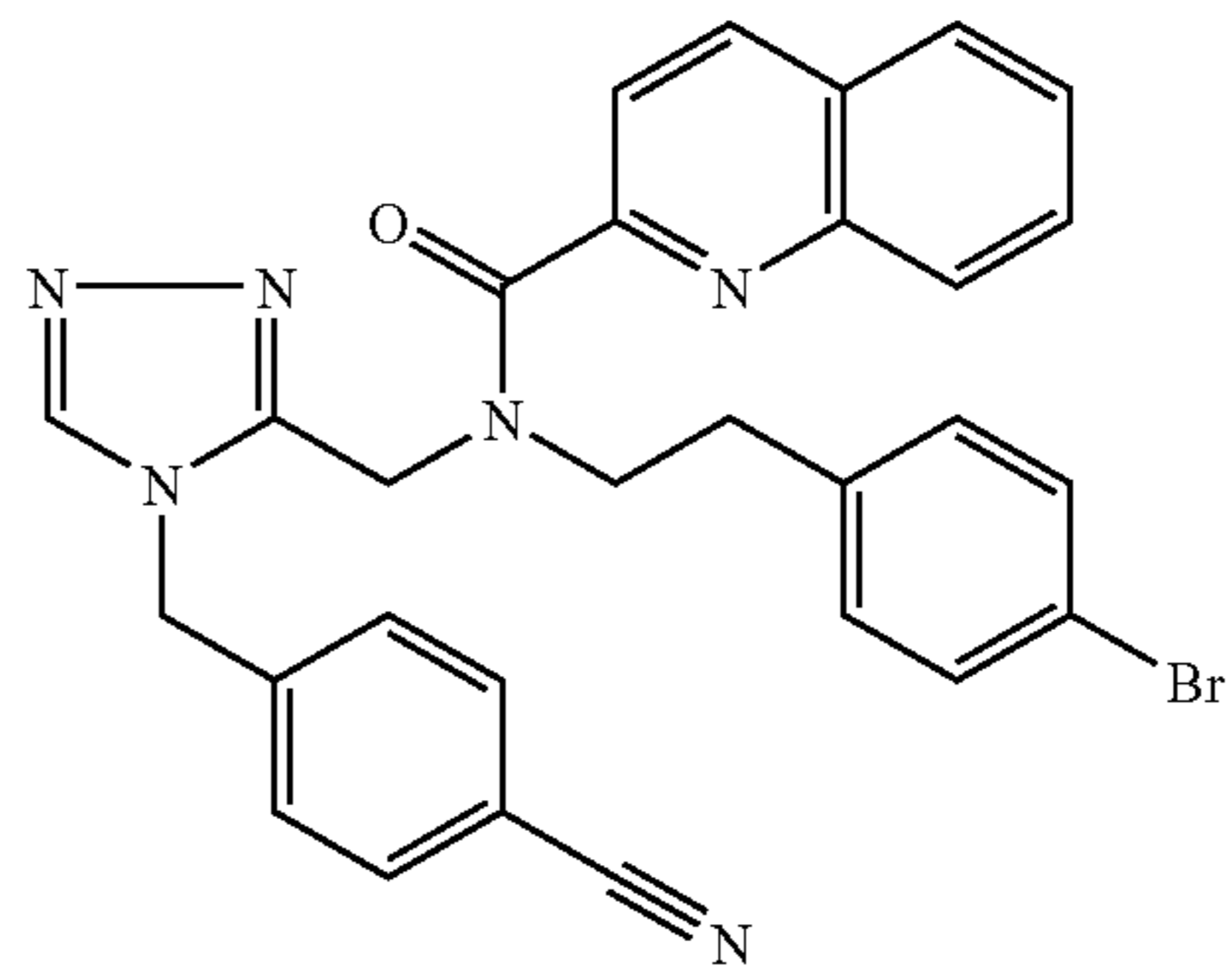
Trifluoroacetate (1:1) comp. 141.
