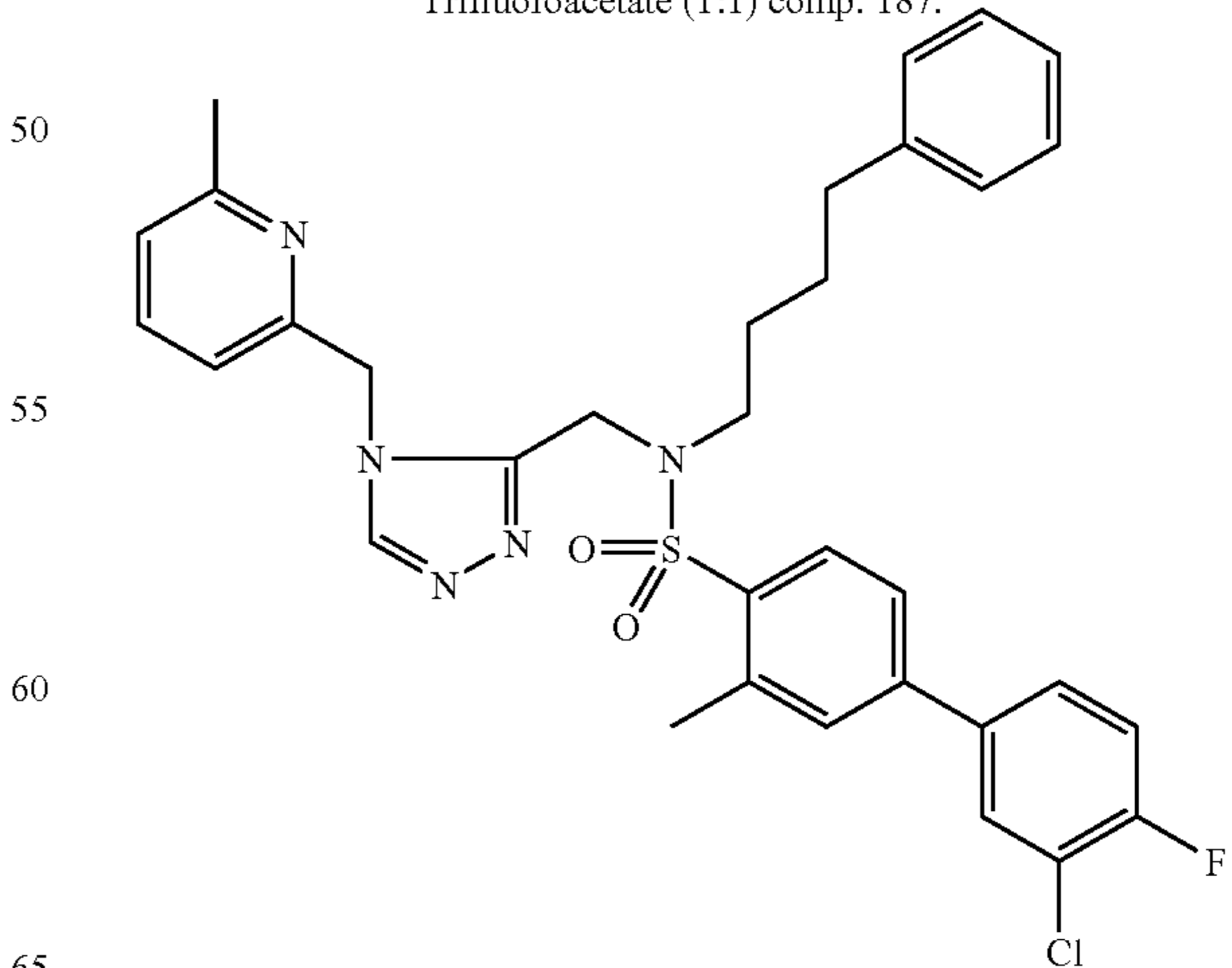
Trifluoroacetate (1:1) comp. 188.
