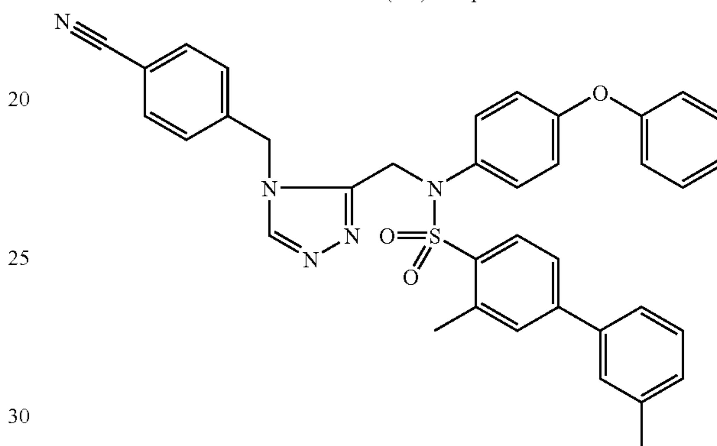
Trifluoroacetate (1:1) comp. 208.
