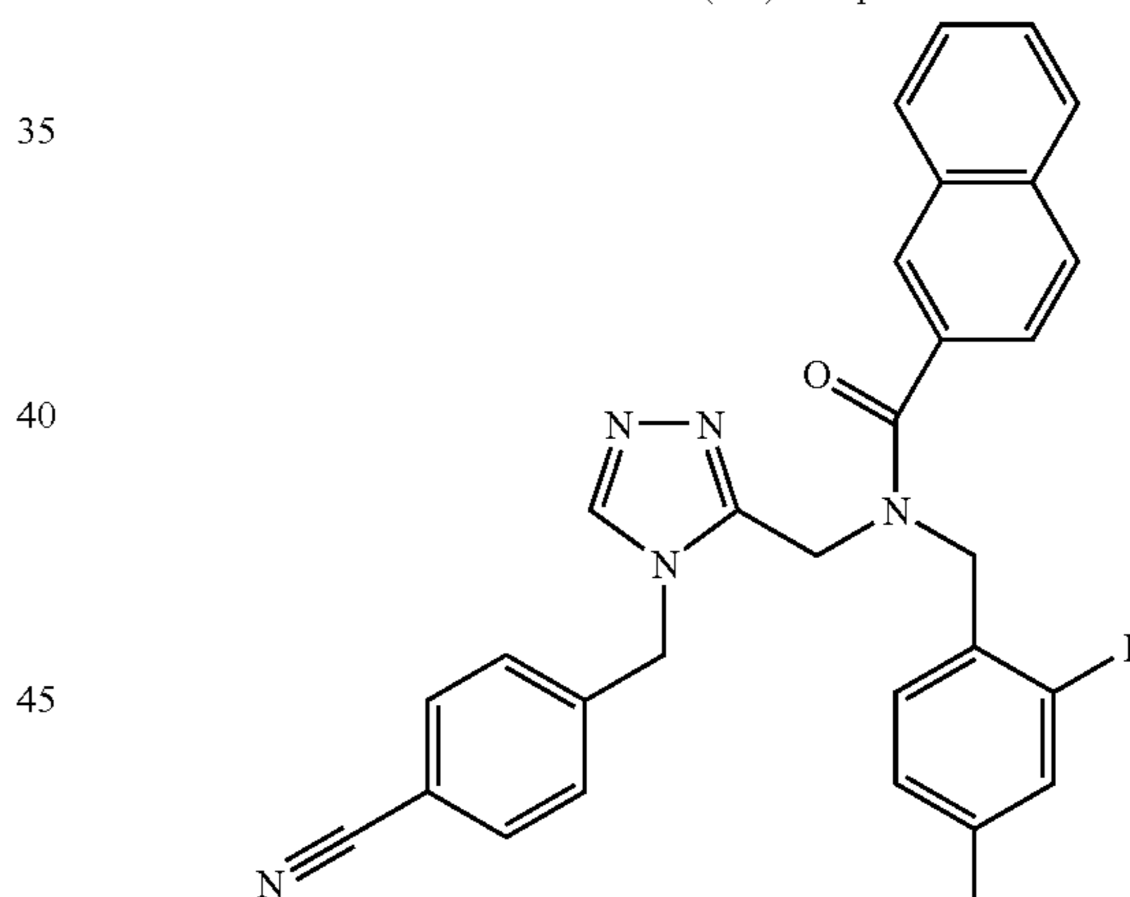
Trifluoroacetate (1:1) comp. 315.
