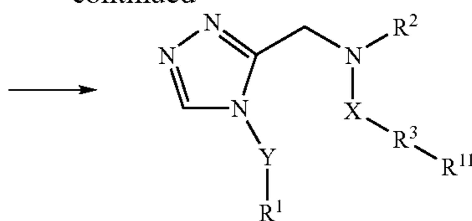
(I-a-1-d)
