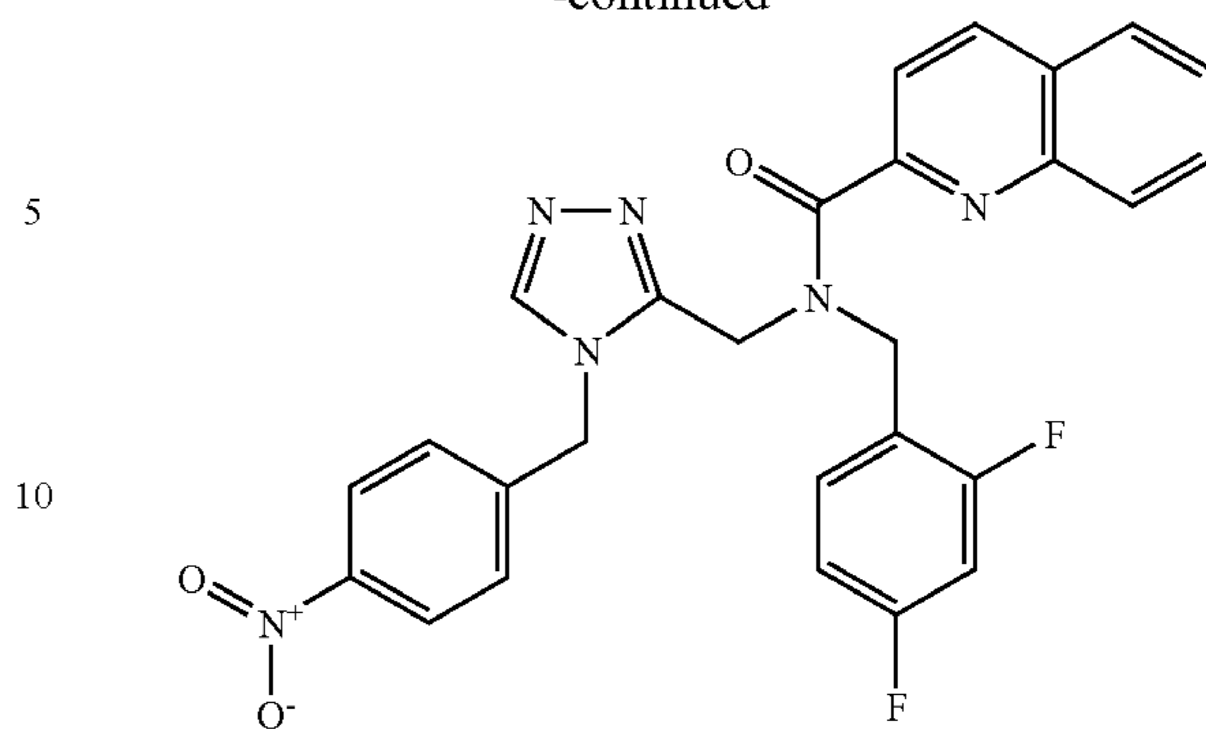
Trifluoroacetate (1:1) comp. 273.
