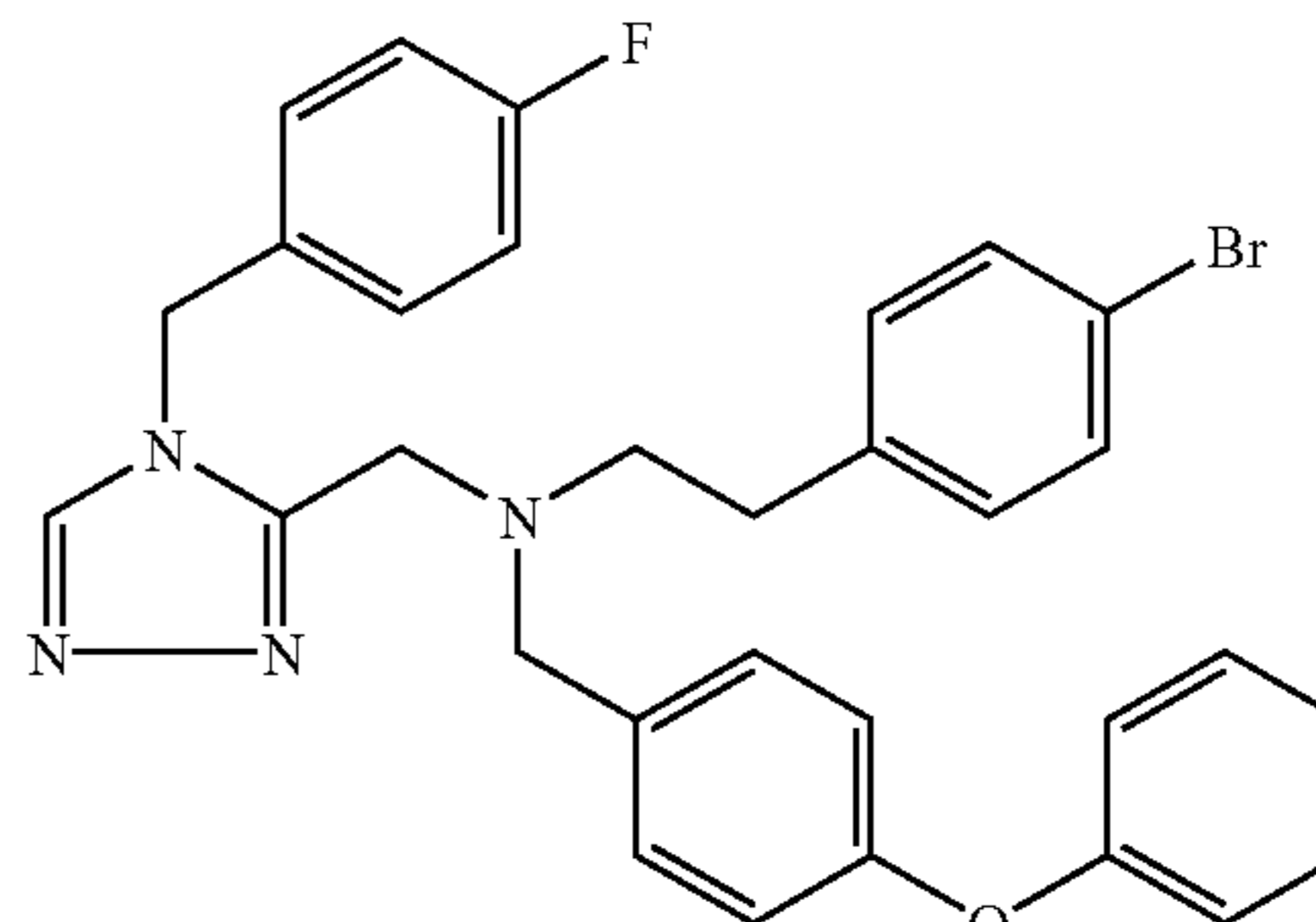
Trifluoroacetate (1:1) comp. 10.
