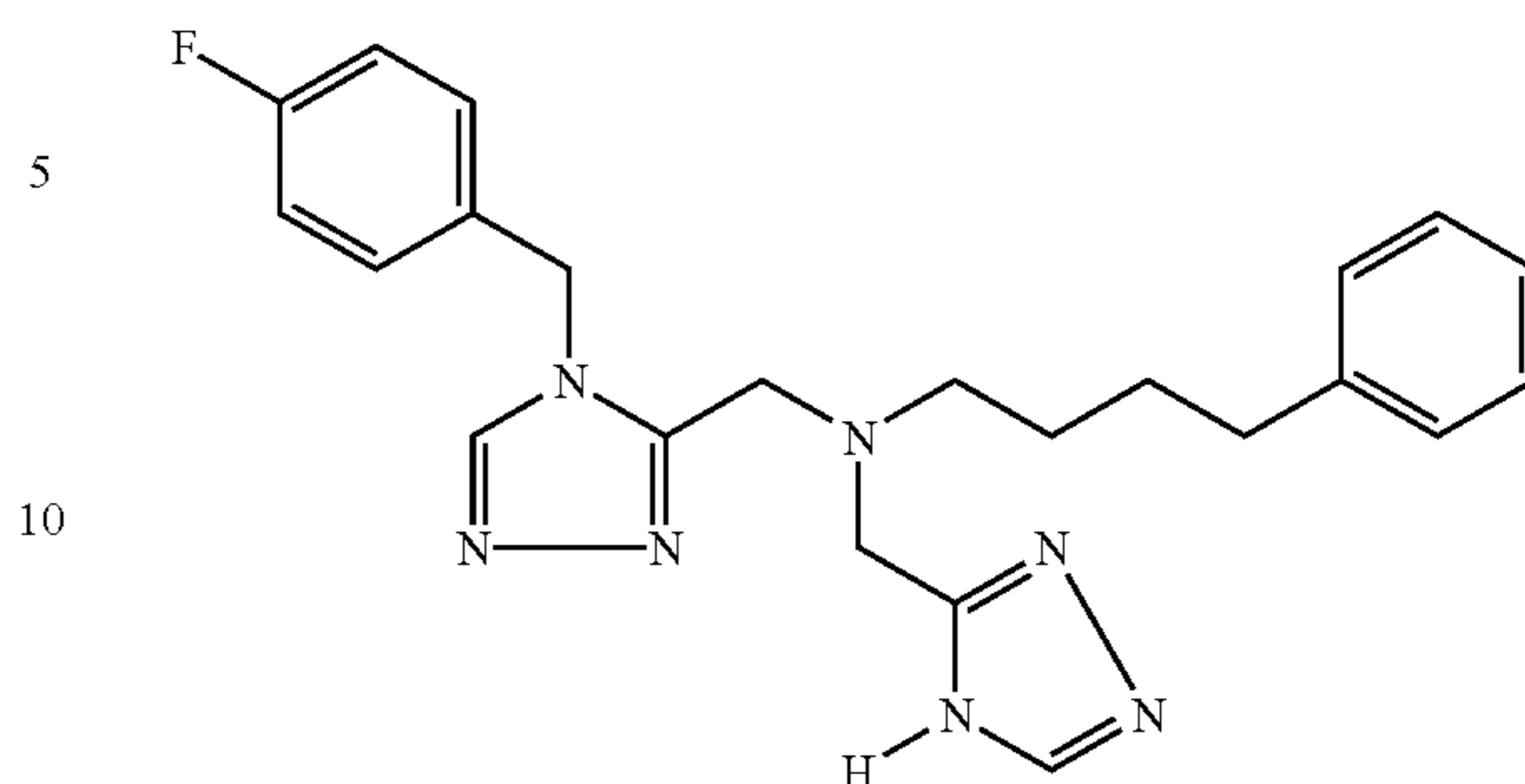
Trifluoroacetate (1:1) comp. 34.
