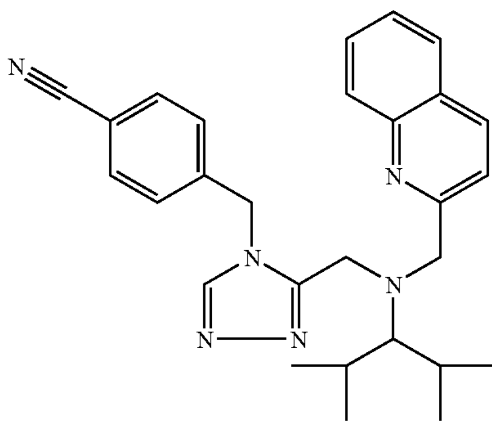
Trifluoroacetate (1:2) comp. 175.
