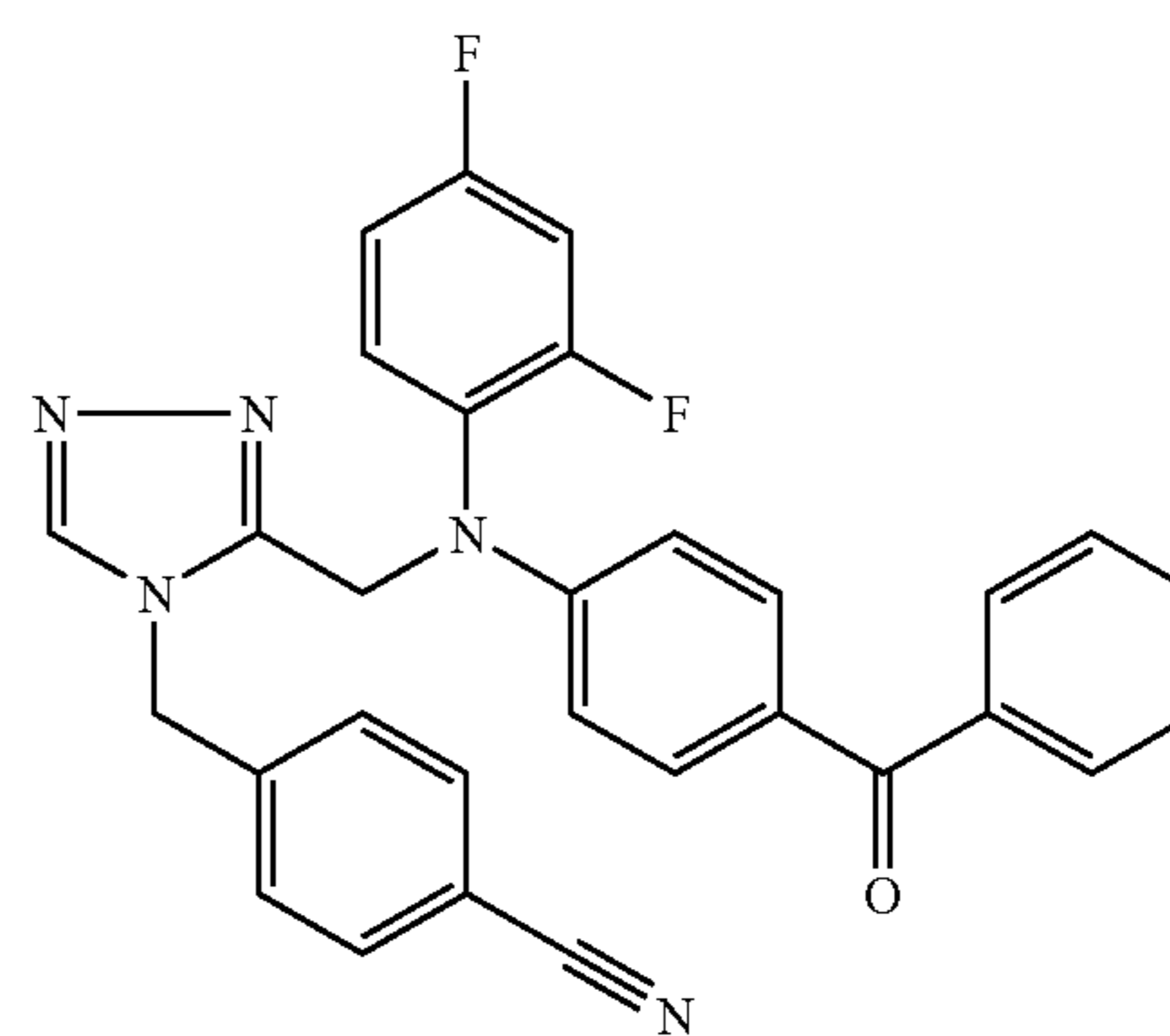
Trifluoroacetate (1:1) comp. 85.
