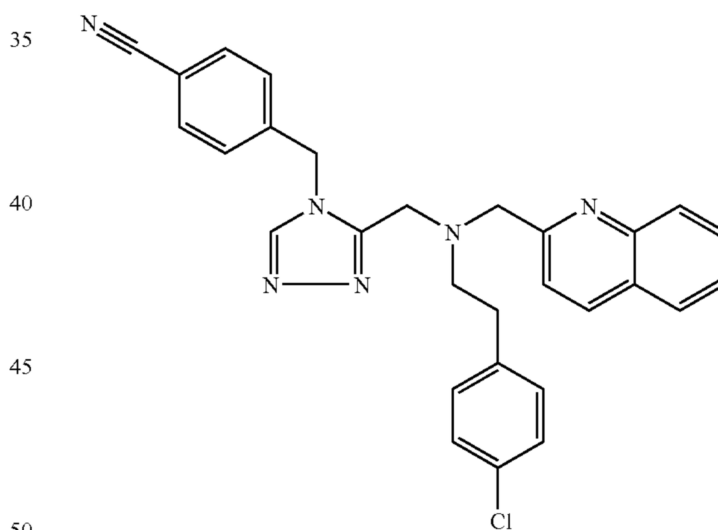
Trifluoroacetate (1:2) comp. 171.
