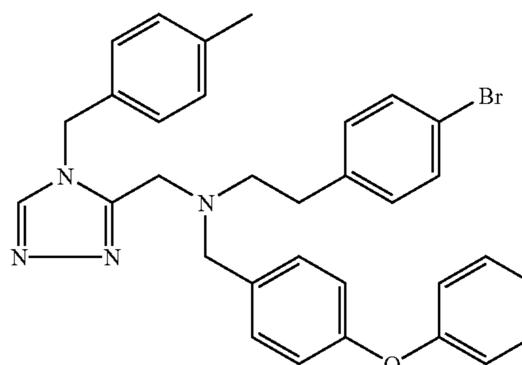
Trifluoroacetate (1:1) comp. 9.
