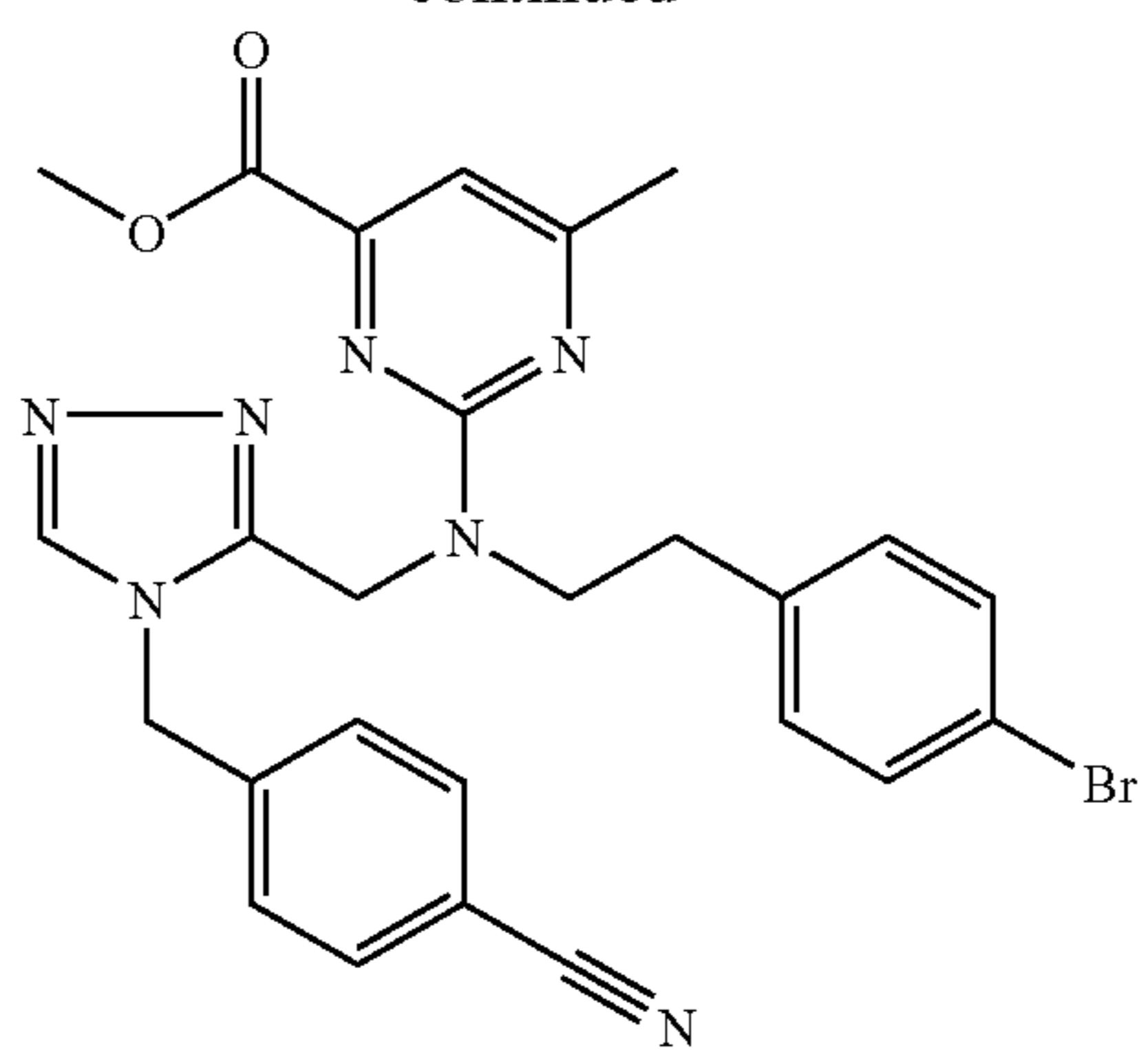
Trifluoroacetate (1:1) comp. 161.
