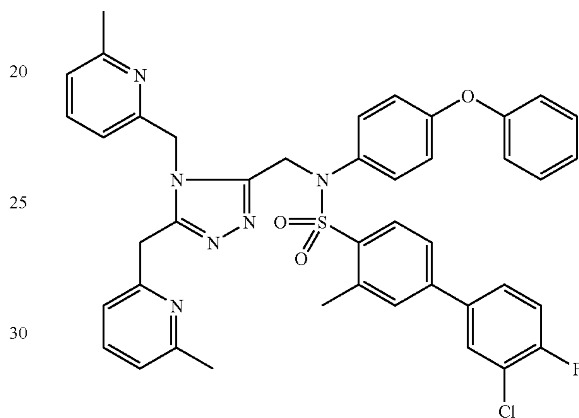
Trifluoroacetate (1:1) comp. 230.
