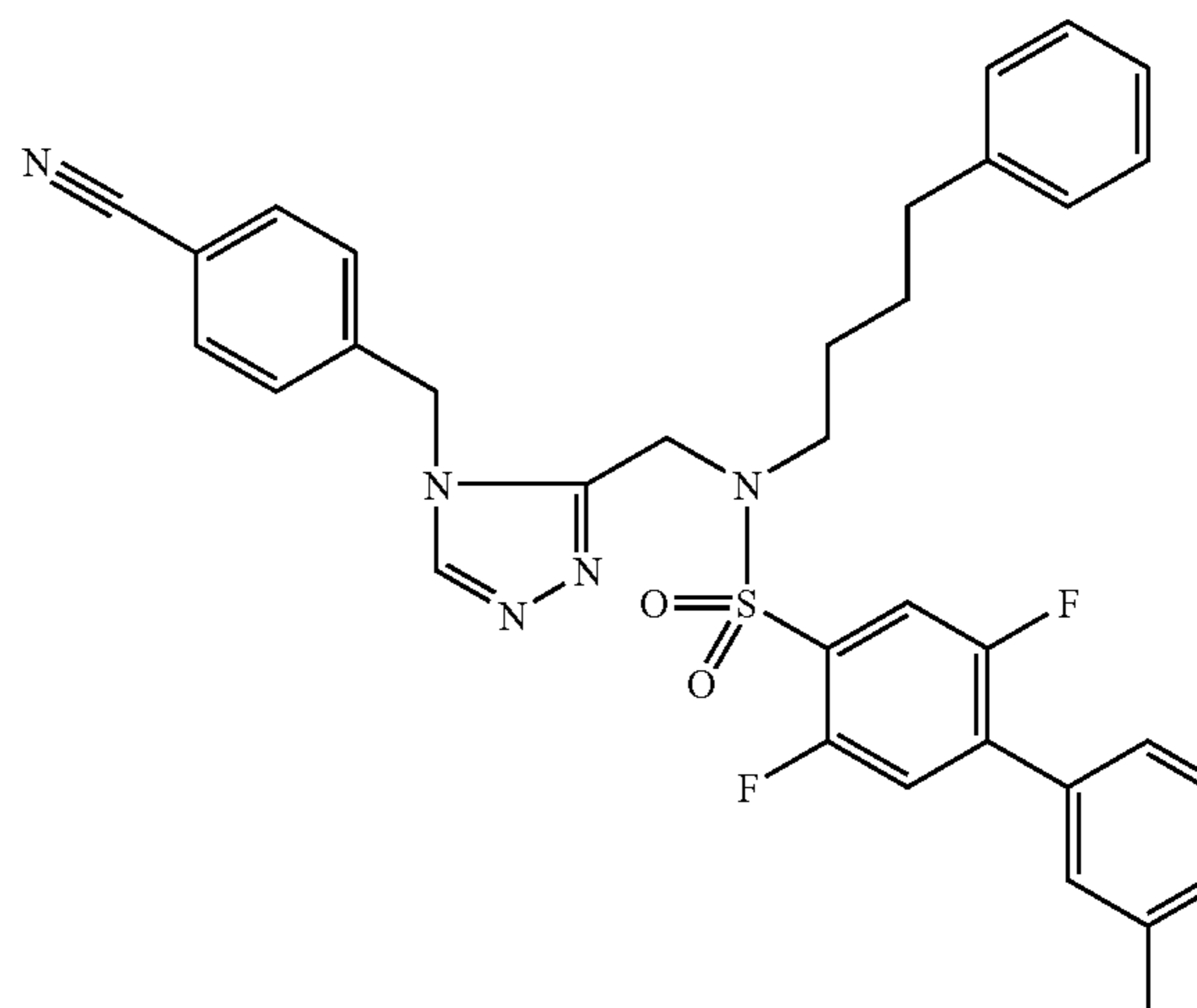
Trifluoroacetate (1:1) comp. 203.
