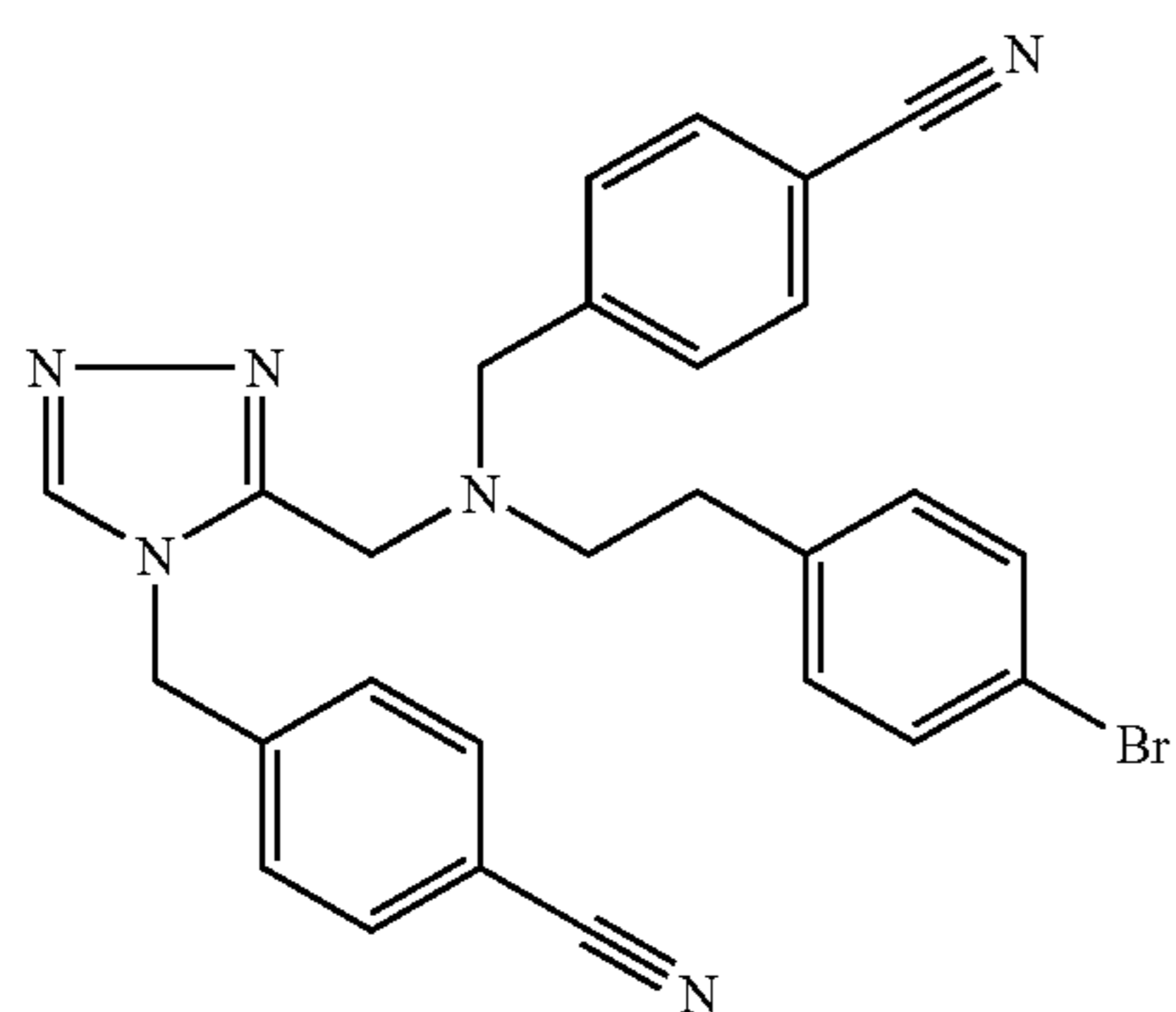
Trifluoroacetate (1:1) comp. 108.
