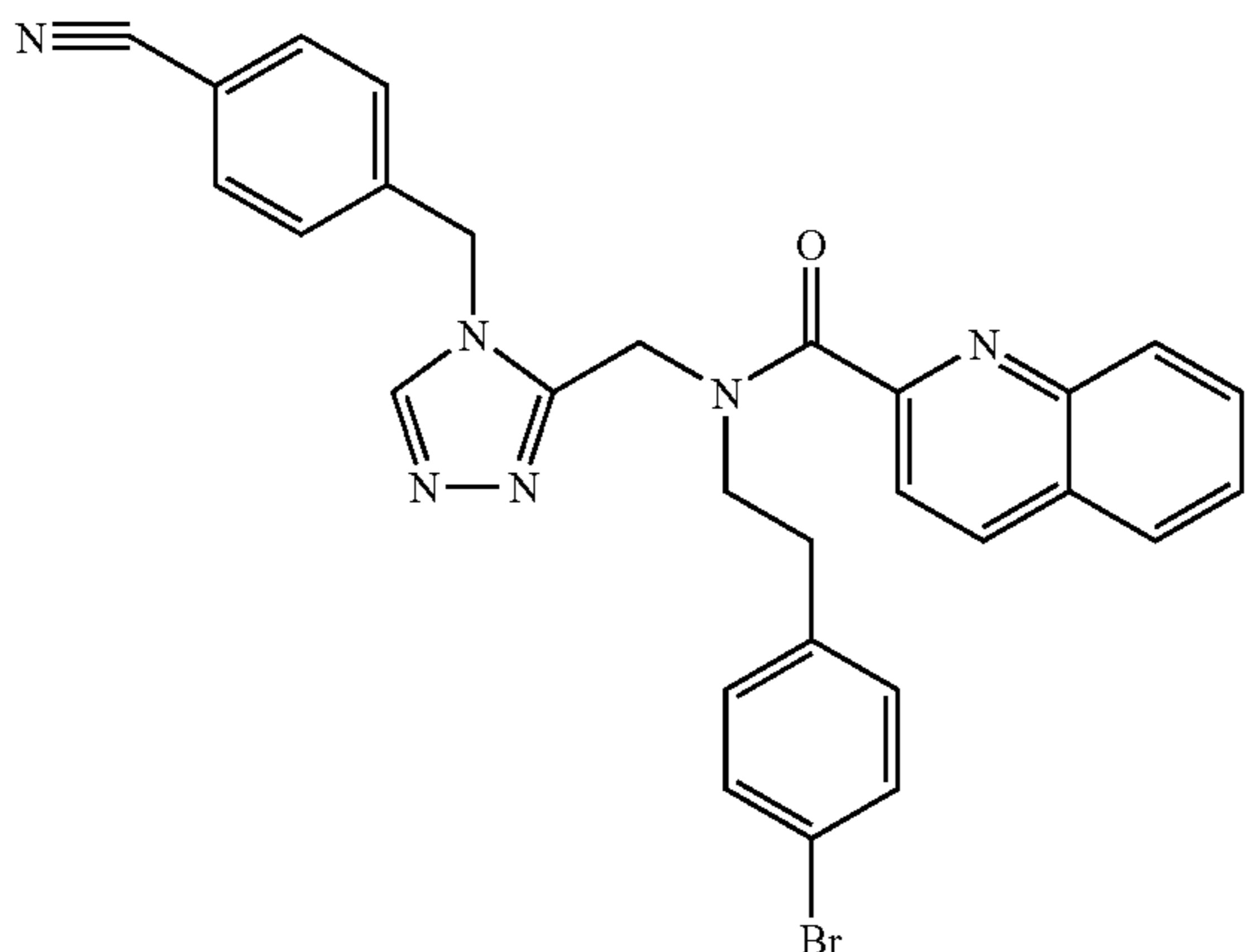
Trifluoroacetate (1:1) comp. 269.
