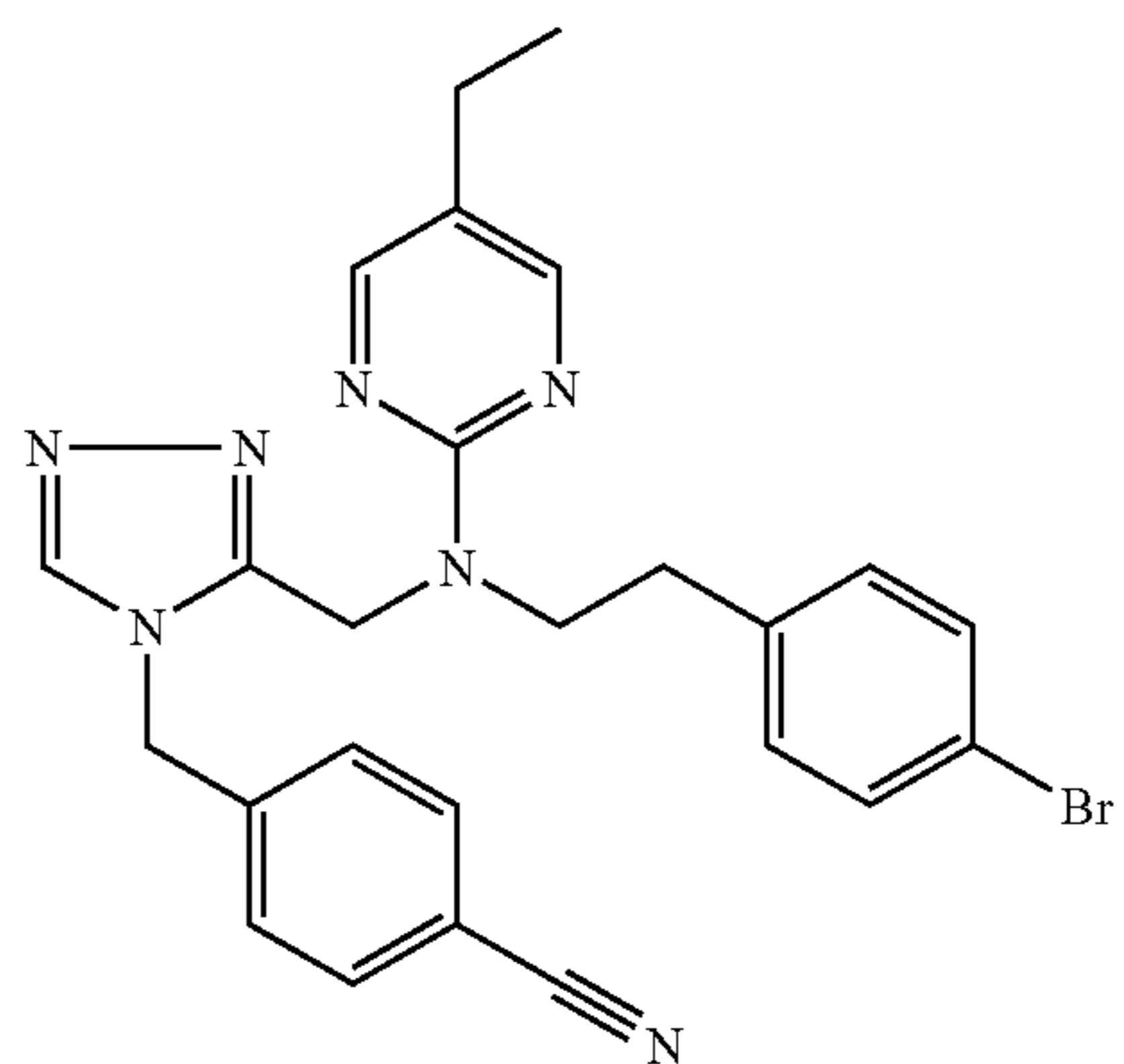
Trifluoroacetate (1:1) comp. 164.
