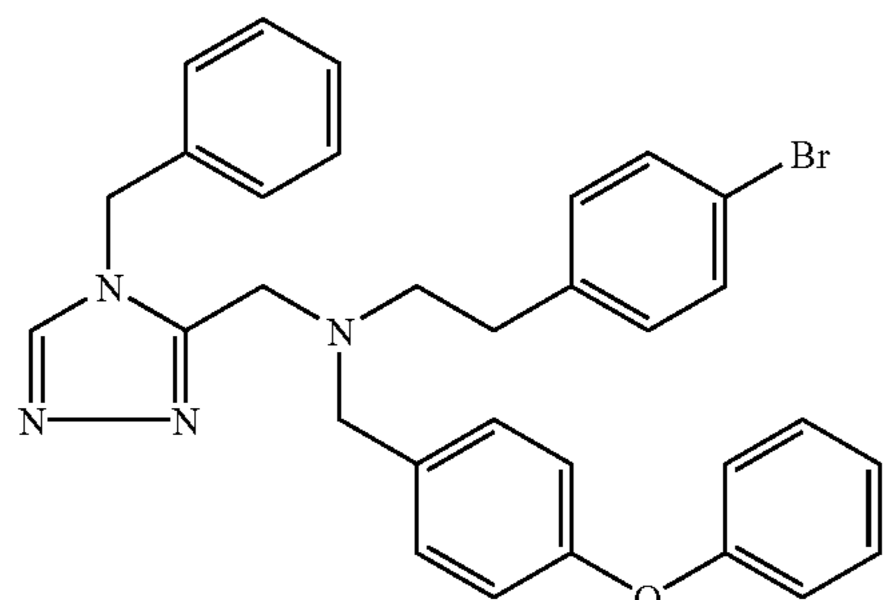
Trifluoroacetate (1:1) comp. 8.
