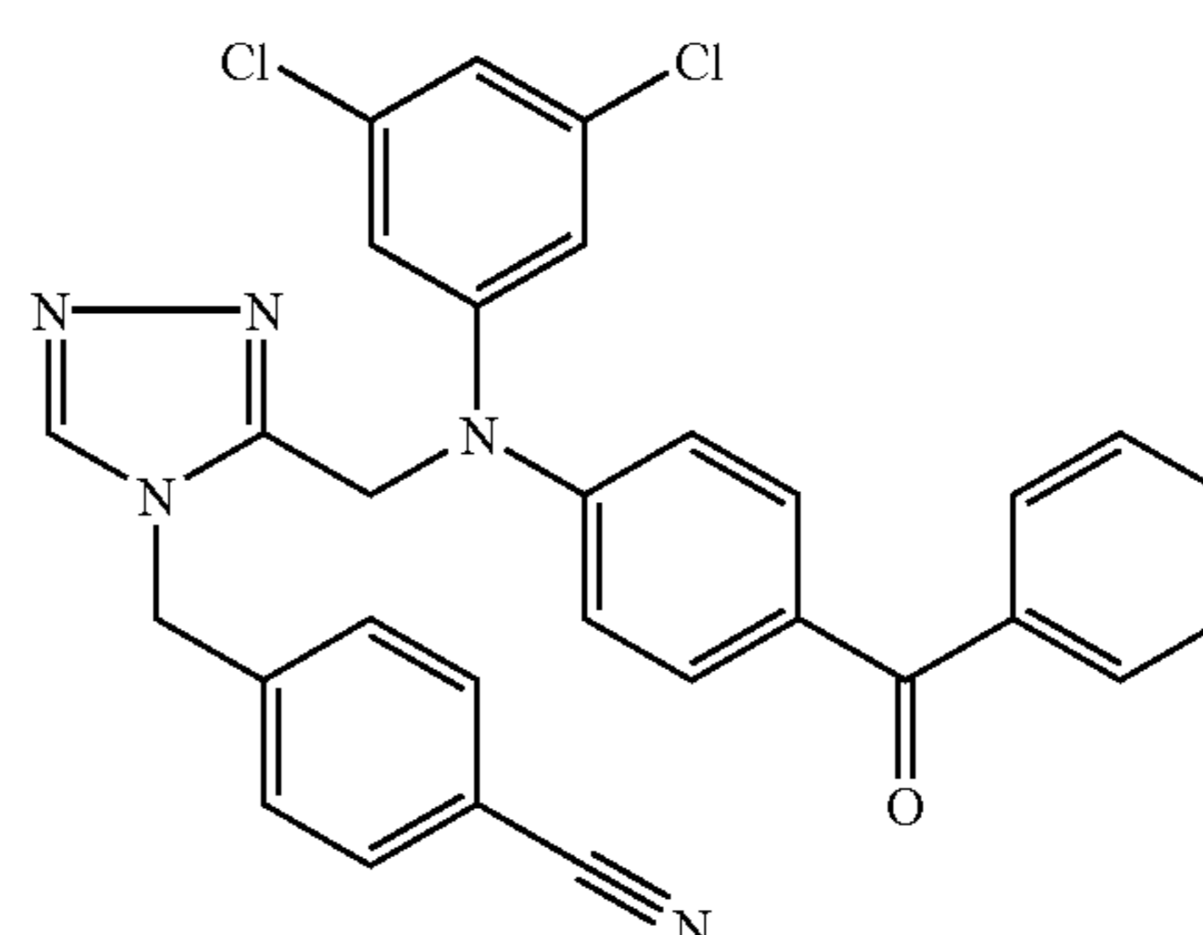
Trifluoroacetate (1:1) comp. 77.
