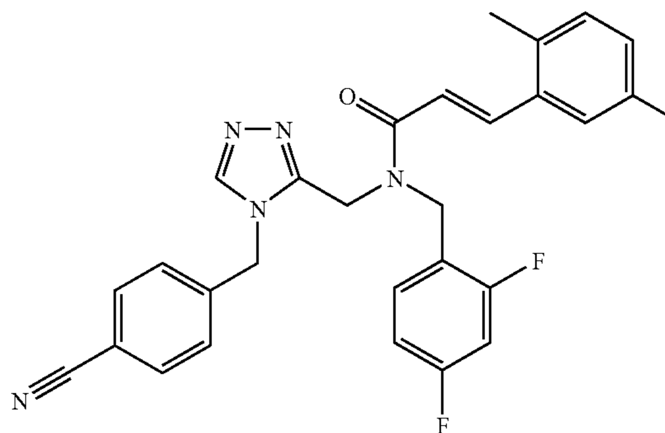
Trifluoroacetate (1:1) comp. 225.
