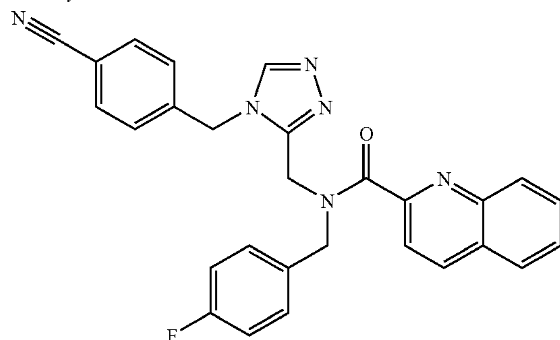
2-Quinolinecarboxamide, N-[[4-[(4-cyanophenyl)methyl]-4H-1,2,4-triazol-3-yl]methyl]-N-[(4-fluorophenyl)methyl]-
