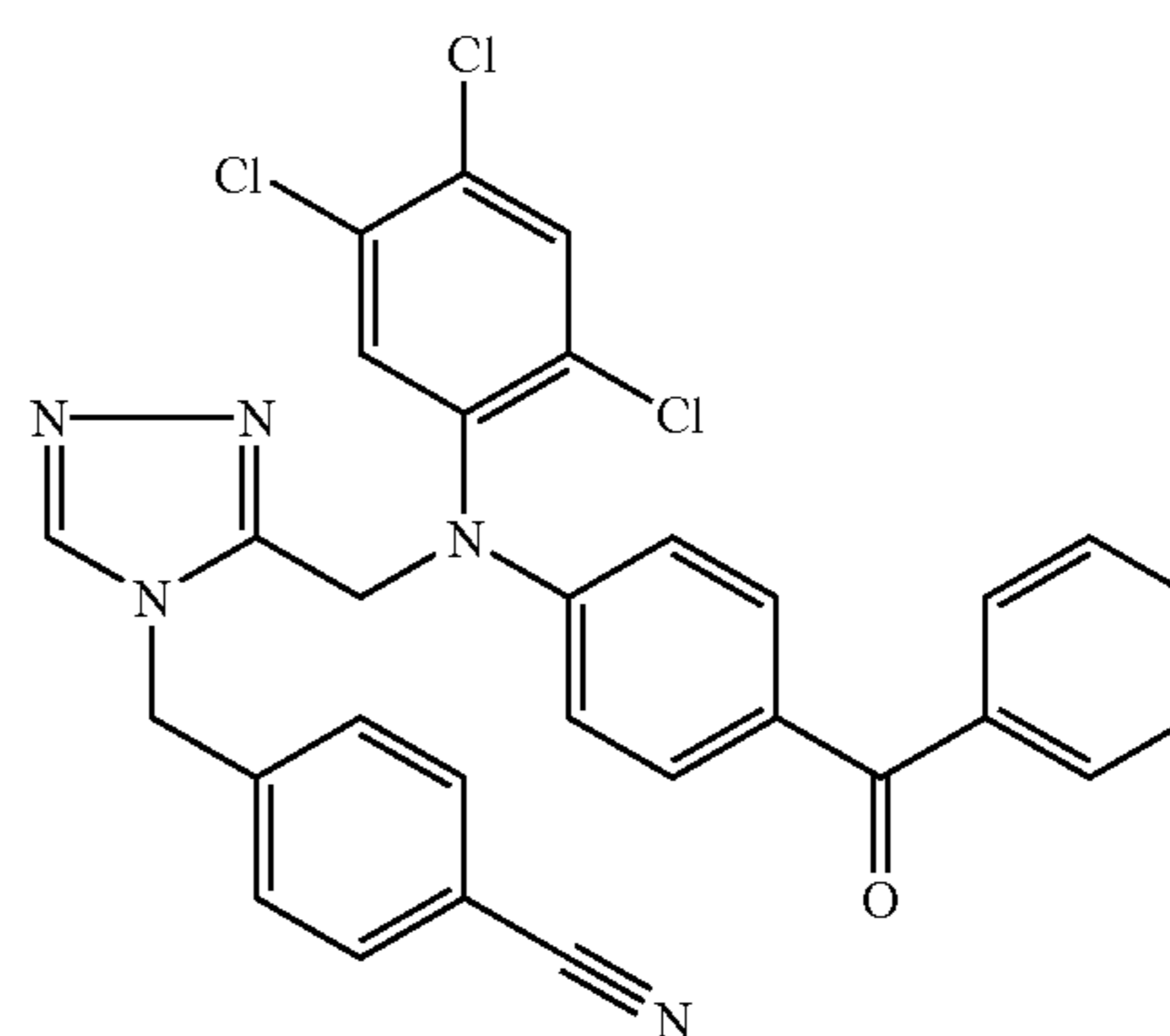
Trifluoroacetate (1:1) comp. 78.
