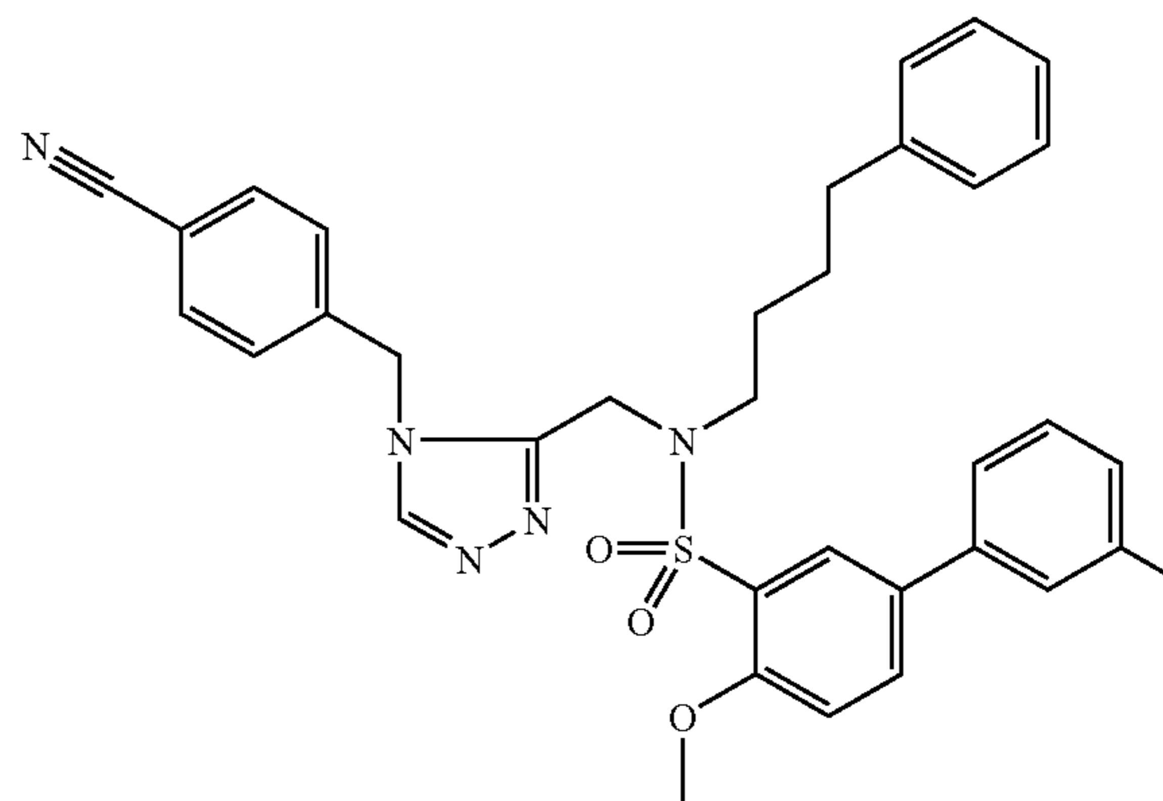
Trifluoroacetate (1:1) comp. 202.
