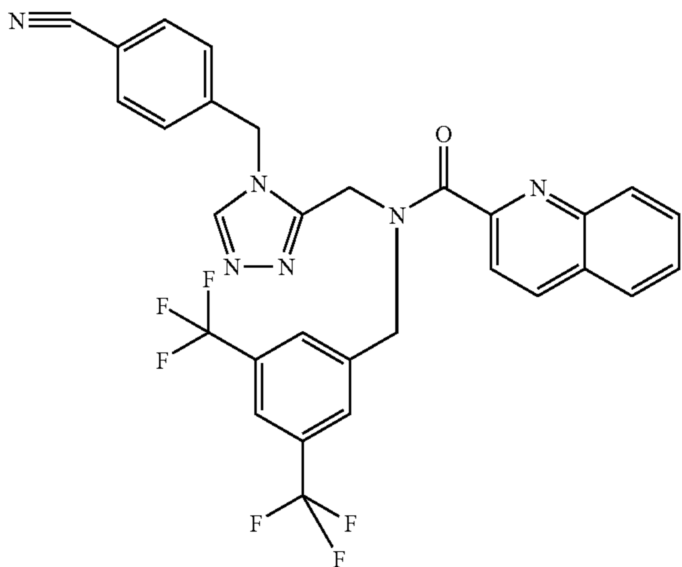
Trifluoroacetate (1:1) comp. 226.
