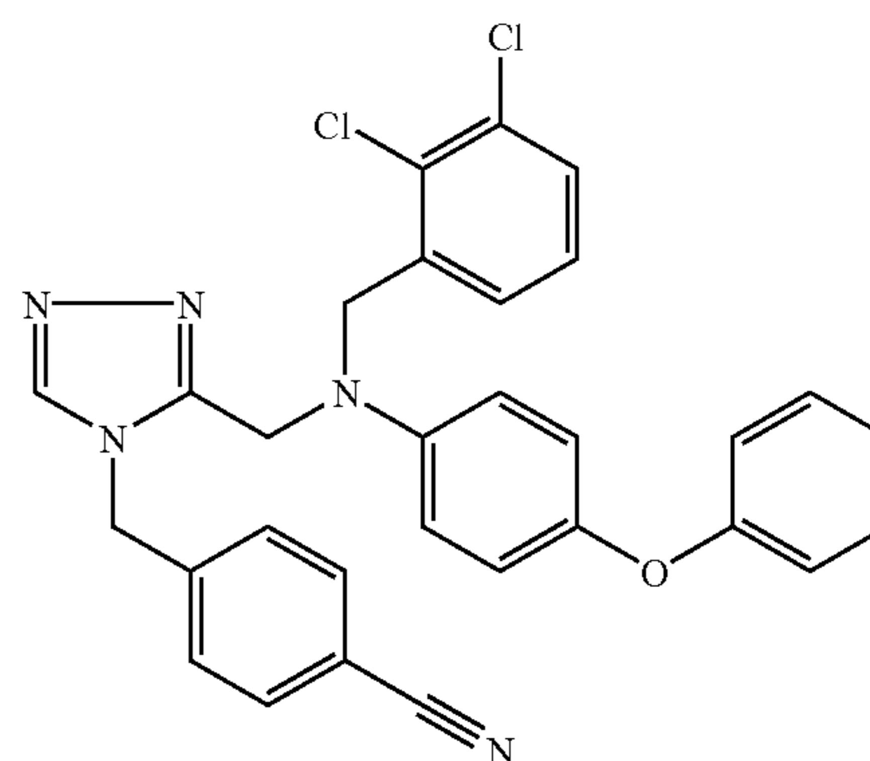
Trifluoroacetate (1:1) comp. 53.
