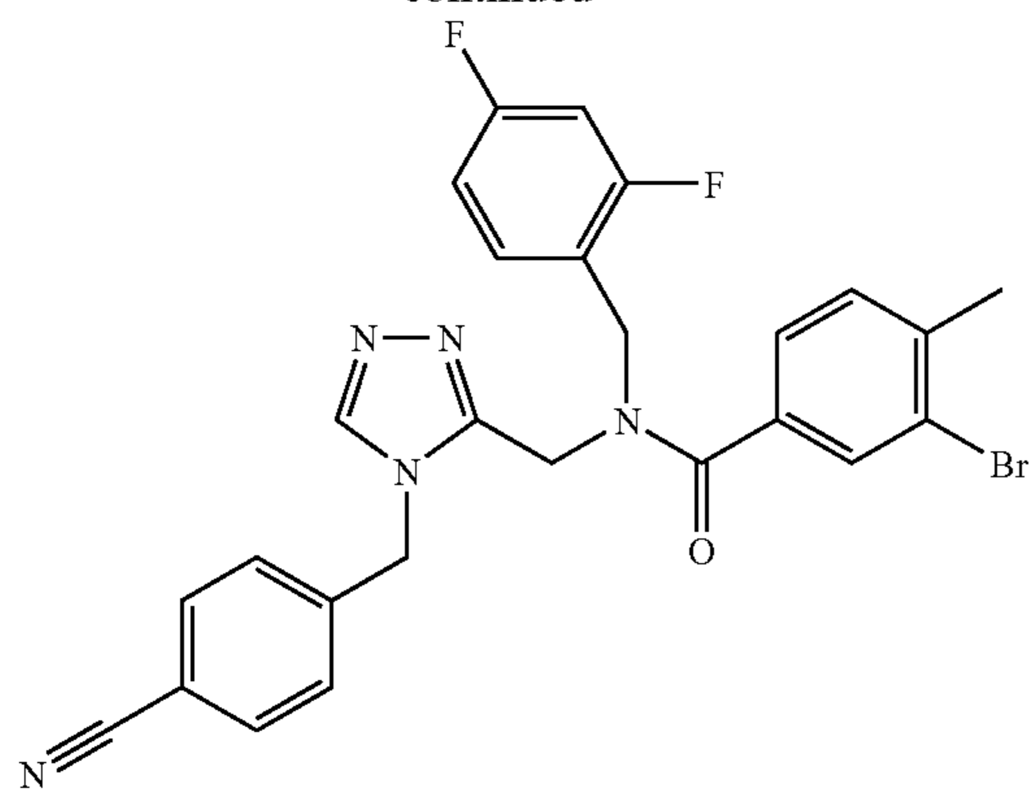
Trifluoroacetate (1:1) comp. 309.
