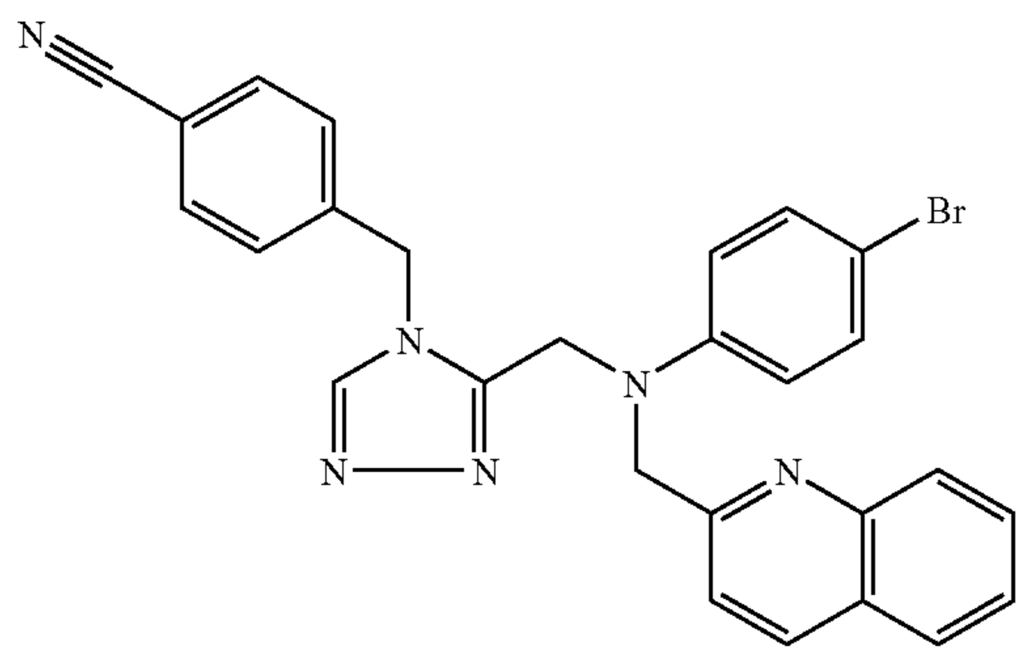
Trifluoroacetate (1:1) comp. 137.
