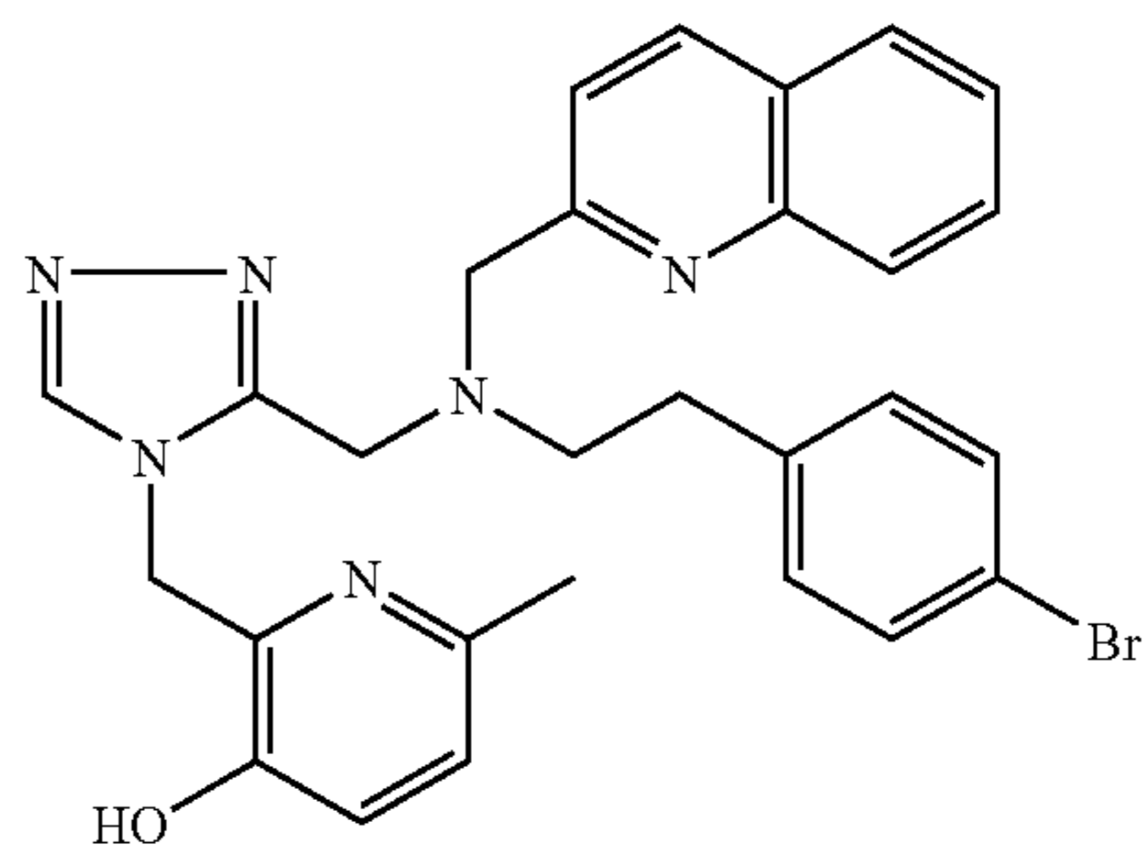
Trifluoroacetate (1:1) comp. 177.
