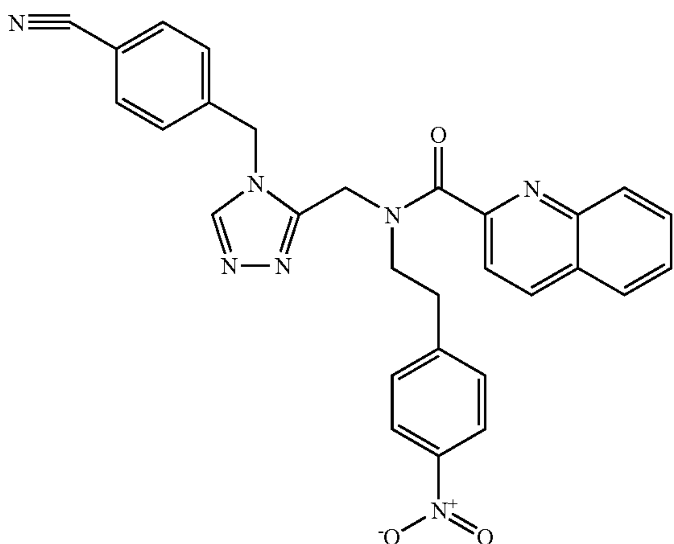
Trifluoroacetate (1:1) comp. 263.
