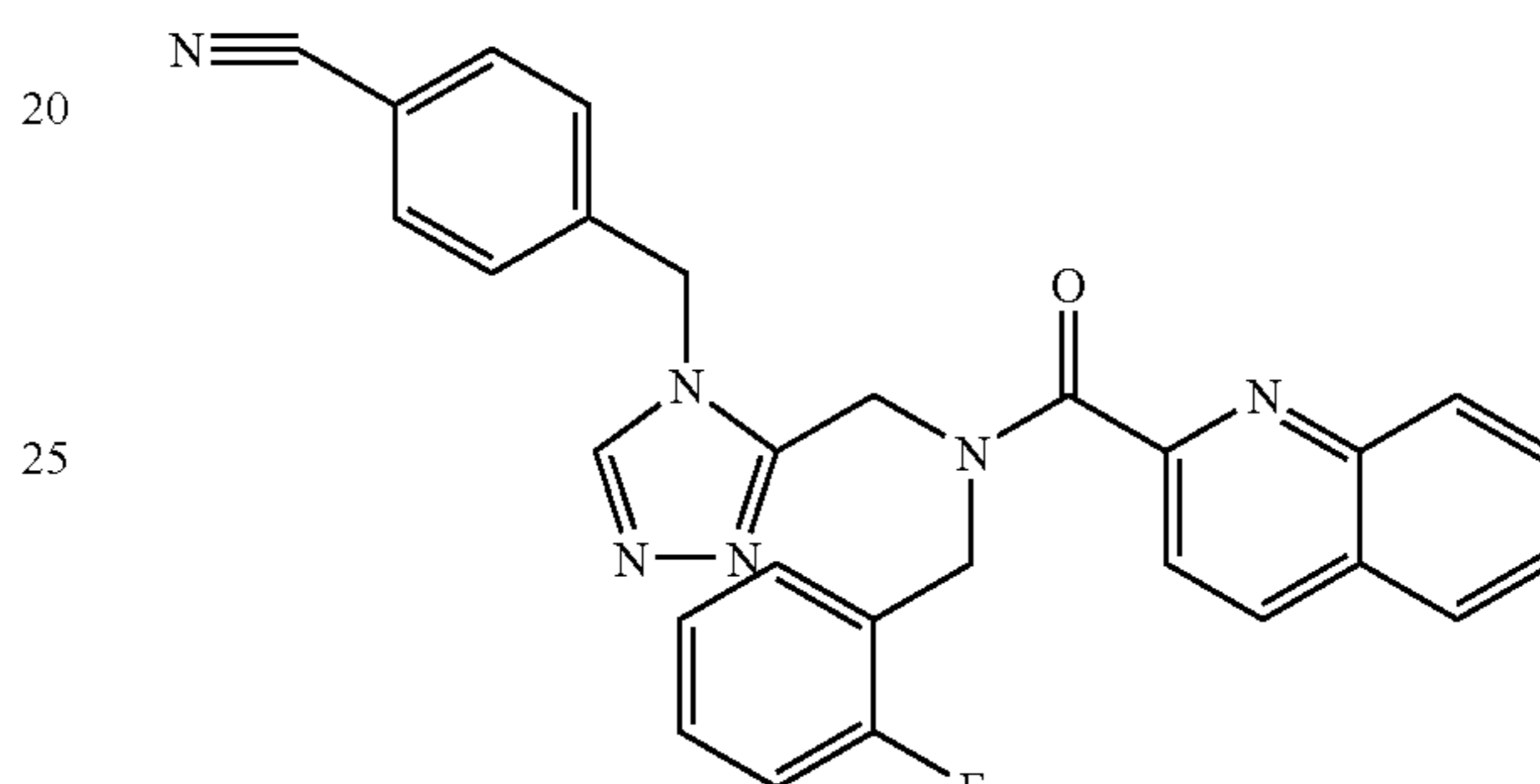
Trifluoroacetate (1:1) comp. 306.
