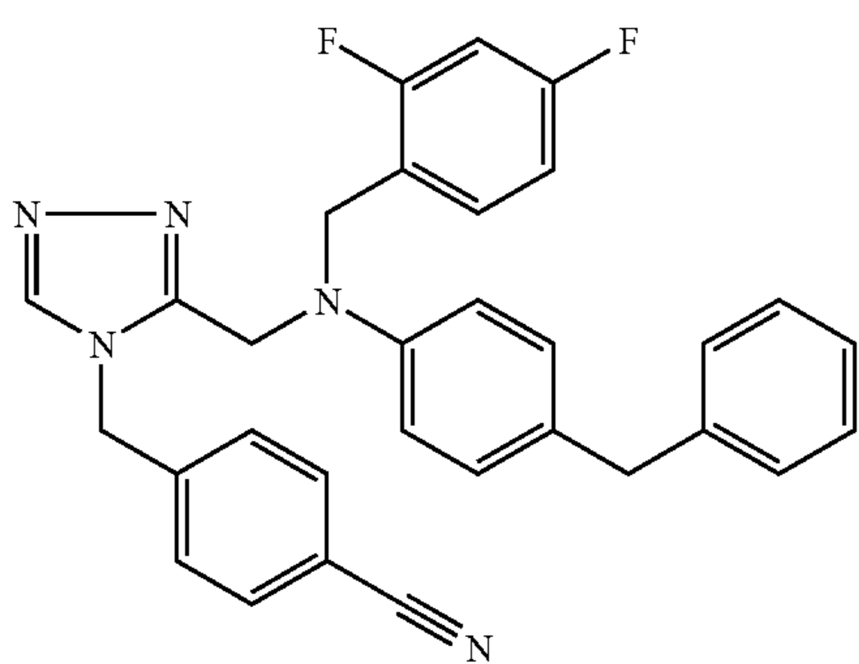
Trifluoroacetate (1:1) comp. 82.
