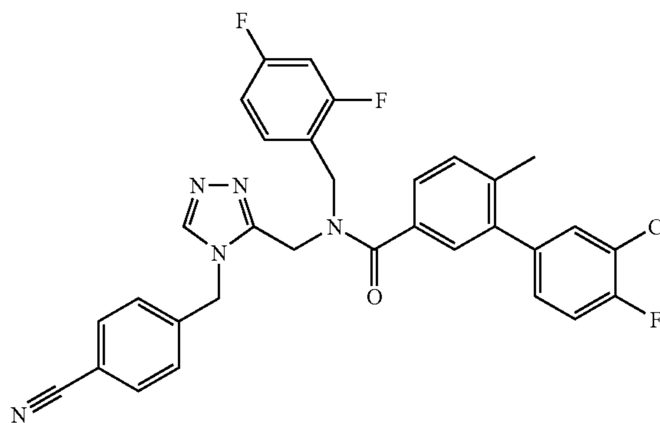
Trifluoroacetate (1:1) comp. 224.
