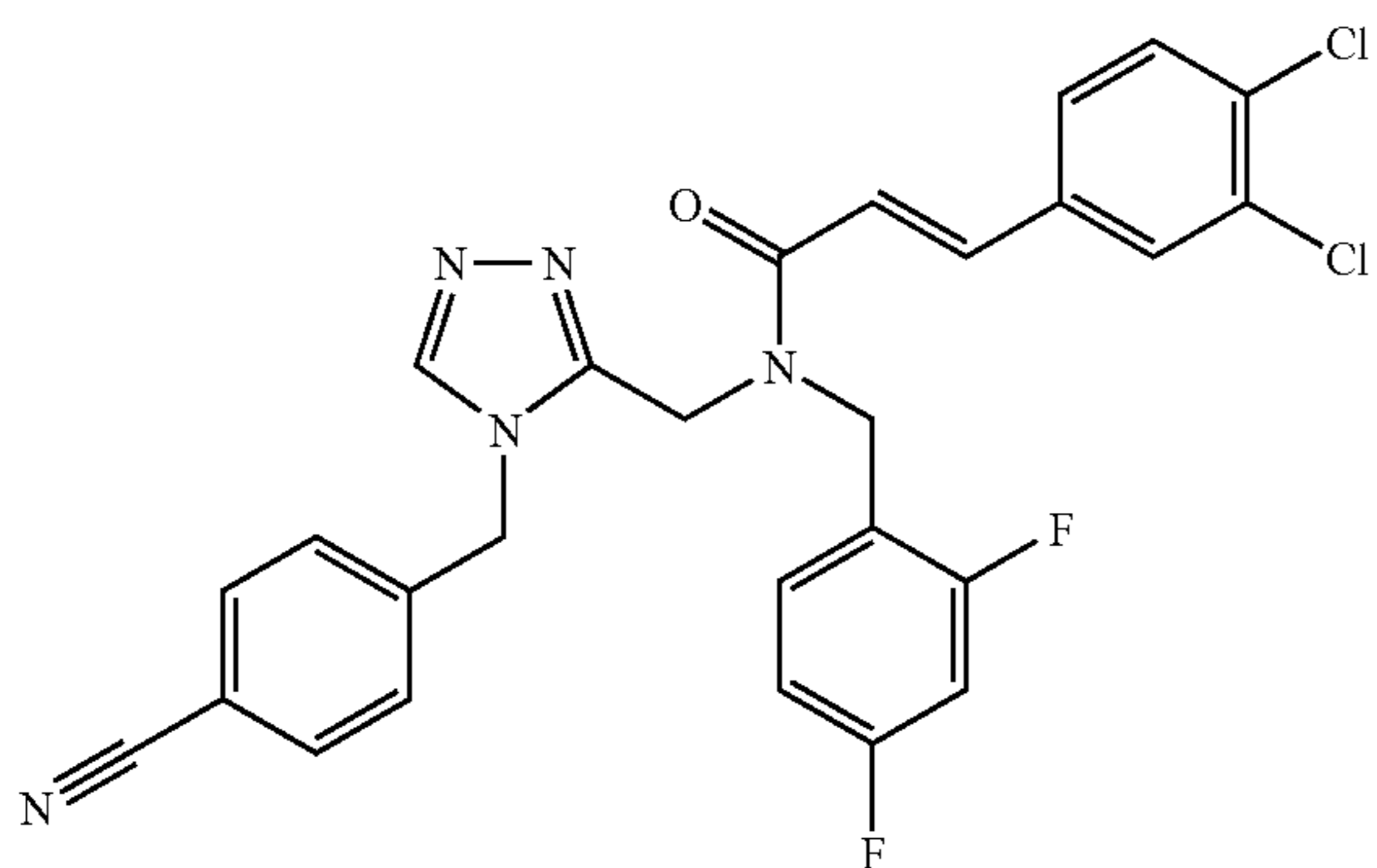
Trifluoroacetate (1:1) comp. 250.
