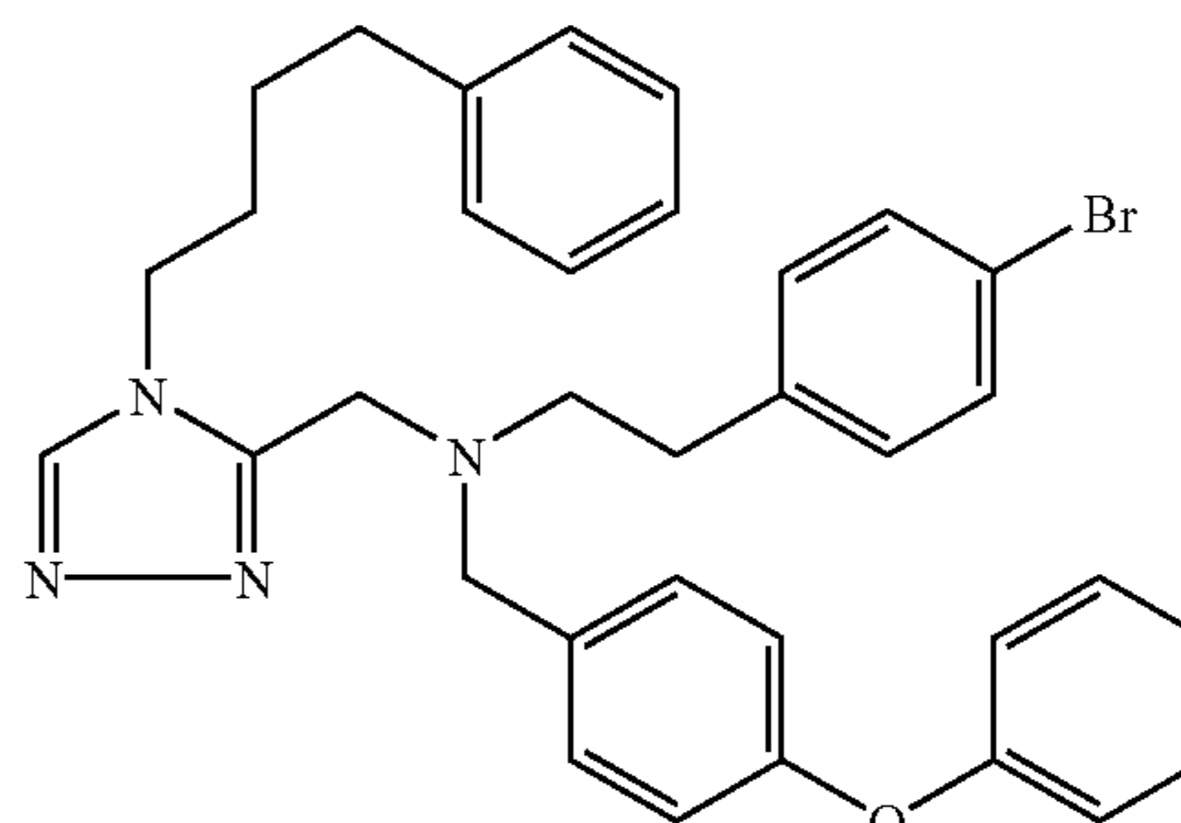
Trifluoroacetate (1:1) comp. 13.
