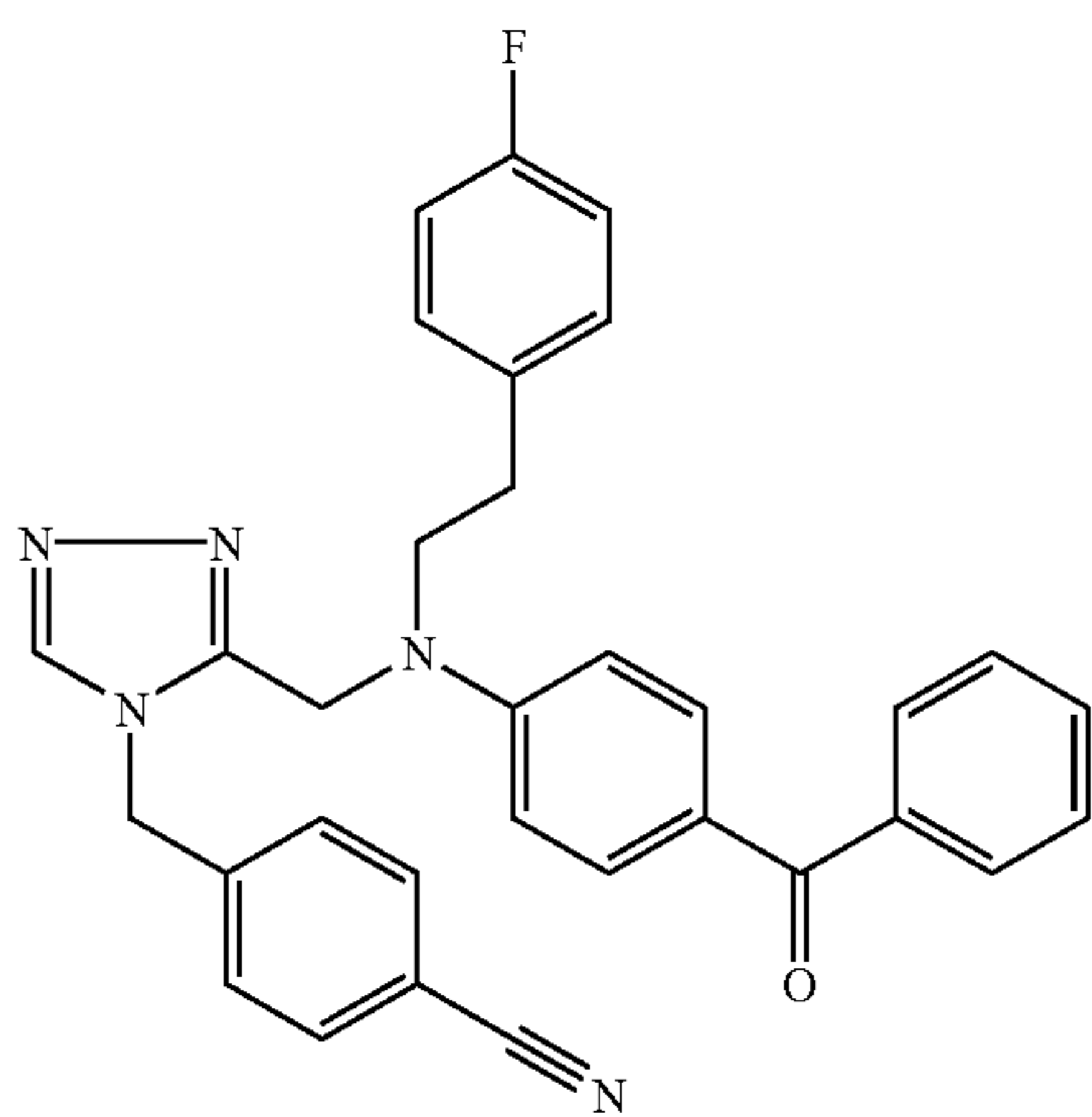
Trifluoroacetate (1:1) comp. 80.
