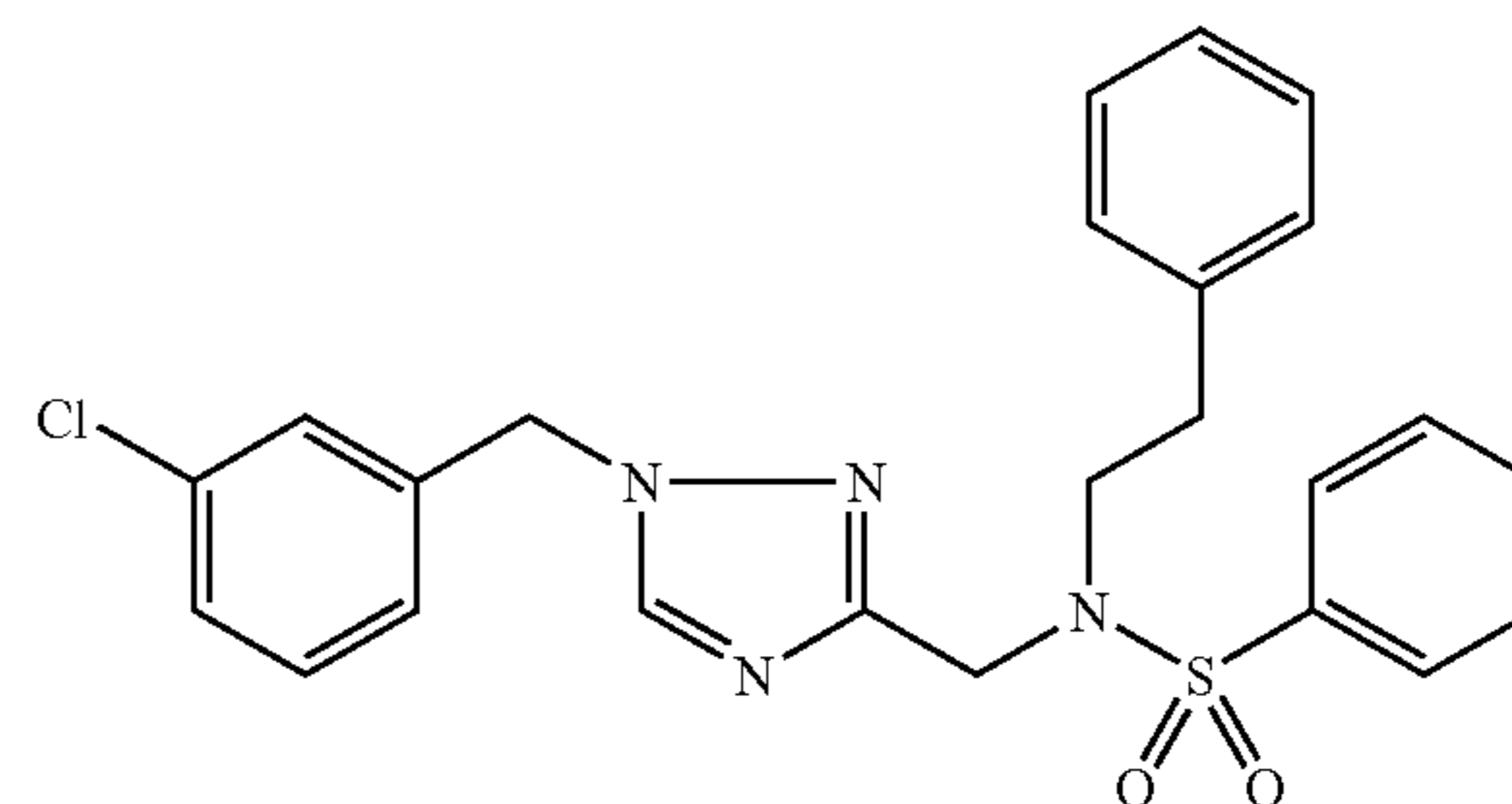
Trifluoroacetate (1:1) comp. 1.
