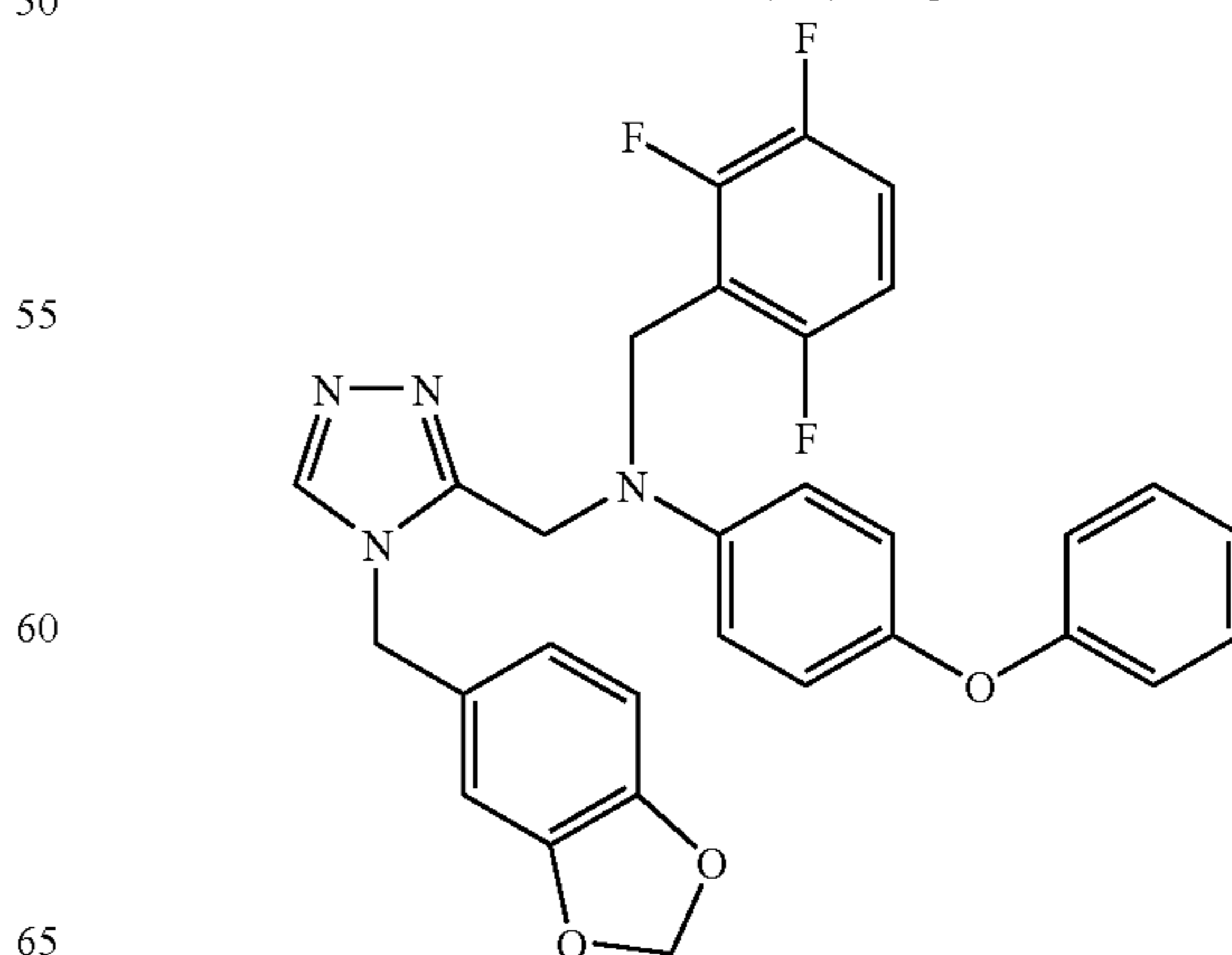
Trifluoroacetate (1:1) comp. 217.
