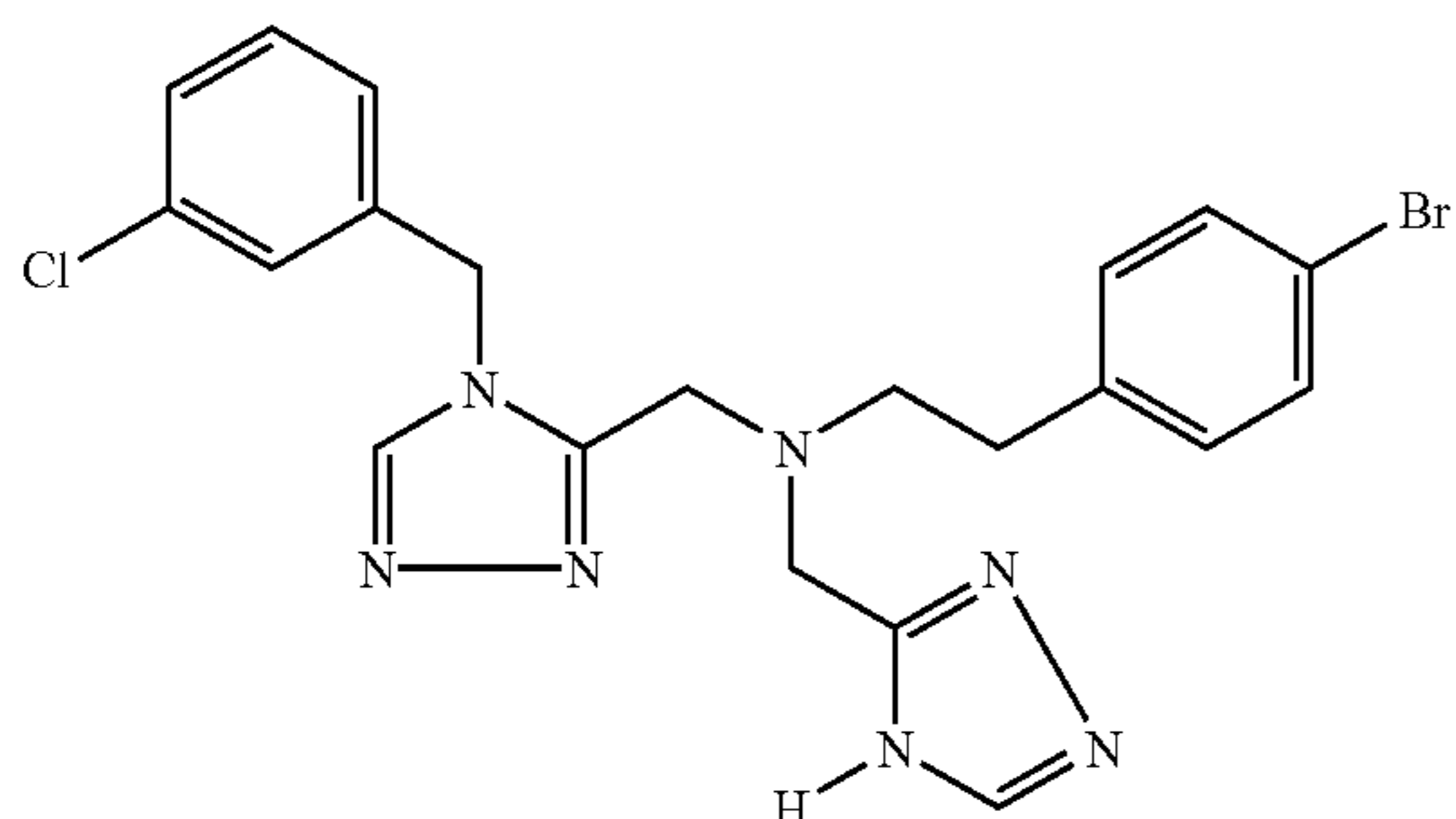
Trifluoroacetate (1:1) comp. 30.
