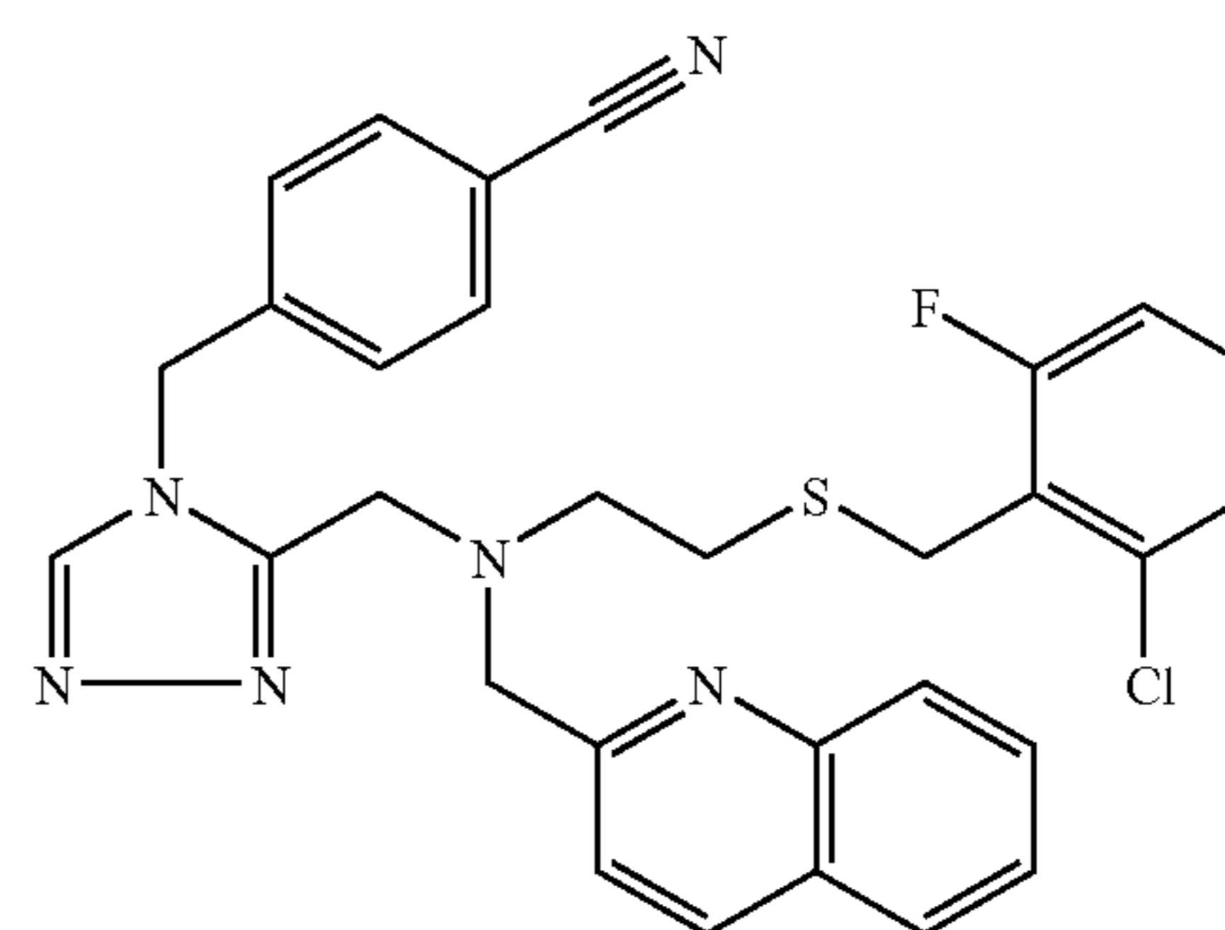
Trifluoroacetate (1:1) comp. 111.
