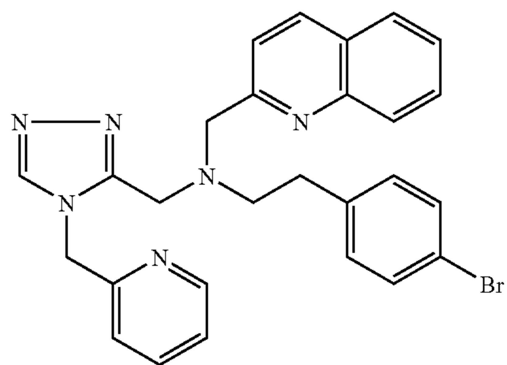
Trifluoroacetate (1:1) comp. 179.
