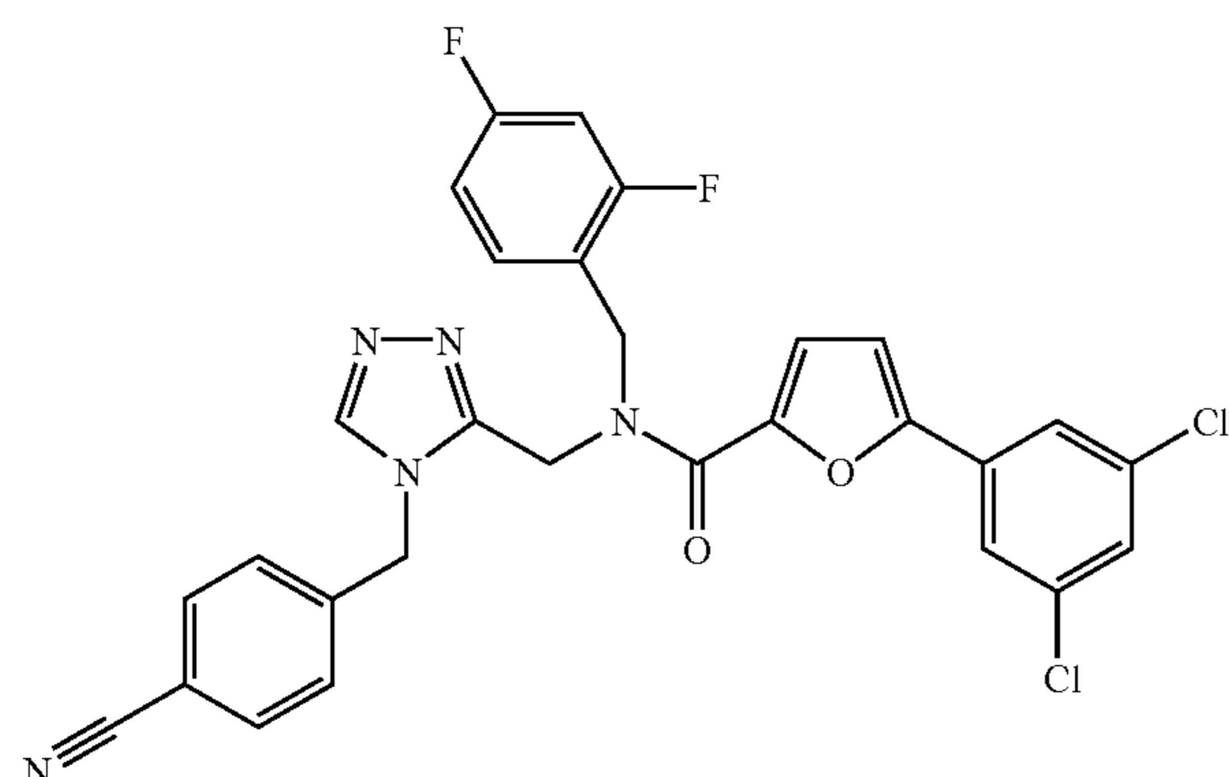
2-Furancarboxamide, N-[[4-[(4-cyanophenyl)methyl]-4H-1,2,4-triazol-3-yl]methyl]-5-(3,5-dichlorophenyl)-N-[(2,4-difluorophenyl)methyl]-
