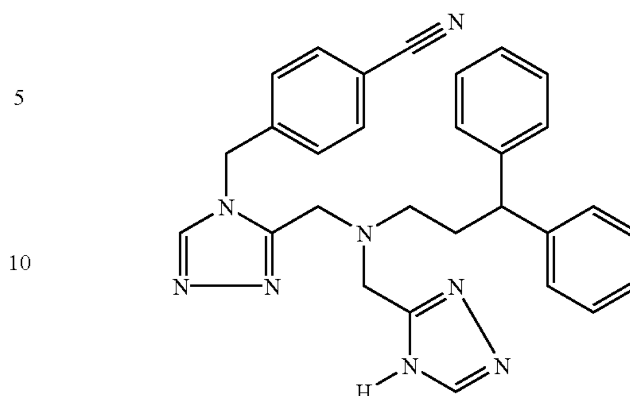
Trifluoroacetate (1:1) comp. 24.
