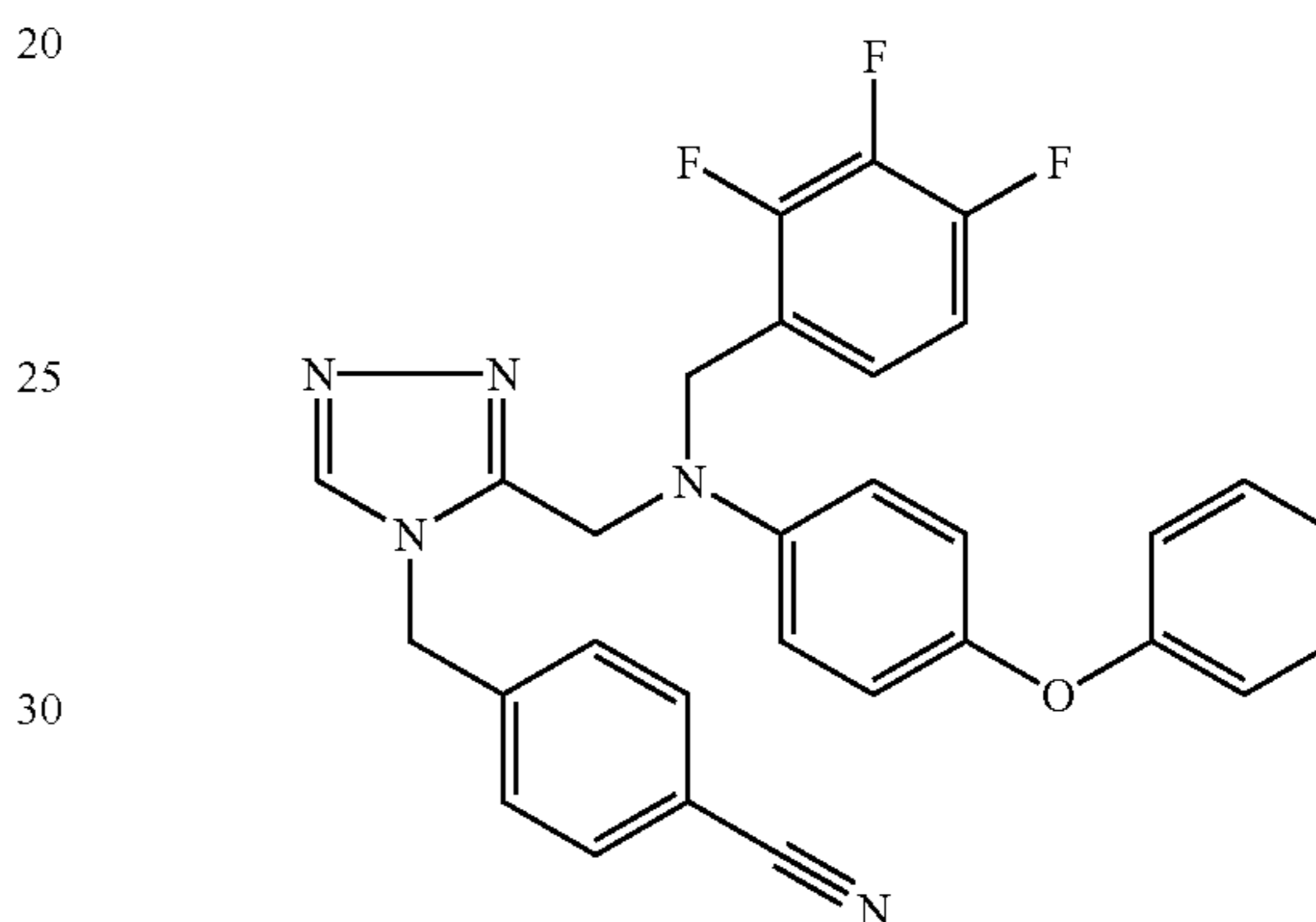
Trifluoroacetate (1:1) comp. 61.
