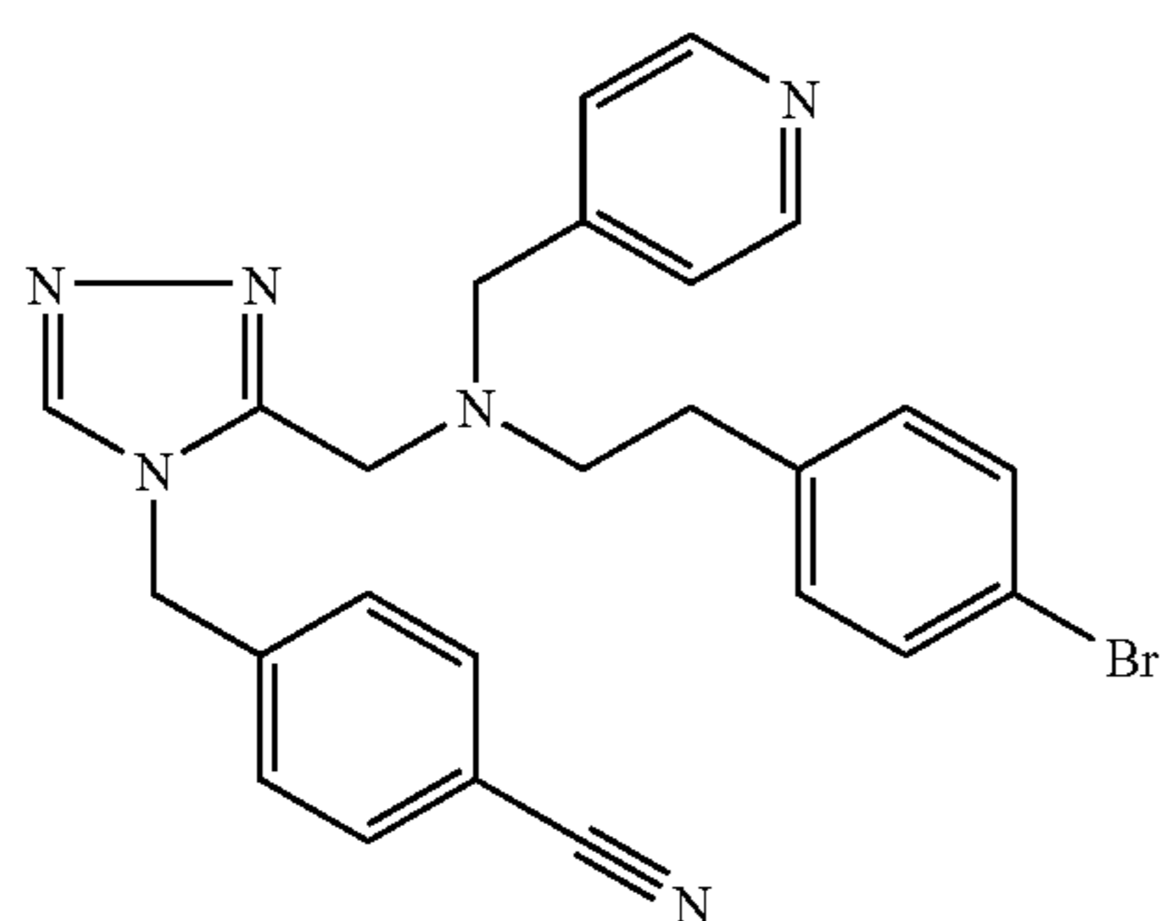
Trifluoroacetate (1:1) comp. 106.
