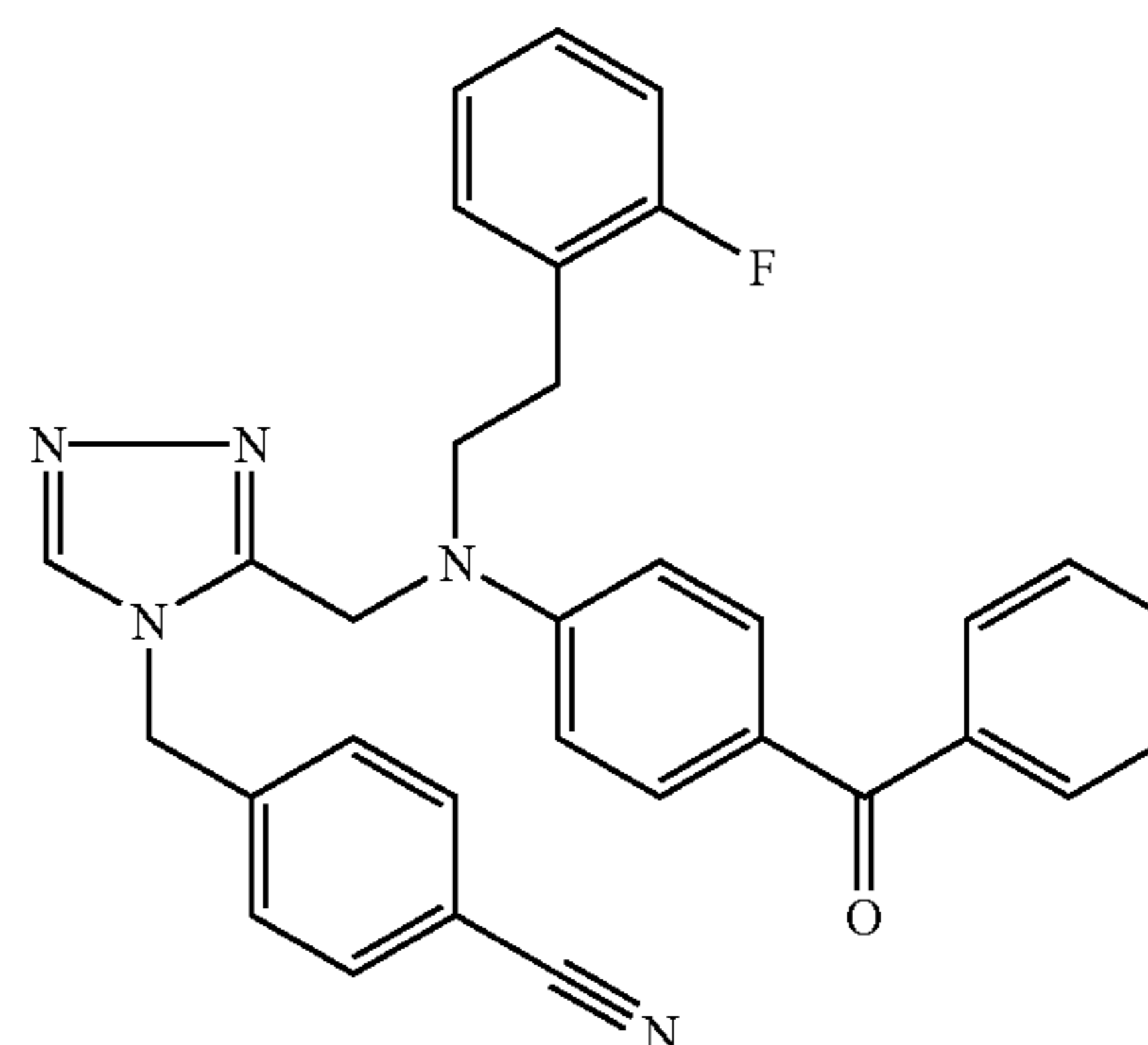
Trifluoroacetate (1:1) comp. 79.
