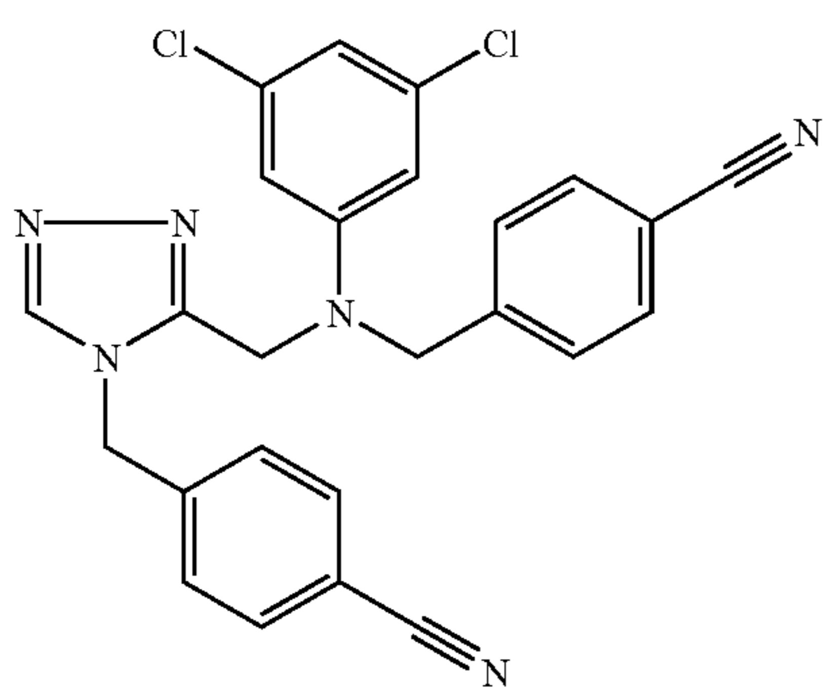
Trifluoroacetate (1:1) comp. 81.
