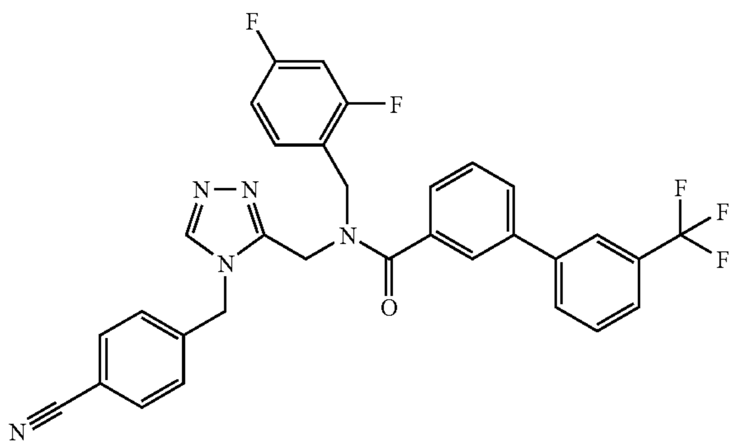
Trifluoroacetate (1:1) comp. 227.
