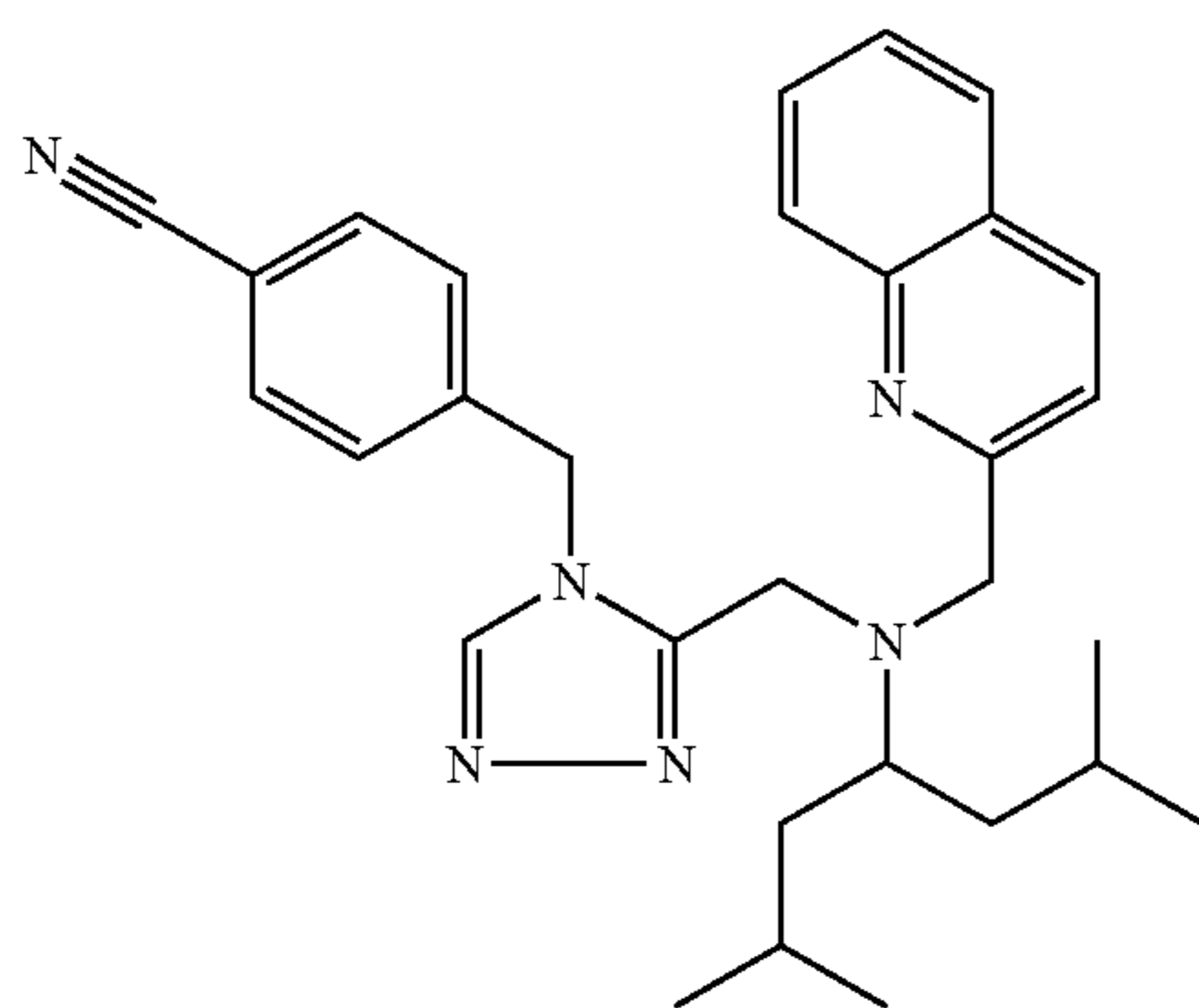
Trifluoroacetate (1:2) comp. 174.
