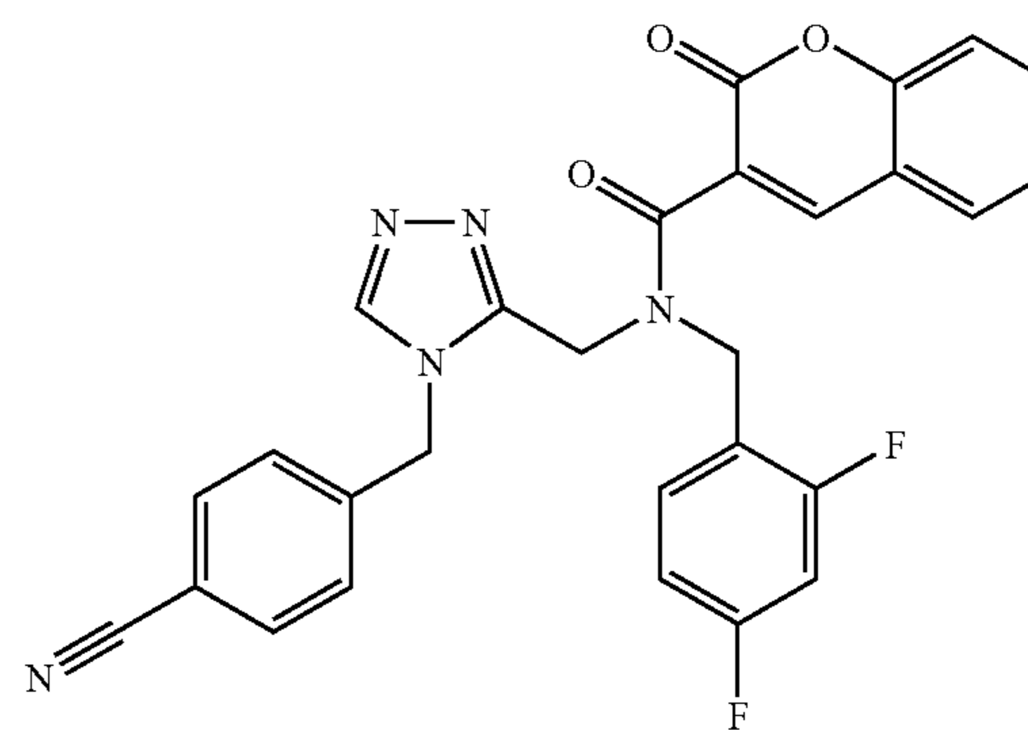
Trifluoroacetate (1:1) comp. 252.
