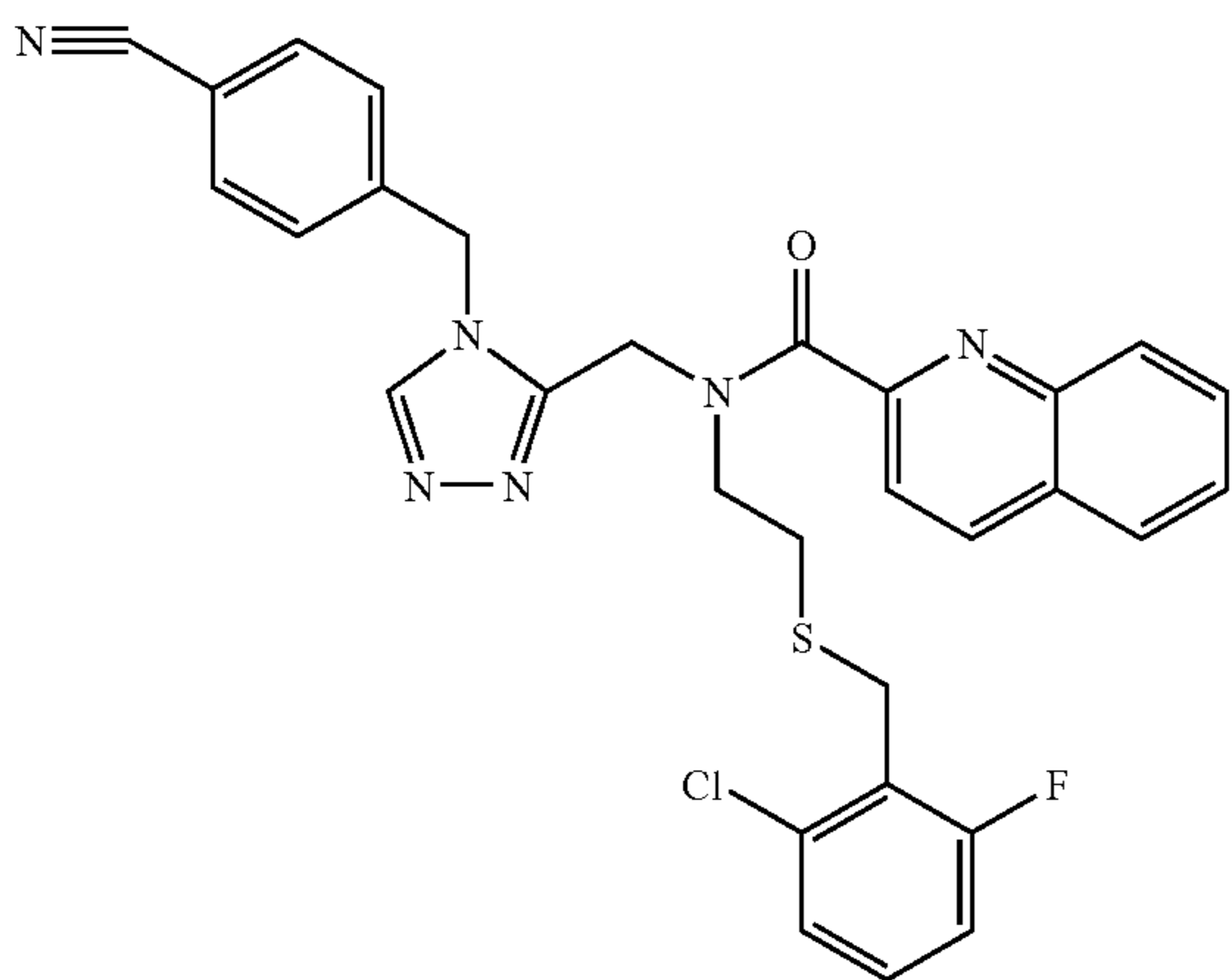
Trifluoroacetate (1:1) comp. 271.
