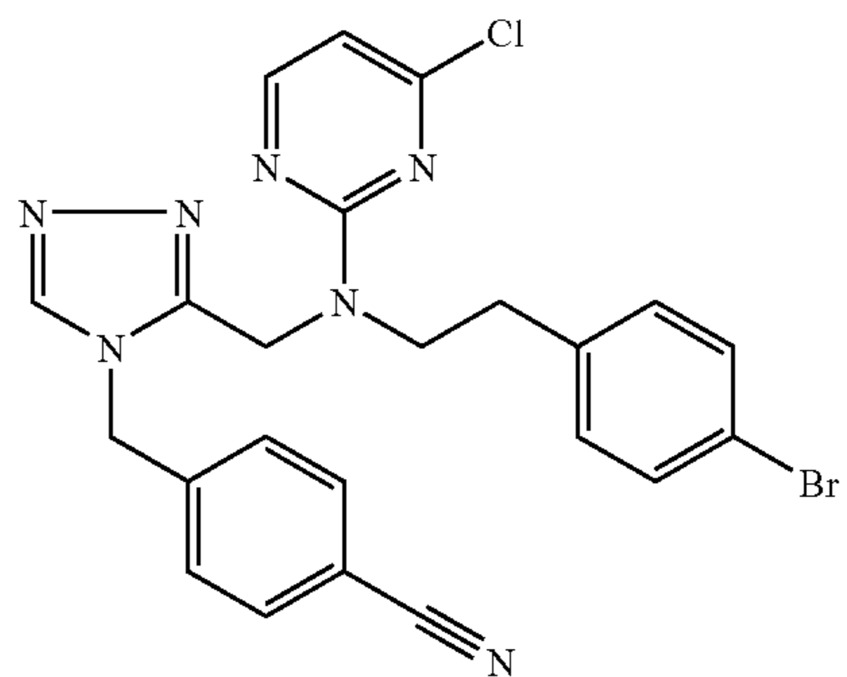
Trifluoroacetate (1:1) comp. 163.
