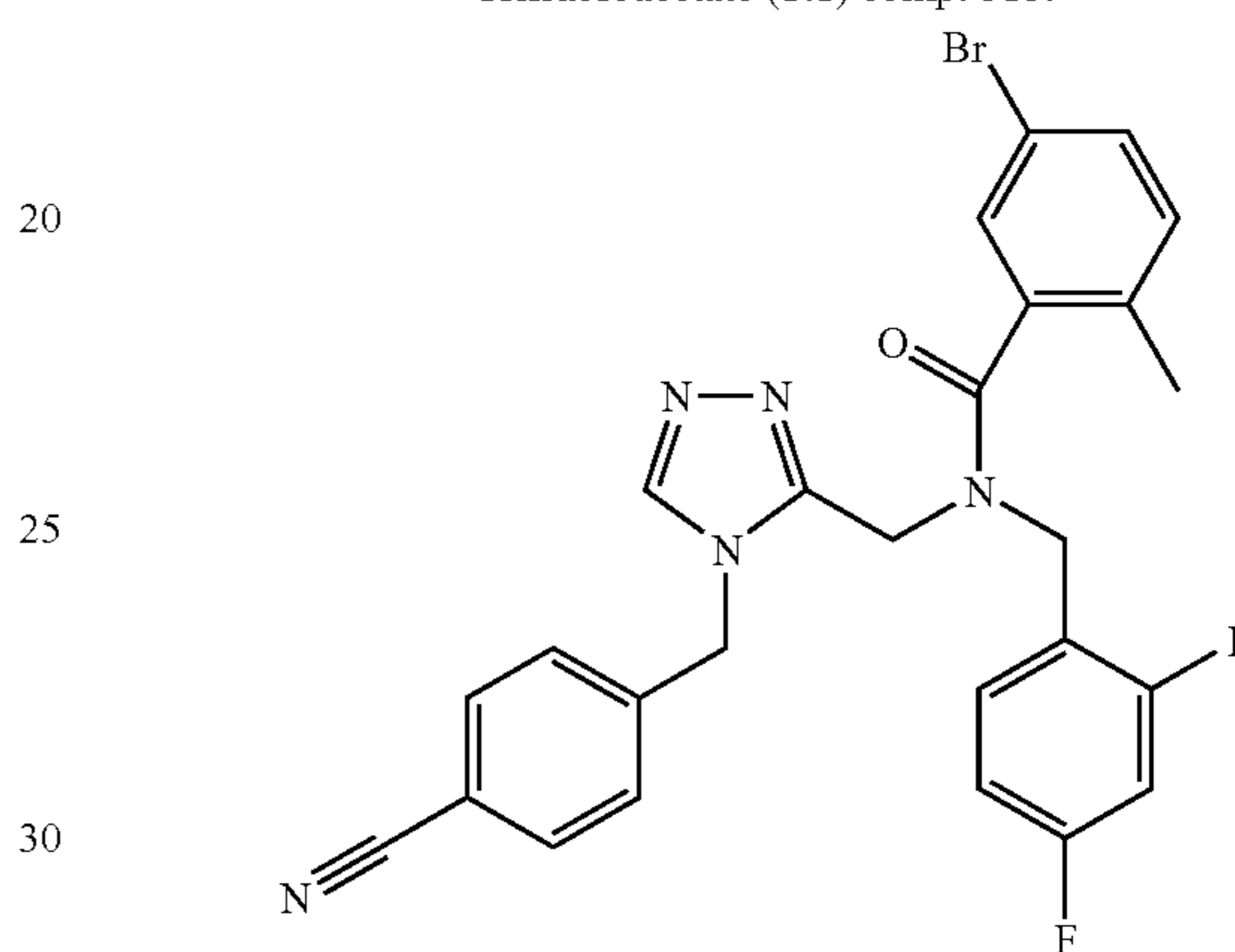
Trifluoroacetate (1:1) comp. 314.
