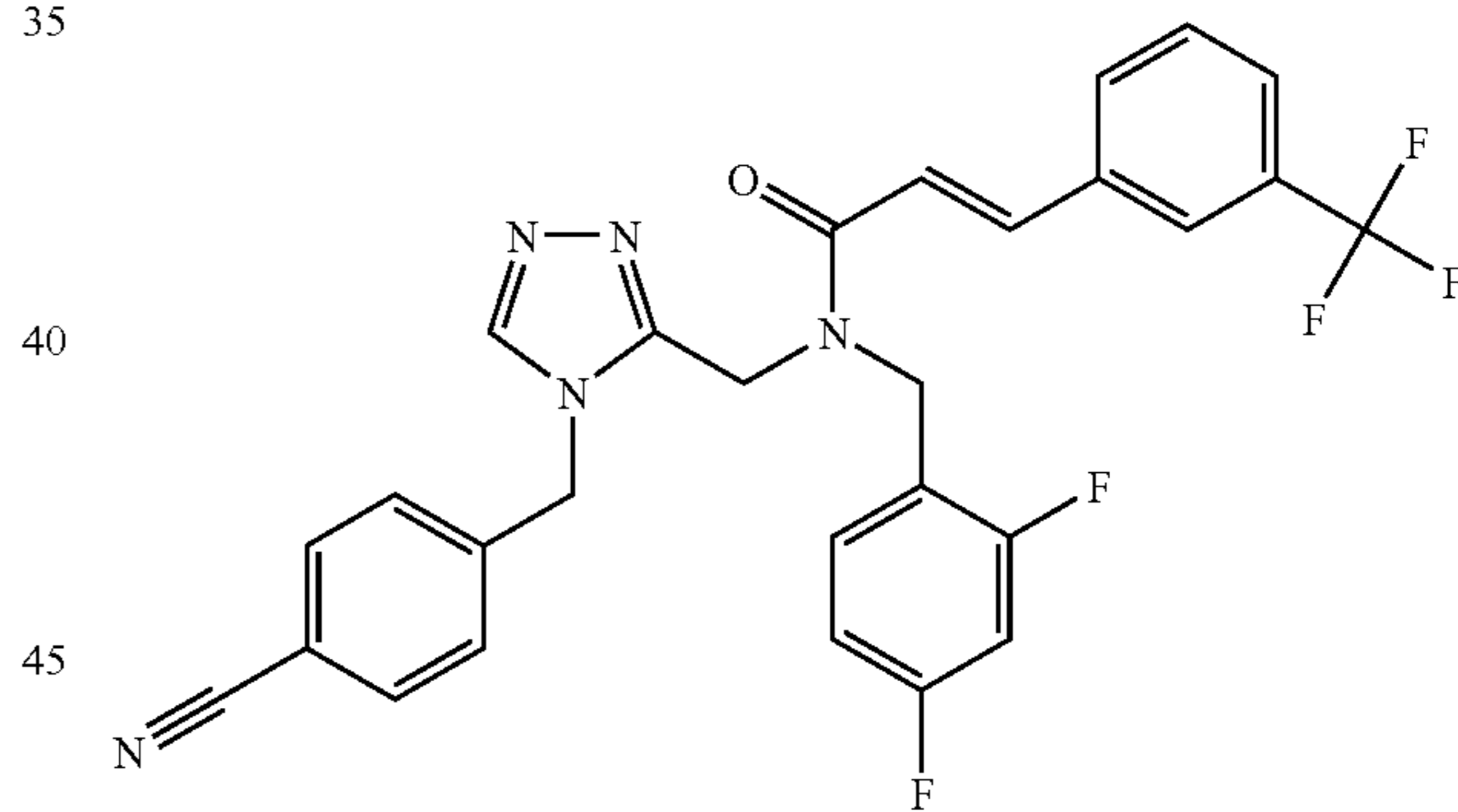
Trifluoroacetate (1:1) comp. 230.
