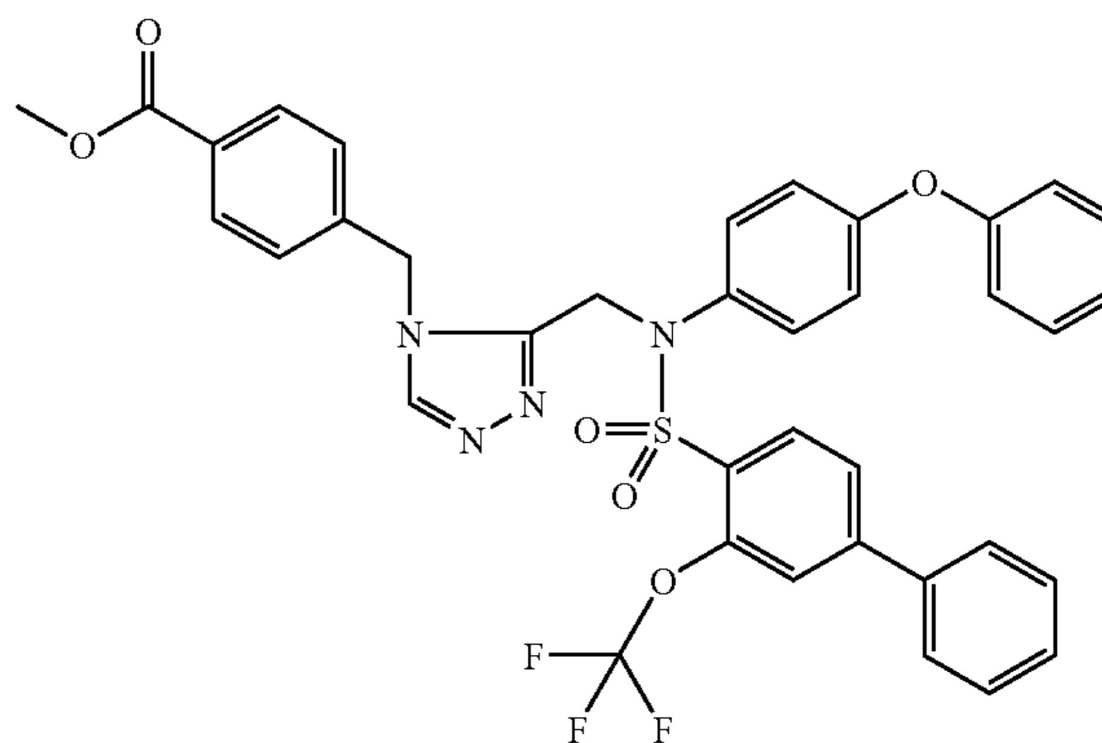
Trifluoroacetate (1:1) comp. 201.
