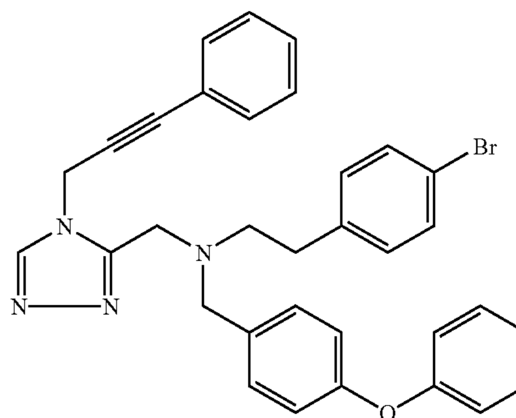
Trifluoroacetate (1:1) comp. 11.
