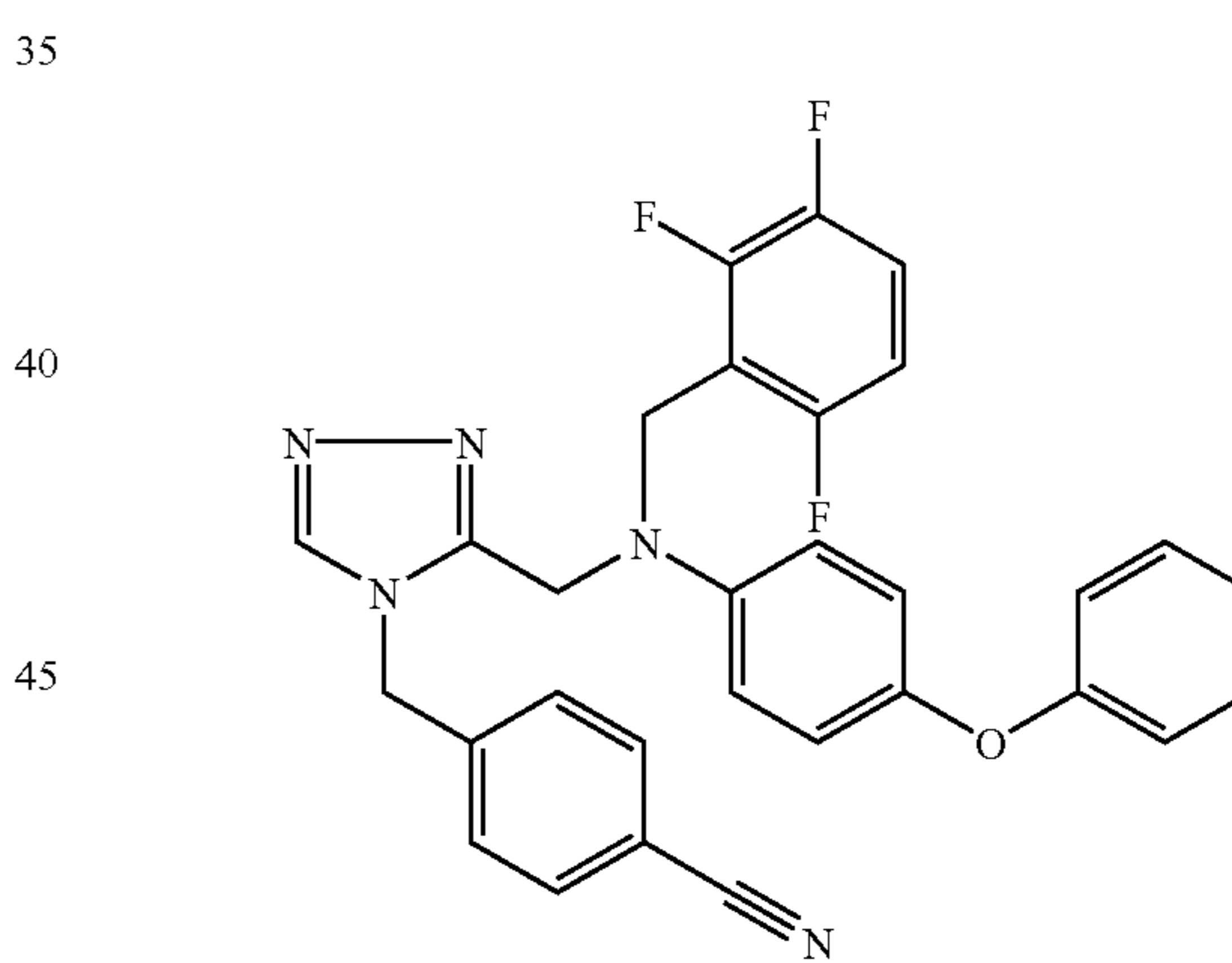
Trifluoroacetate (1:1) comp. 62.
