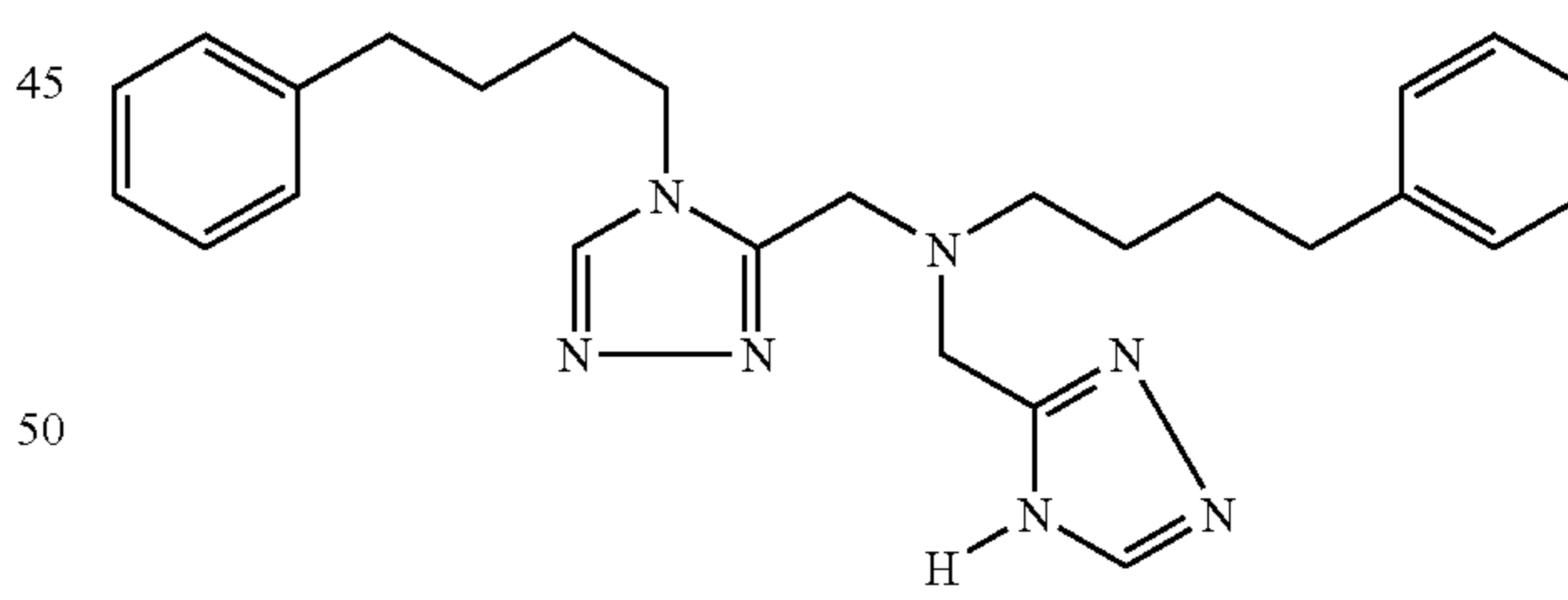
Trifluoroacetate (1:1) comp. 37.
