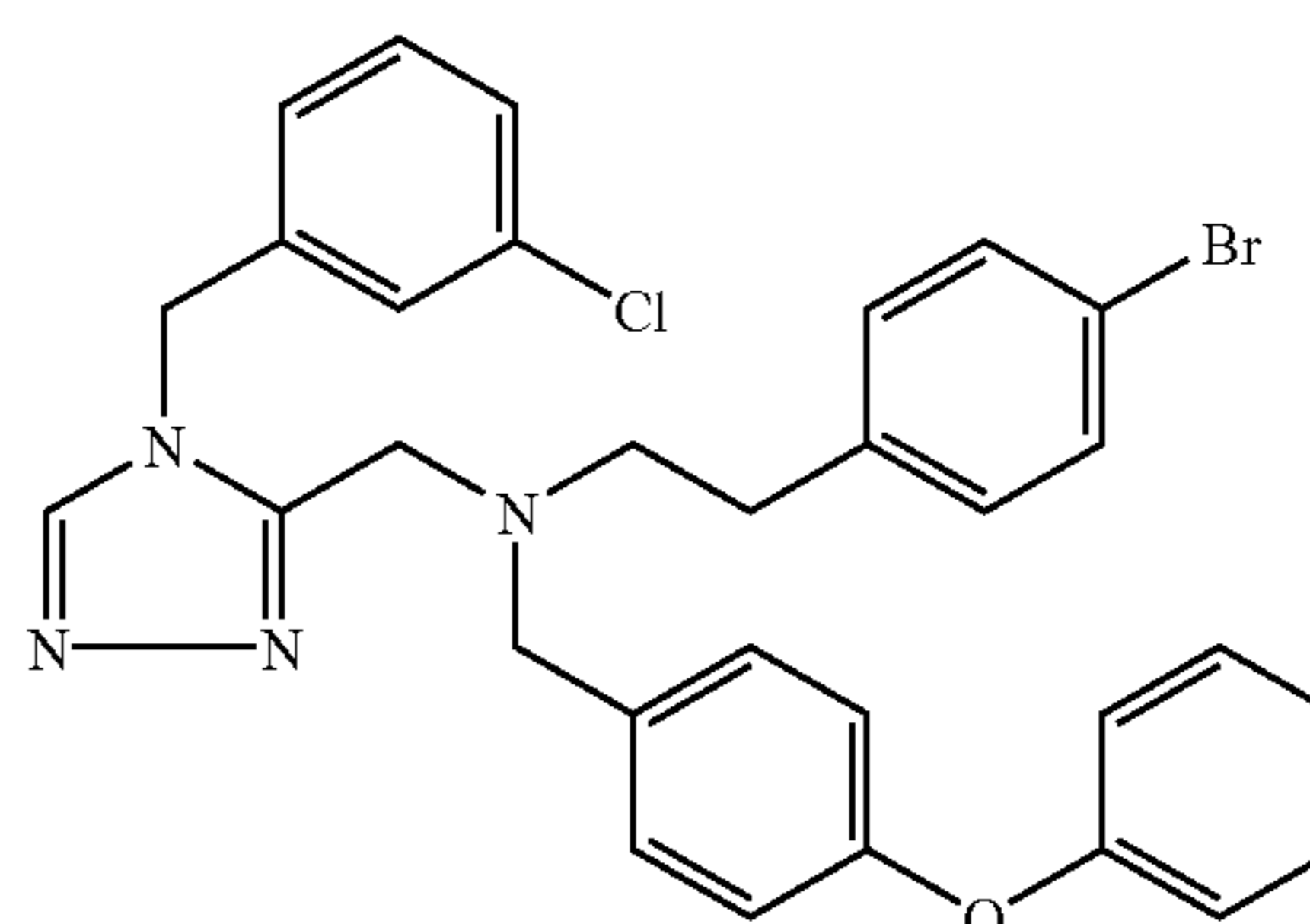
Trifluoroacetate (1:1) comp. 12.
