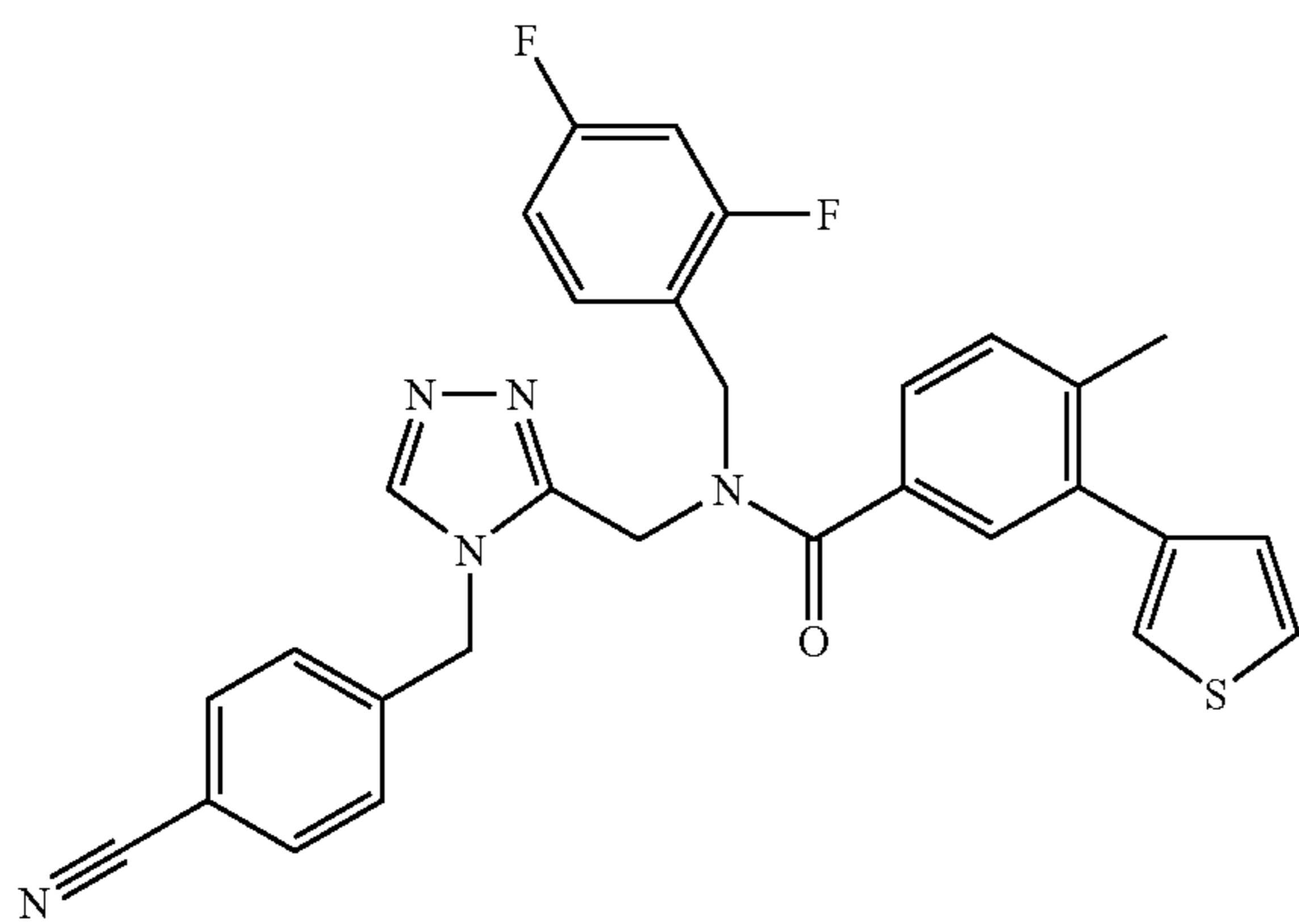
Trifluoroacetate (1:1) comp. 288.
