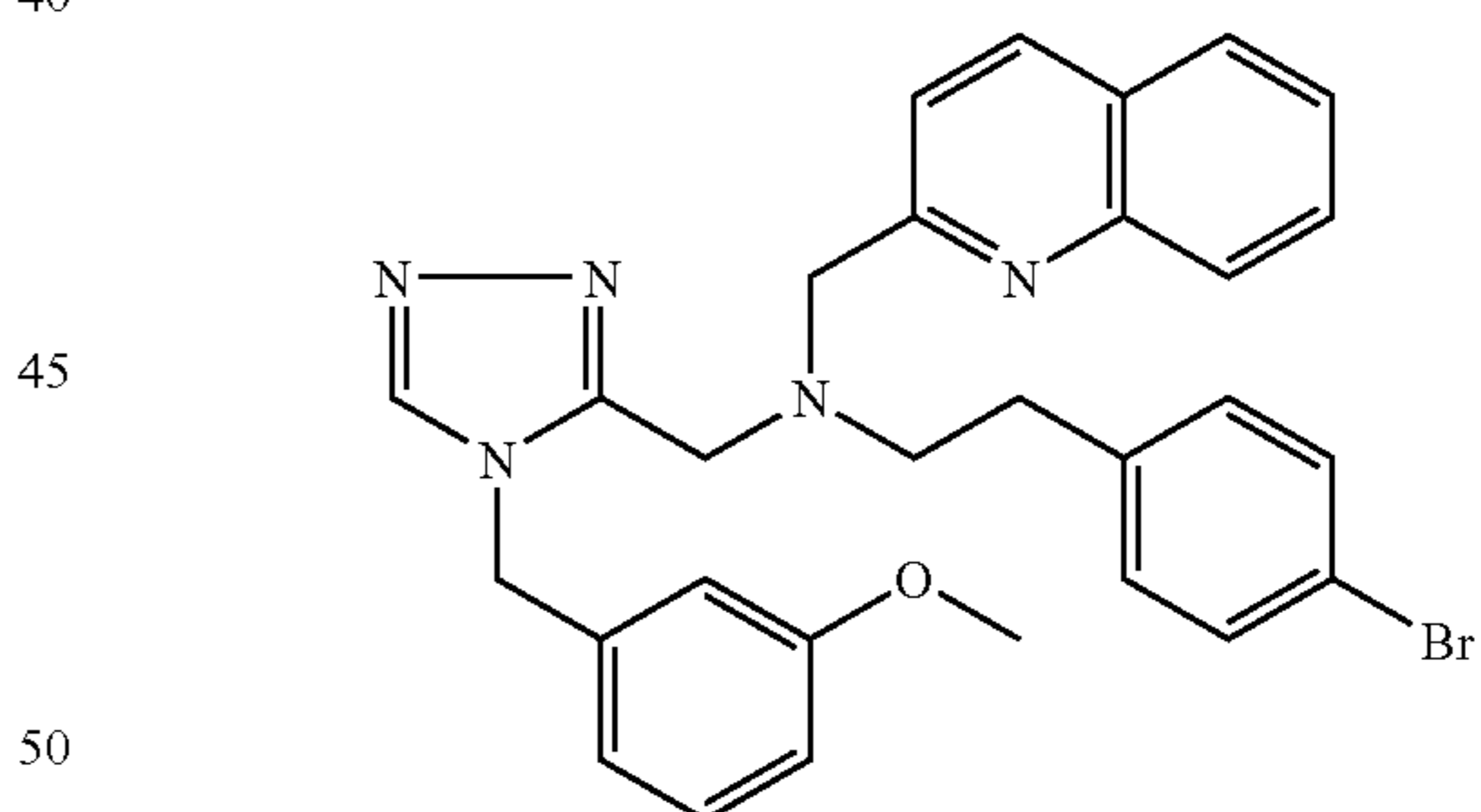
Trifluoroacetate (1:1) comp. 103.
