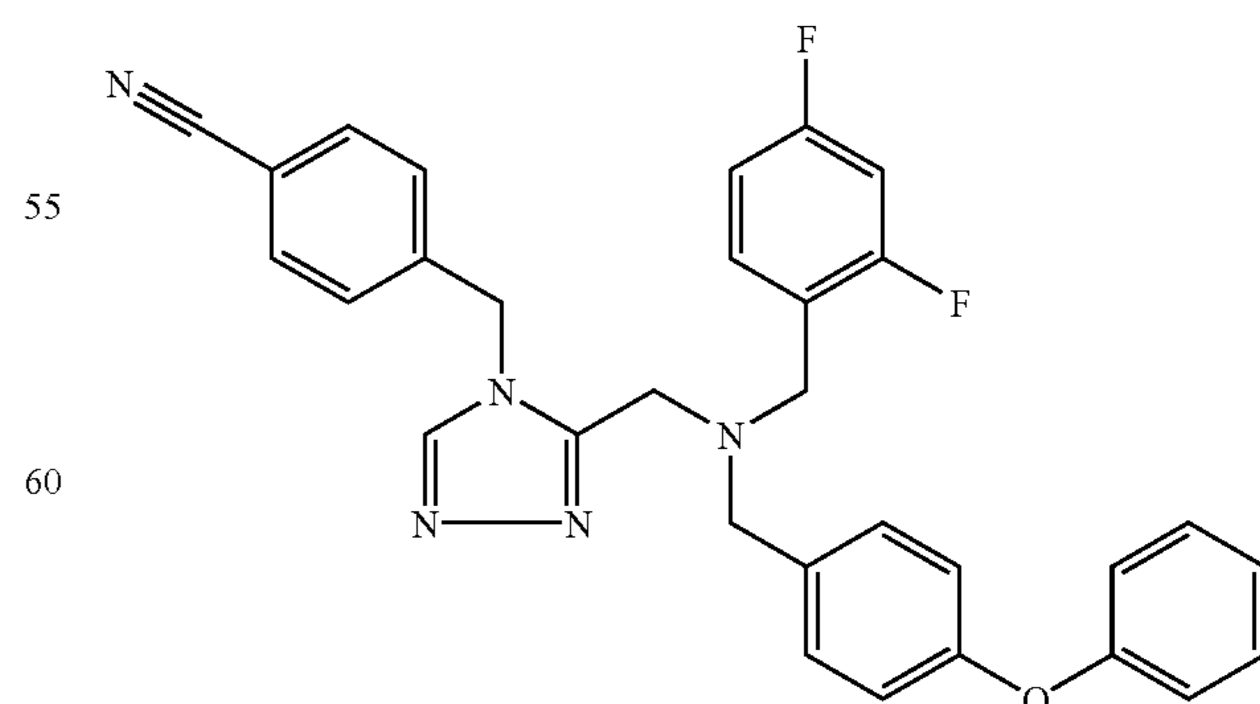
Trifluoroacetate (1:1) comp. 47.
