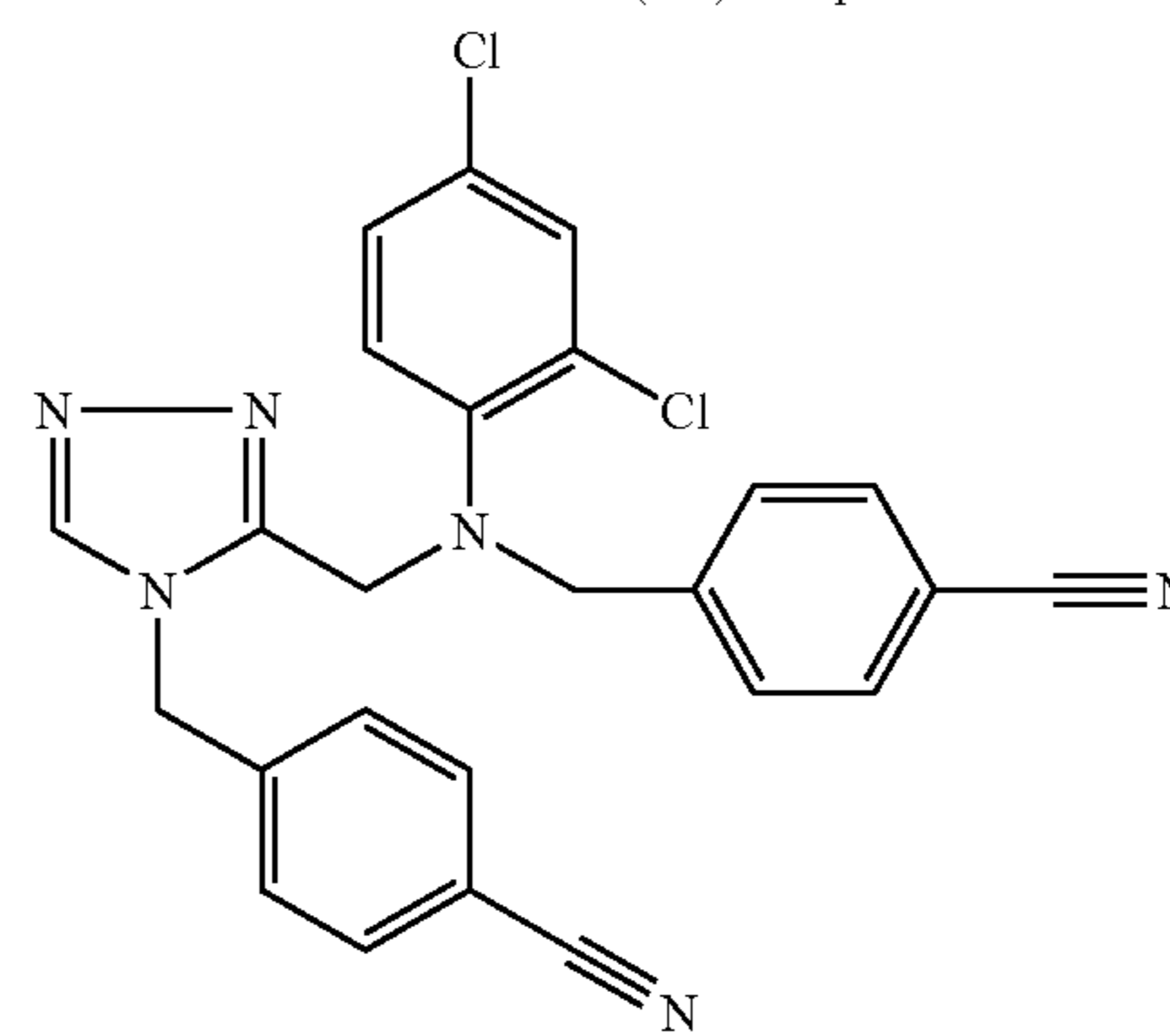
Trifluoroacetate (1:1) comp. 86.
