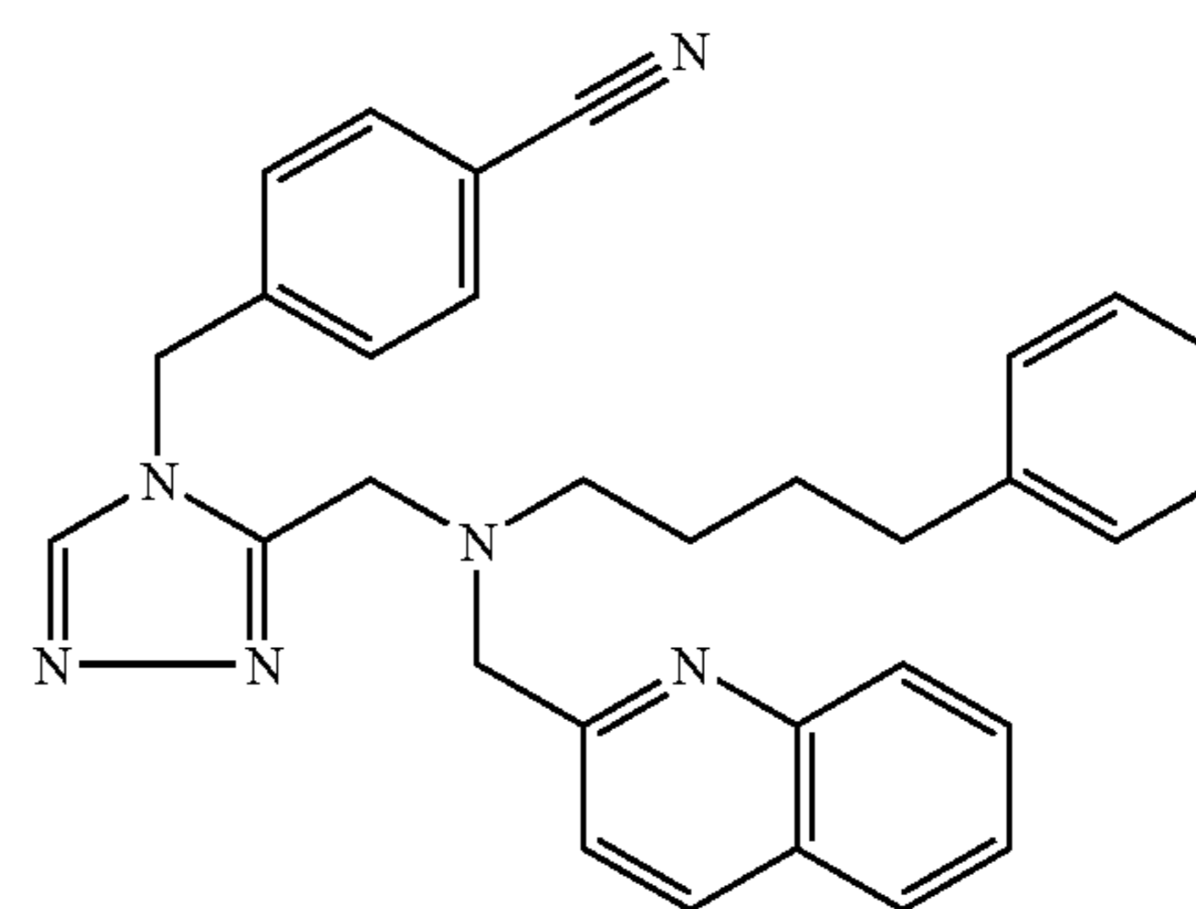
Trifluoroacetate (1:1) comp. 112.
