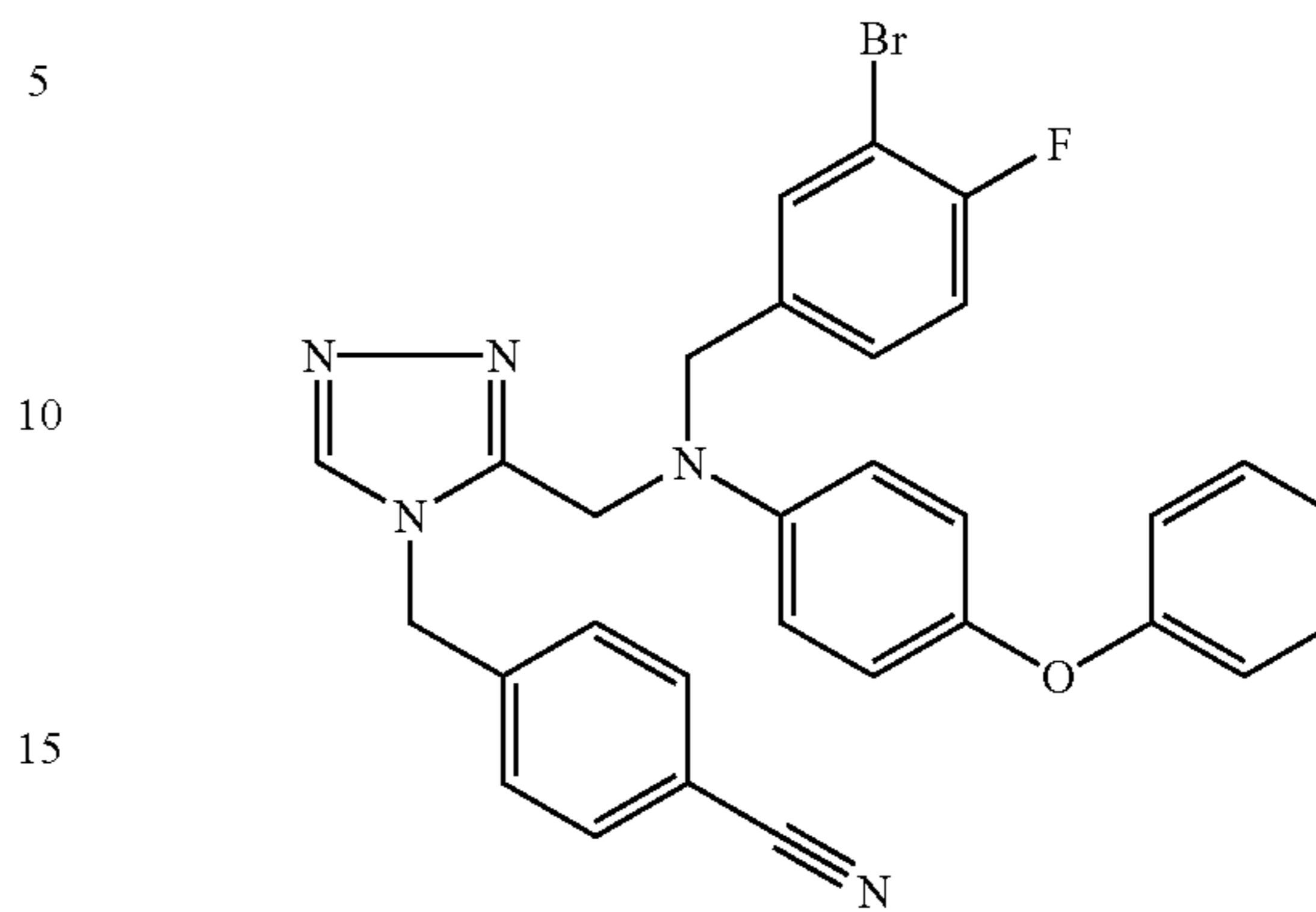
Trifluoroacetate (1:1) comp. 60.
