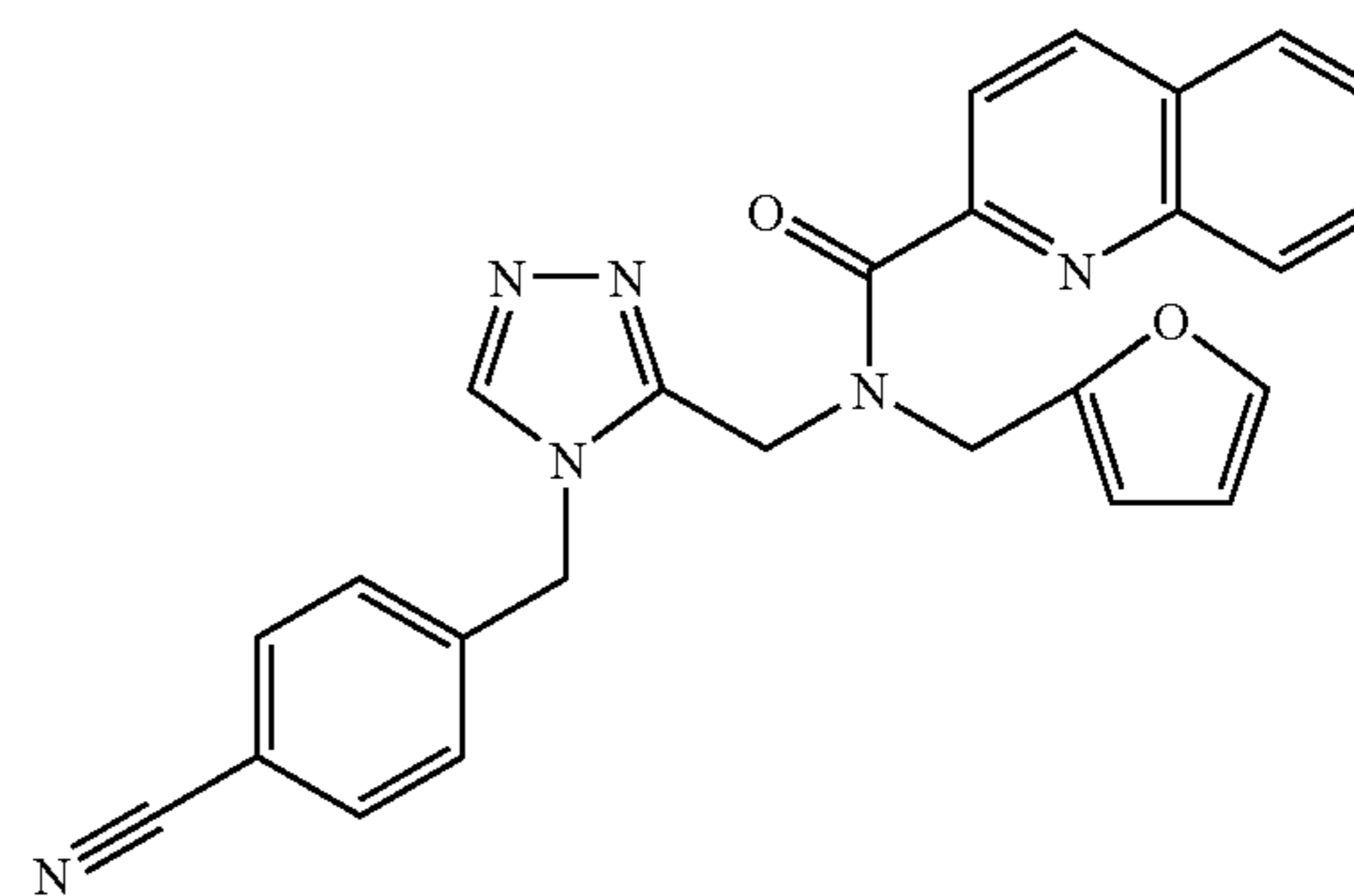
Trifluoroacetate (1:1) comp. 247.
