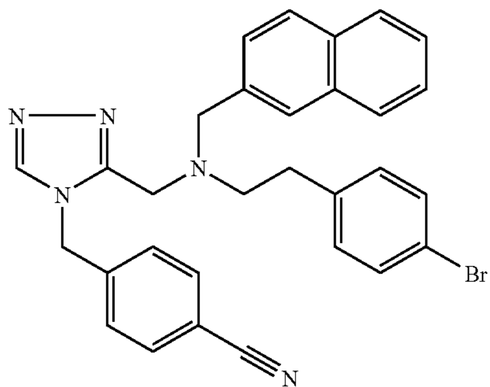
Trifluoroacetate (1:1) comp. 139.
