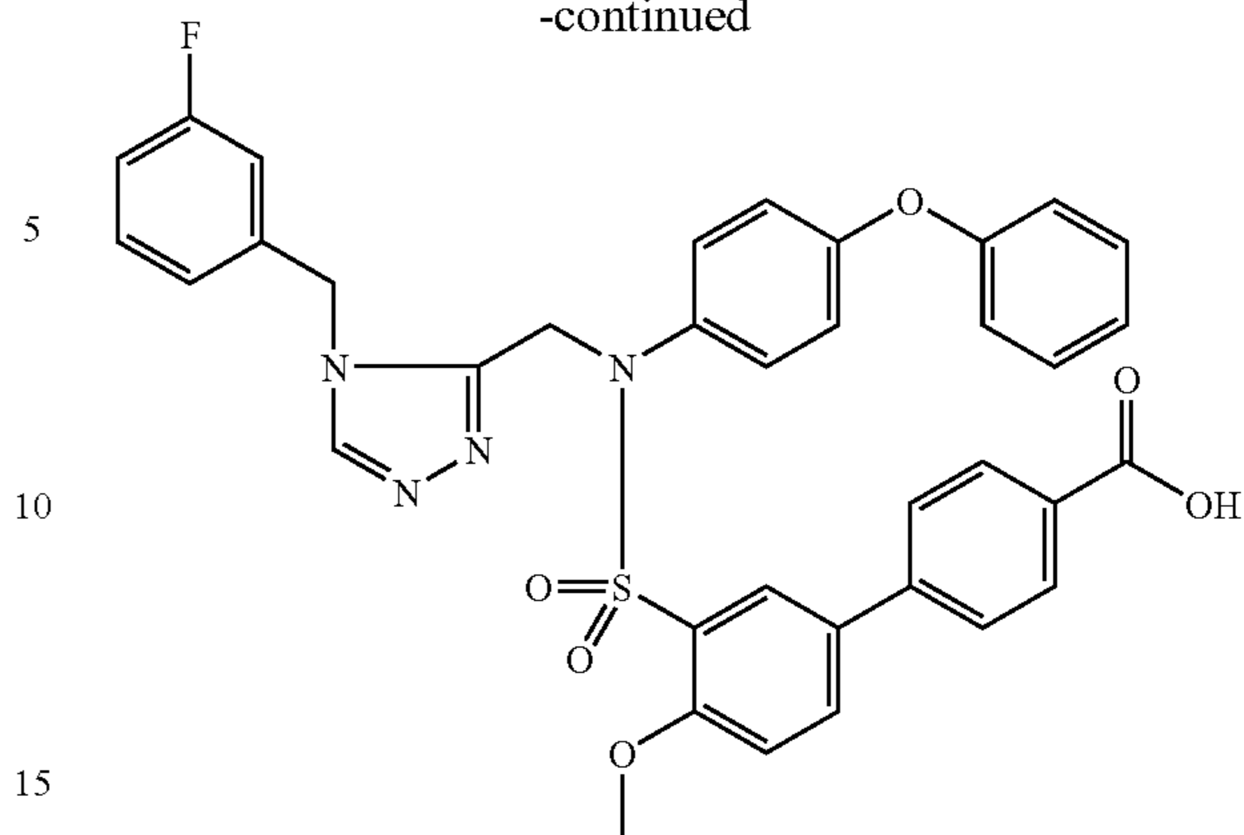
Trifluoroacetate (1:1) comp. 214.
