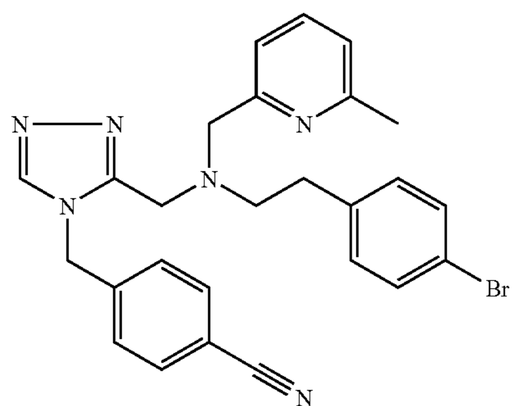
Trifluoroacetate (1:1) comp. 107.
