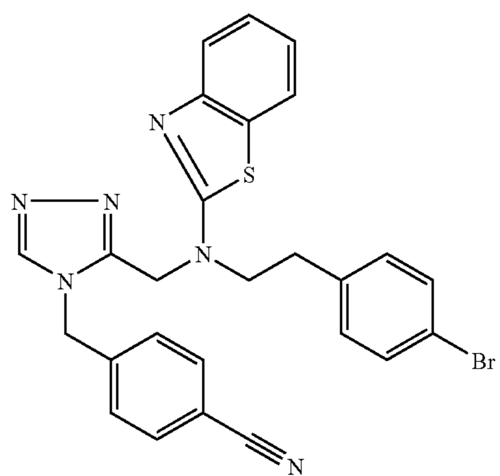
Trifluoroacetate (1:1) comp. 162.
