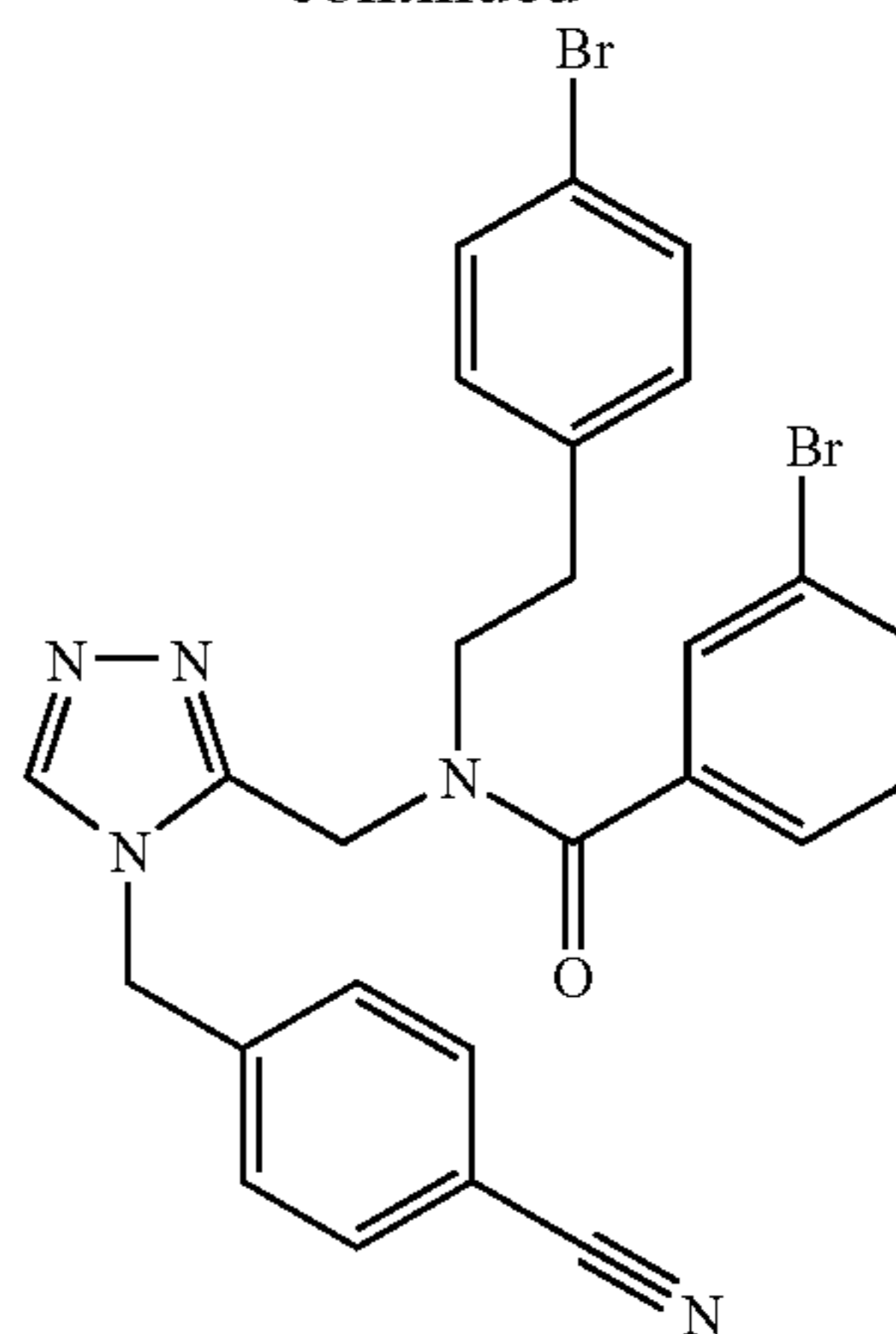
Trifluoroacetate (1:1) comp. 222.
