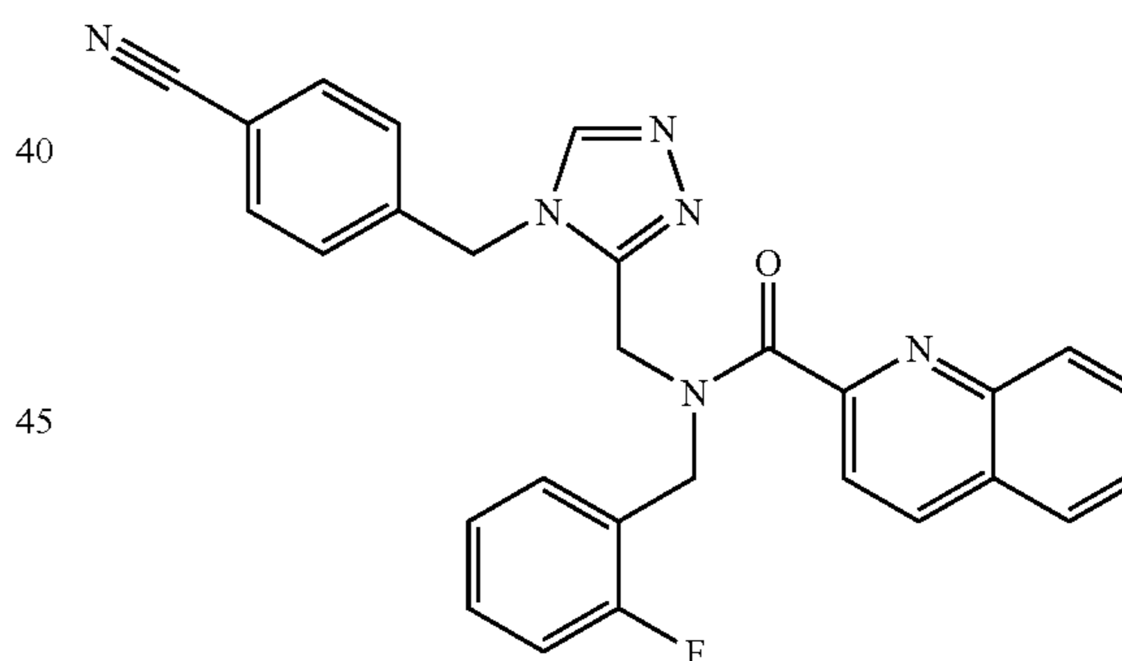
2-Quinolinecarboxamide, N-[[4-[(4-cyanophenyl)methyl]-4H-1,2,4-triazol-3-yl]methyl]-N-[(2-fluorophenyl)methyl]-
