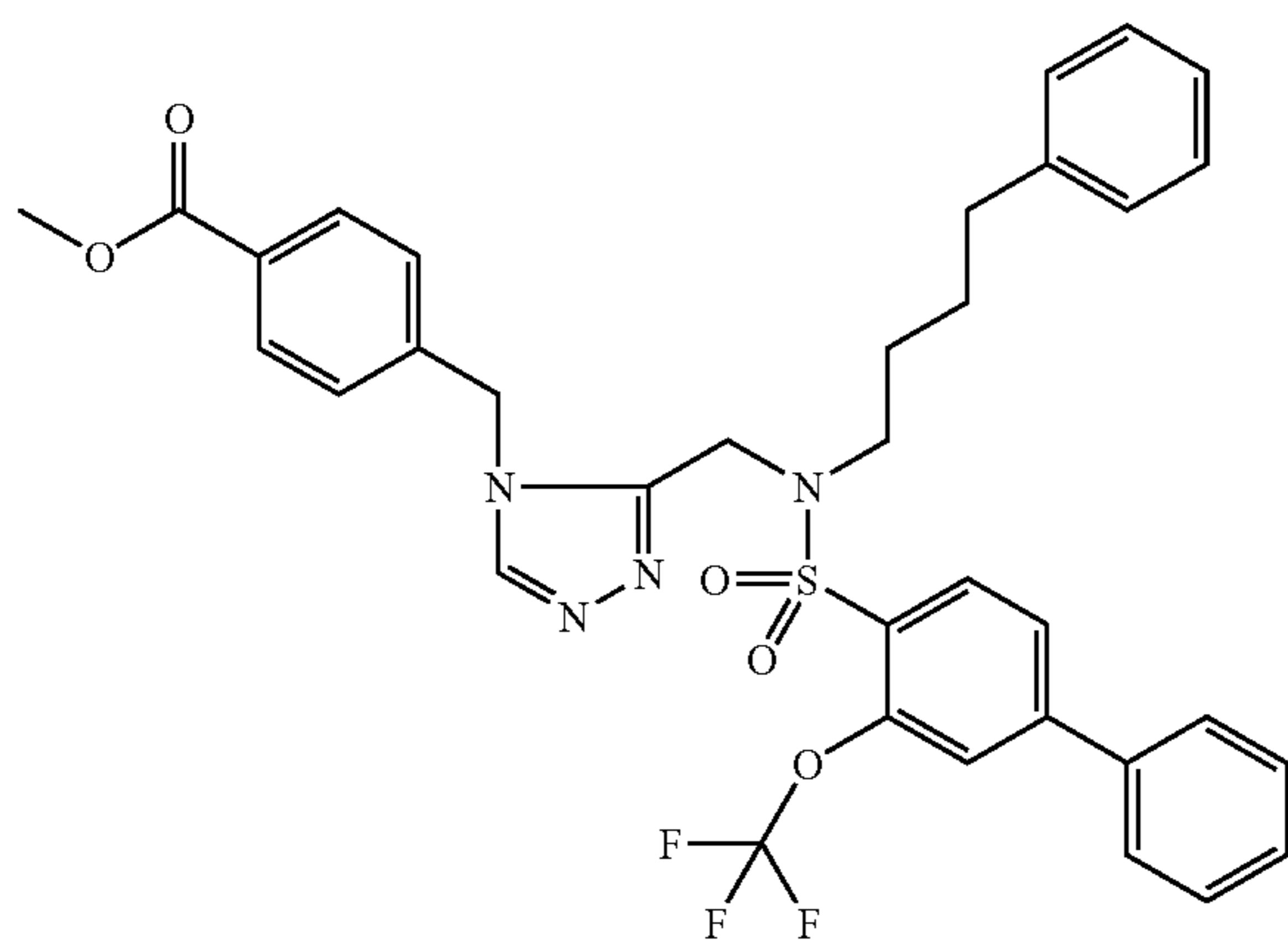
Trifluoroacetate (1:1) comp. 197.
