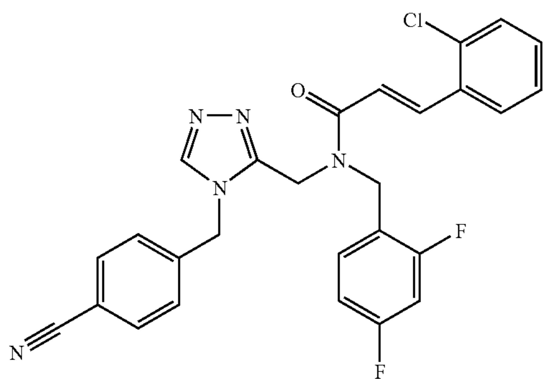
Trifluoroacetate (1:1) comp. 249.
