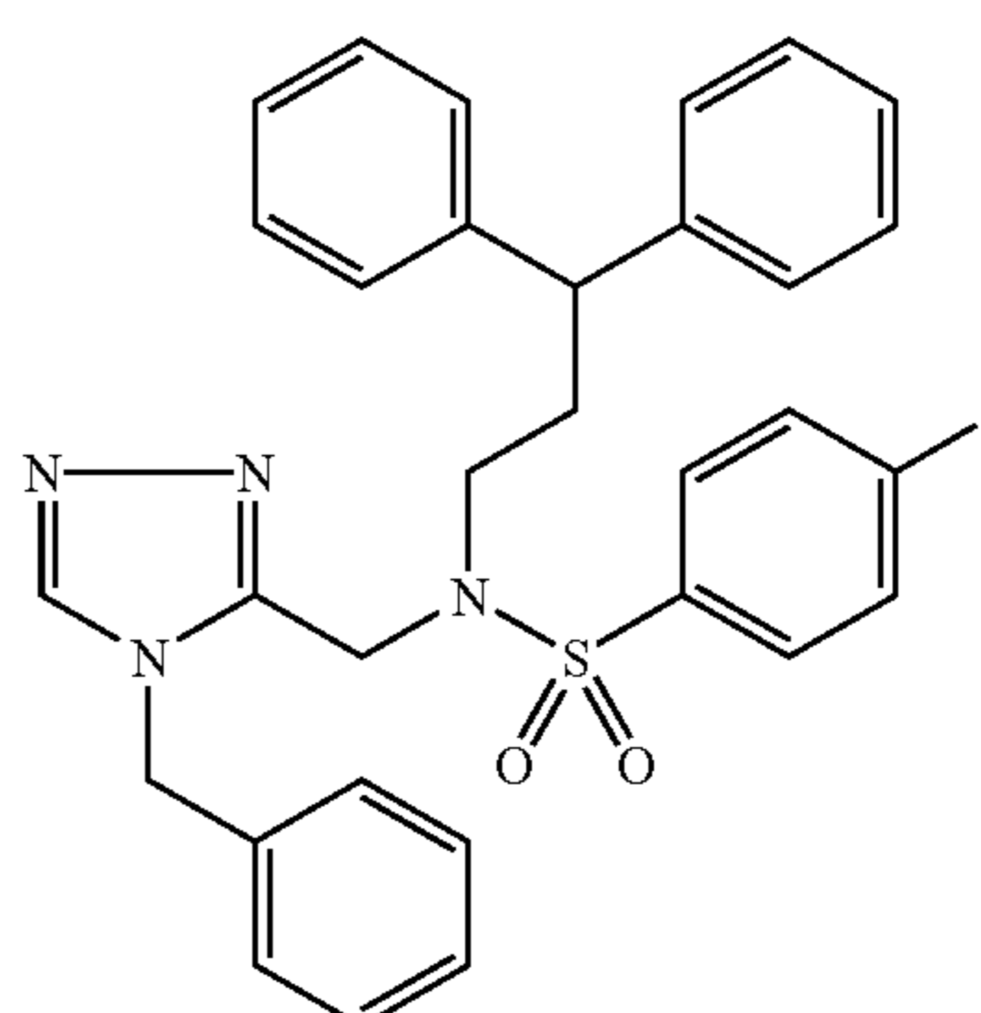
Trifluoroacetate (1:1) comp. 19.
