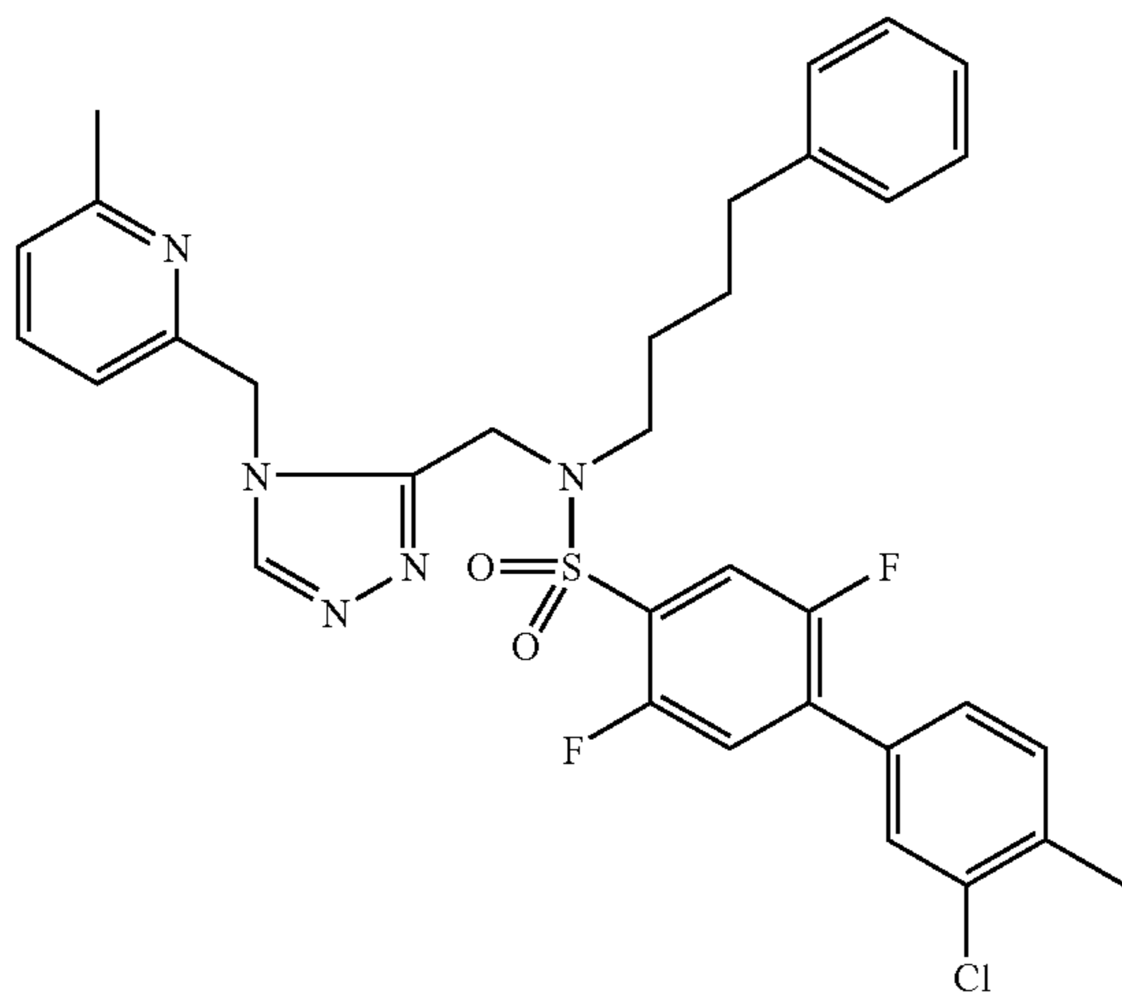
Trifluoroacetate (1:1) comp. 228.
