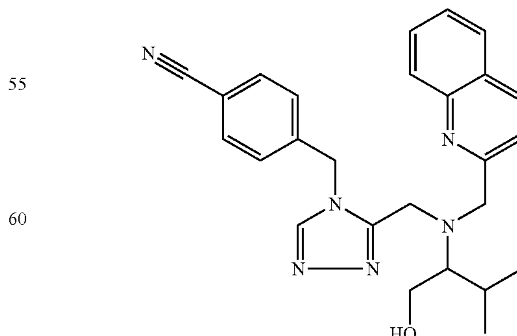
Trifluoroacetate (1:2) comp. 172.
