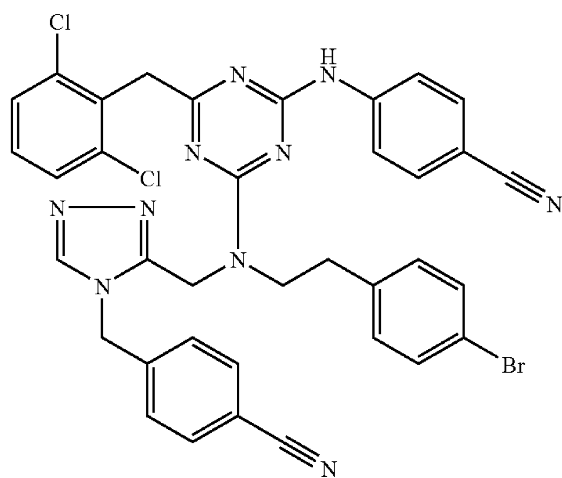
Trifluoroacetate (1:1) comp. 167.
