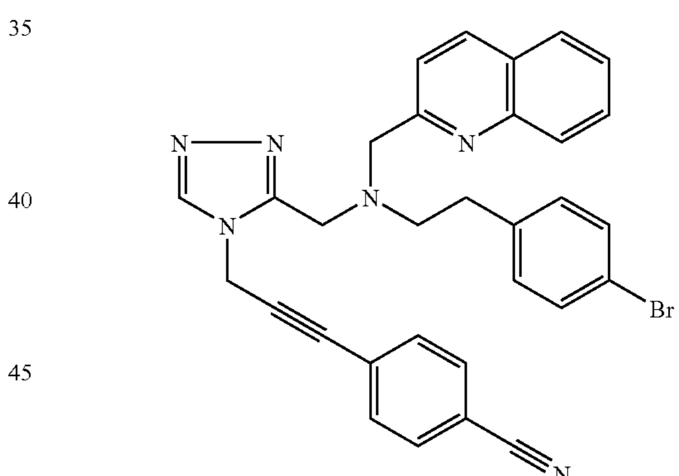
Trifluoroacetate (1:1) comp. 94.
