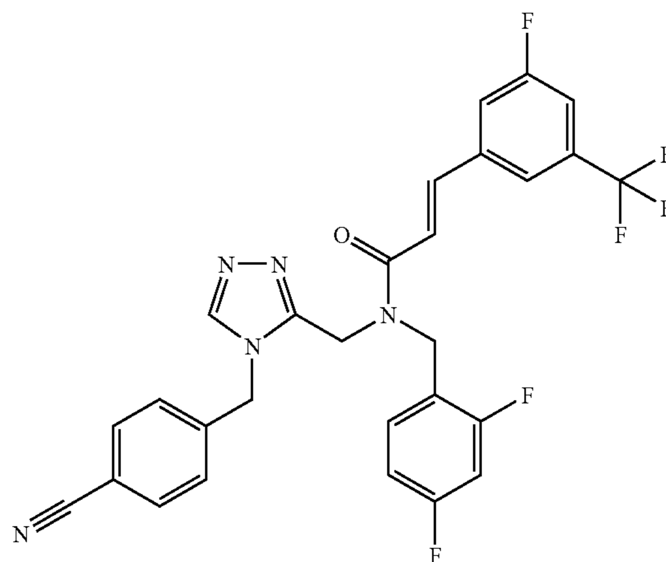
Trifluoroacetate (1:1) comp. 245.
