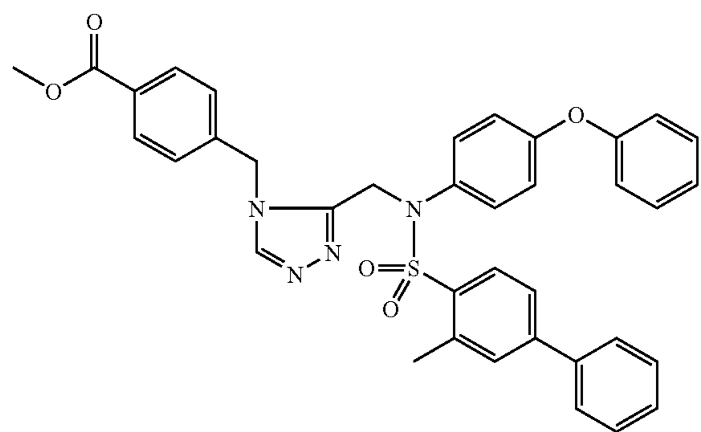
Trifluoroacetate (1:1) comp. 200.
