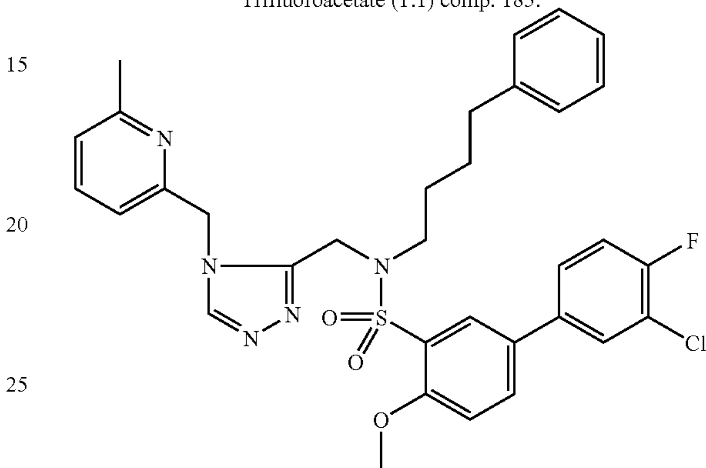
Trifluoroacetate (1:1) comp. 186.
