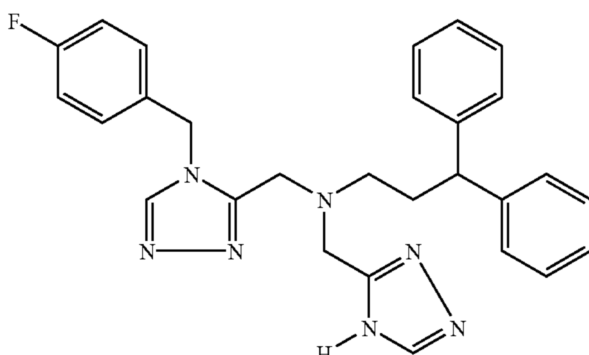
Trifluoroacetate (1:1) comp. 40.
