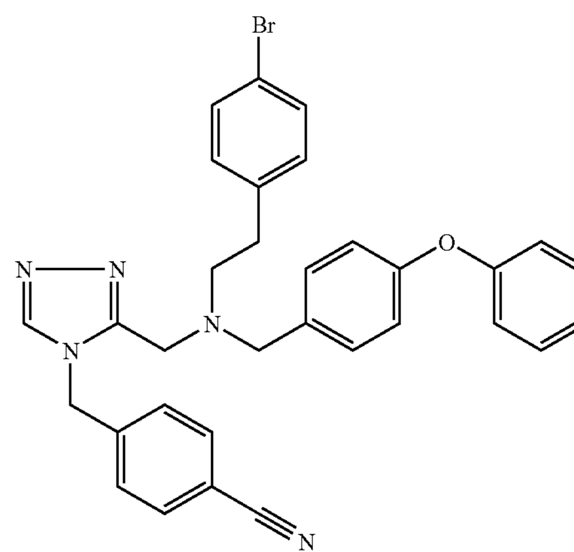
Trifluoroacetate (1:1) comp. 3.
