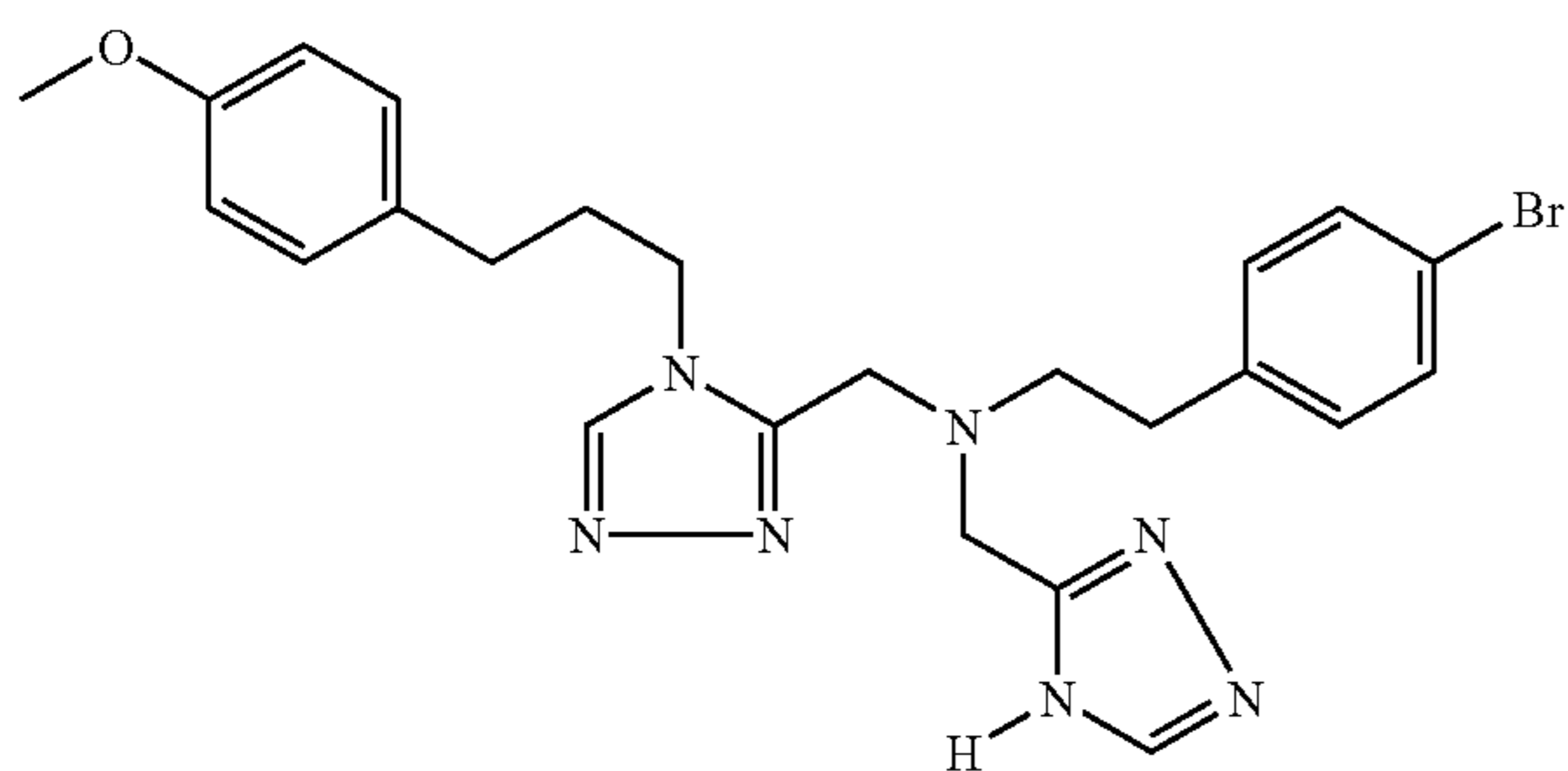
Trifluoroacetate (1:1) comp. 31.
