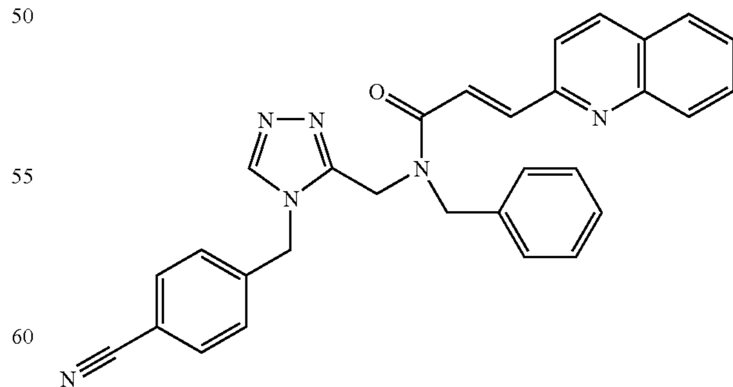
Trifluoroacetate (1:1) comp. 231.
