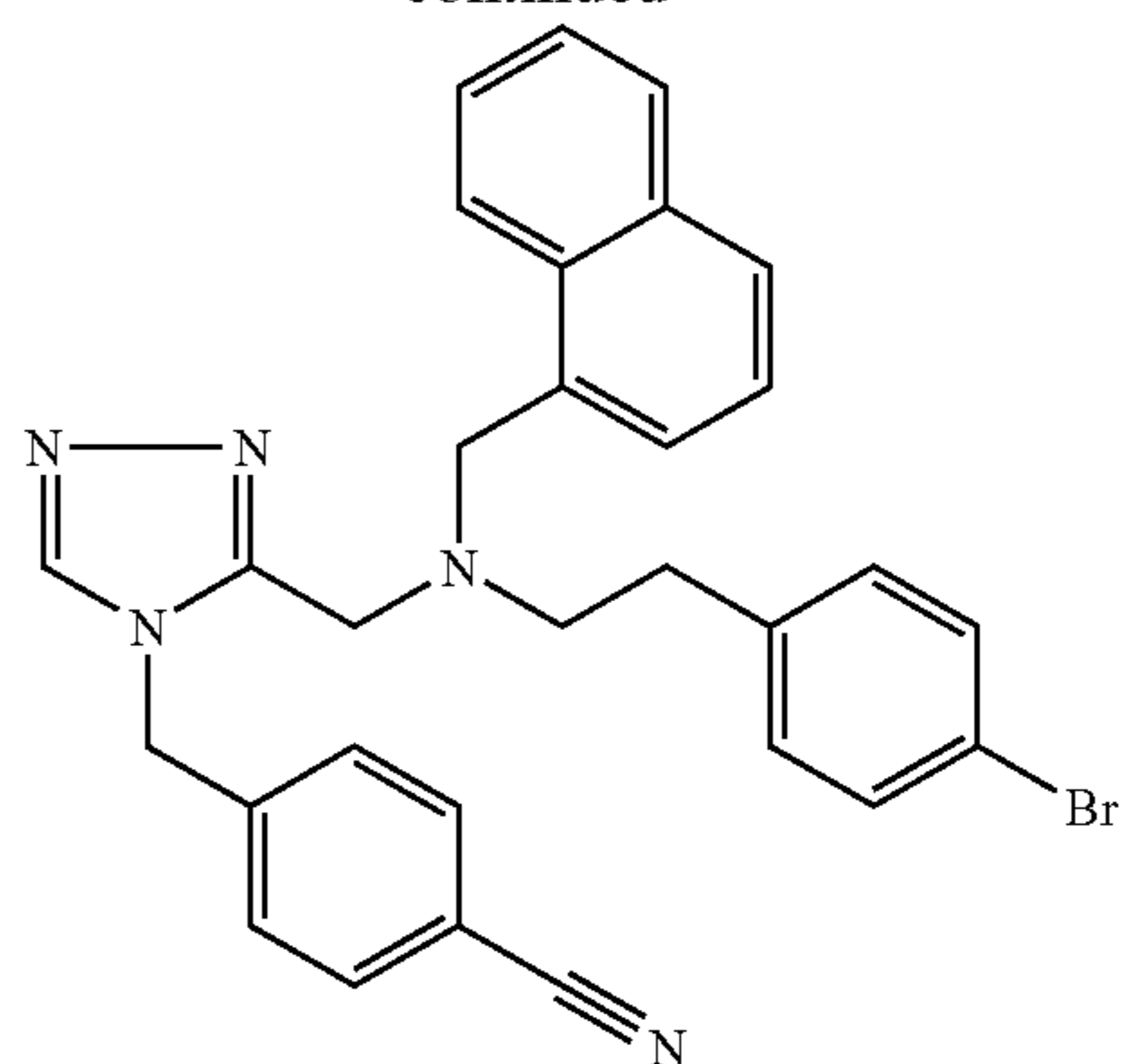
Trifluoroacetate (1:1) comp. 109.
