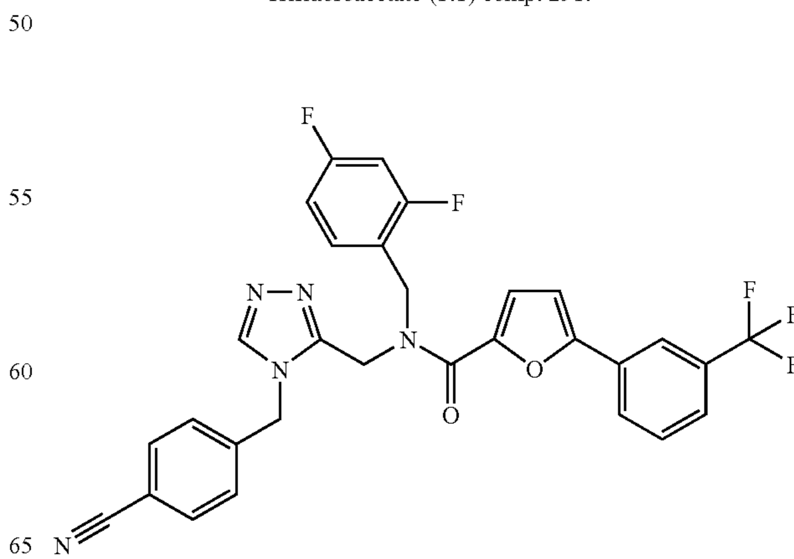
Trifluoroacetate (1:1) comp. 292.
