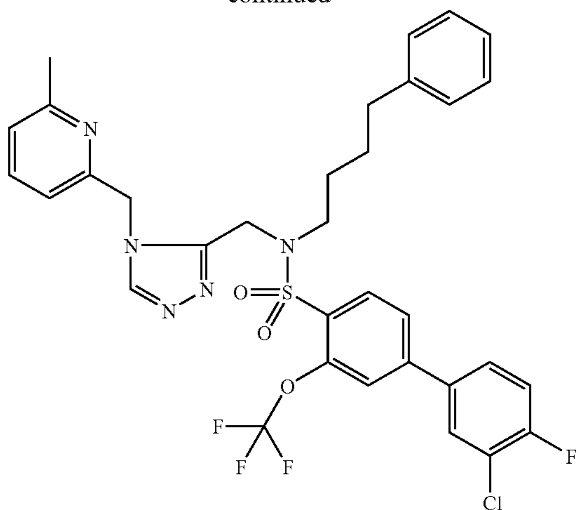
Trifluoroacetate (1:1) comp. 189.
