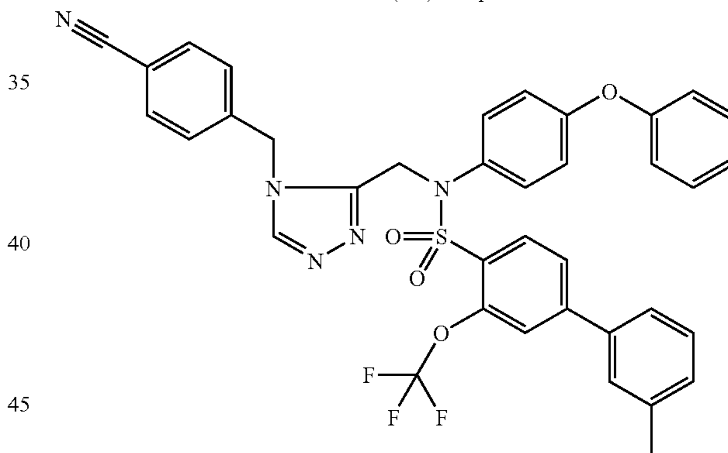
Trifluoroacetate (1:1) comp. 209.
