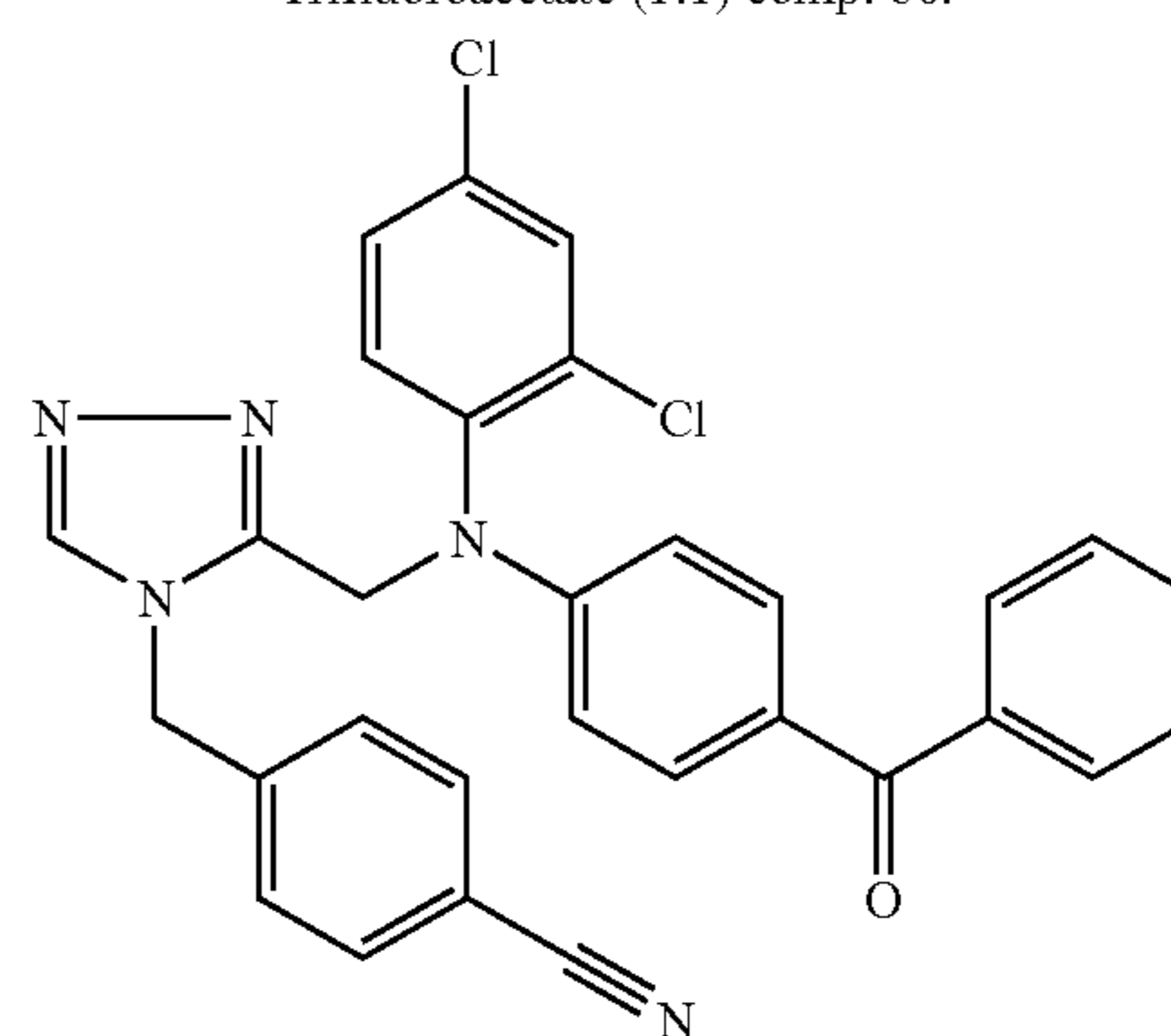
Trifluoroacetate (1:1) comp. 87.
