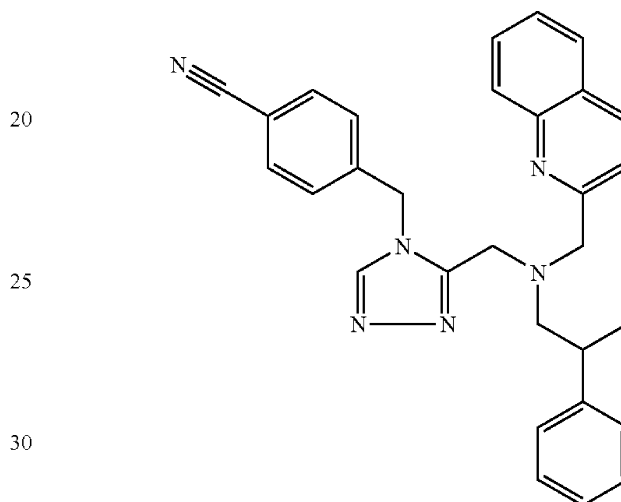
Trifluoroacetate (1:2) comp. 170.
