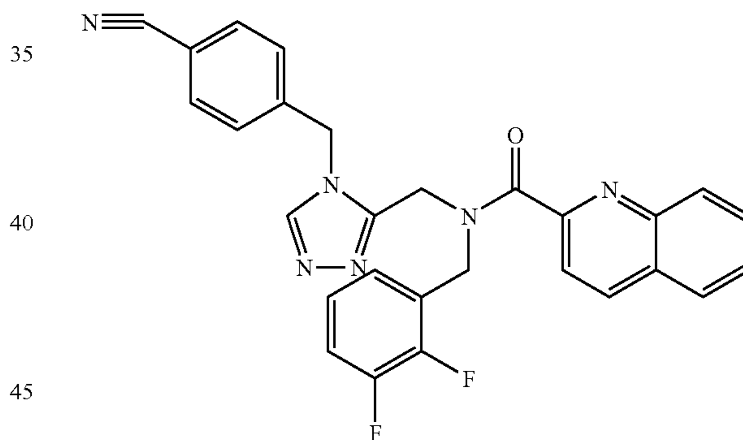
Trifluoroacetate (1:1) comp. 307.
