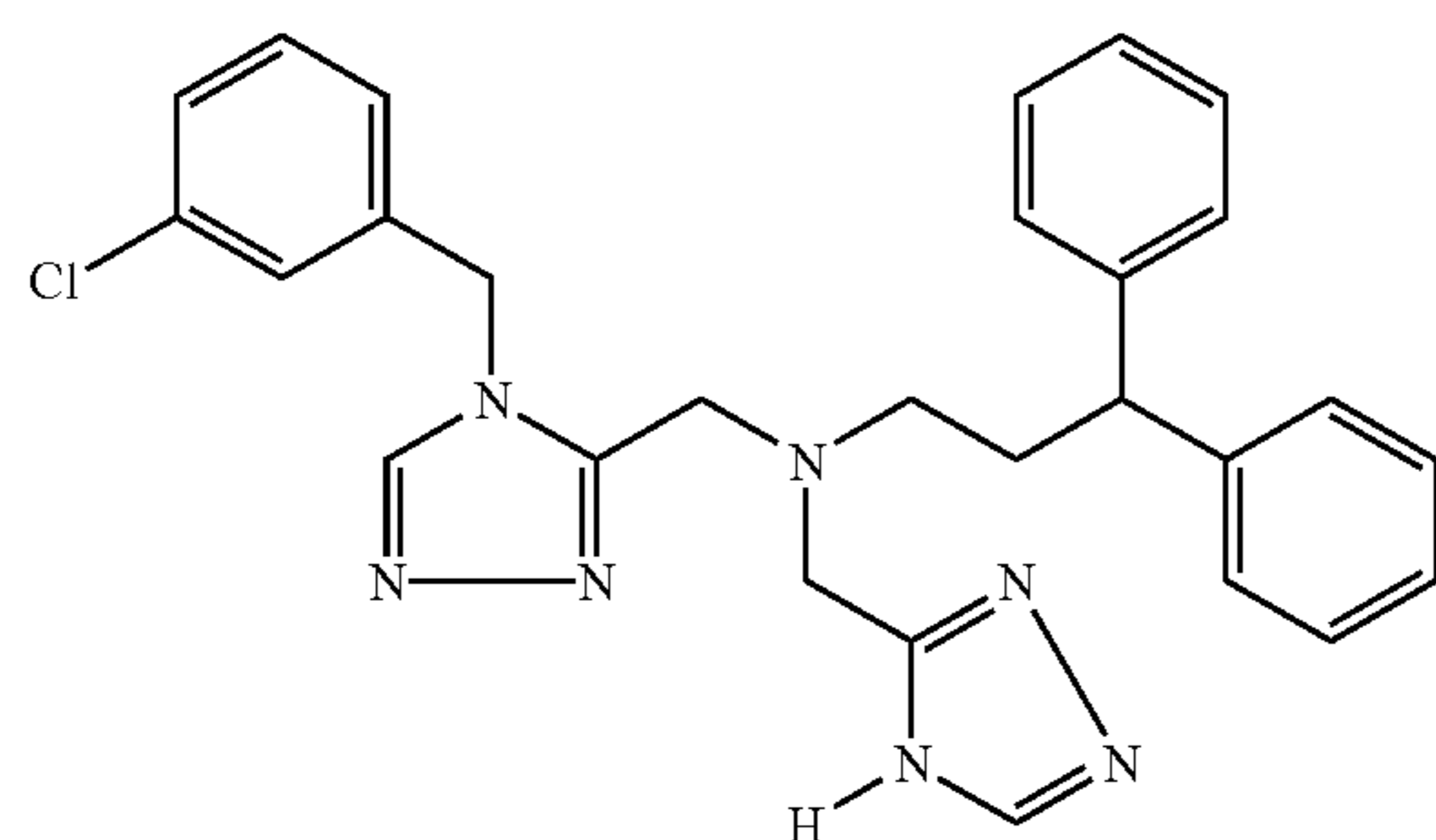
Trifluoroacetate (1:1) comp. 42.
