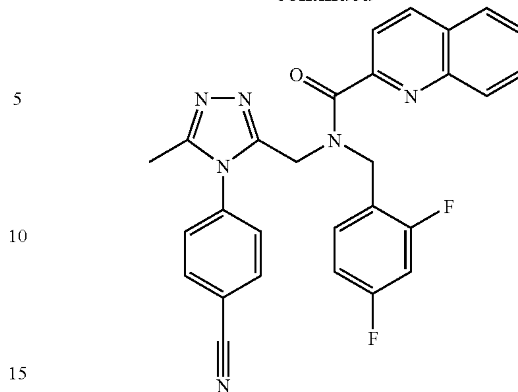
Trifluoroacetate (1:1) comp. 313.
