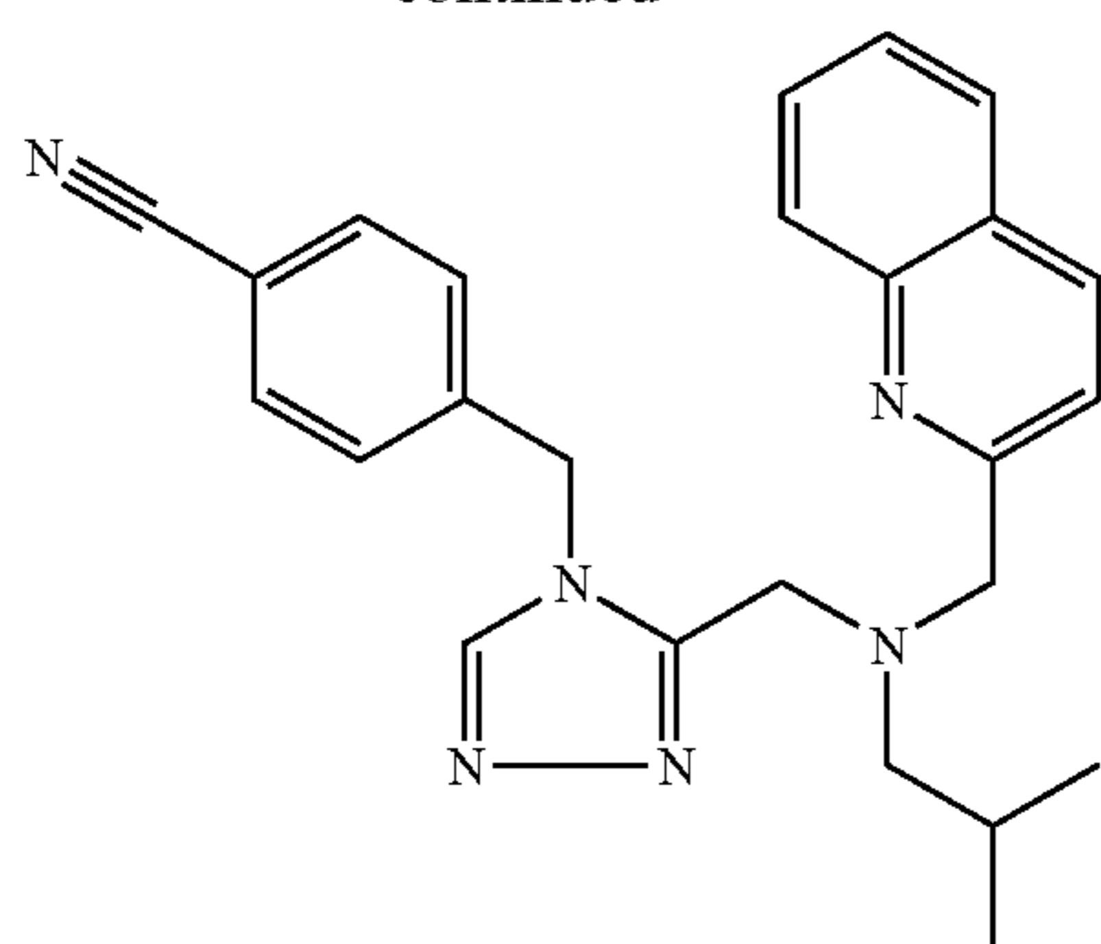
Trifluoroacetate (1:2) comp. 173.
