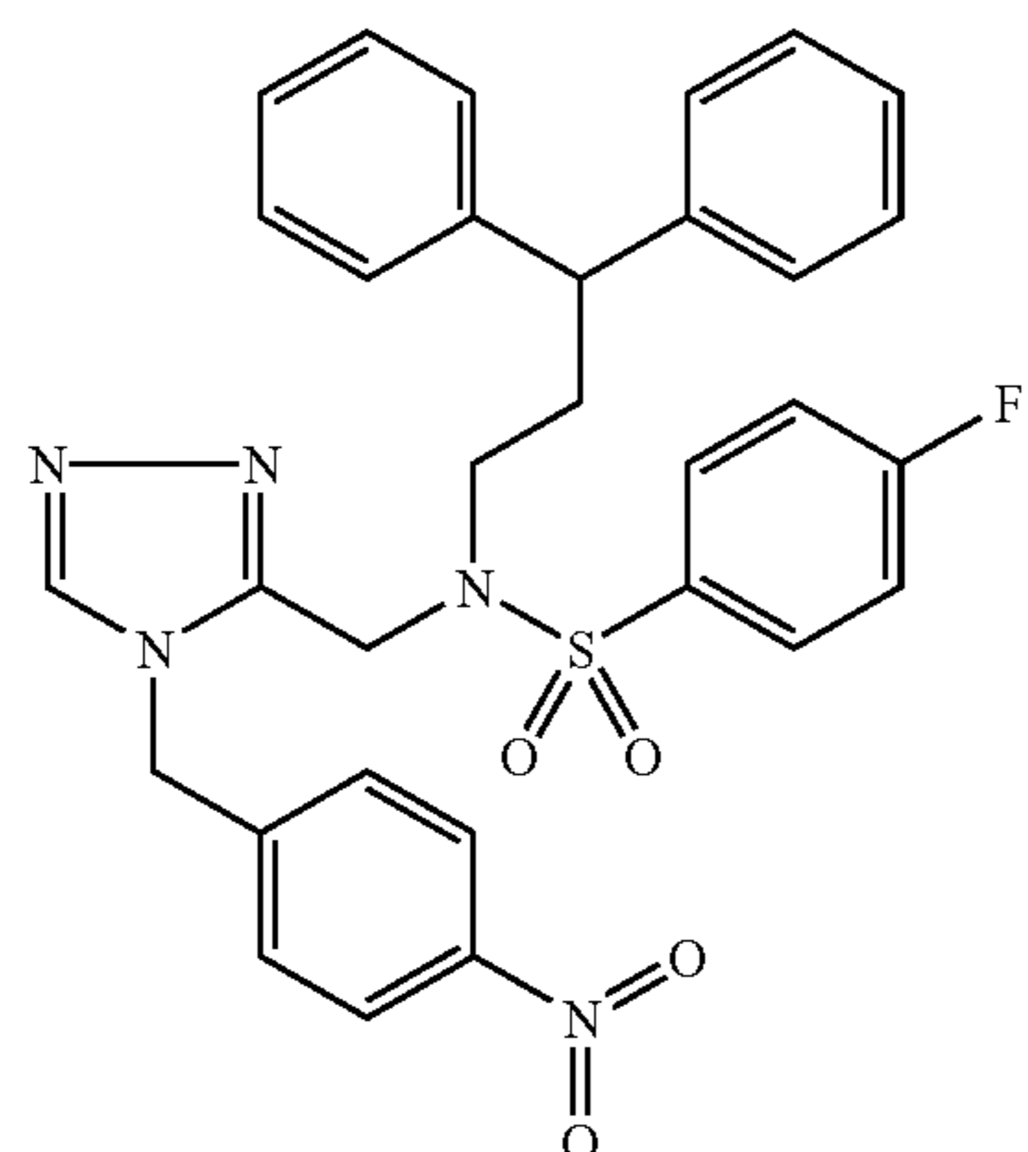
Trifluoroacetate (1:1) comp. 5.
