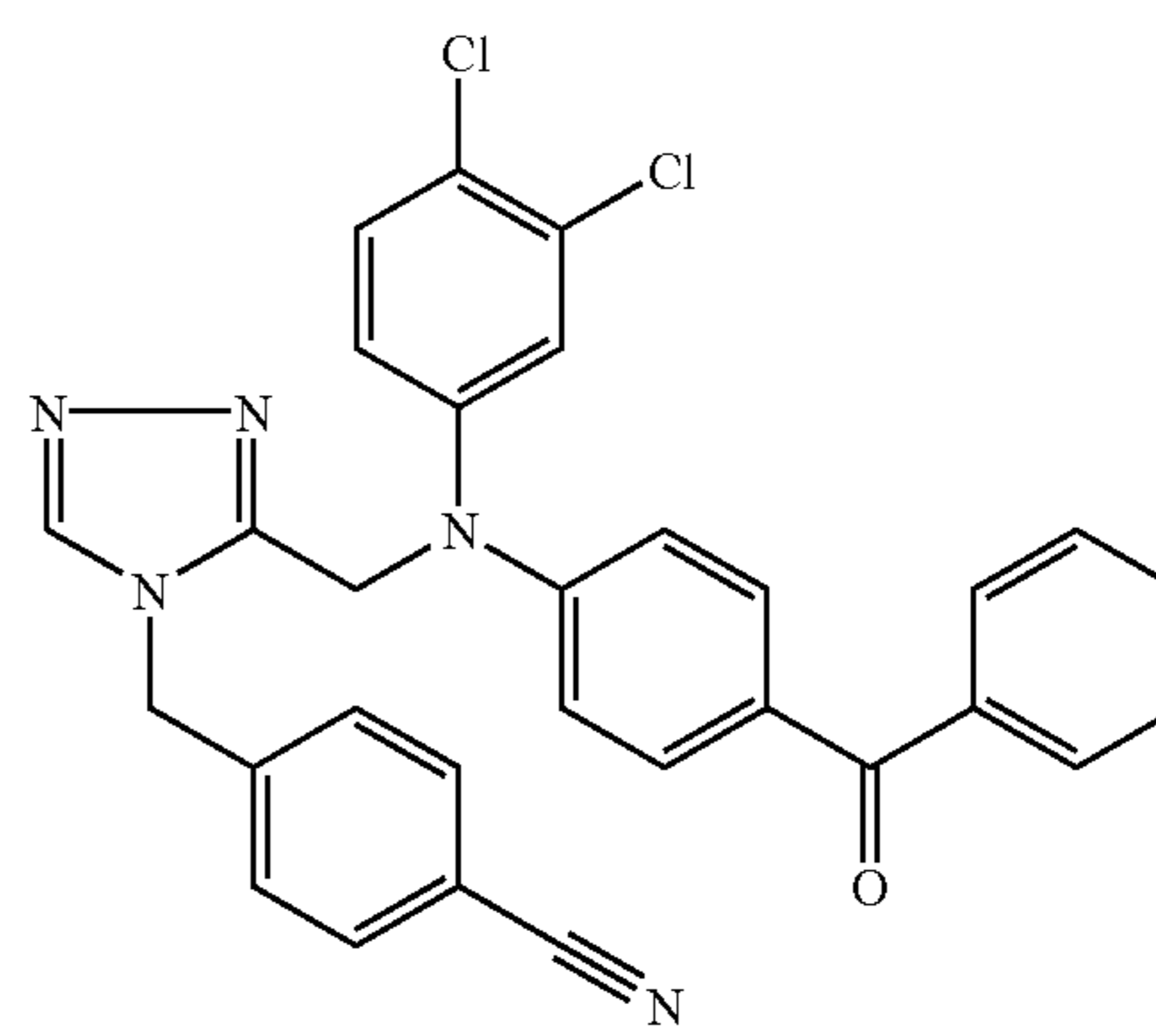
Trifluoroacetate (1:1) comp. 76.
