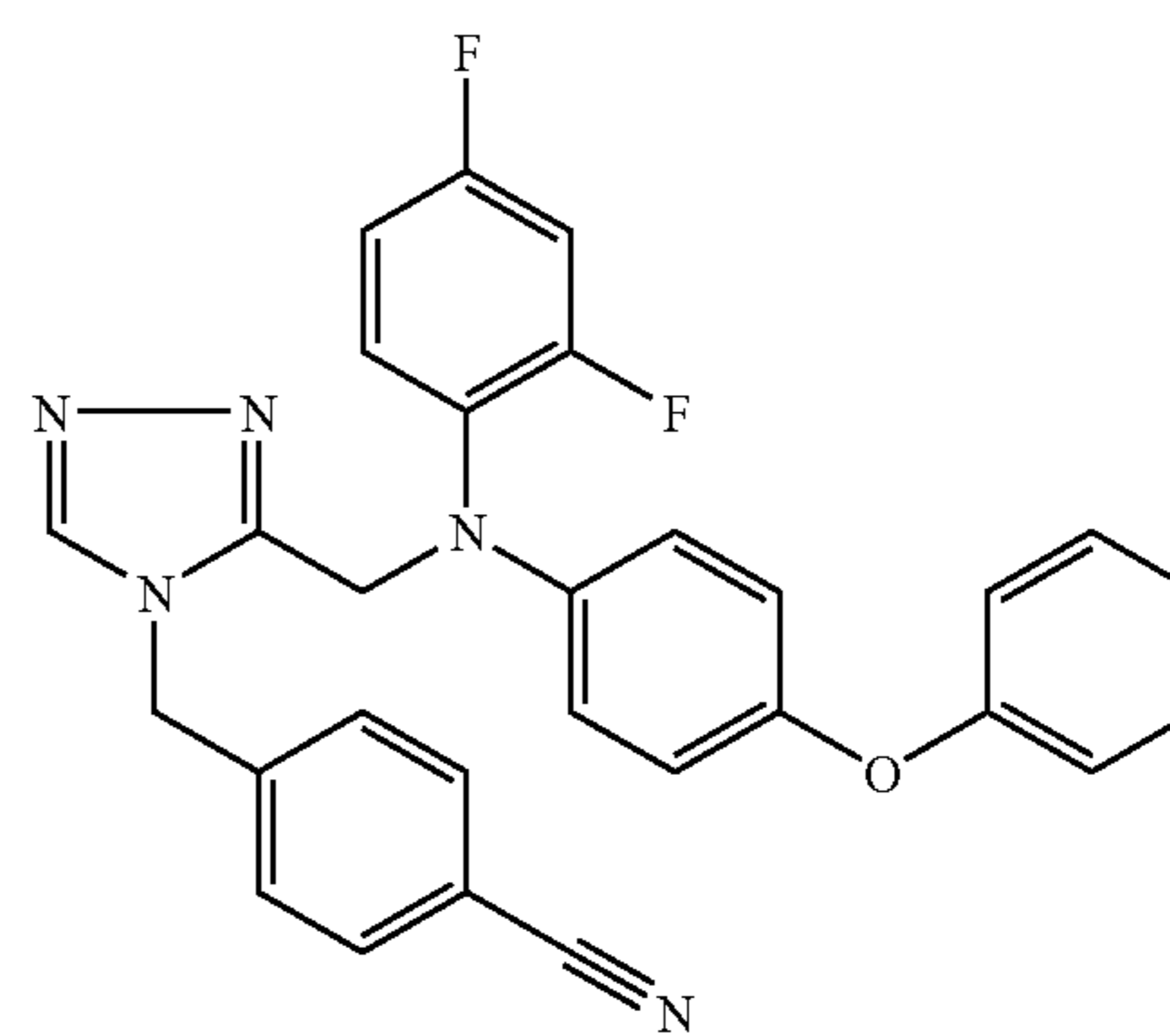
Trifluoroacetate (1:1) comp. 84.
