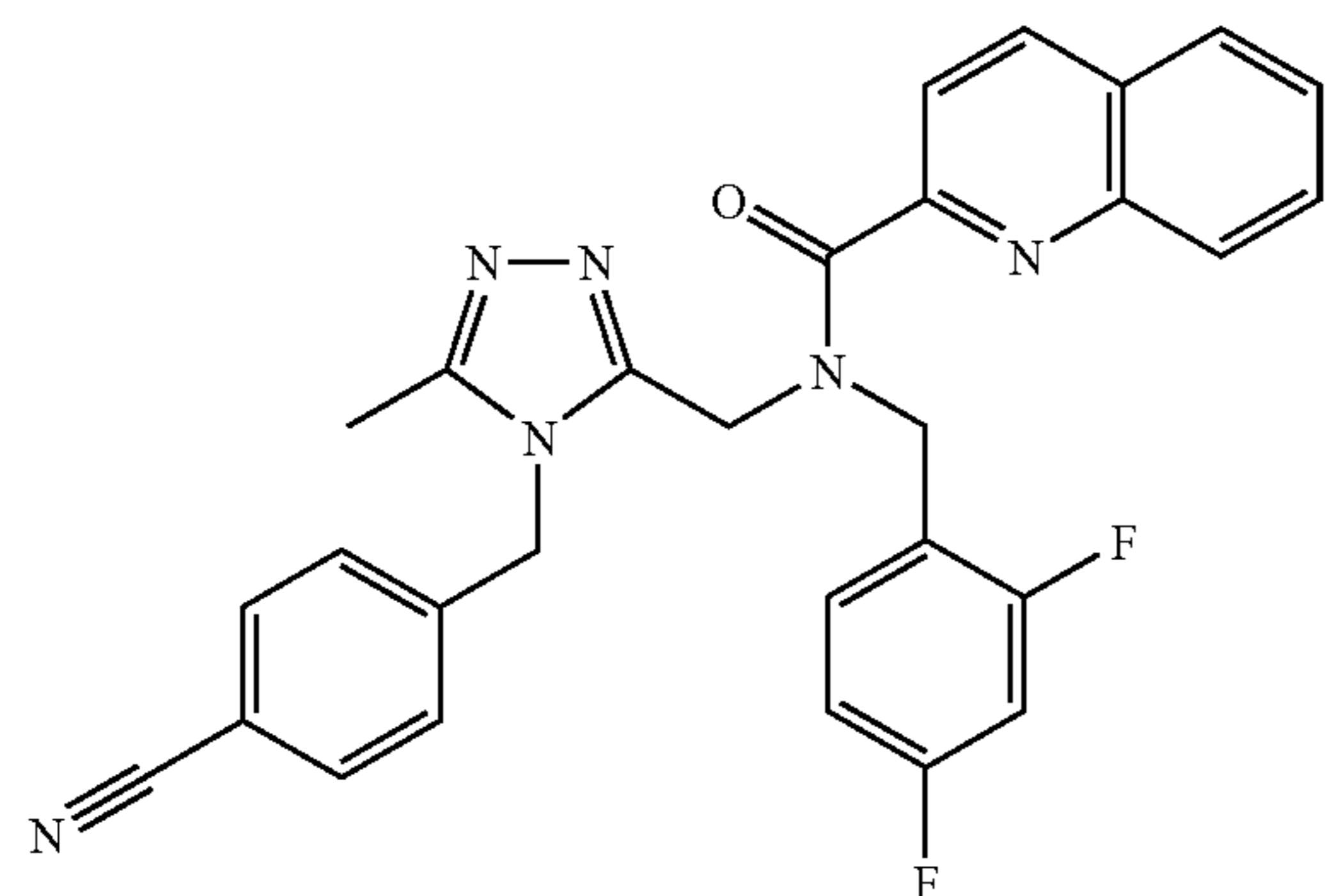
2-Quinolinecarboxamide, N-[[4-[(4-cyanophenyl)methyl]-5-methyl-4H-1,2,4-triazol-3-yl]methyl]-N-[(2,4-difluorophenyl)methyl]-
