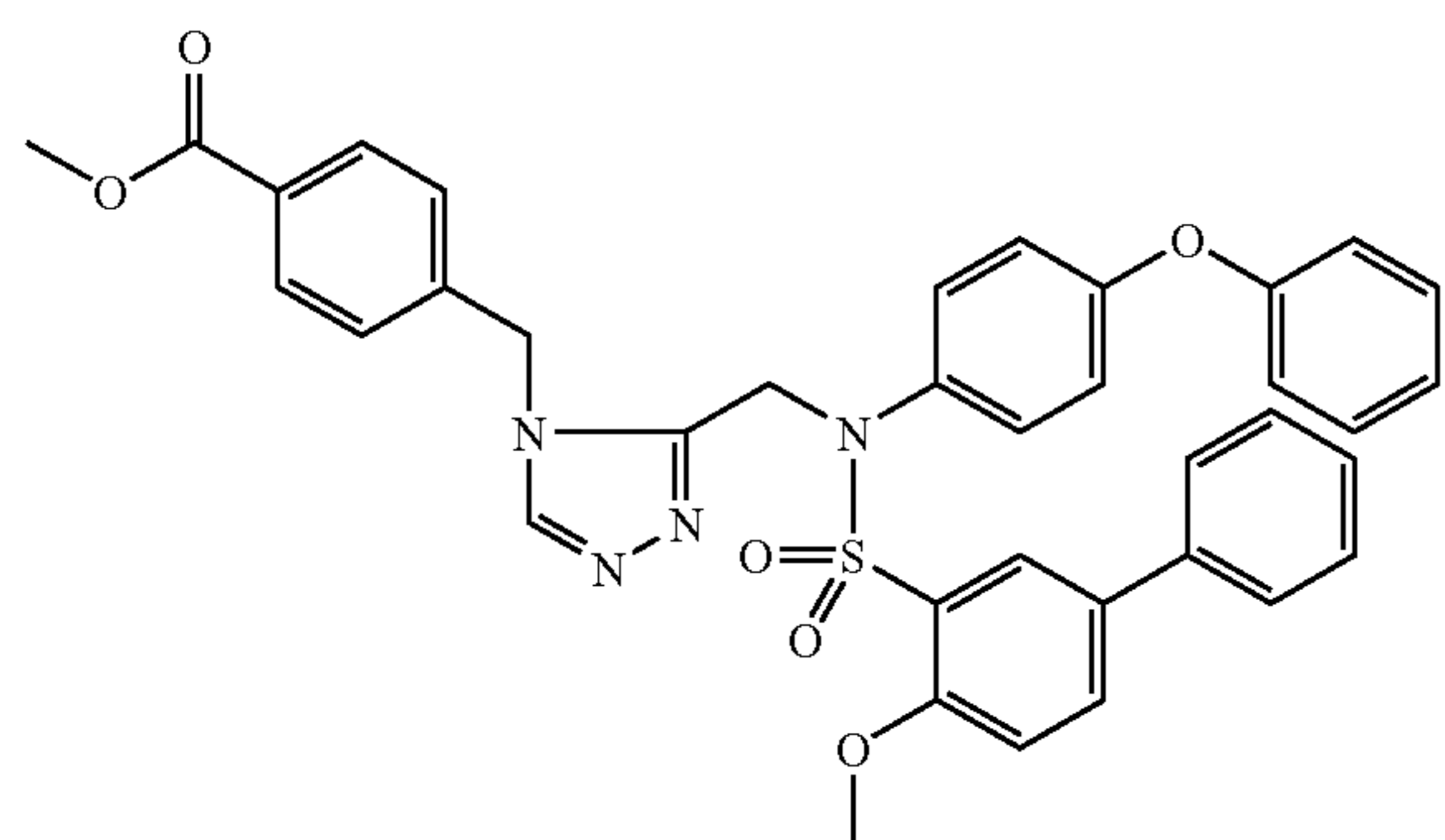
Trifluoroacetate (1:1) comp. 198.
