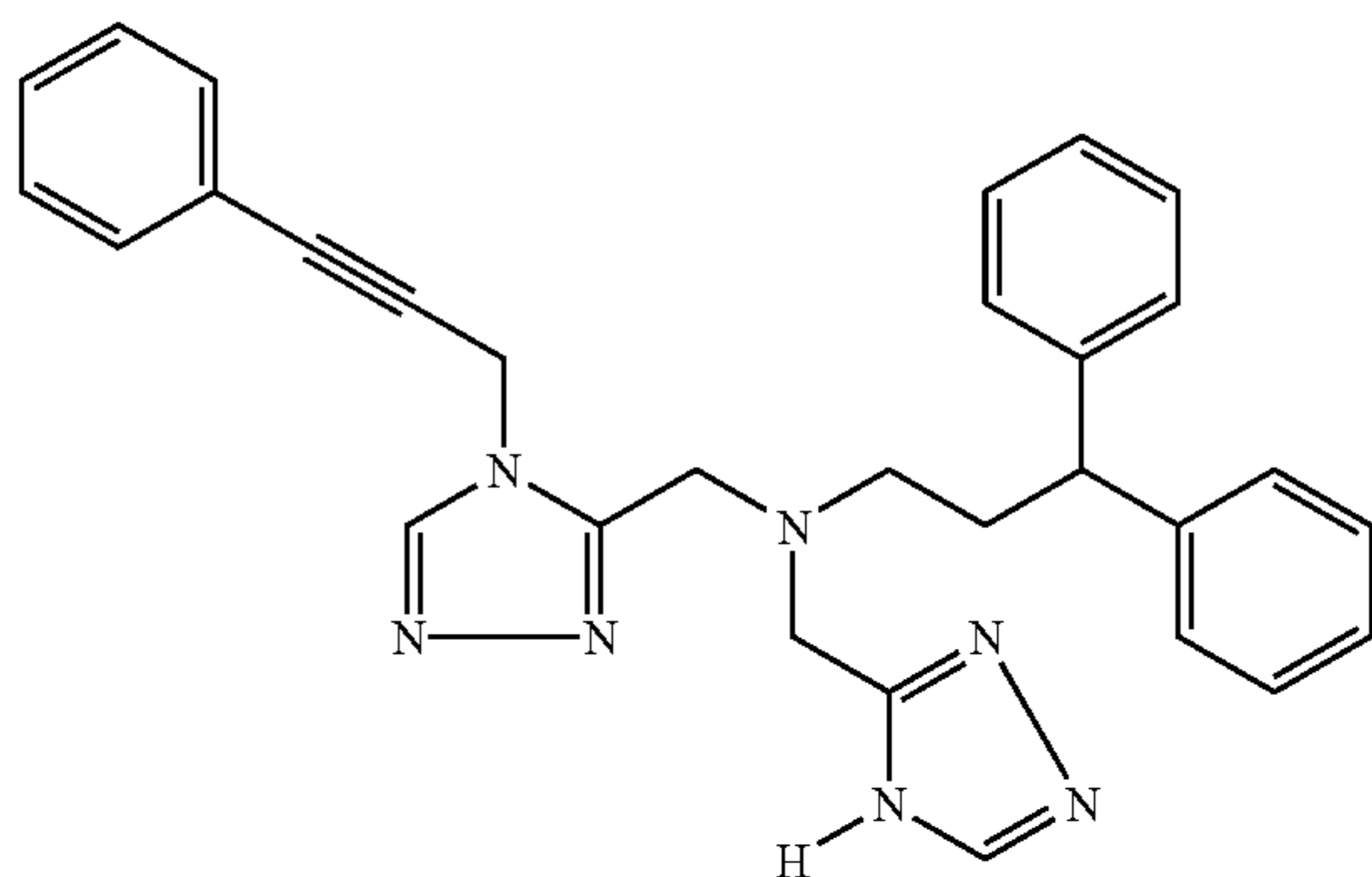
Trifluoroacetate (1:1) comp. 41.
