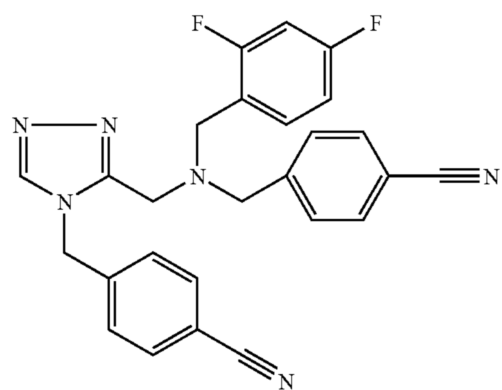
Trifluoroacetate (1:1) comp. 83.
