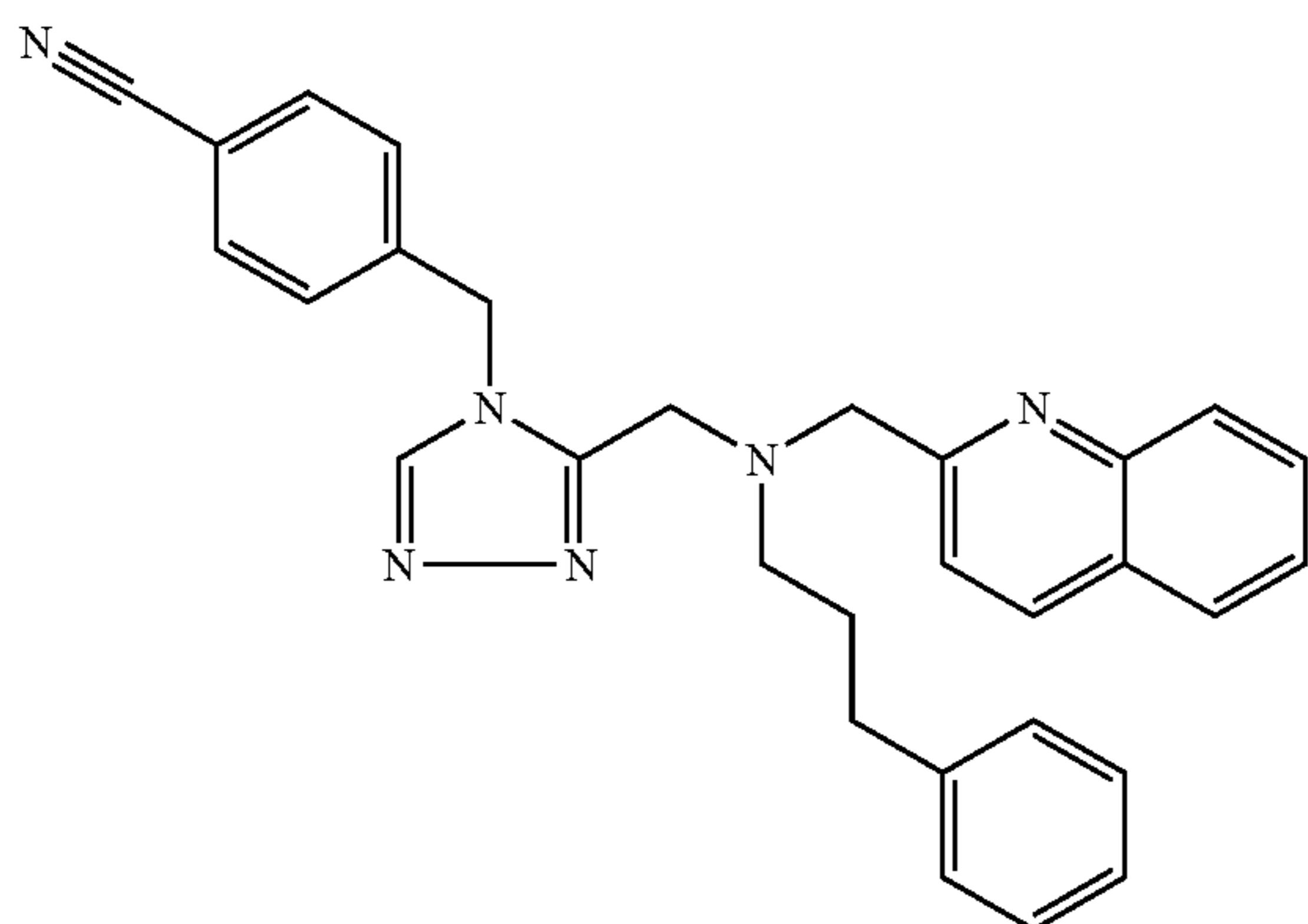
Trifluoroacetate (1:2) comp. 176.
