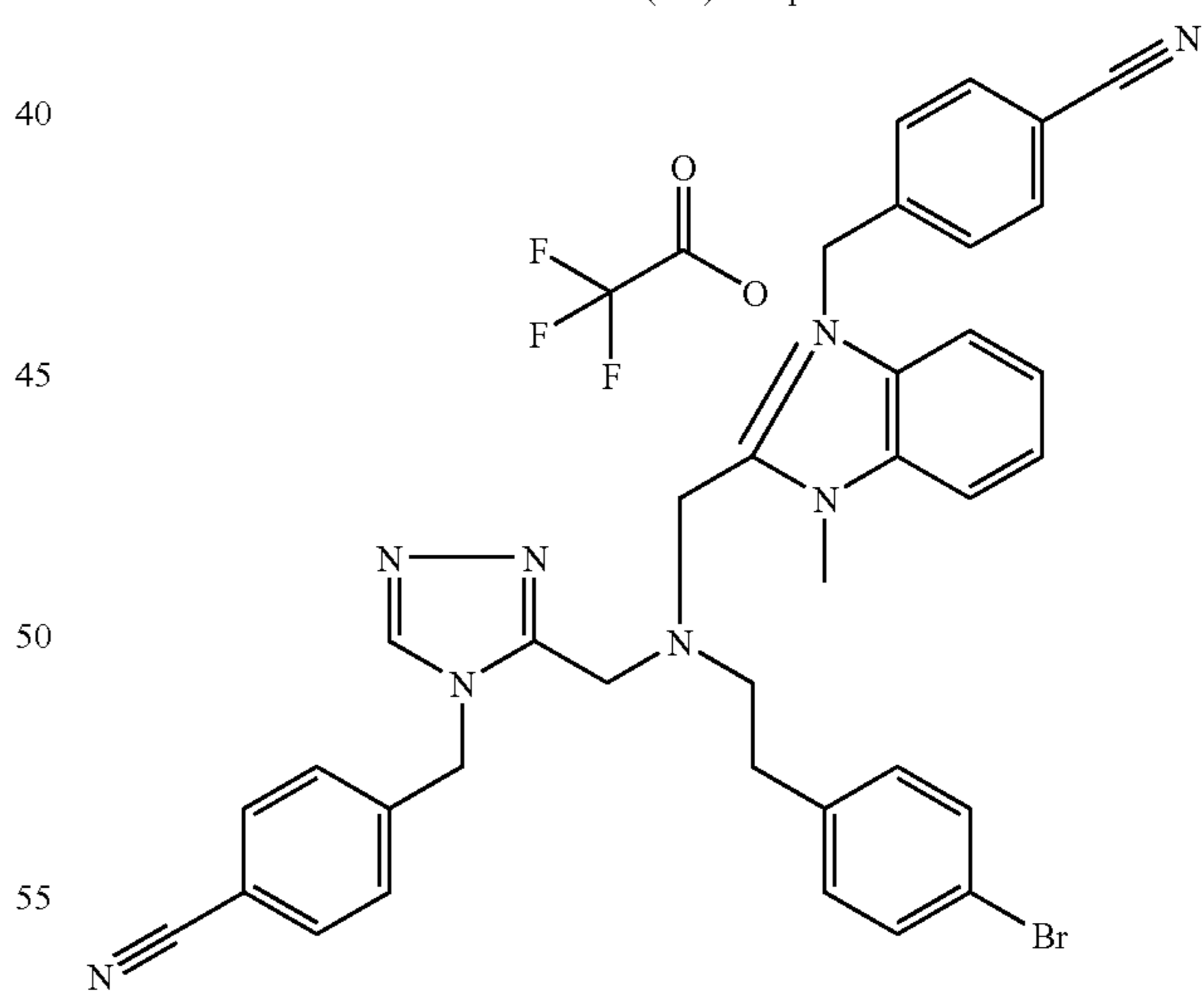
Trifluoroacetate (1:1) comp. 155.
