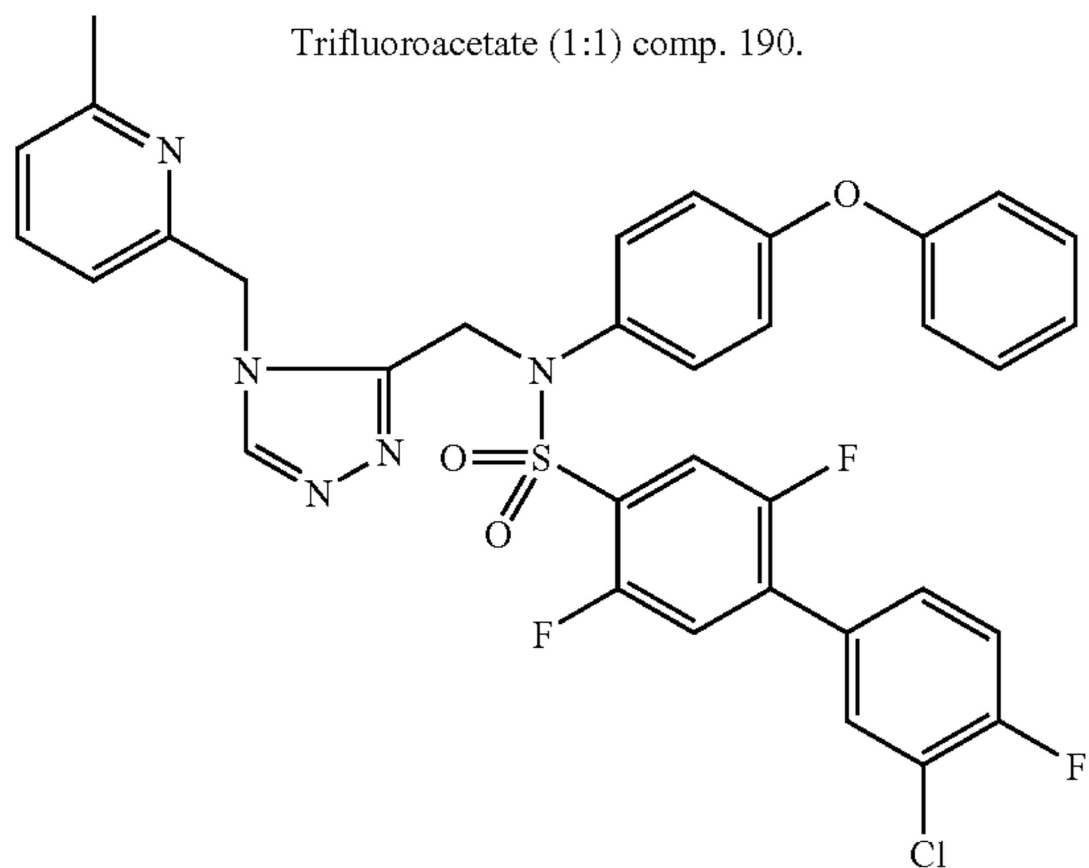
Trifluoroacetate (1:1) comp. 191.
