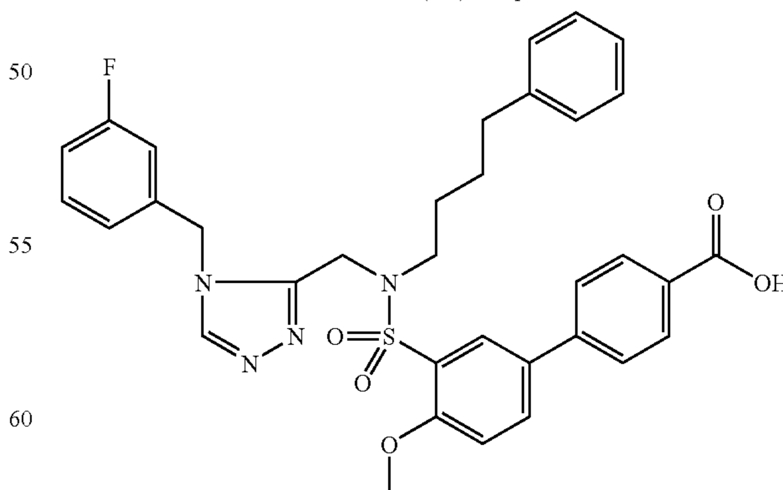
Trifluoroacetate (1:1) comp. 209.
