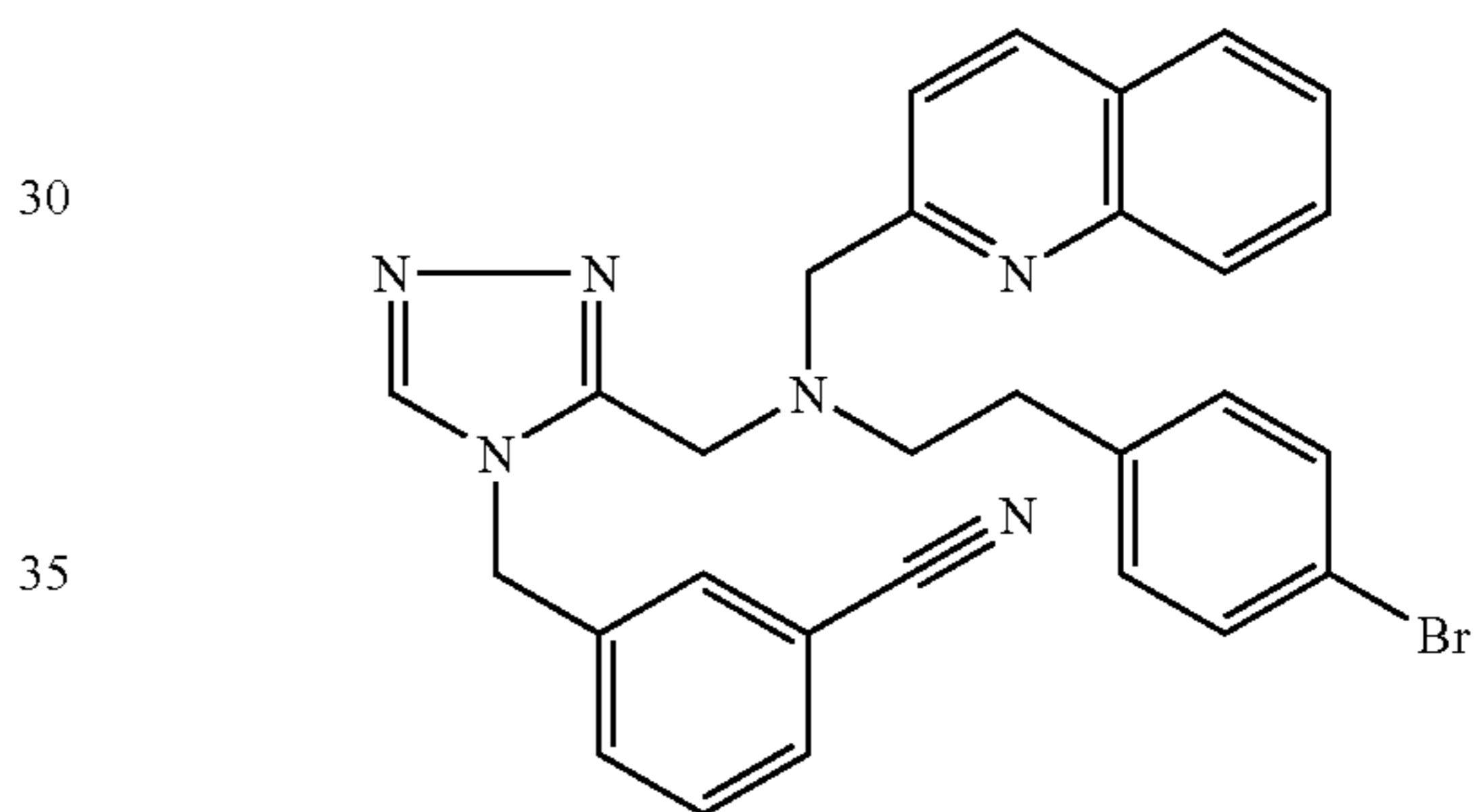
Trifluoroacetate (1:1) comp. 102.
