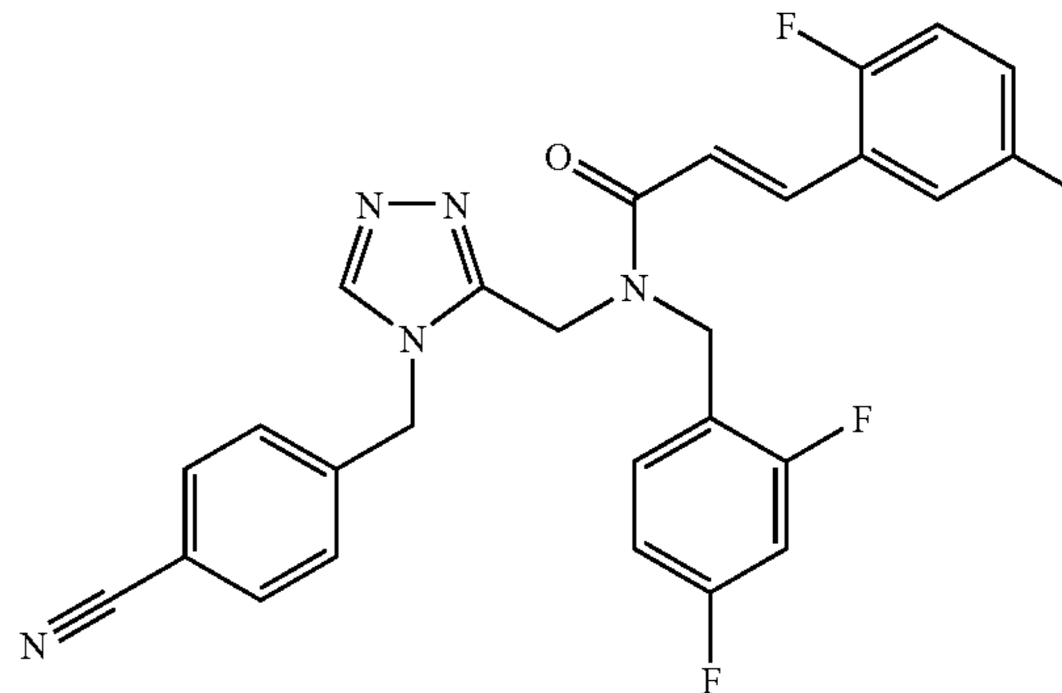
Trifluoroacetate (1:1) comp. 240.
