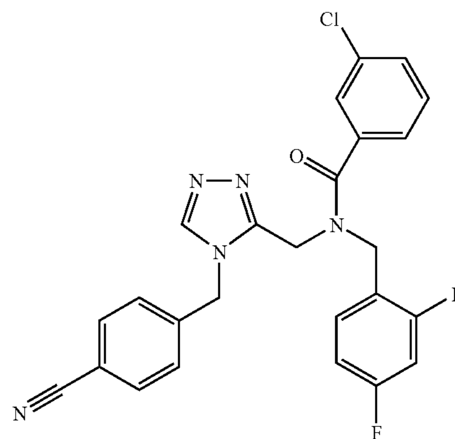
Trifluoroacetate (1:1) comp. 246.
