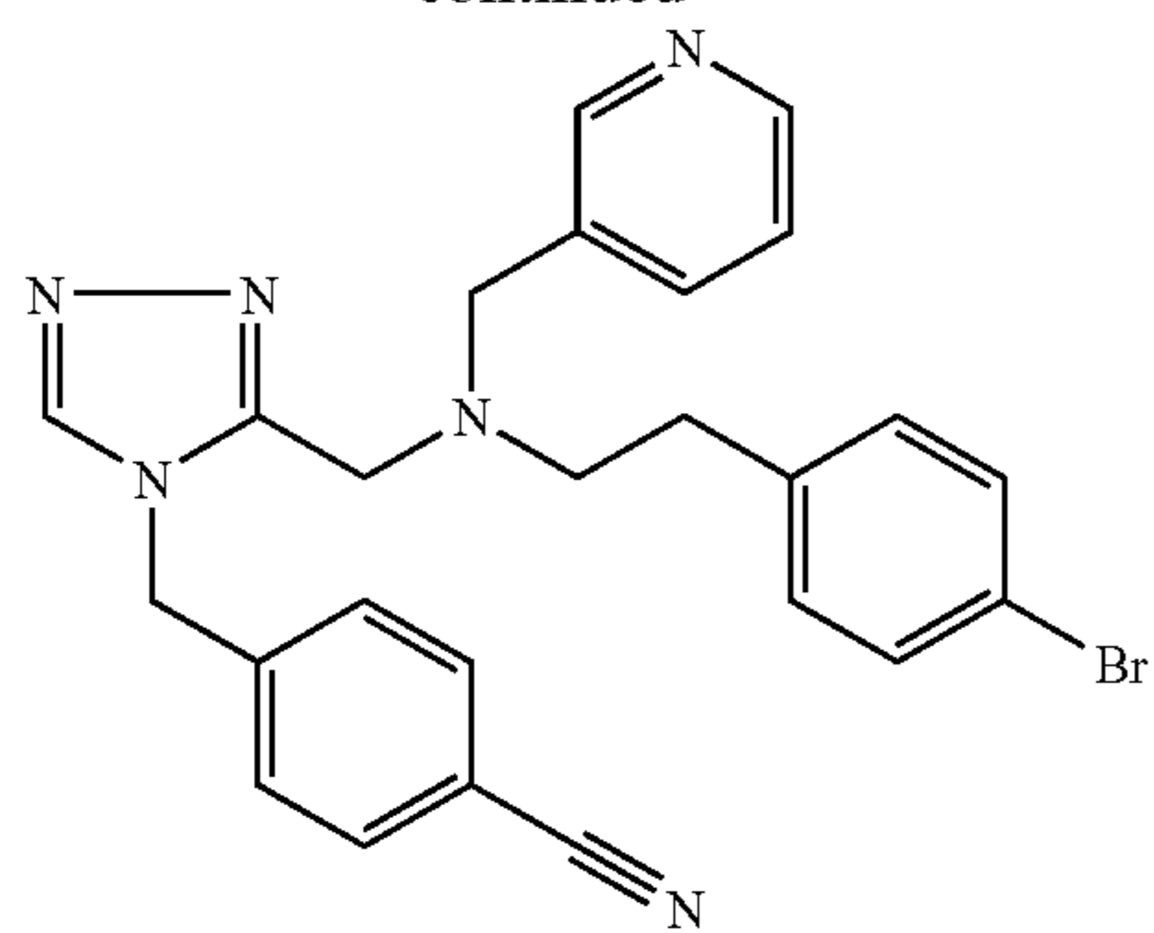
Trifluoroacetate (1:1) comp. 105.
