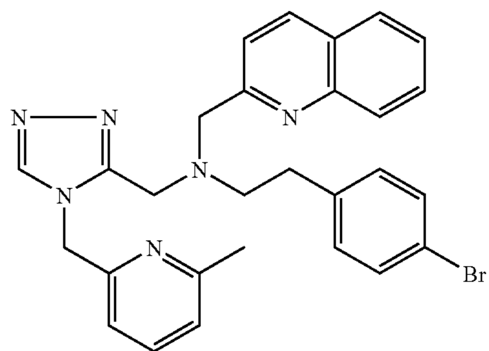
Trifluoroacetate (1:1) comp. 180.
