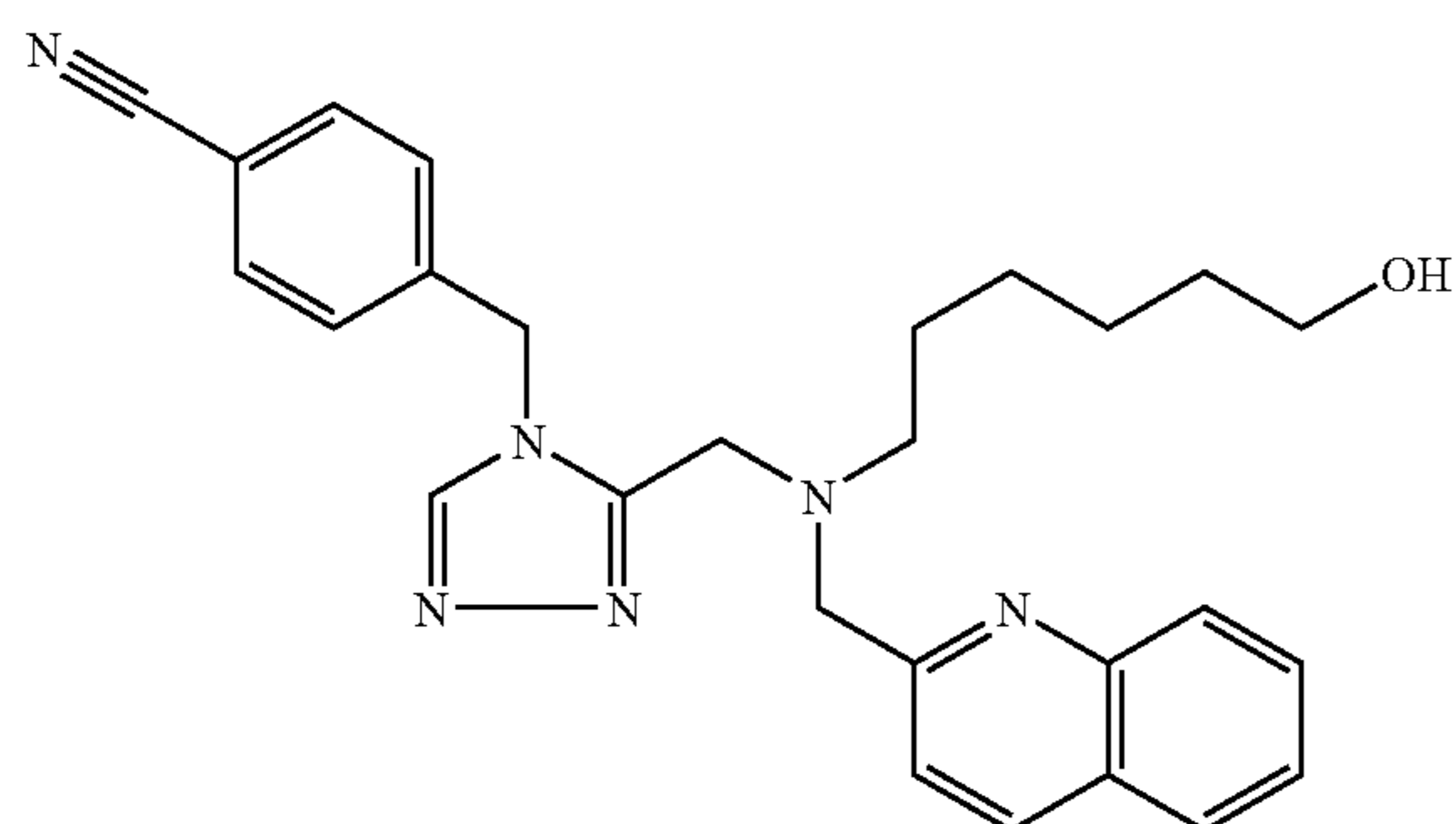
Trifluoroacetate (1:1) comp. 124.
