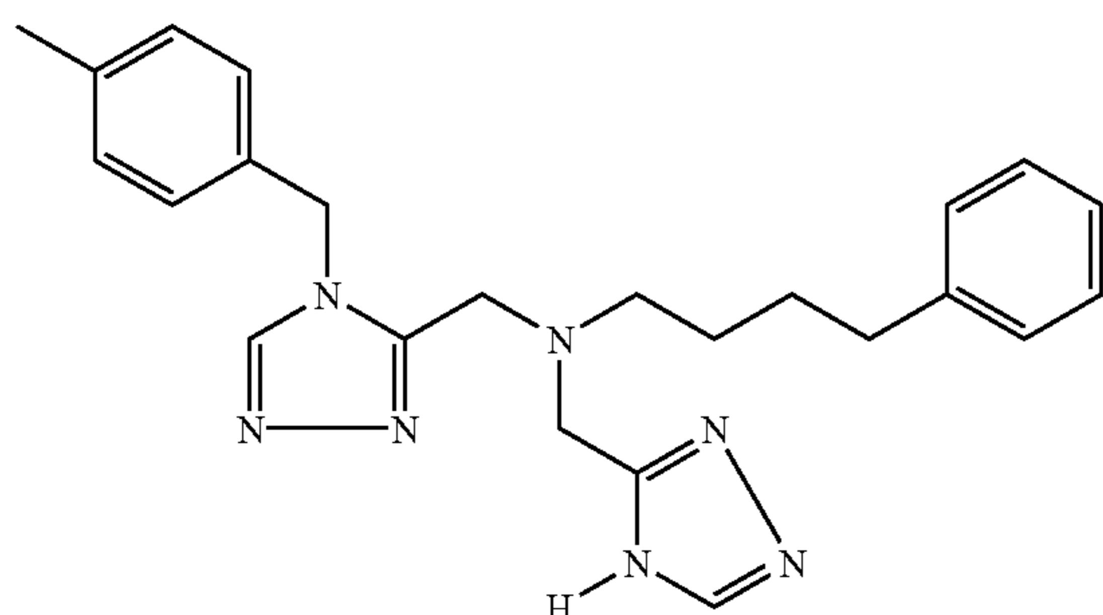
Trifluoroacetate (1:1) comp. 33.
