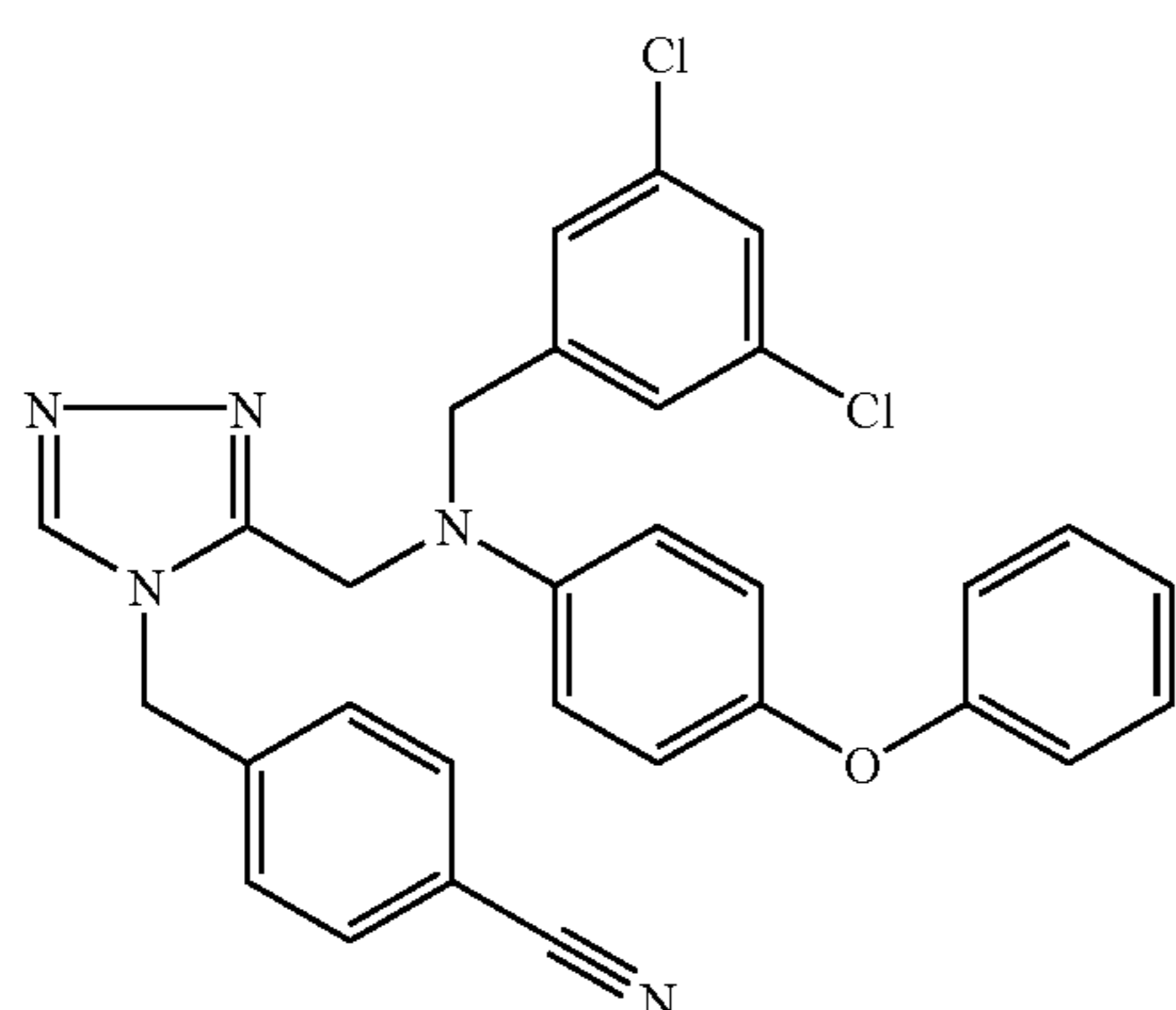
Trifluoroacetate (1:1) comp. 56.
