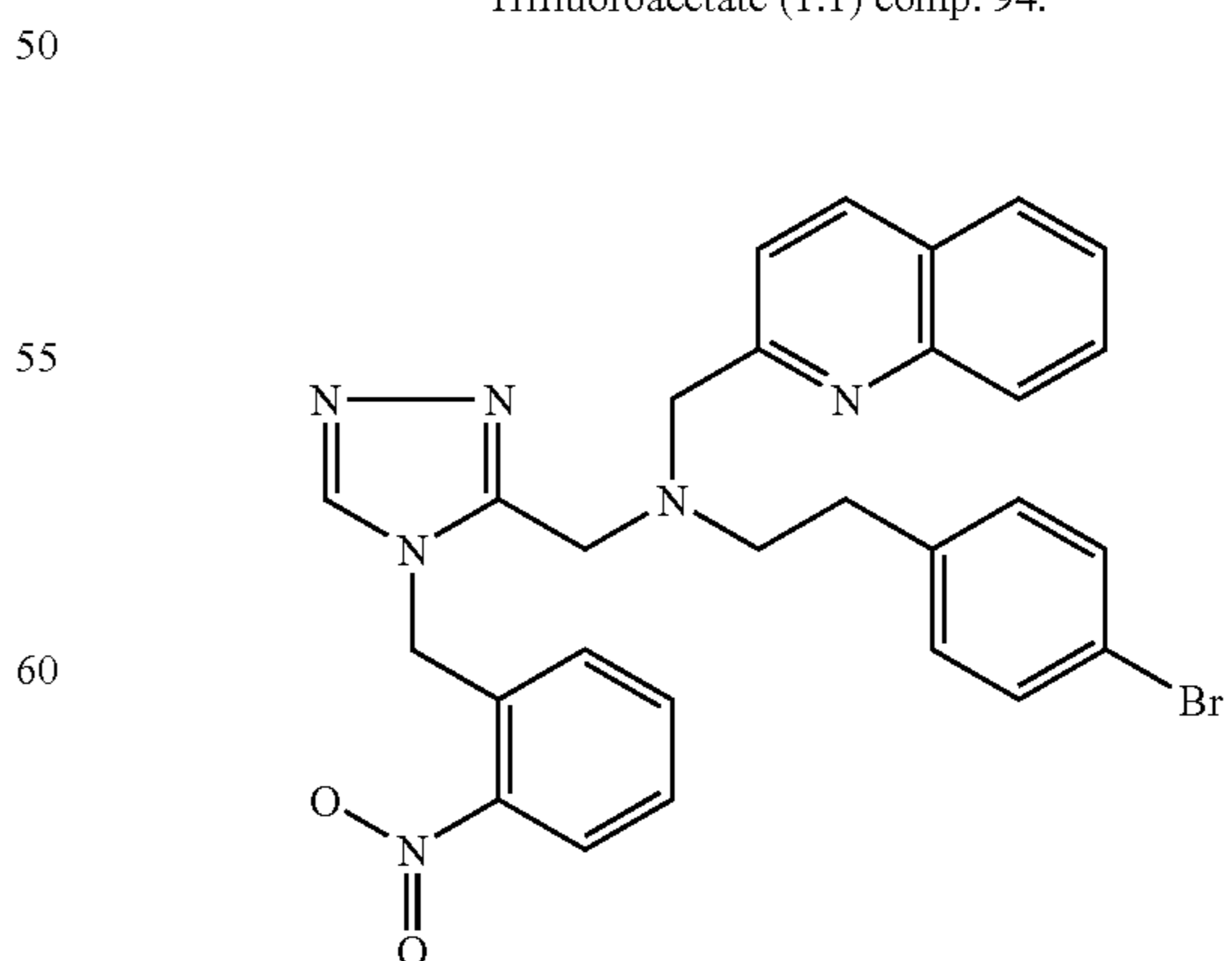
Trifluoroacetate (1:1) comp. 95.
