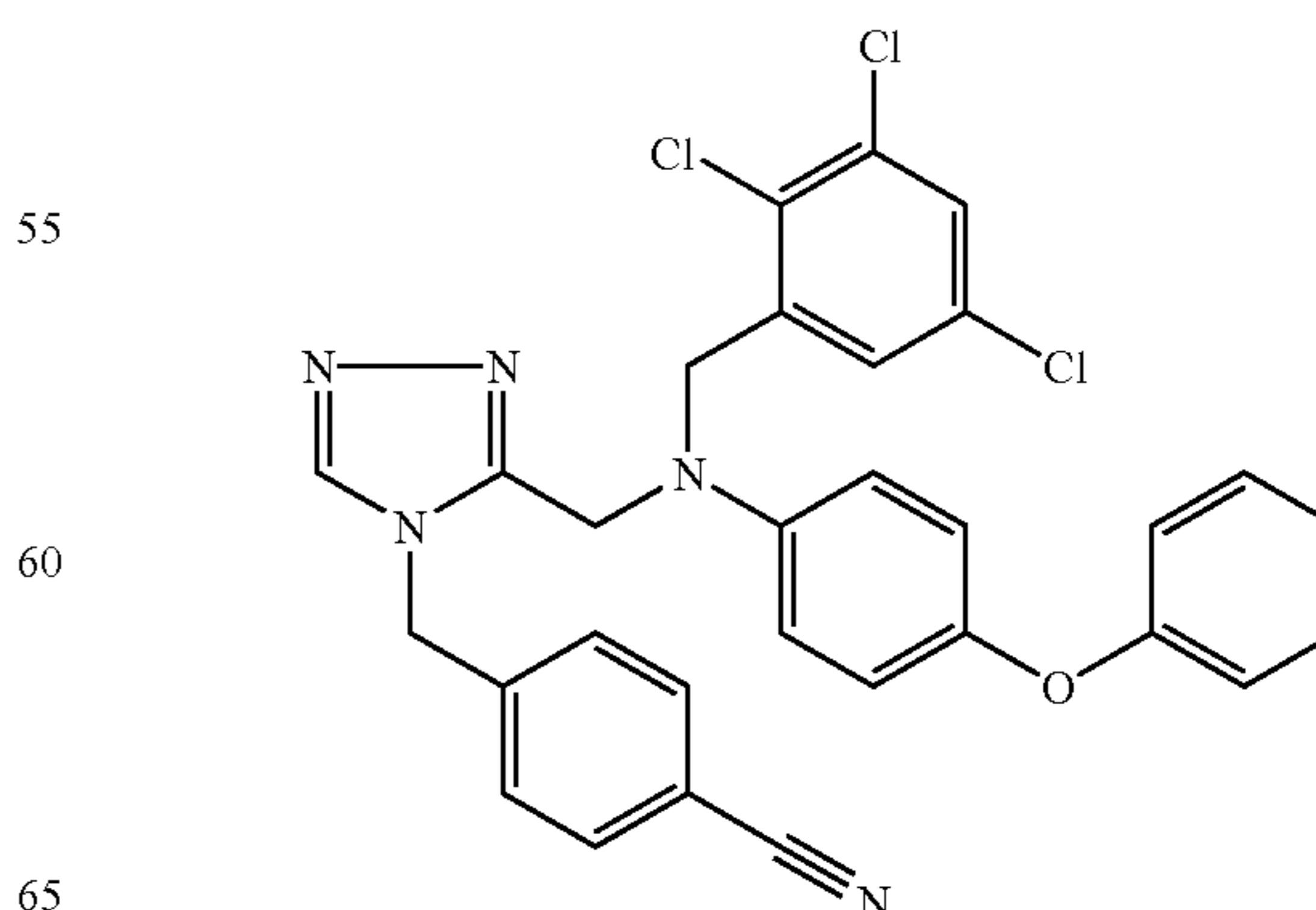
Trifluoroacetate (1:1) comp. 63.
