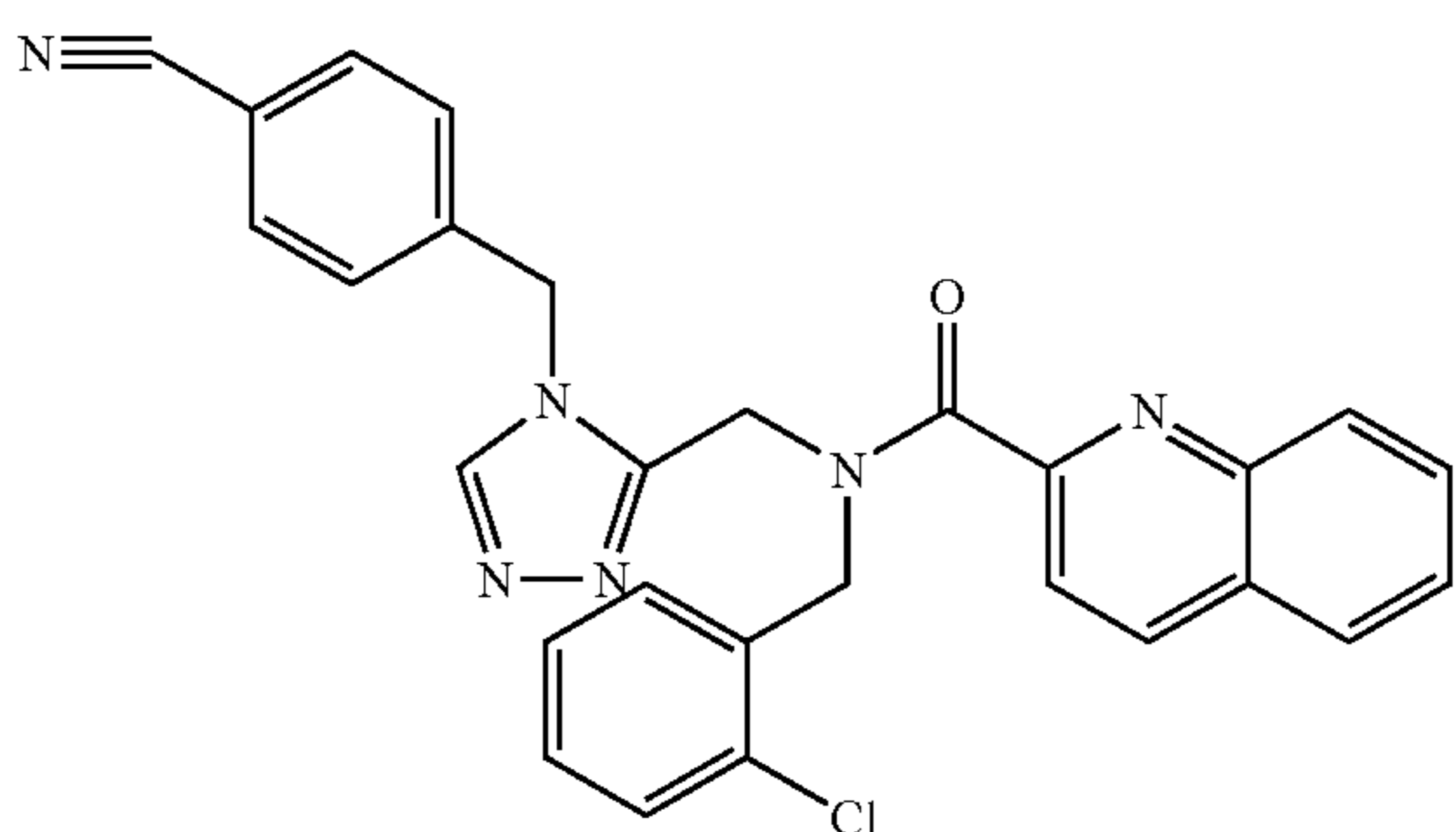
Trifluoroacetate (1:1) comp. 294.
