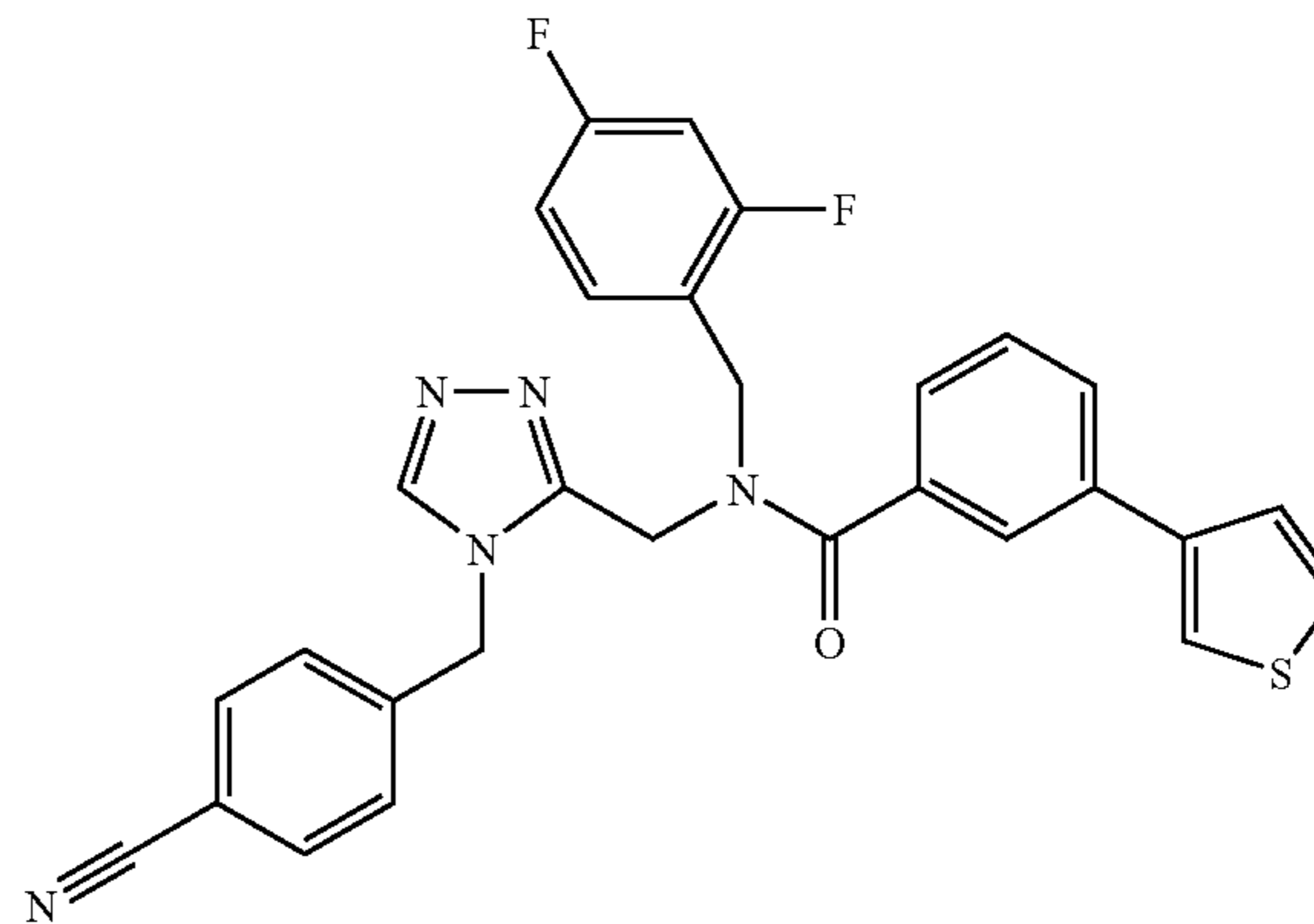
Trifluoroacetate (1:1) comp. 239.
