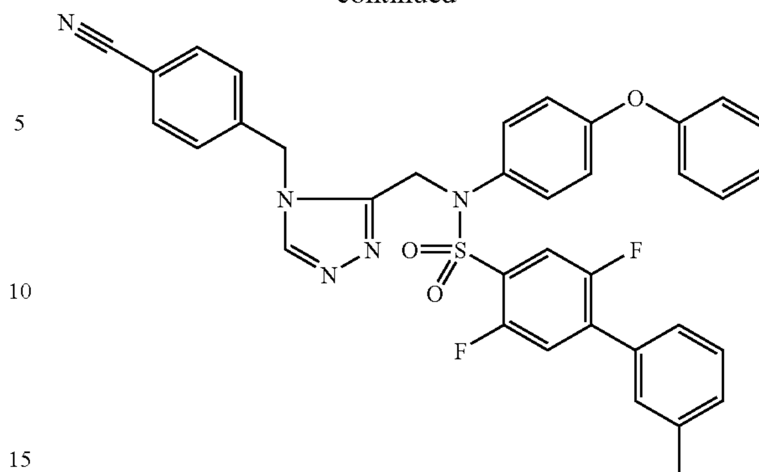
Trifluoroacetate (1:1) comp. 207.
