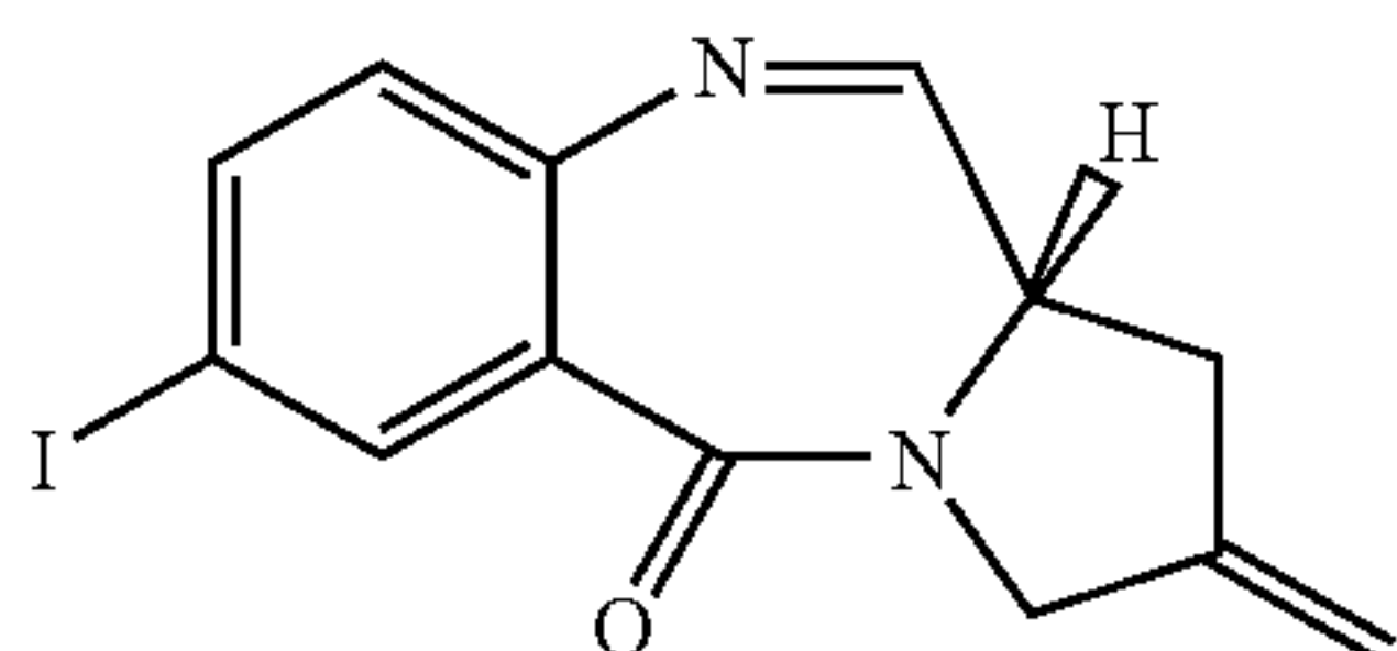
(S)-N-(Allyloxycarbonyl)-2-(tert-butyl dimethylsilyloxymethyl)-4-methylidenepyrrolidine (57)
