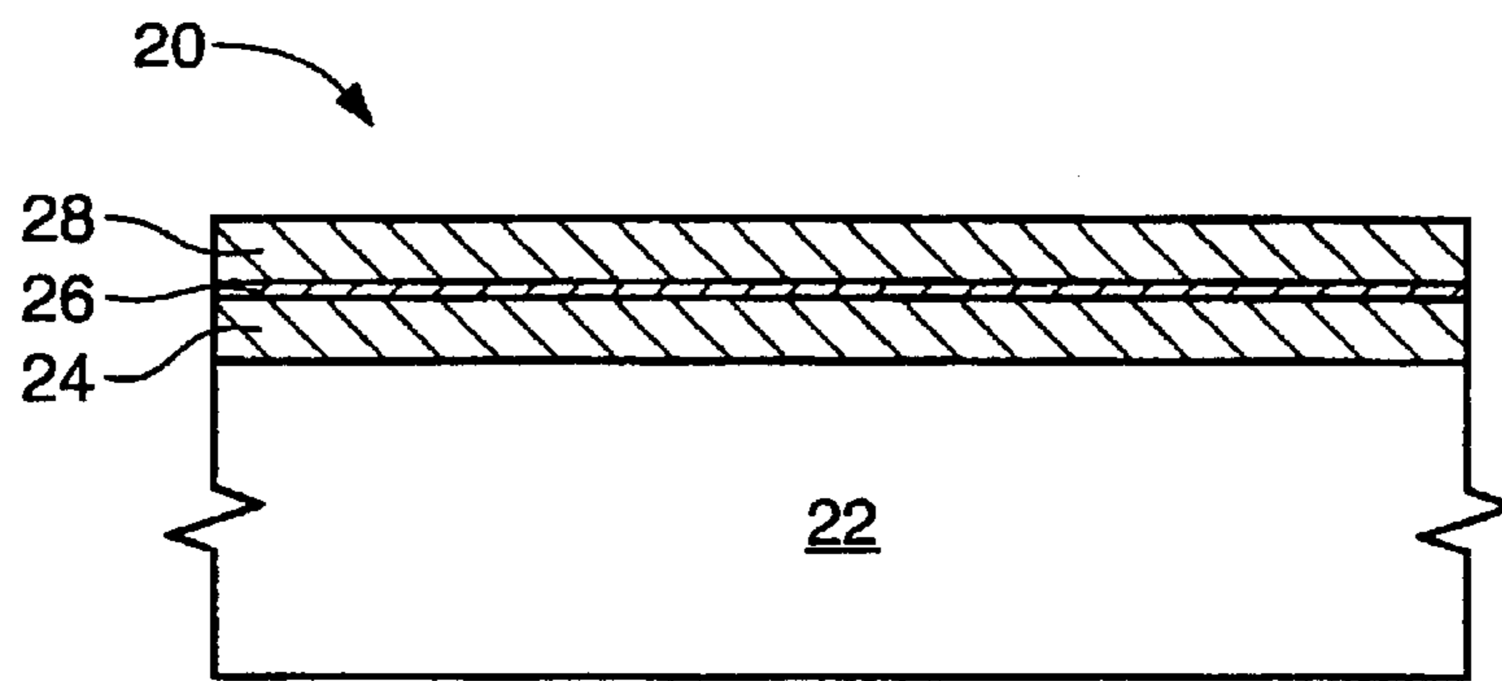
FIG. 1 (PRIOR ART)
