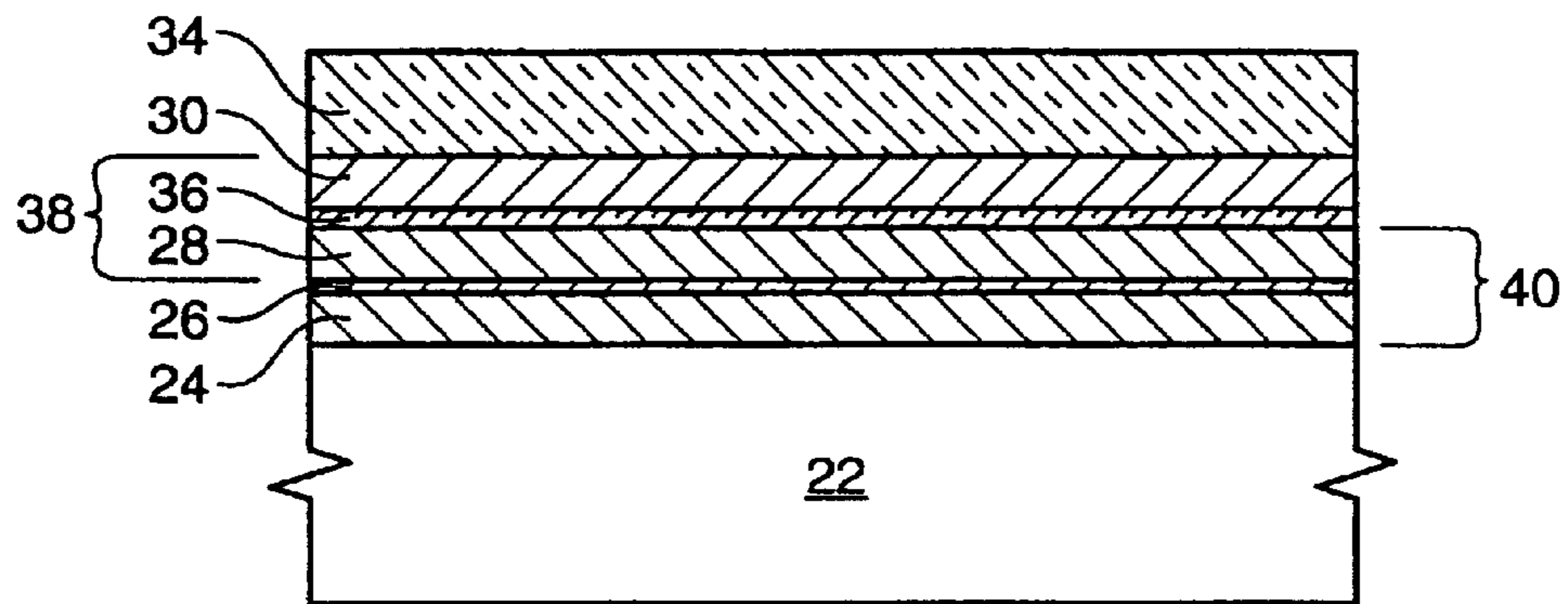
FIG. 3 (PRIOR ART)
