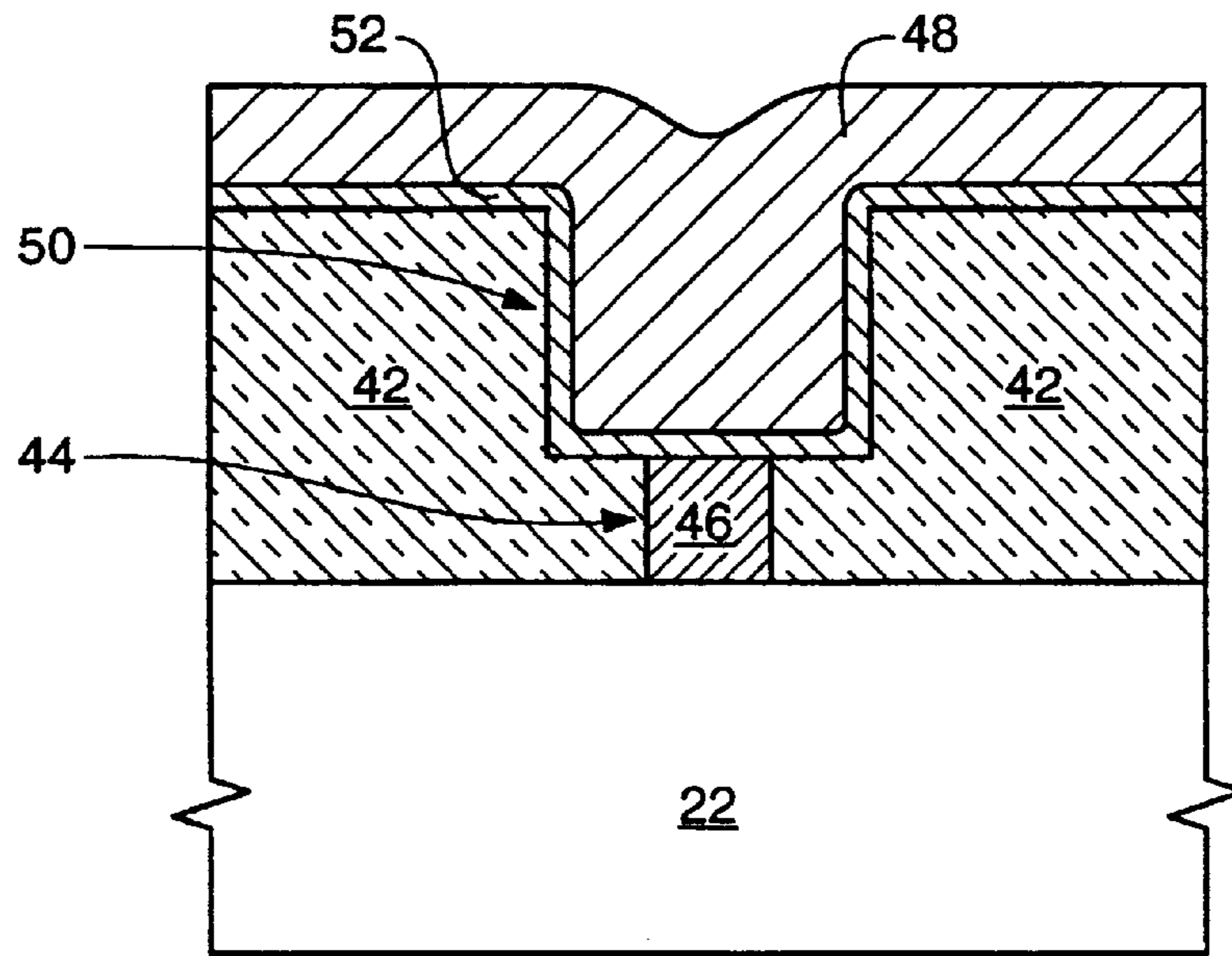
FIG. 7 (PRIOR ART)
