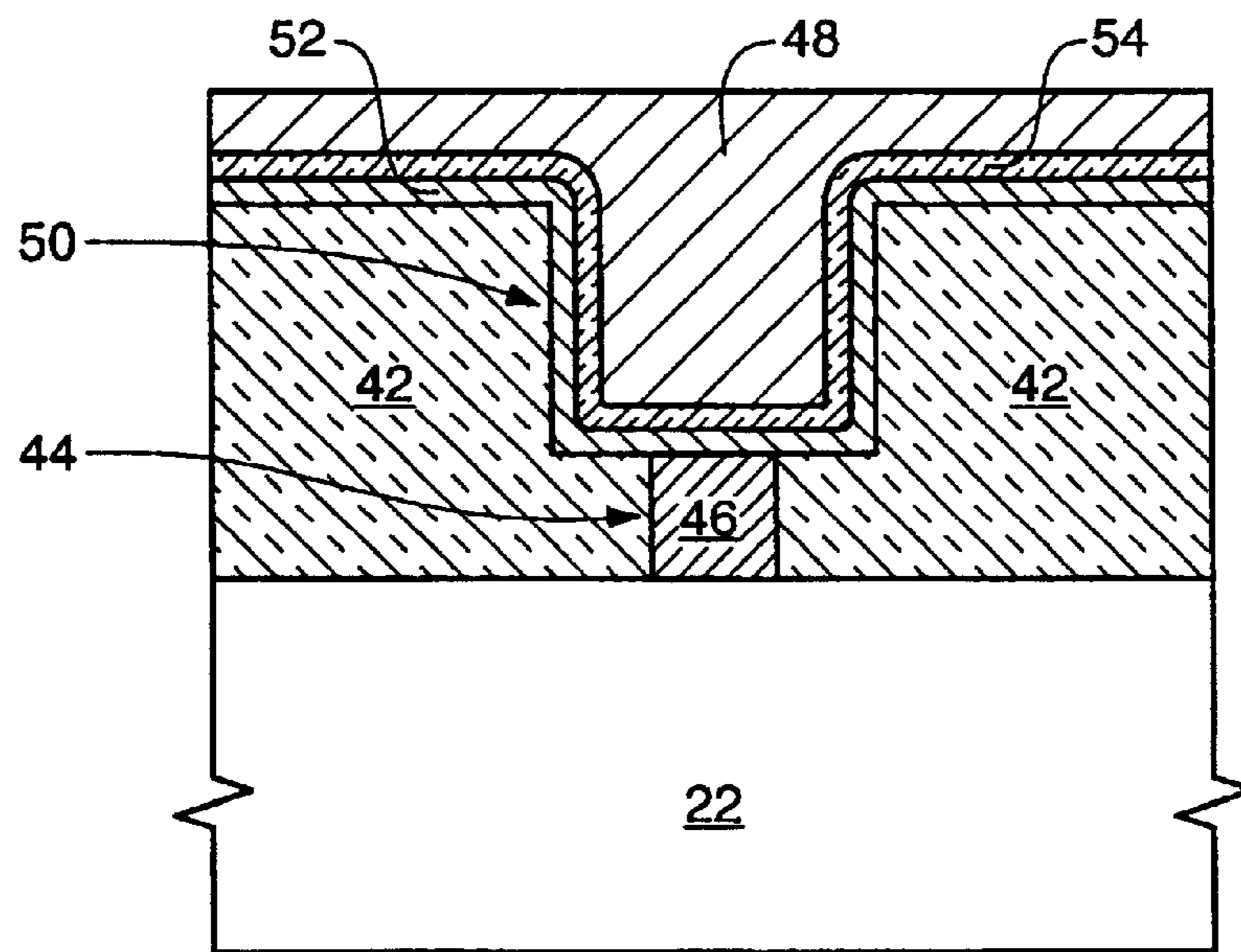
FIG. 8 (PRIOR ART)
