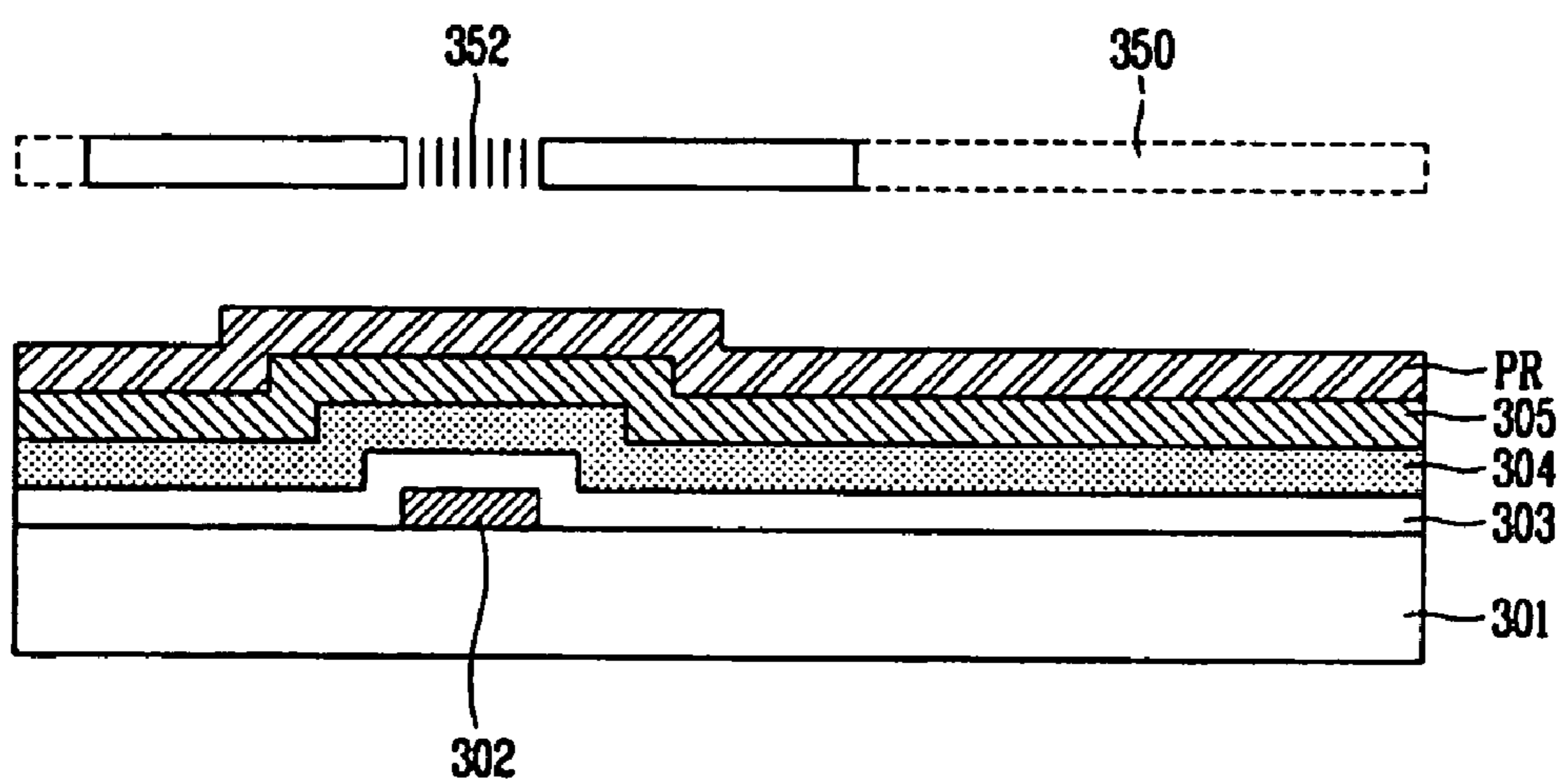
FIG. 3D
