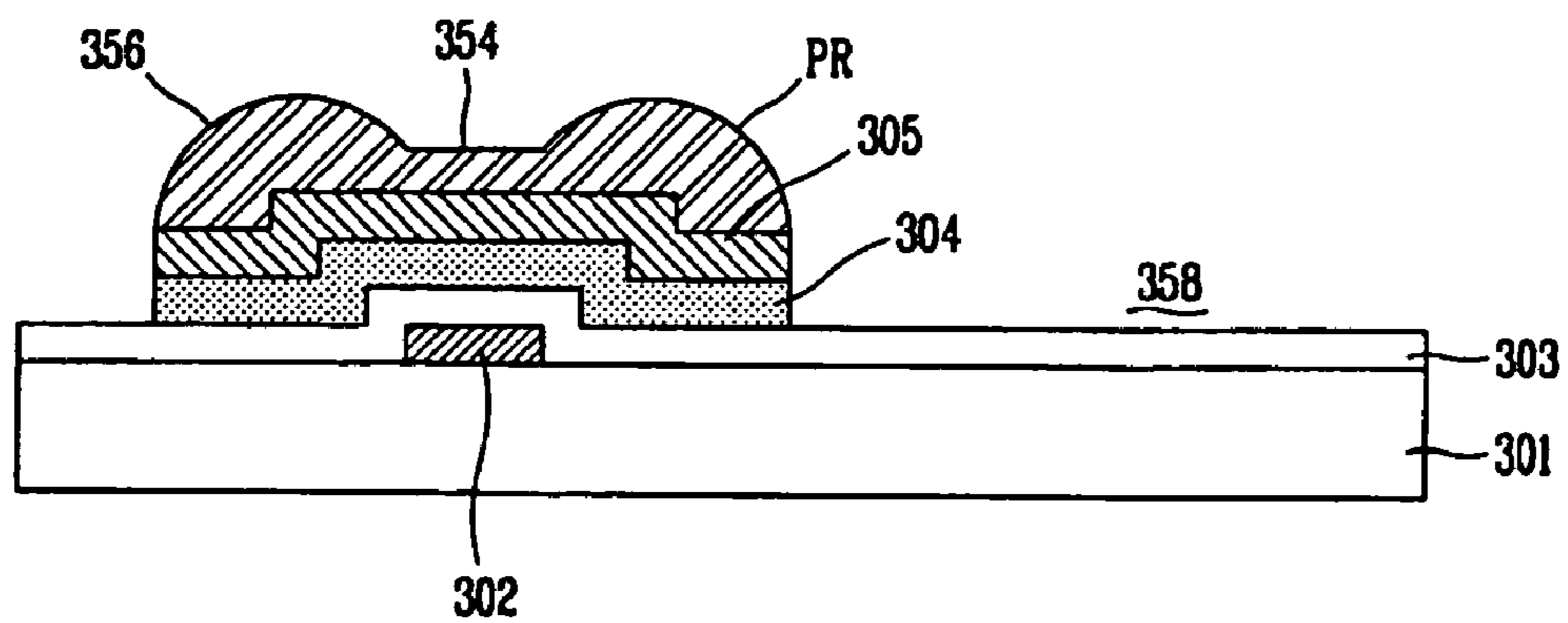
FIG. 3D
