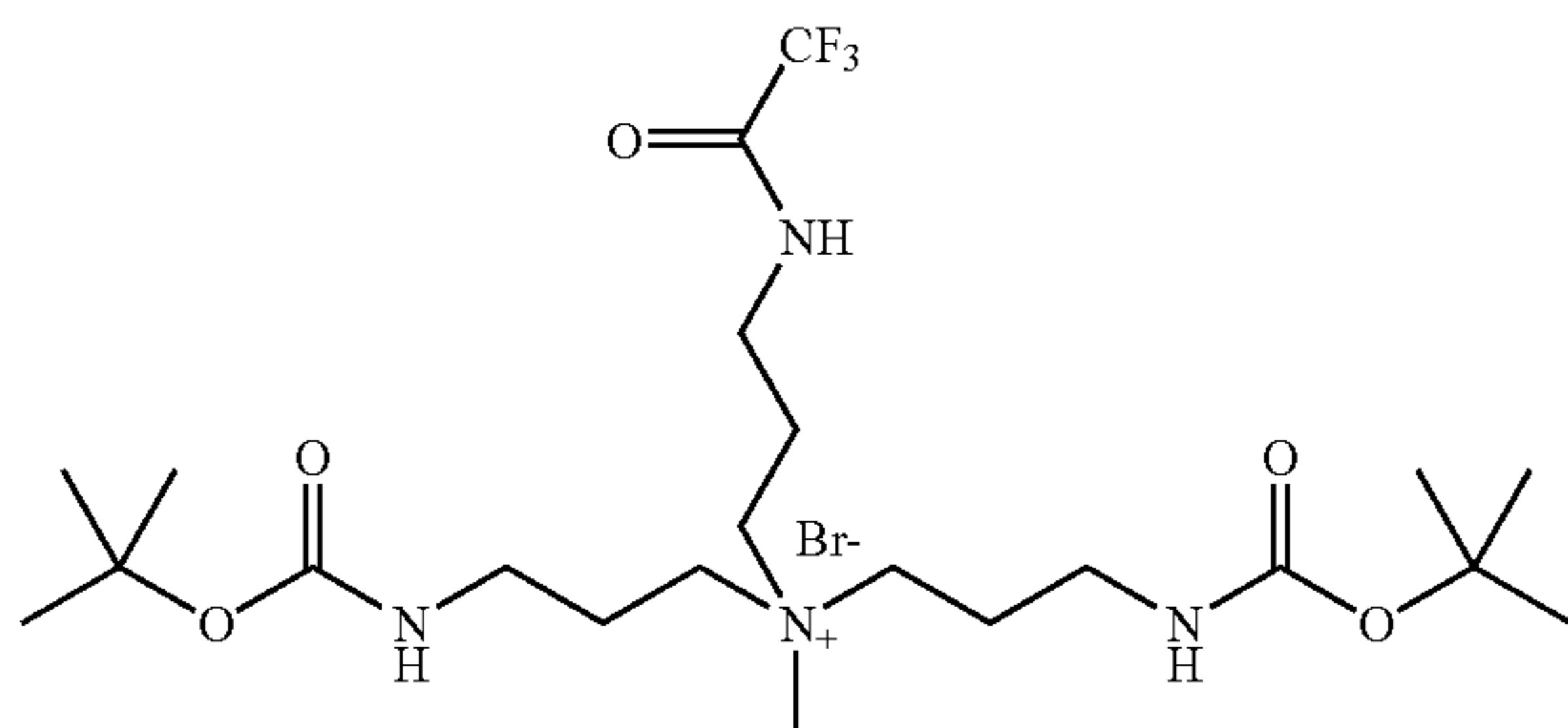
Compound 13
