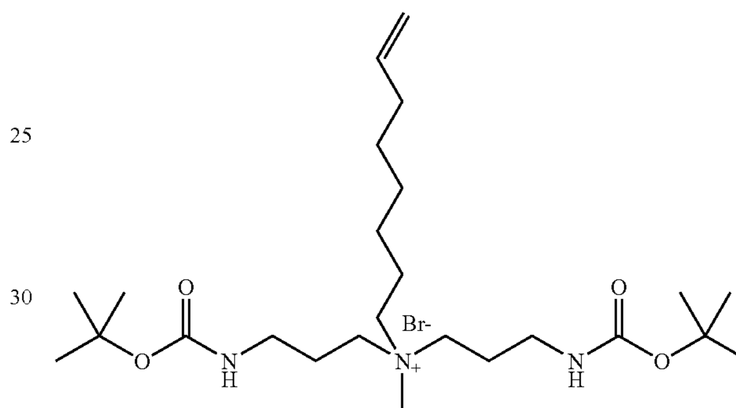
Compound 6
