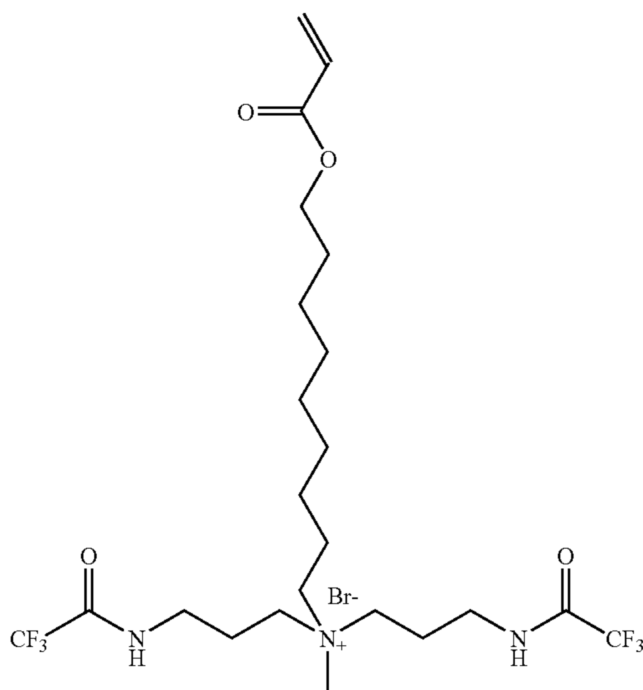
Compound 12
