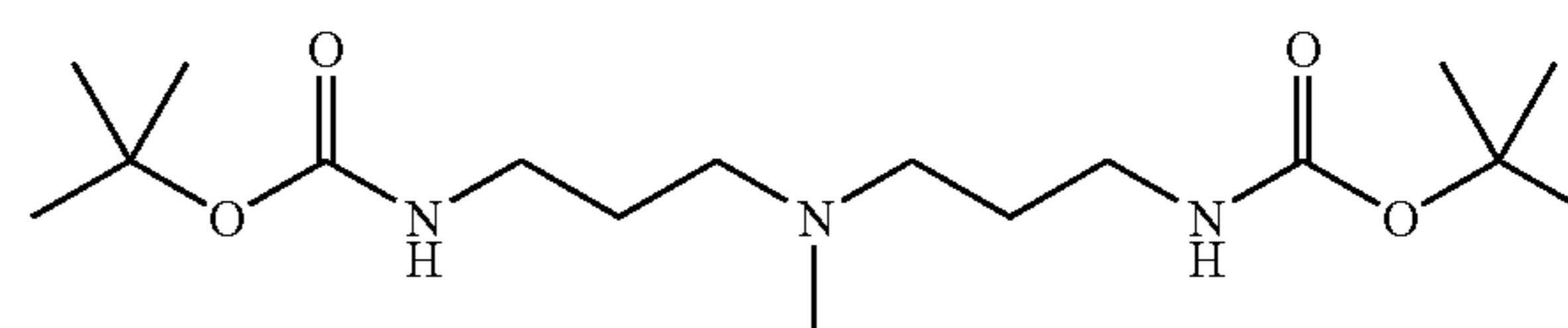
Compound 1
