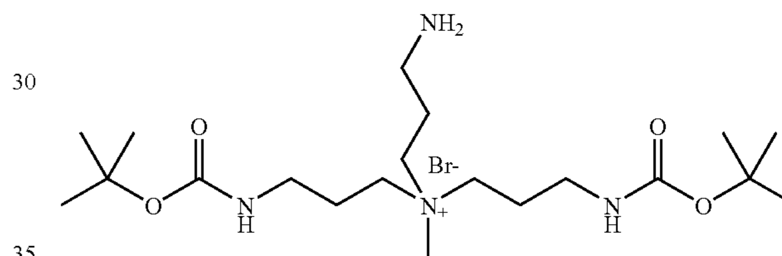
Compound 14
