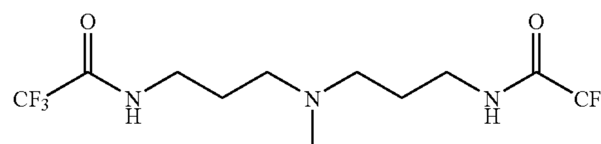
Compound 2
