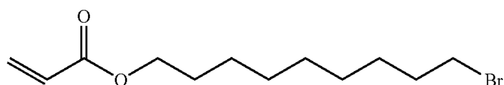
Compound 3
